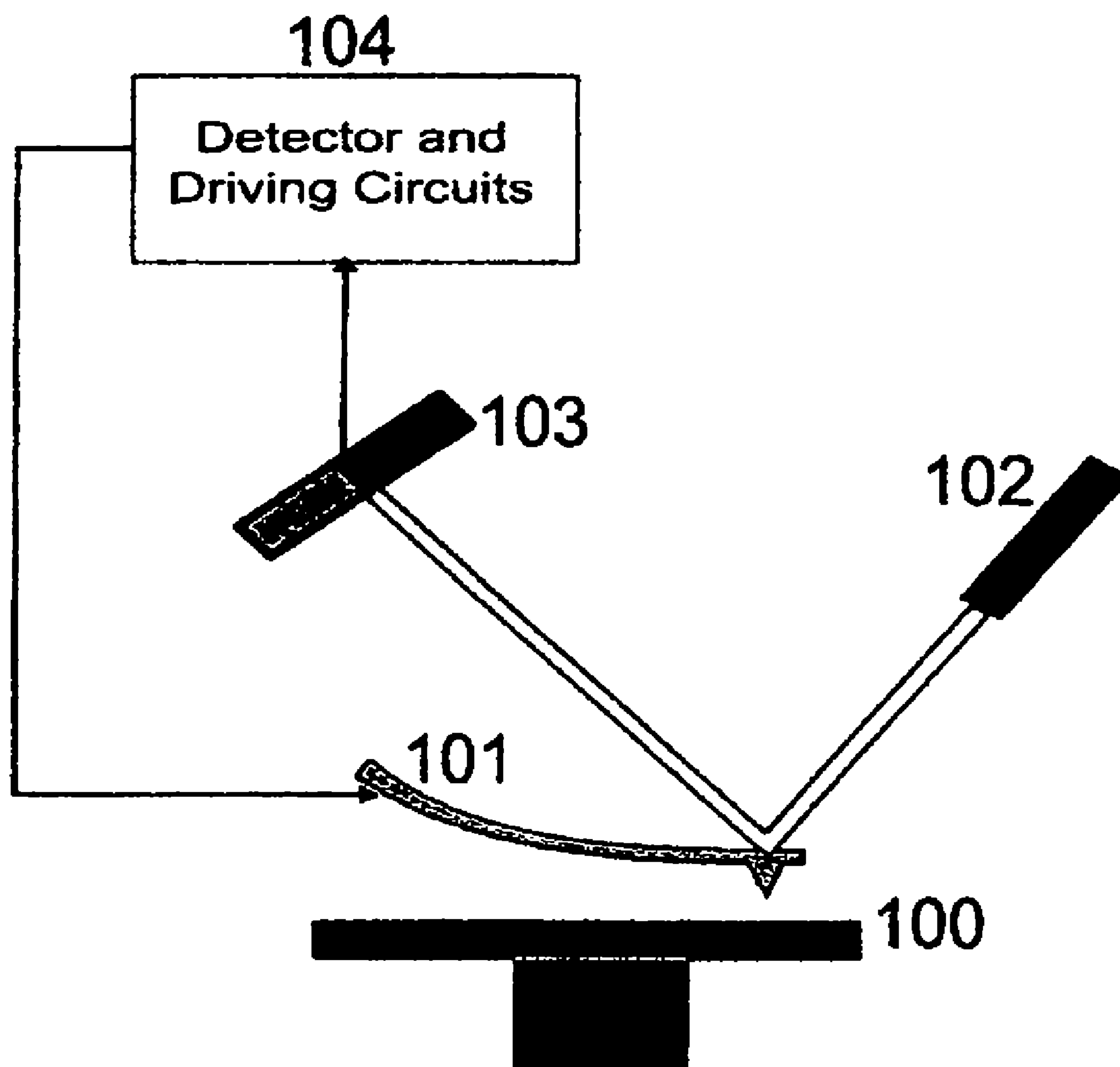
Fig. 1 - Prior Art
