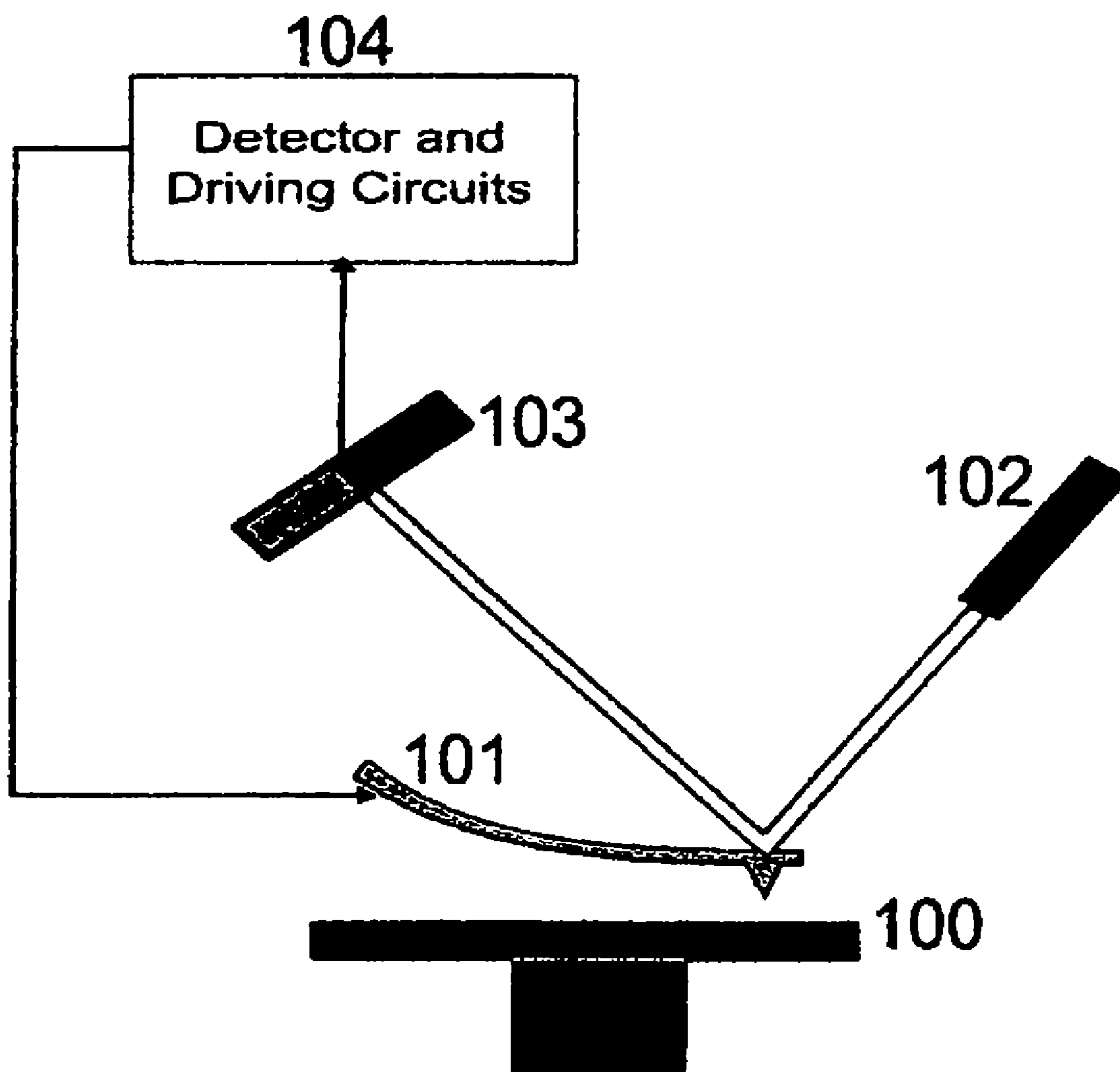
Fig. 1 - Prior Art
