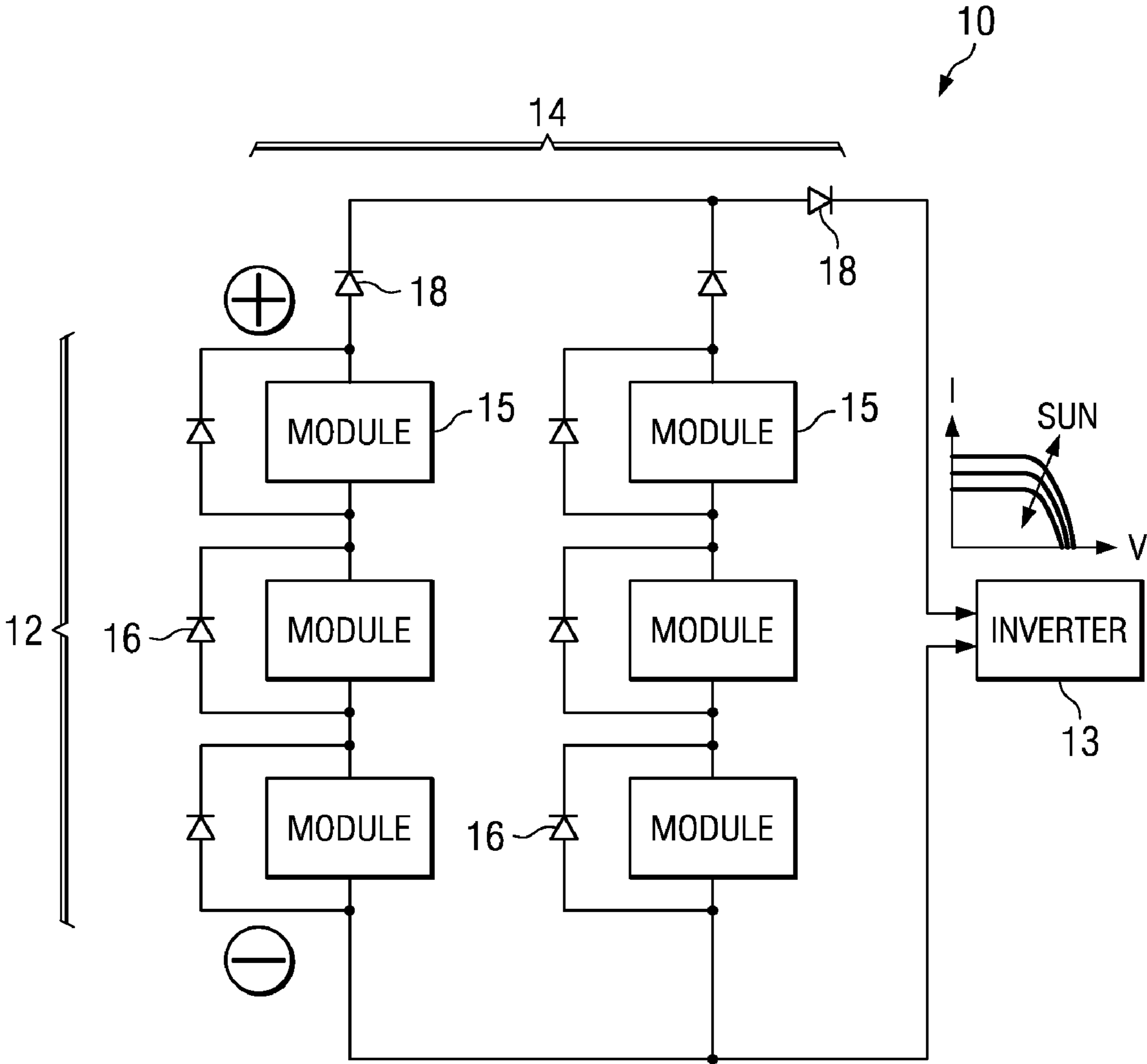
FIG. 1 (PRIOR ART)
