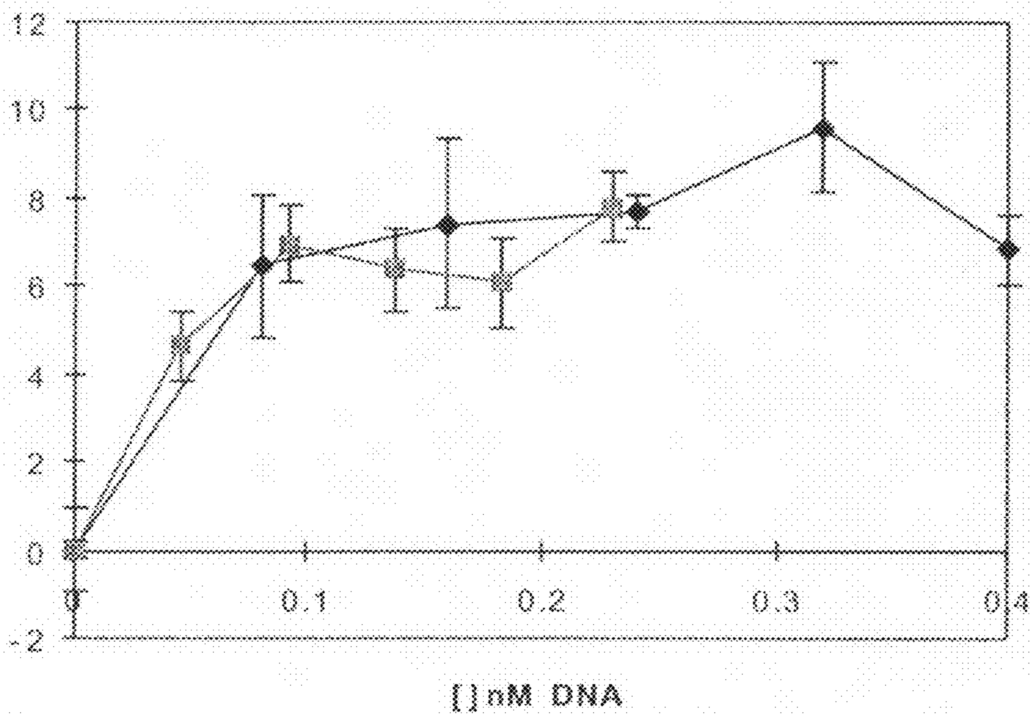
Expression of DHFR from genes in solution and on beads
