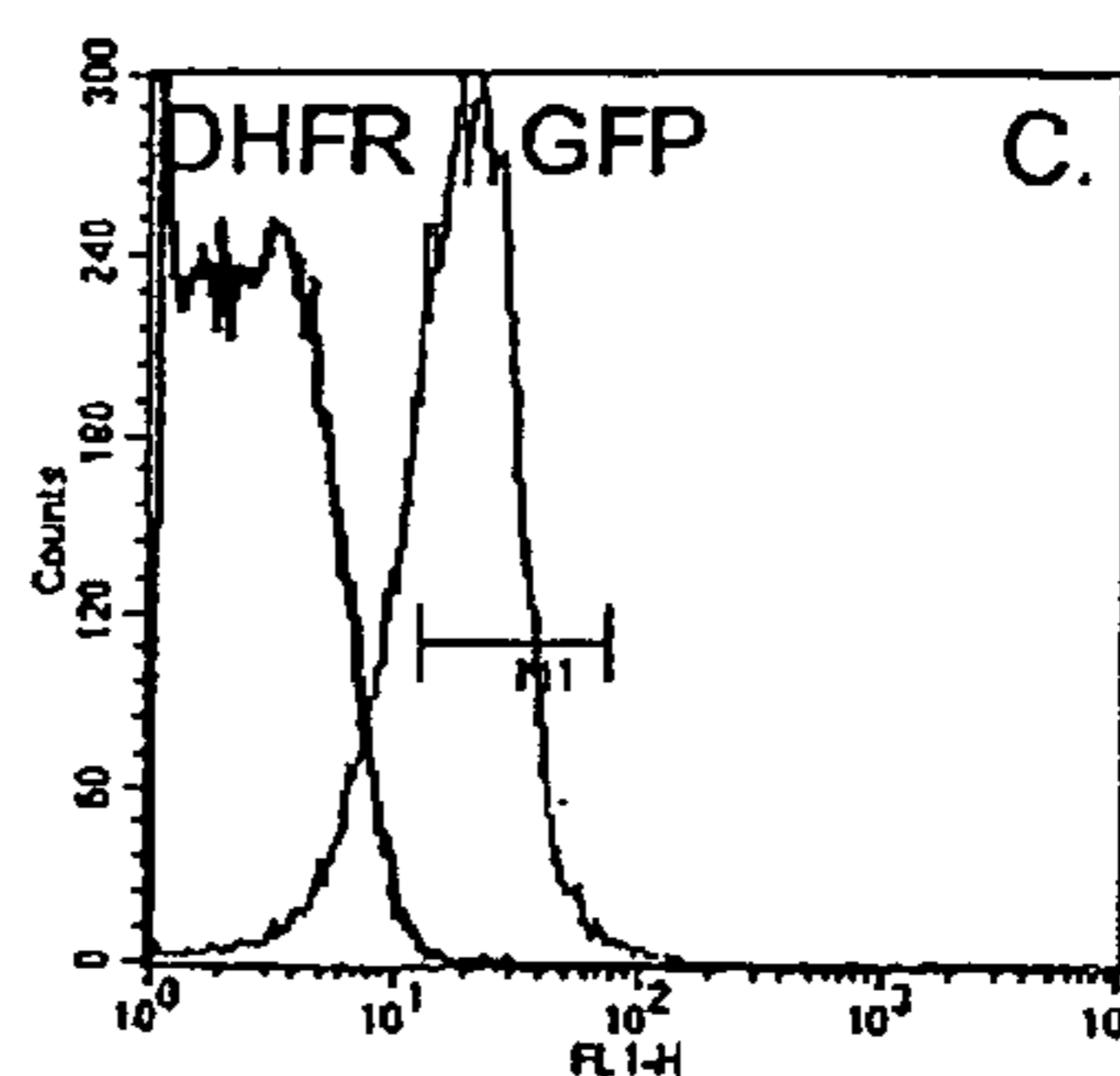
Fluorescence of beads recovered from emulsion
