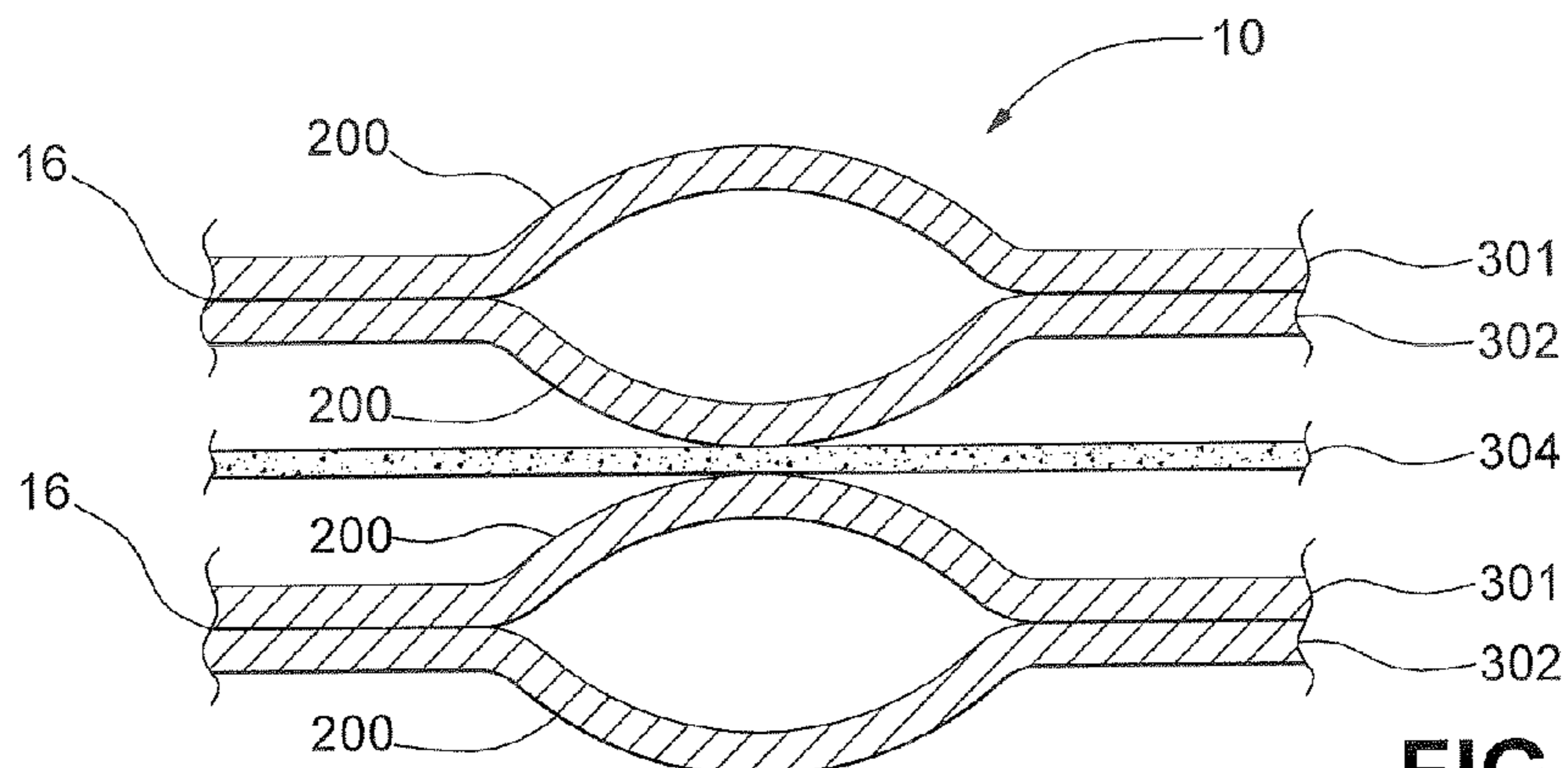
FIG. 2 (Prior Art)
