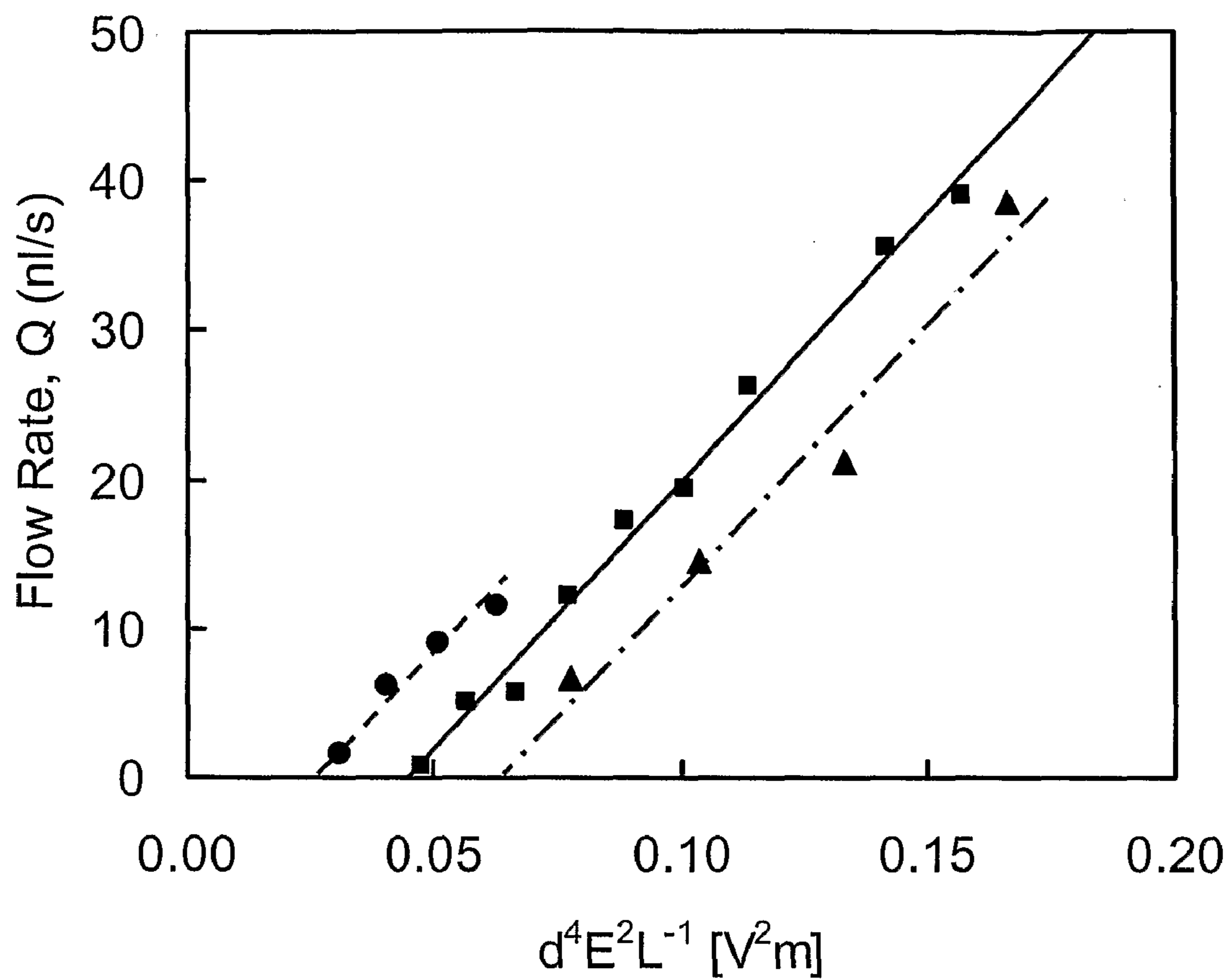
Figure 20: Flow rate of drop formation supporting Q \sim d^4 E^2 L^{-1} scaling law.
