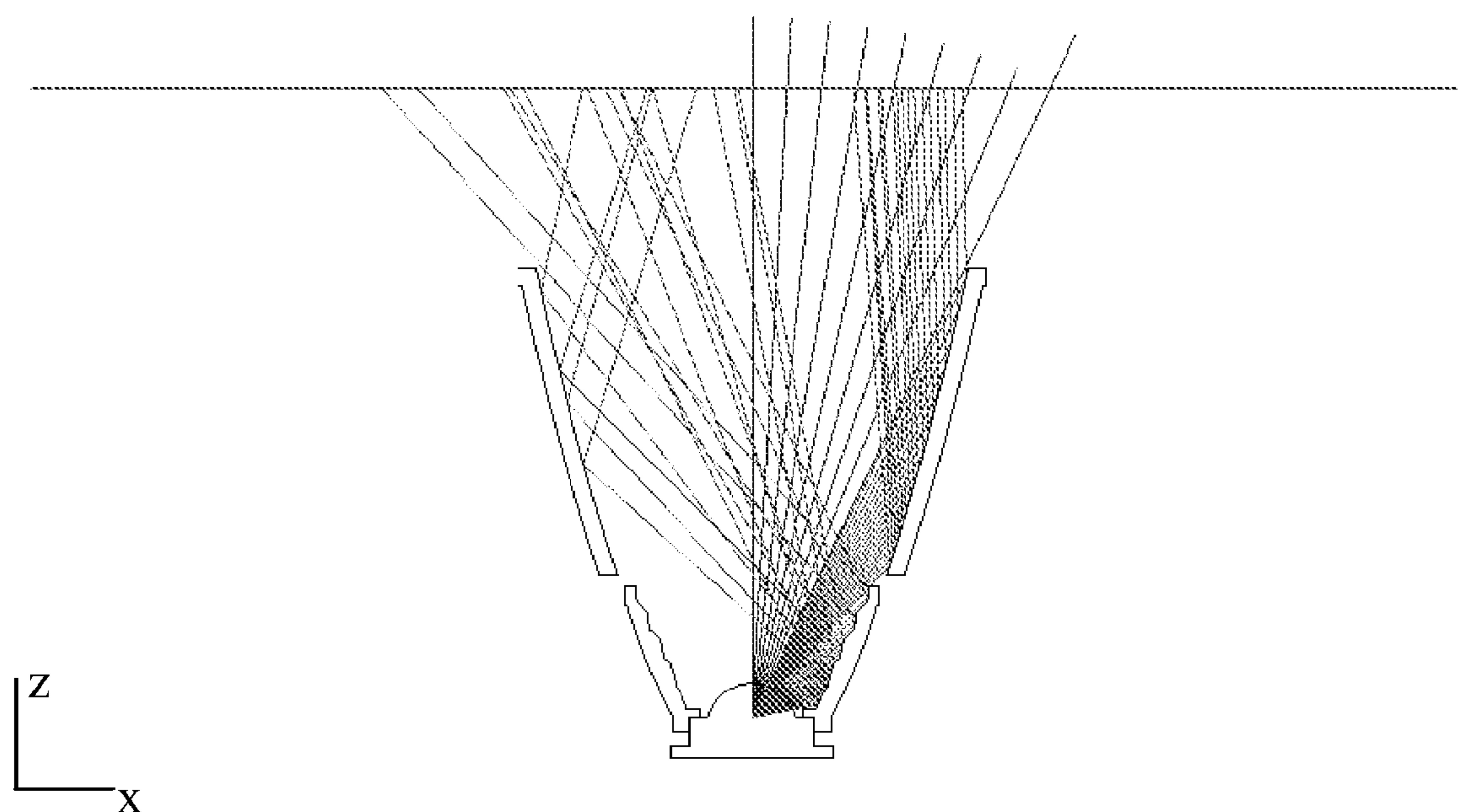
Figure 29: outer reflector (and inner) ray path details
