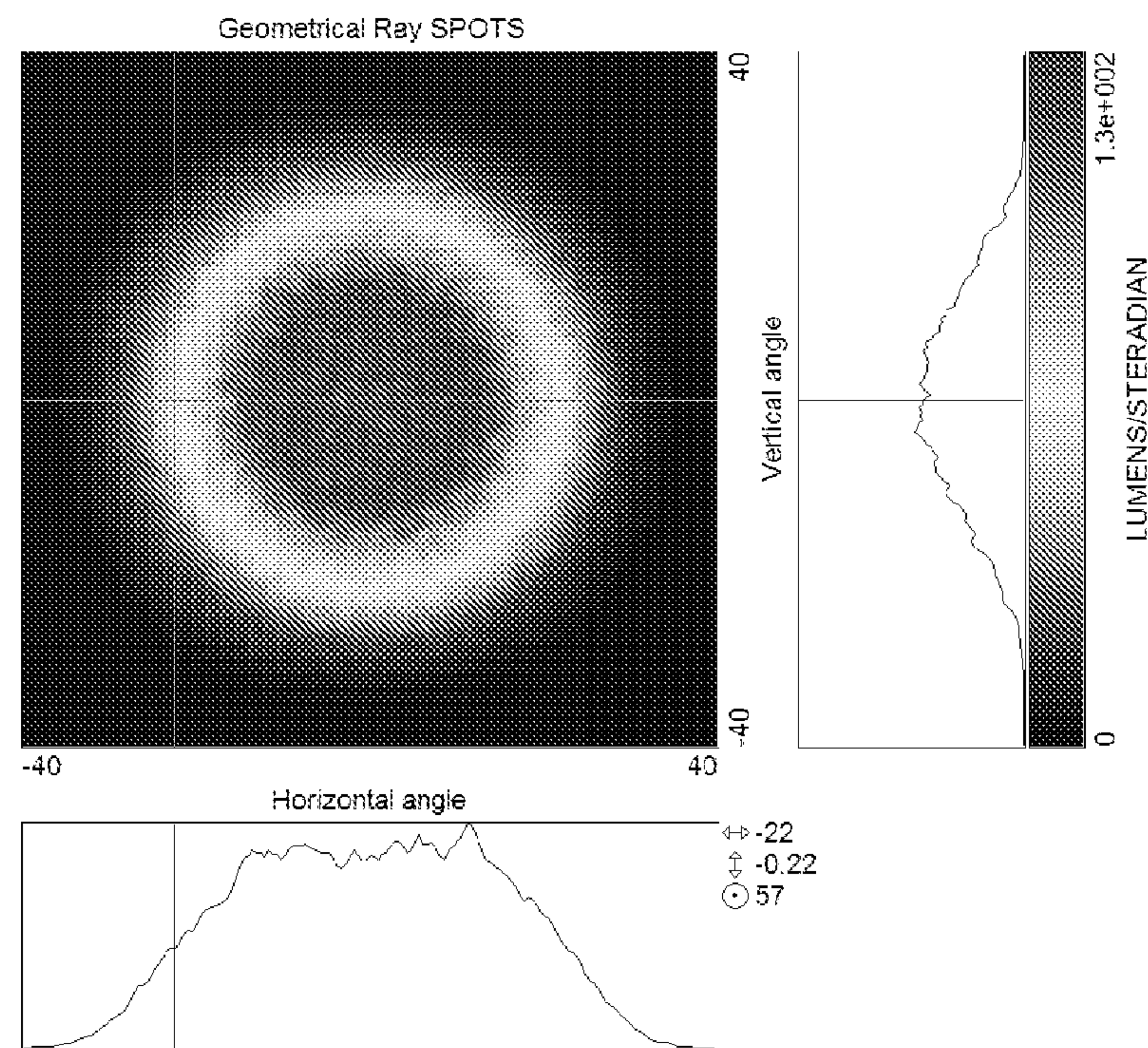
Figure 13 – “FAR” or “WIDE” POSITION: 1.3 CD/LM MAXIMUM
