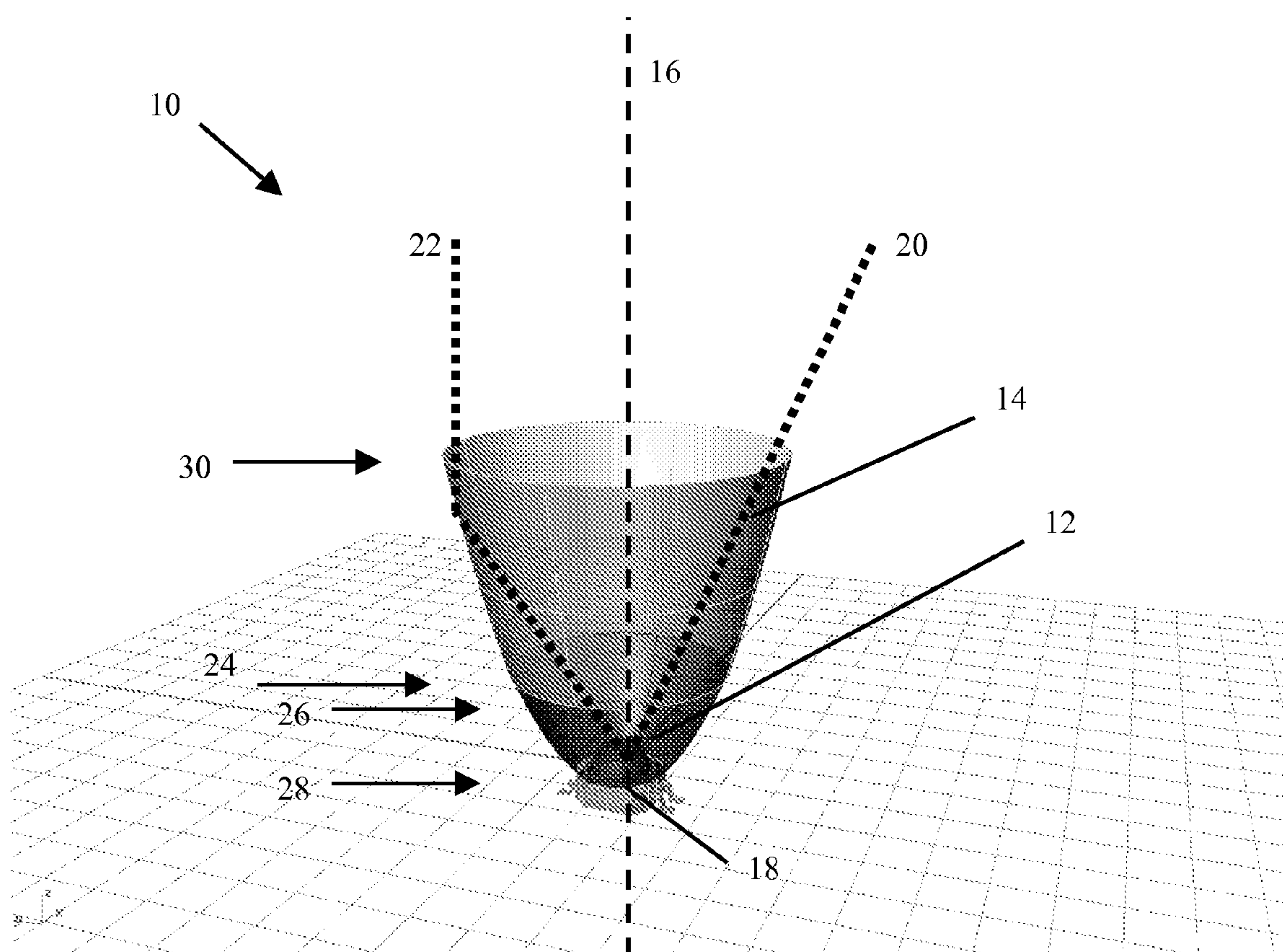
Figure 1: Multi-stage reflector in fully extended position
