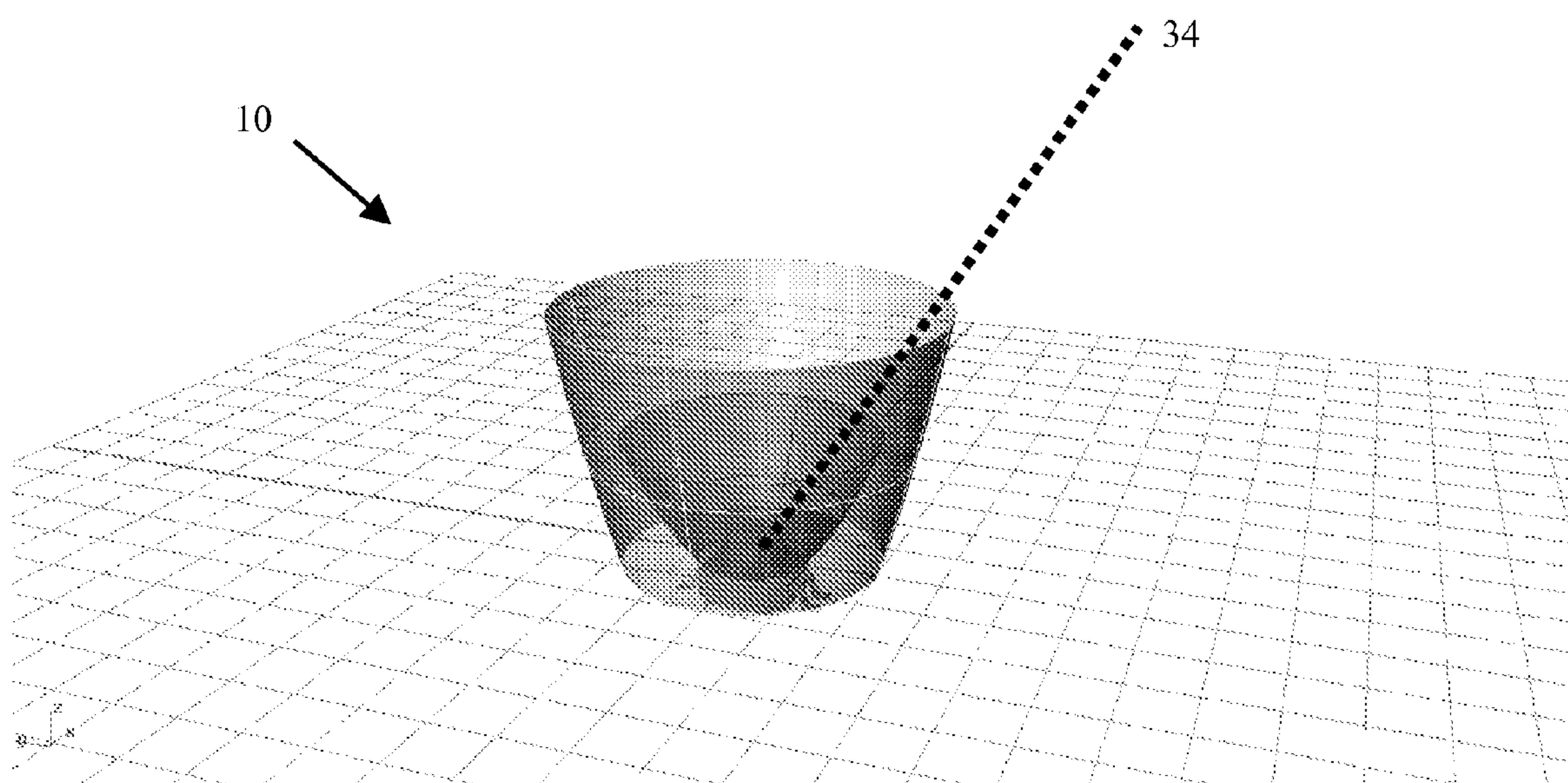
Figure 3: Multi-stage reflector in fully retracted position
