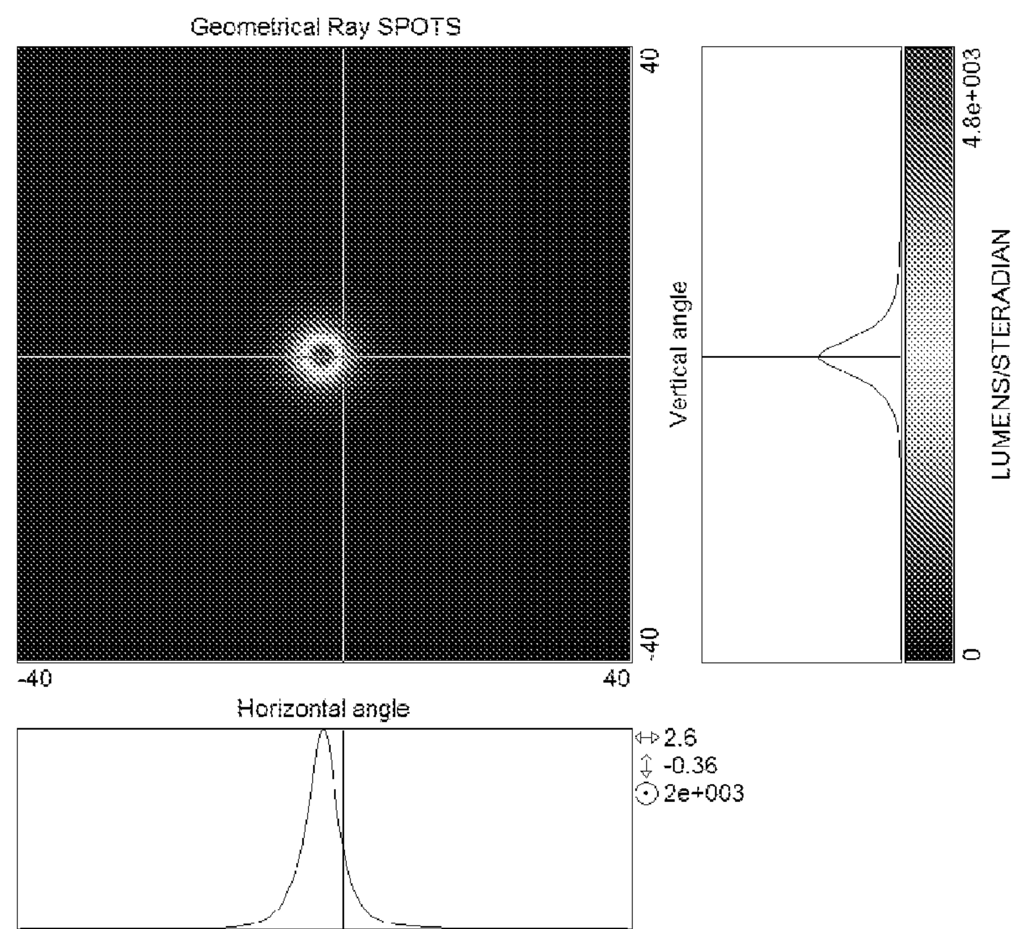
Figure 12 – “CLOSE” or “NARROW” POSITION: 48 CD/LM MAXIMUM
