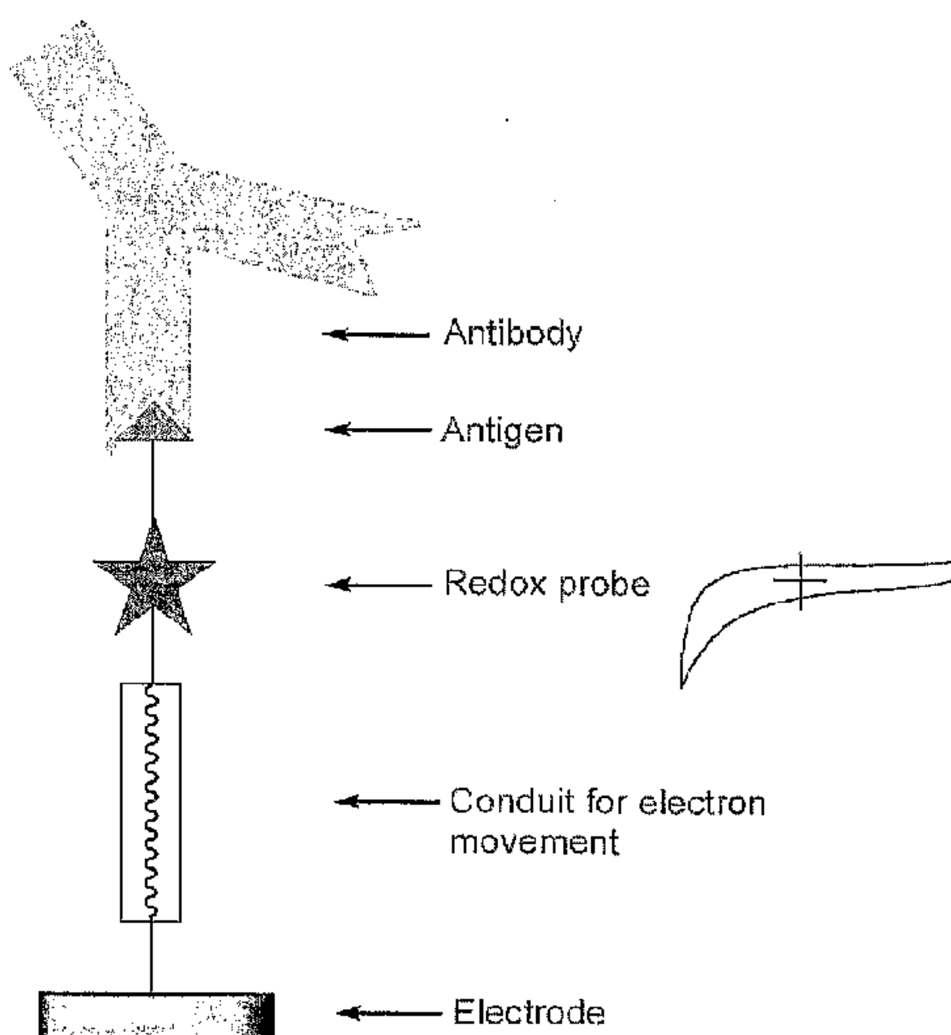
Second Sensor
