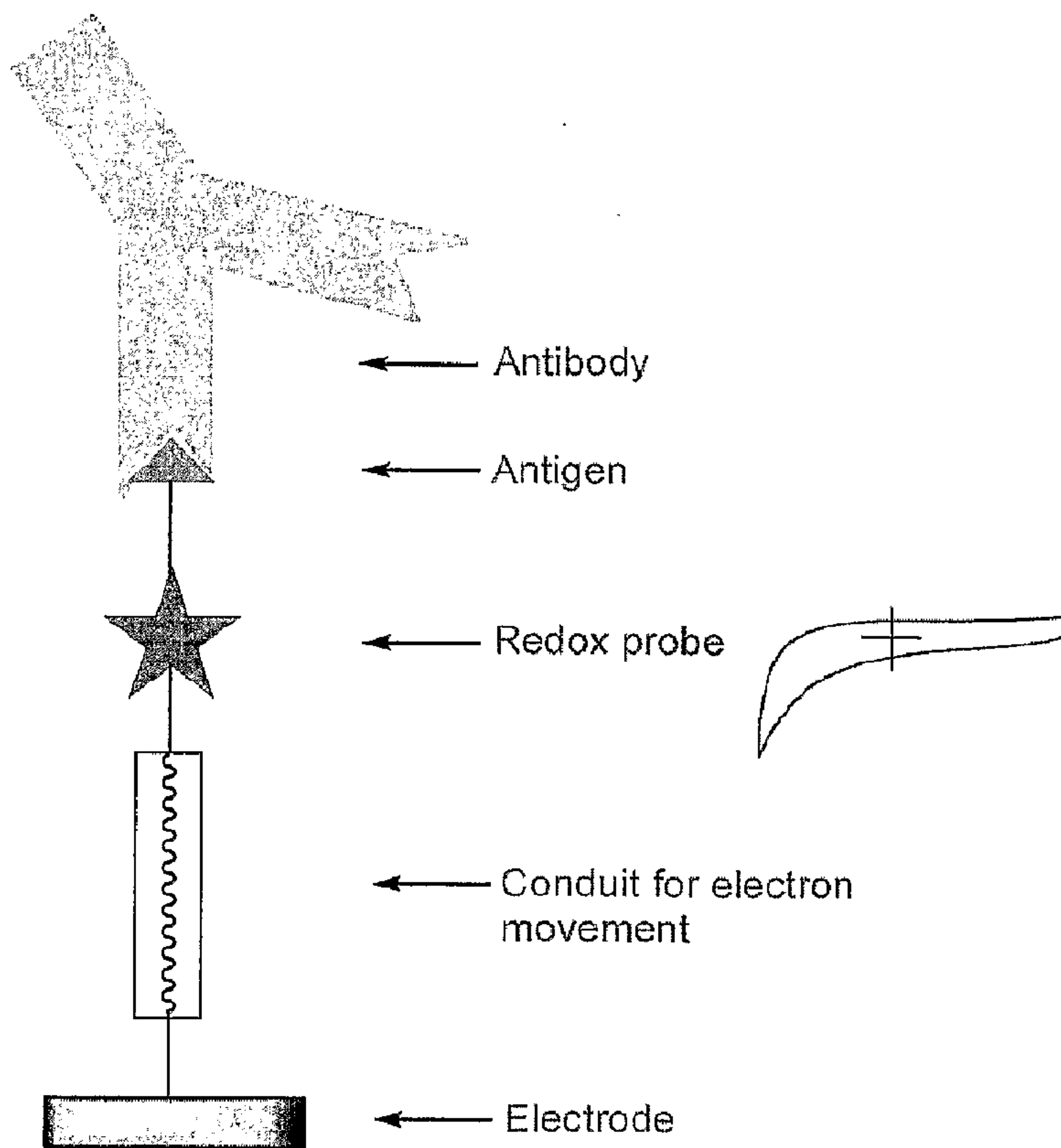
Second Sensor
