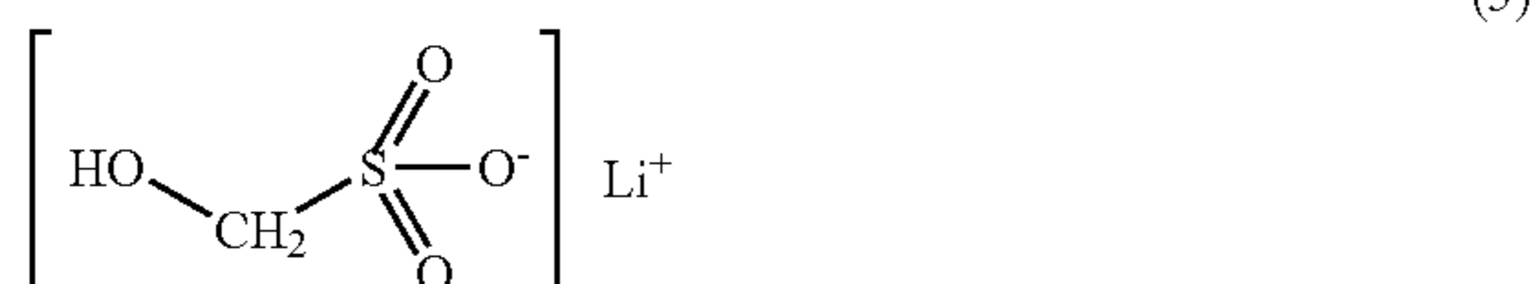
[Chemical Formula 14]
