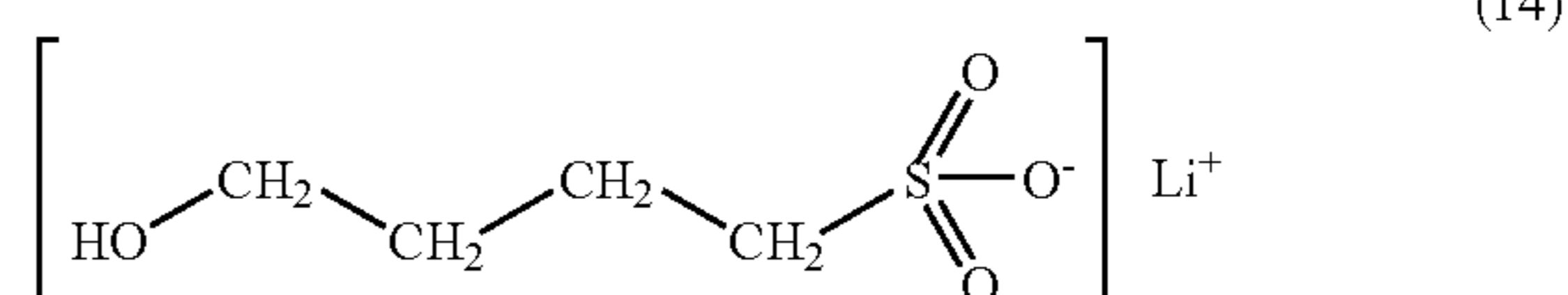
[Chemical Formula 23]
