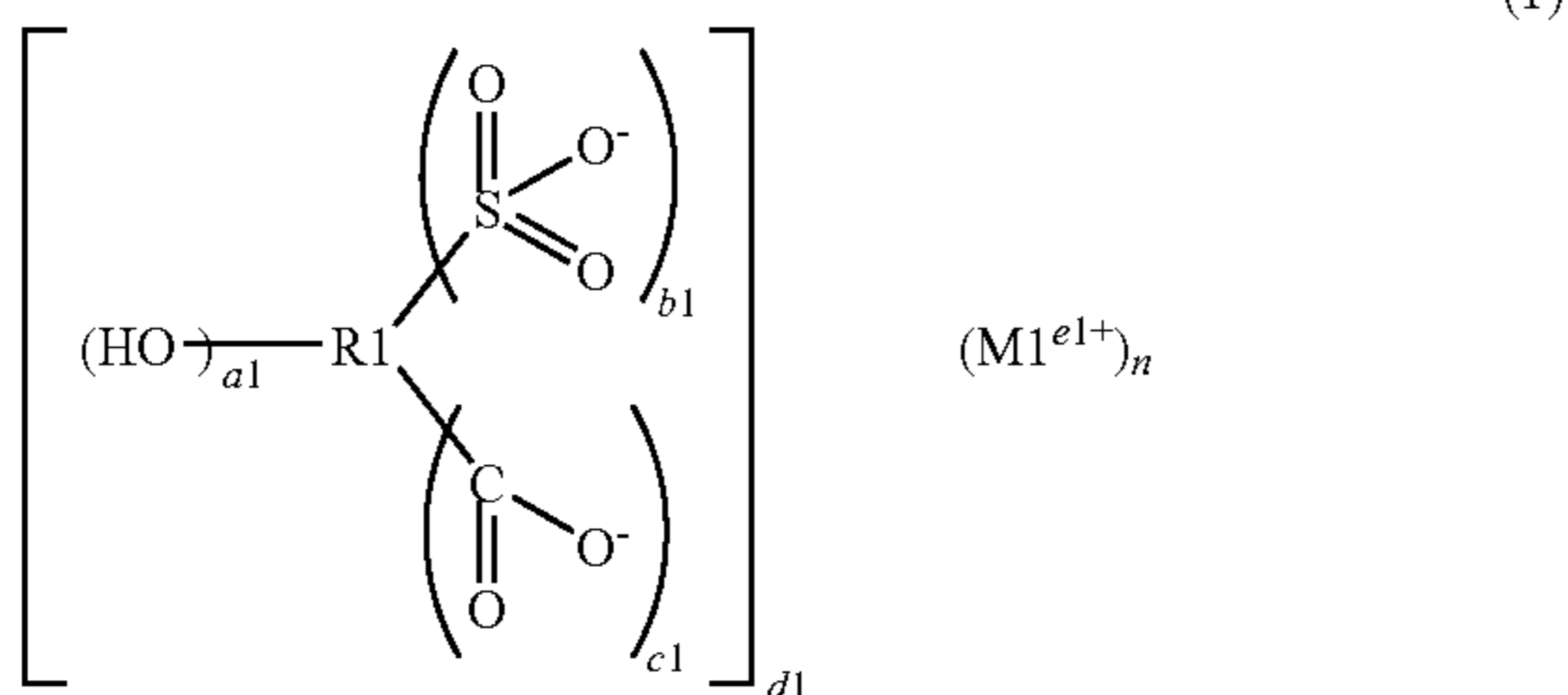
[Chemical Formula 4]
