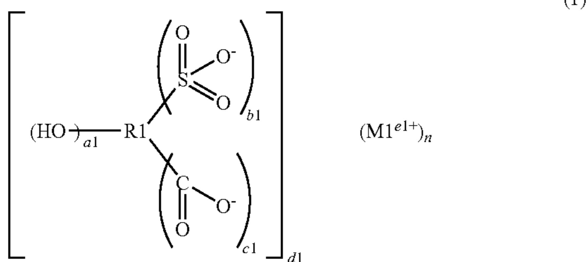
[Chemical Formula 6]
