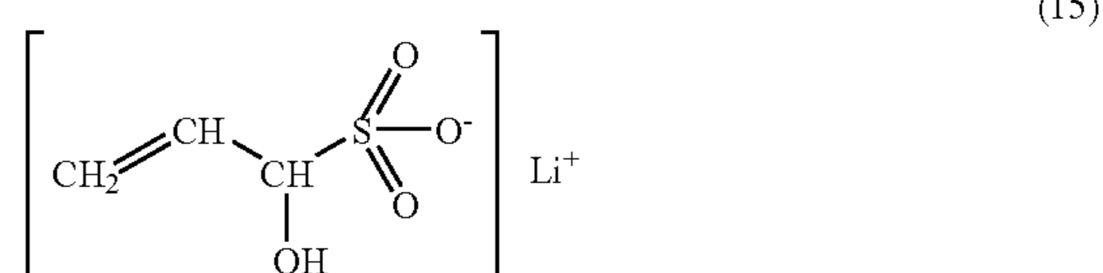
[Chemical Formula 23]
