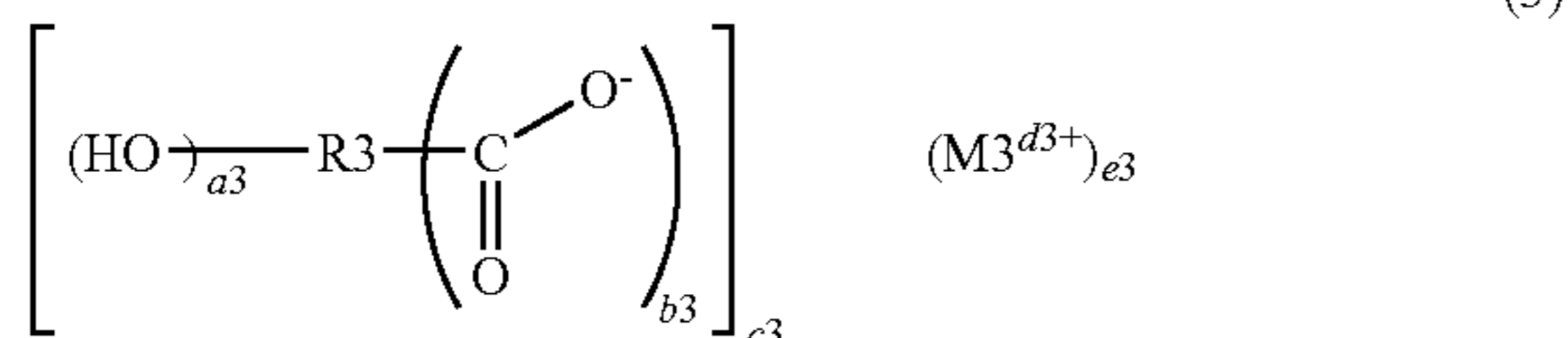
[Chemical Formula 11]
