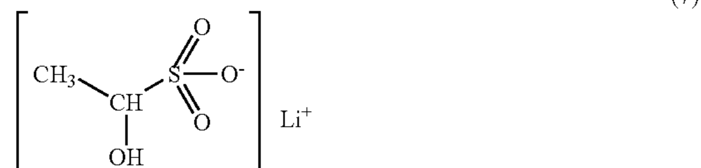
[Chemical Formula 16]
