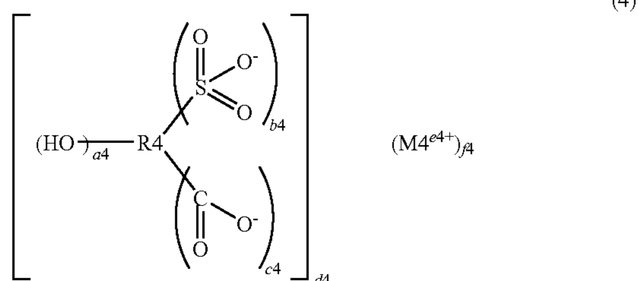
[Chemical Formula 12]
