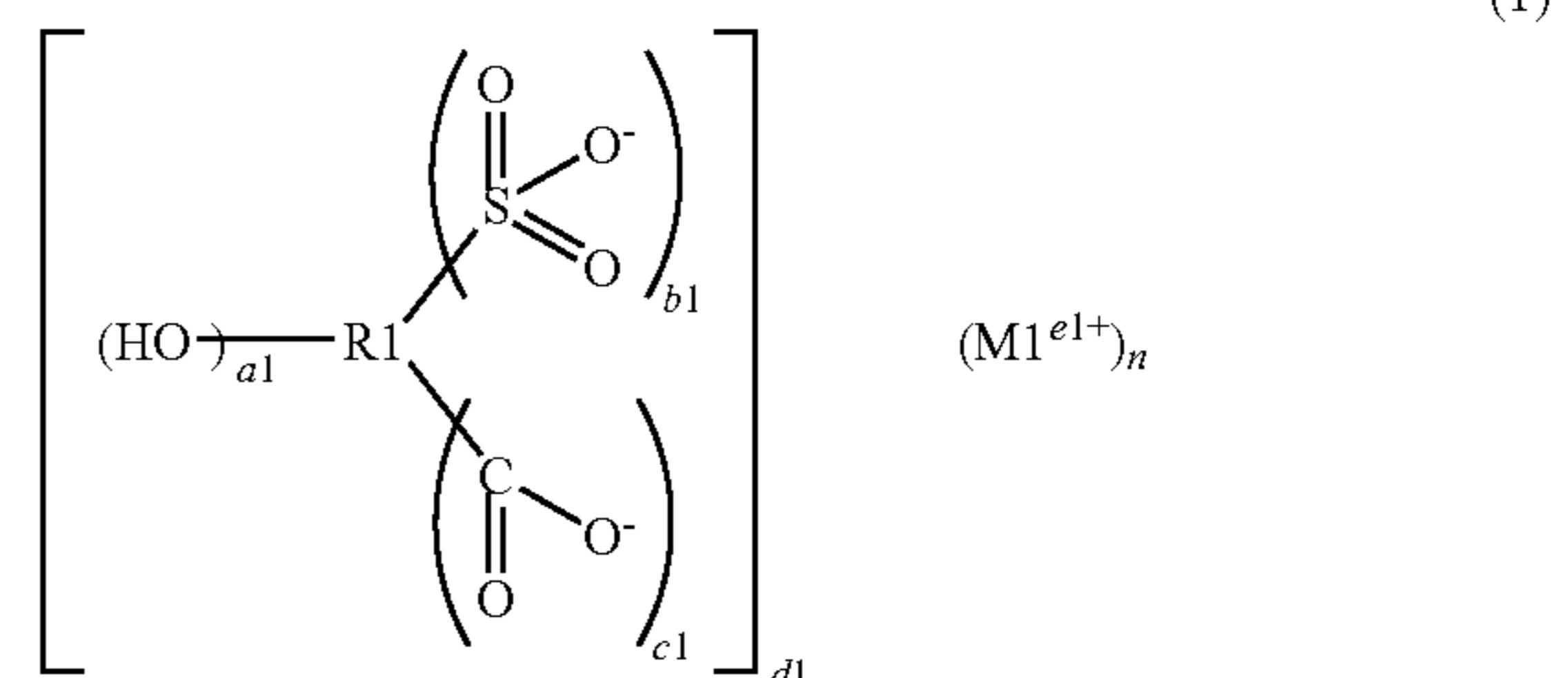
[Chemical Formula 8]
