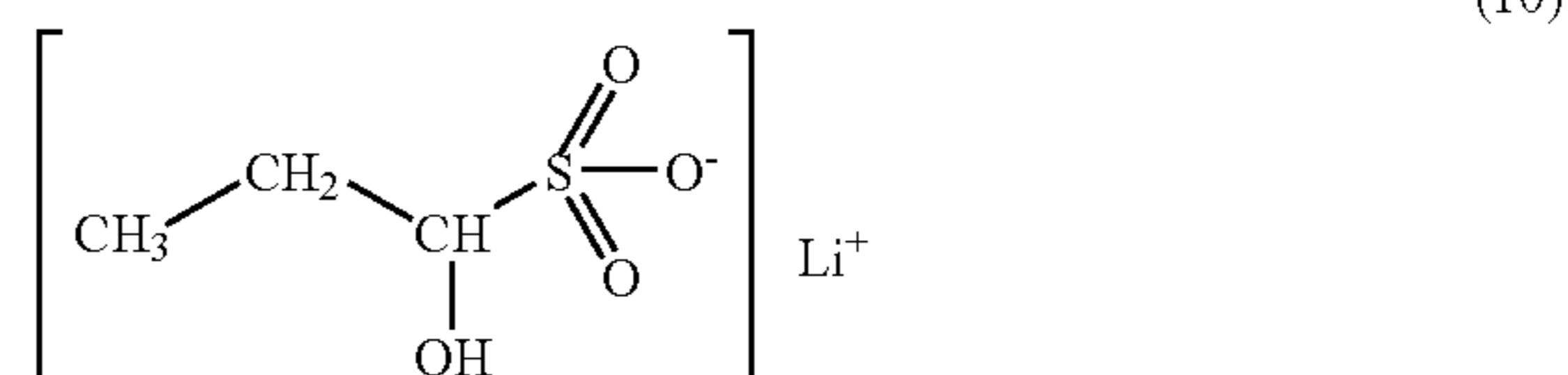
[Chemical Formula 19]
