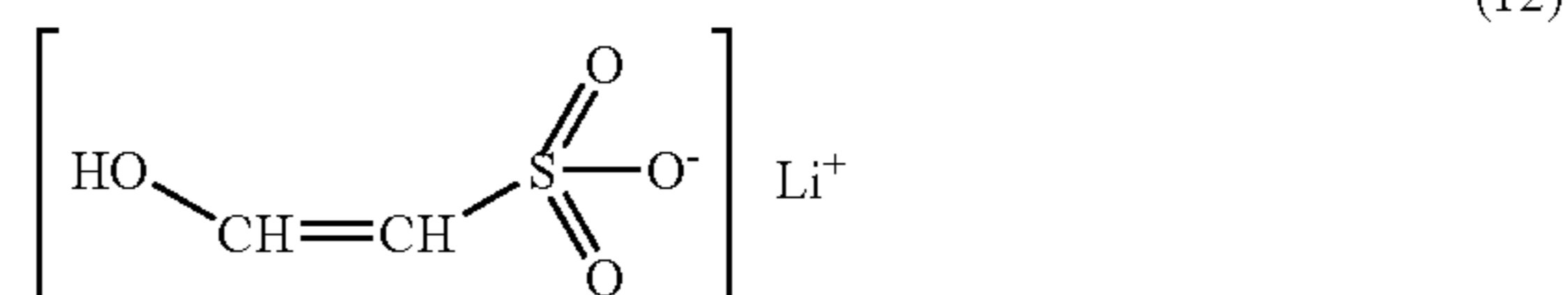
[Chemical Formula 21]
