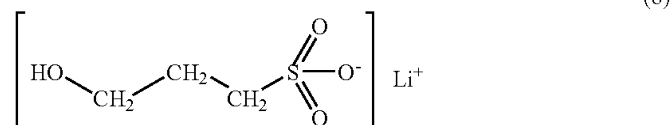
[Chemical Formula 17]
