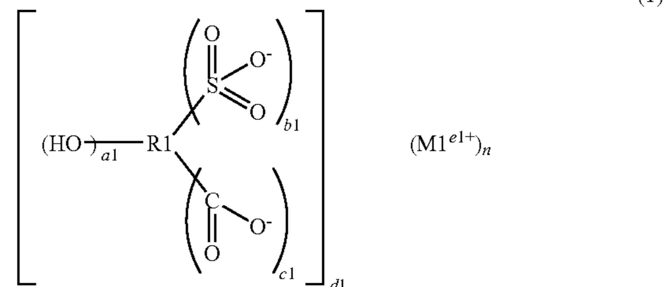
[Chemical Formula 7]
