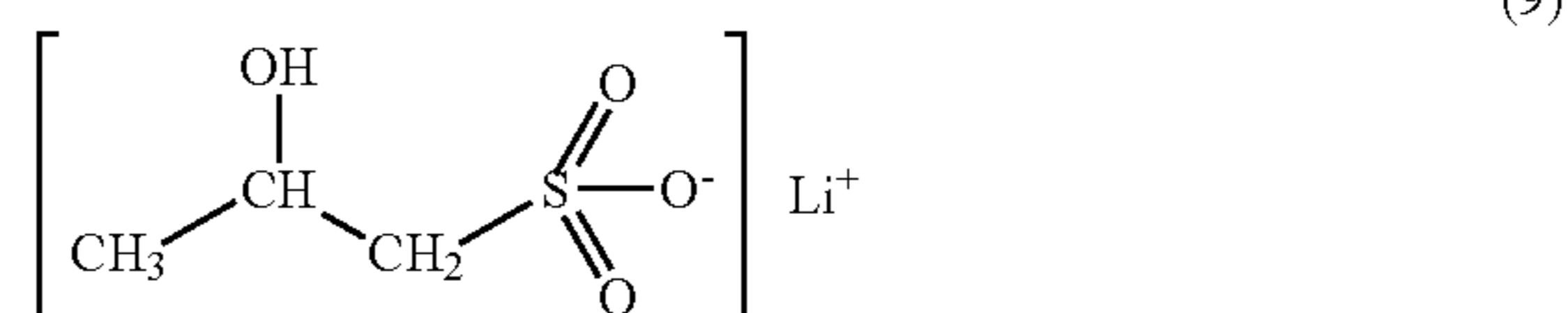
[Chemical Formula 18]
