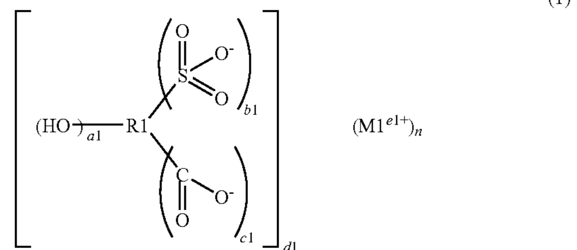
[Chemical Formula 5]
