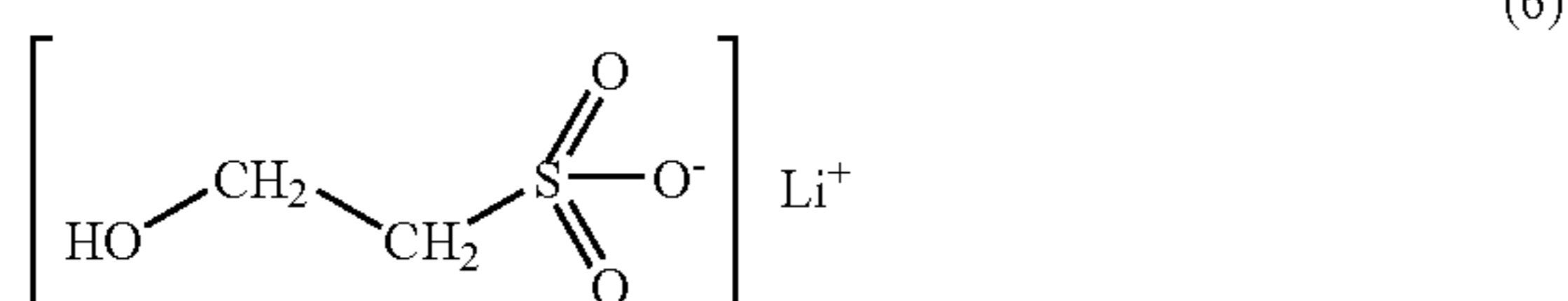
[Chemical Formula 14]
