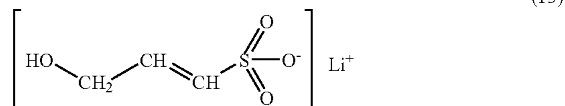
[Chemical Formula 22]
