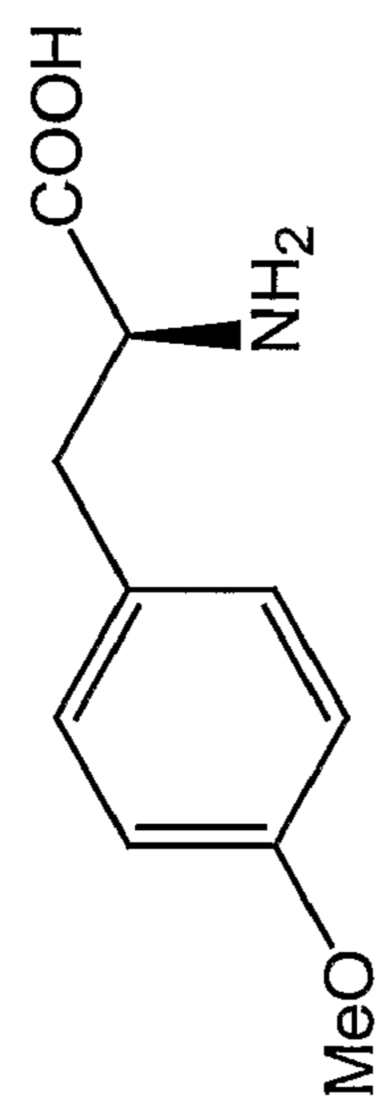
O-methyl tyrosine
