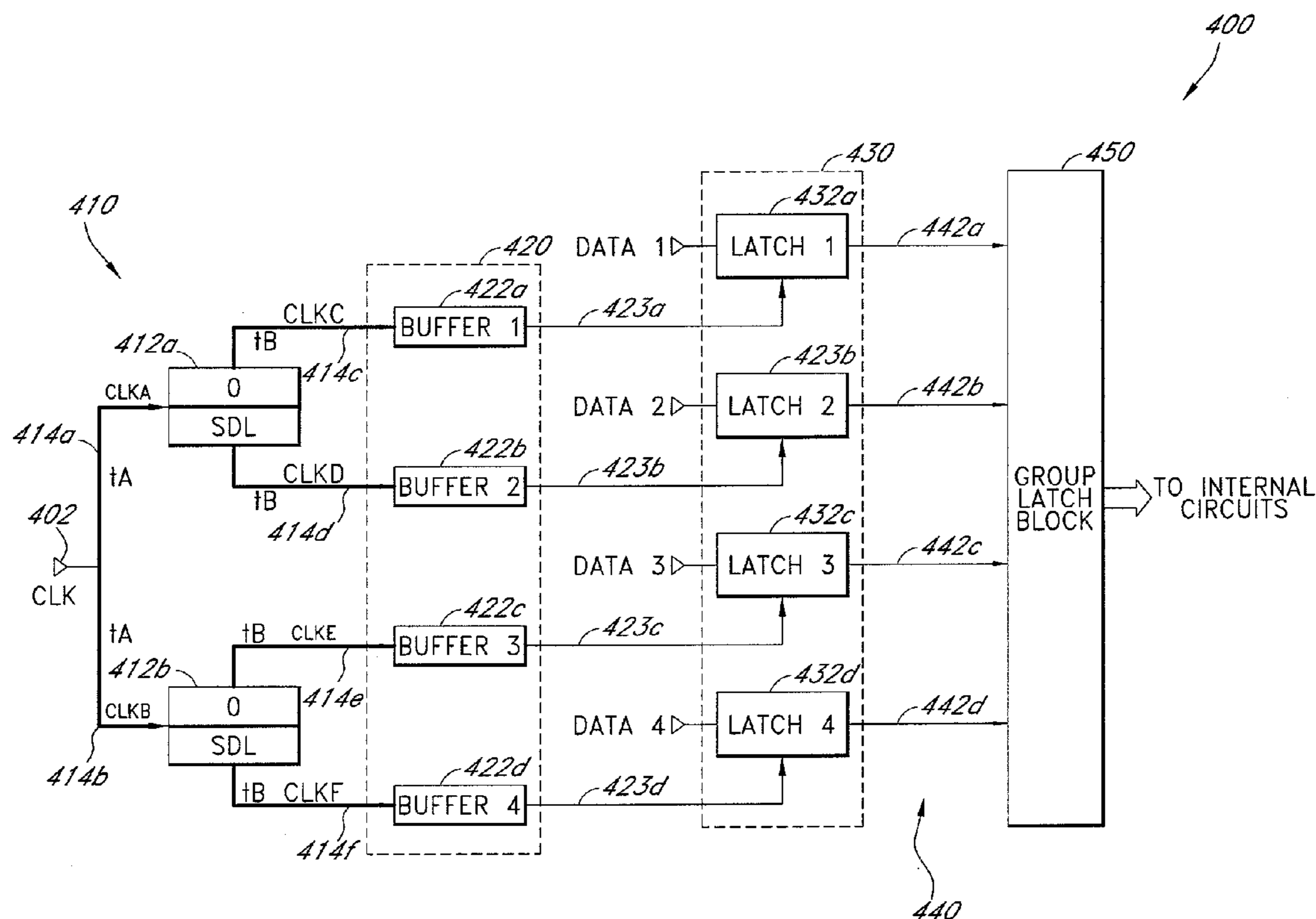
Receiver Circuit
