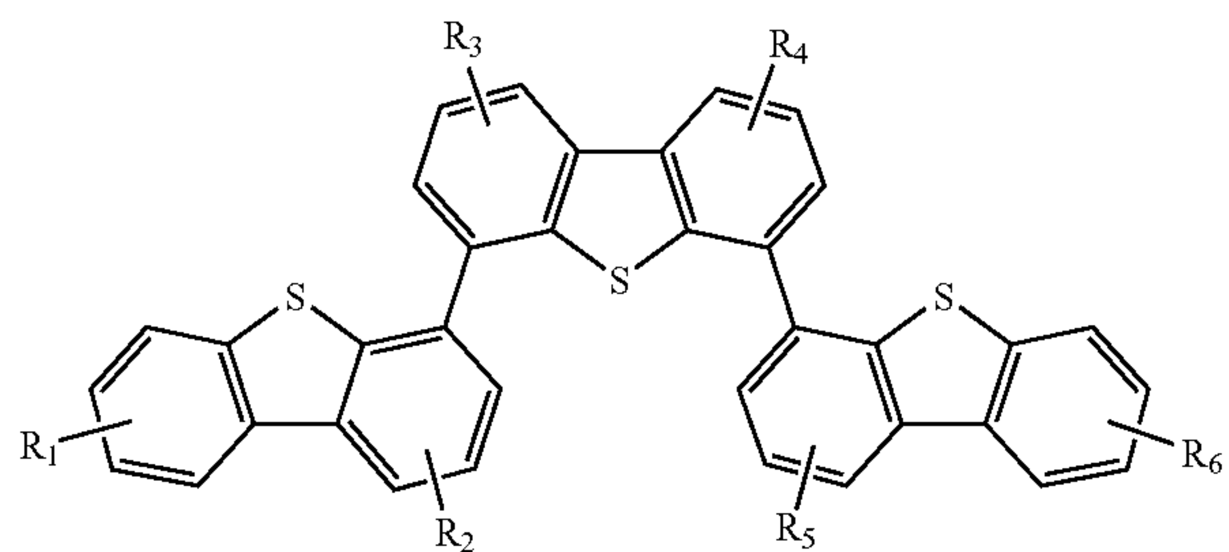
Compound 4G
