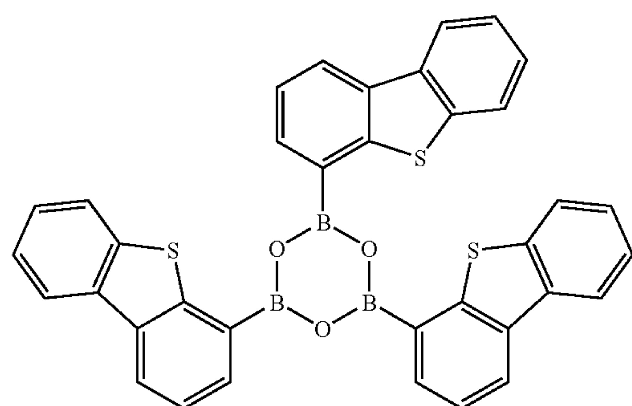
Compound 9
