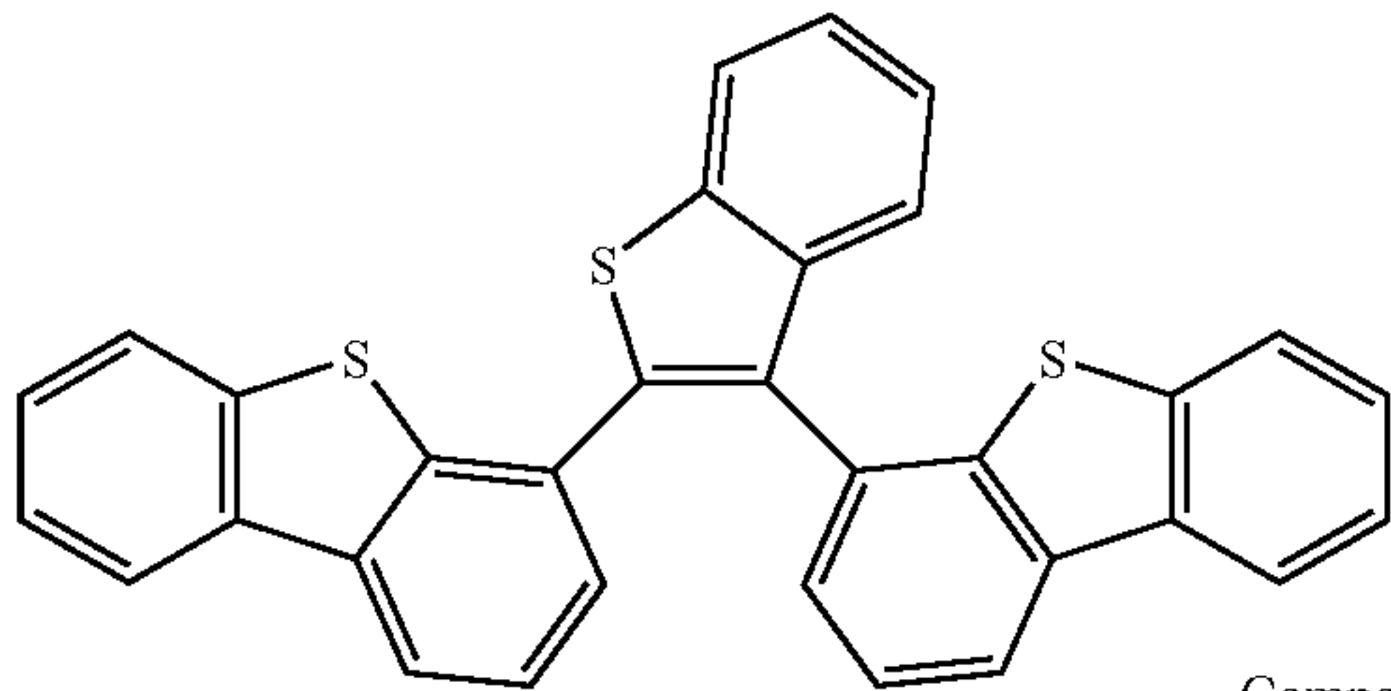
Compound 11
