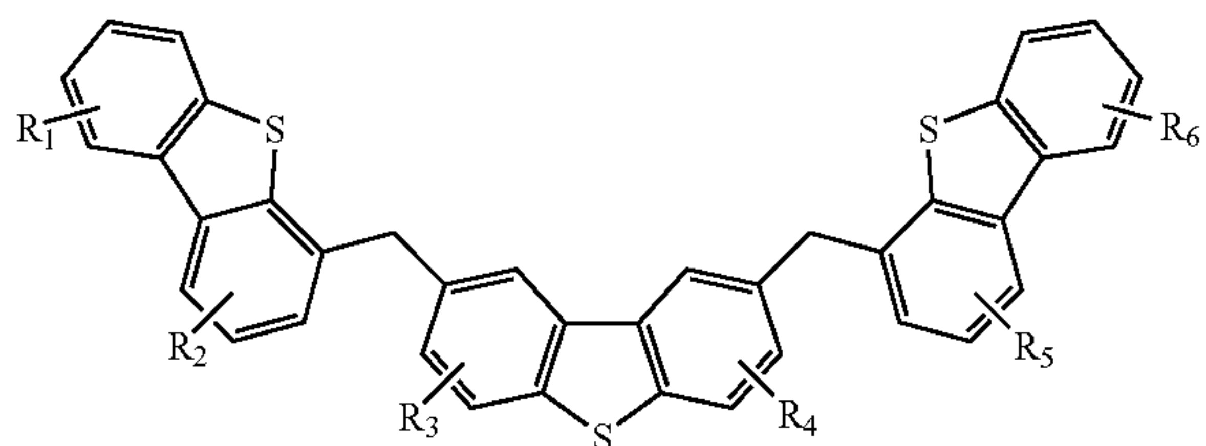
Compound 15G
