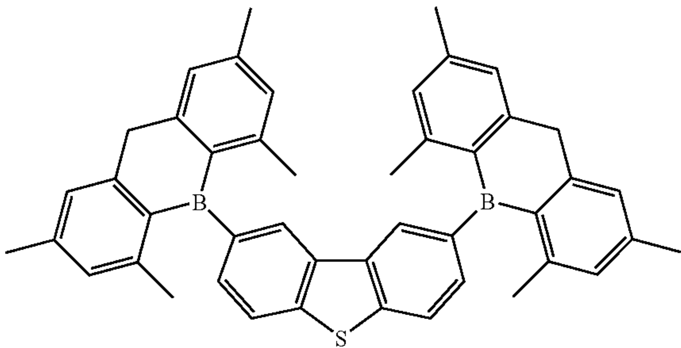
Compound 8
