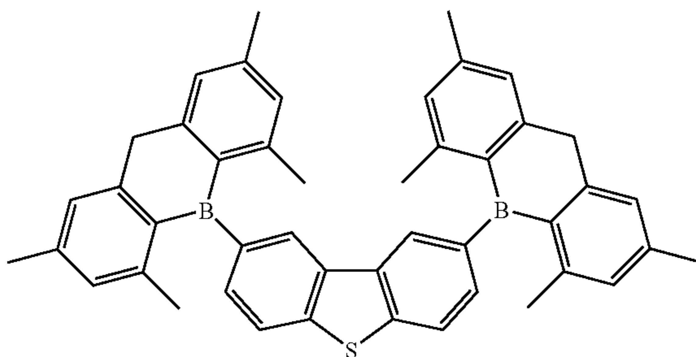
Compound 7
