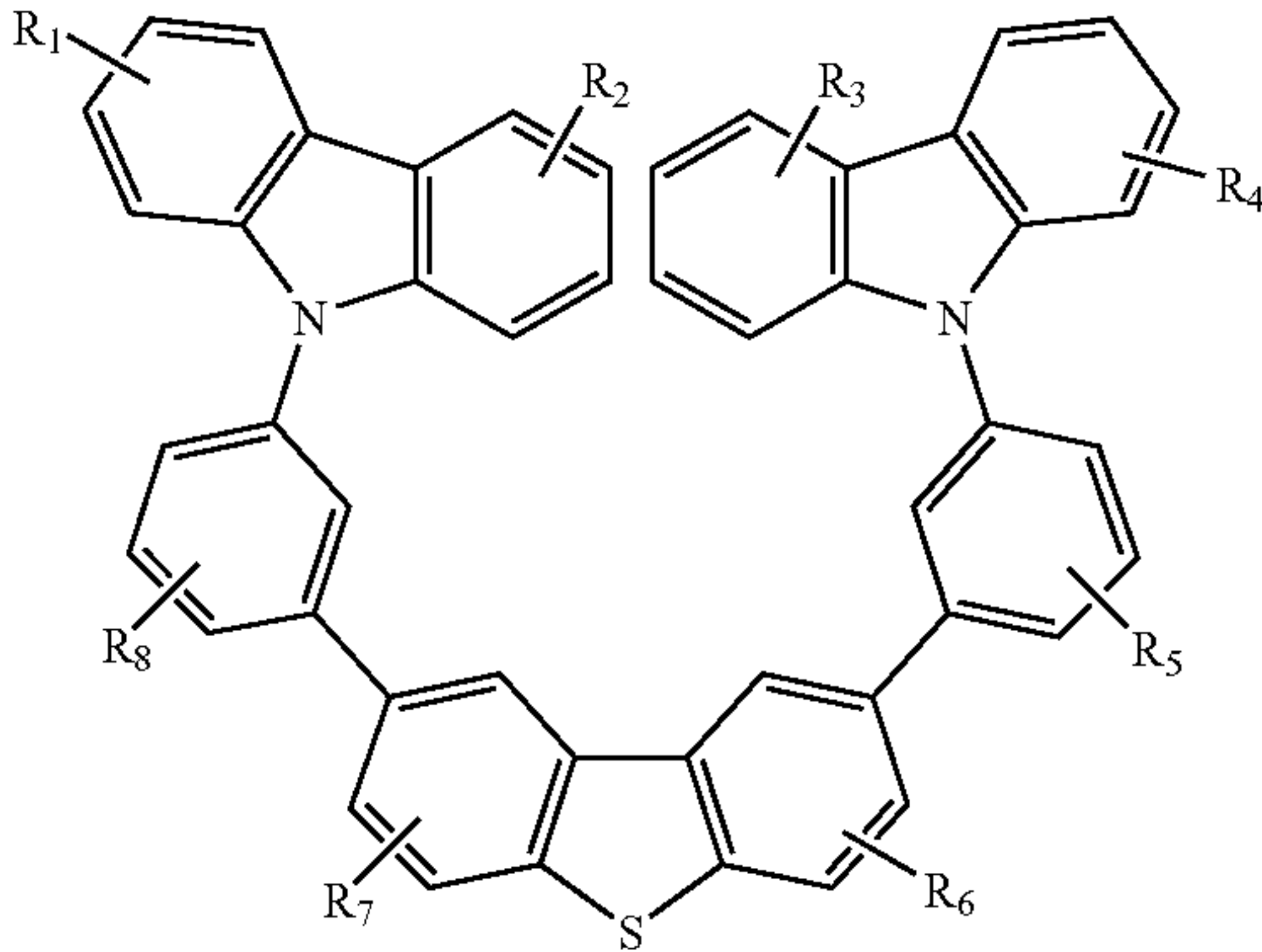
Compound 19G
