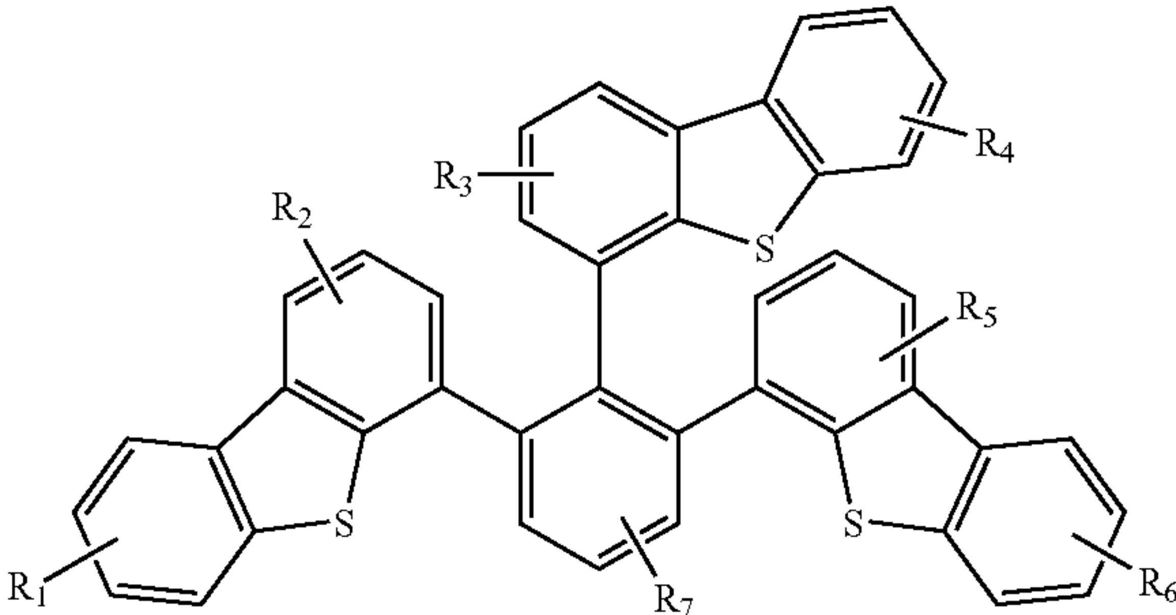
Compound 20G
