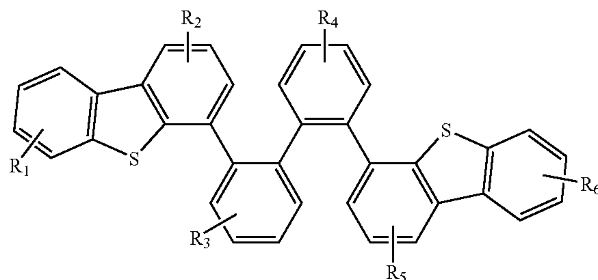
Compound 3G
