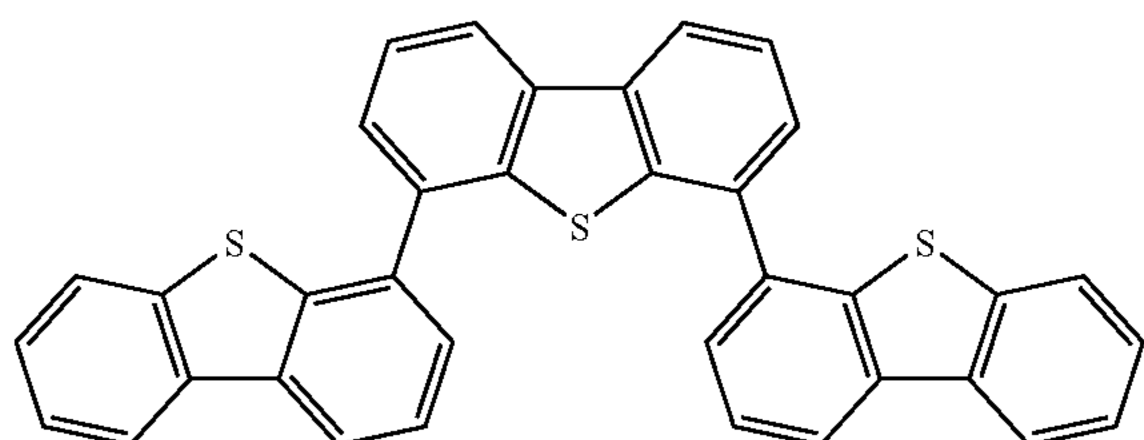
Compound 3
