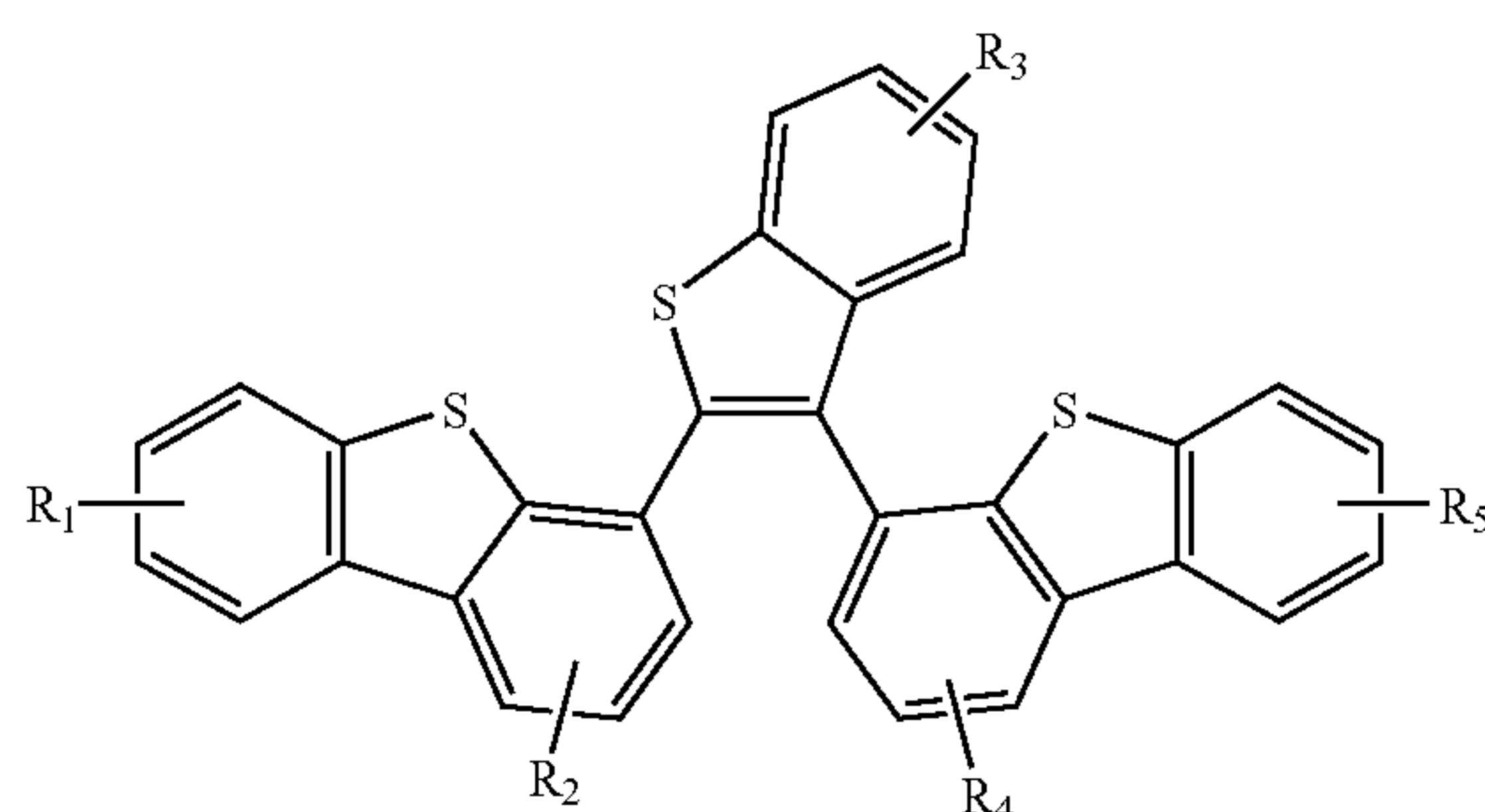
Compound 10G
