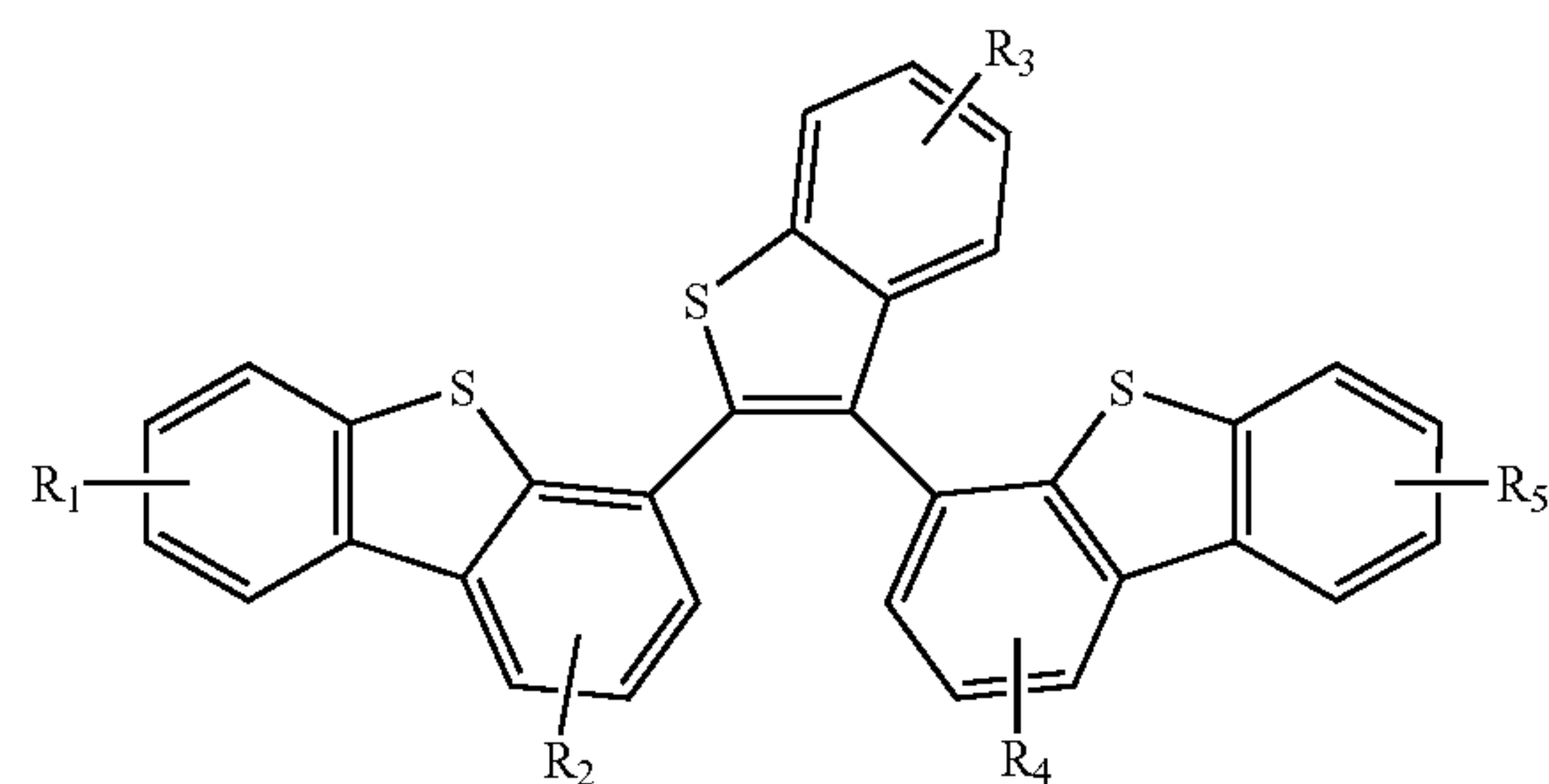
Compound 11G
