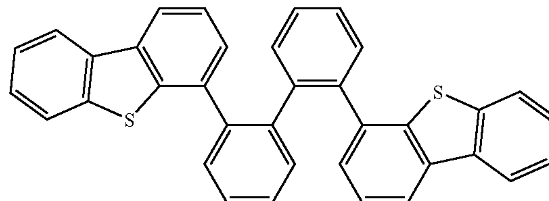
Compound 3
