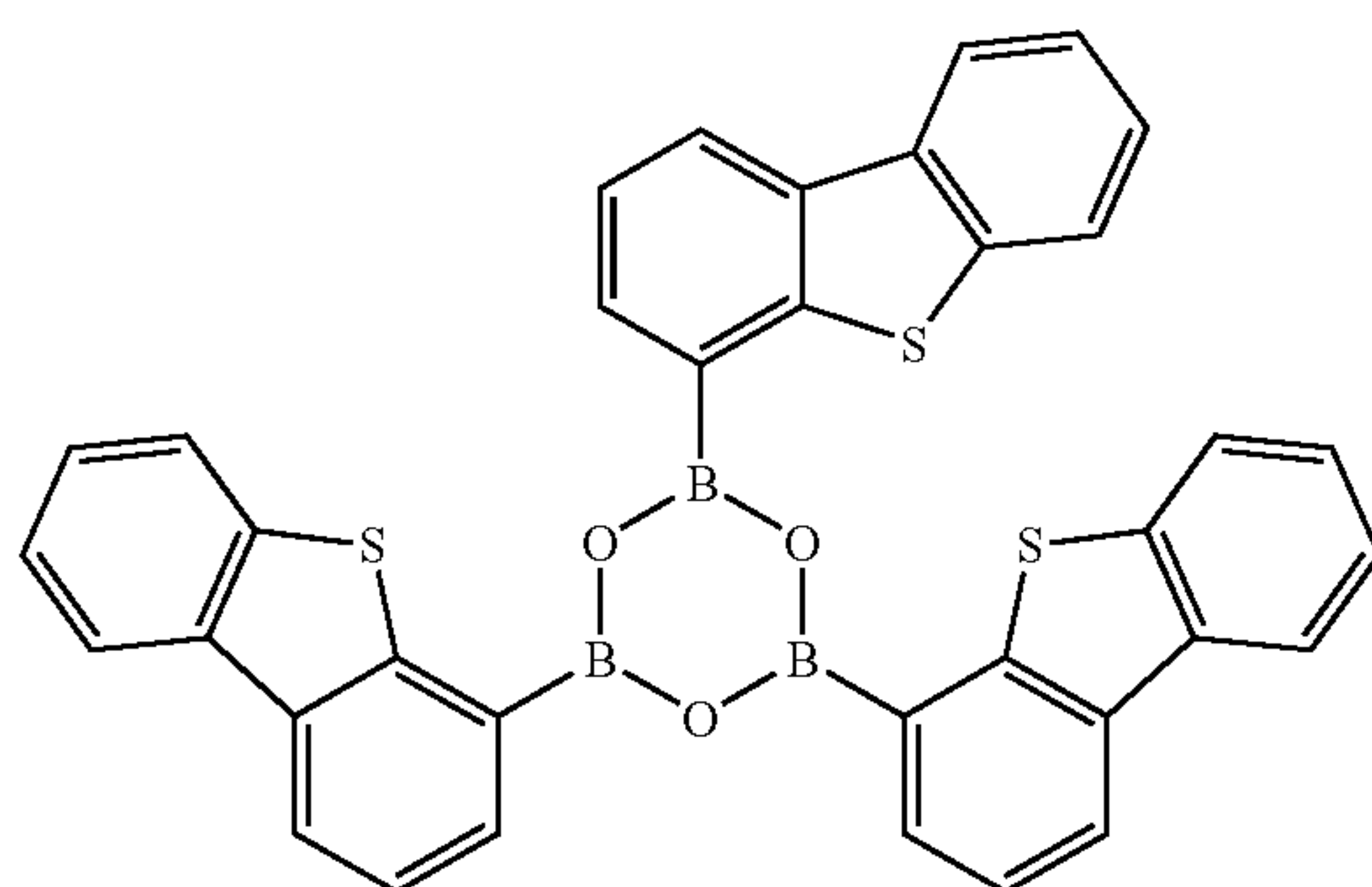
Compound 8
