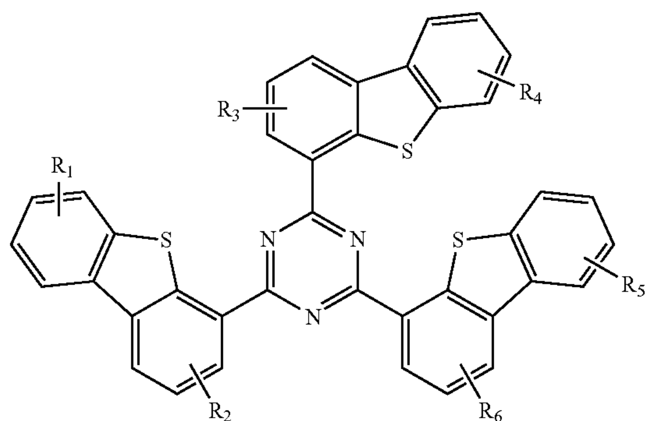
Compound 7G
