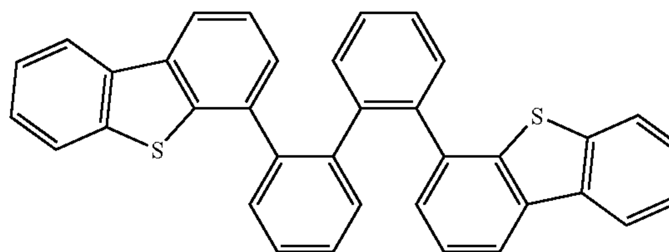
Compound 2
