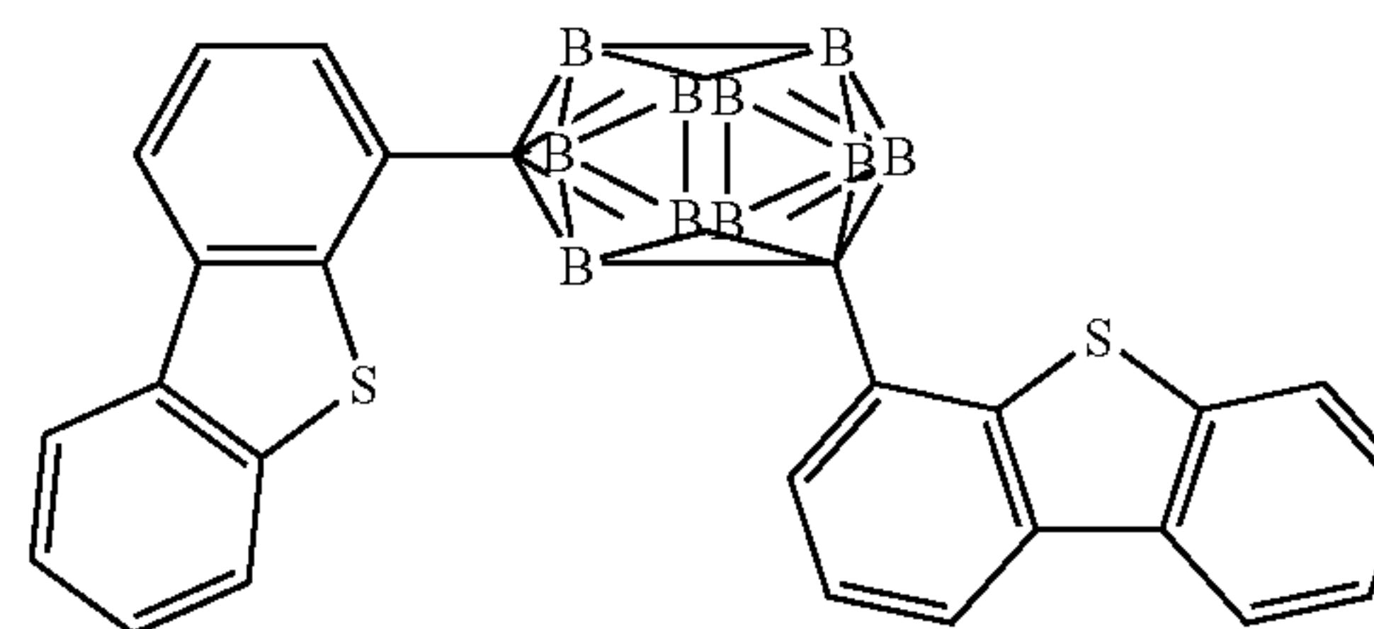
Compound 14
