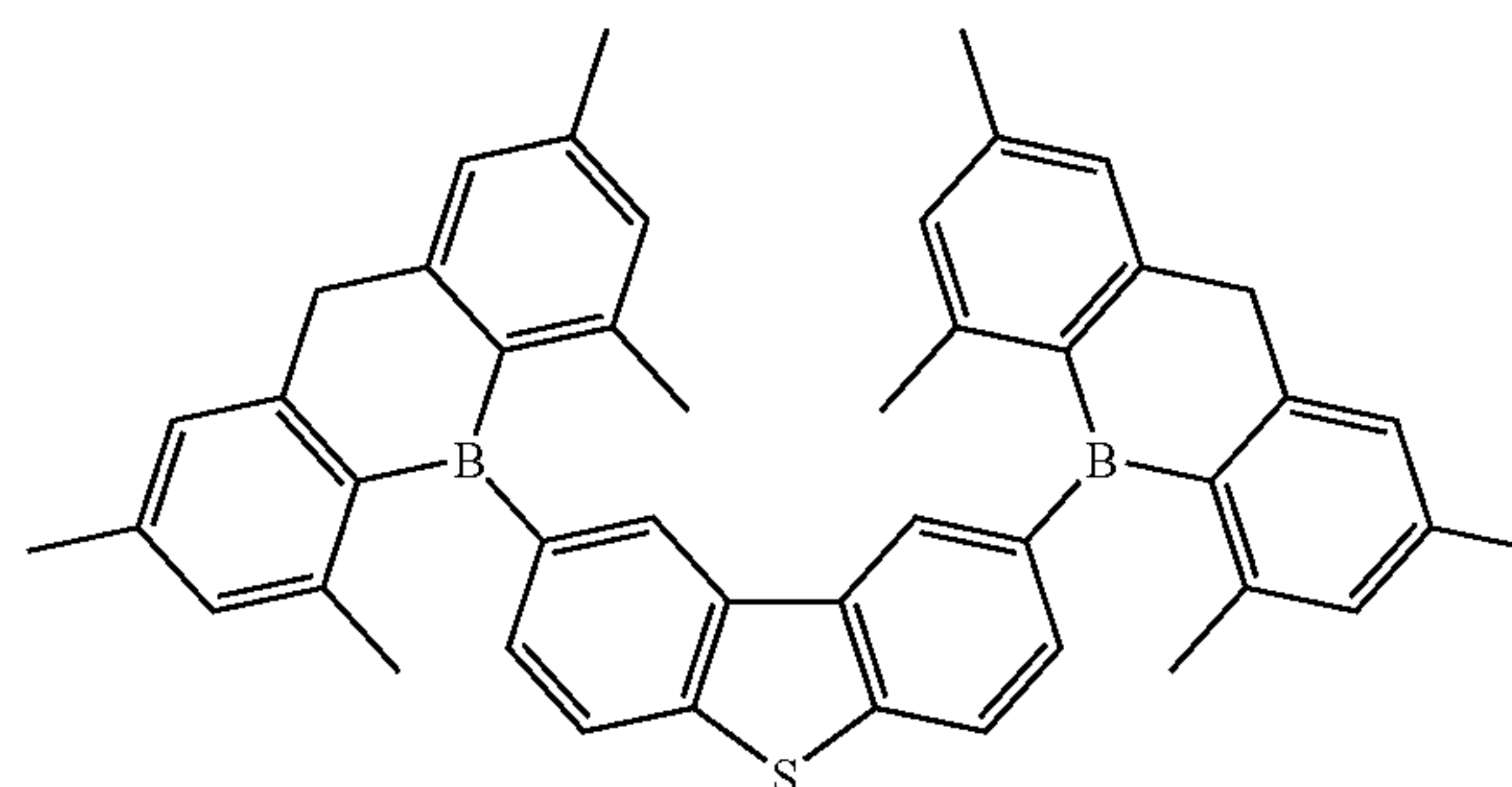
Compound 7
