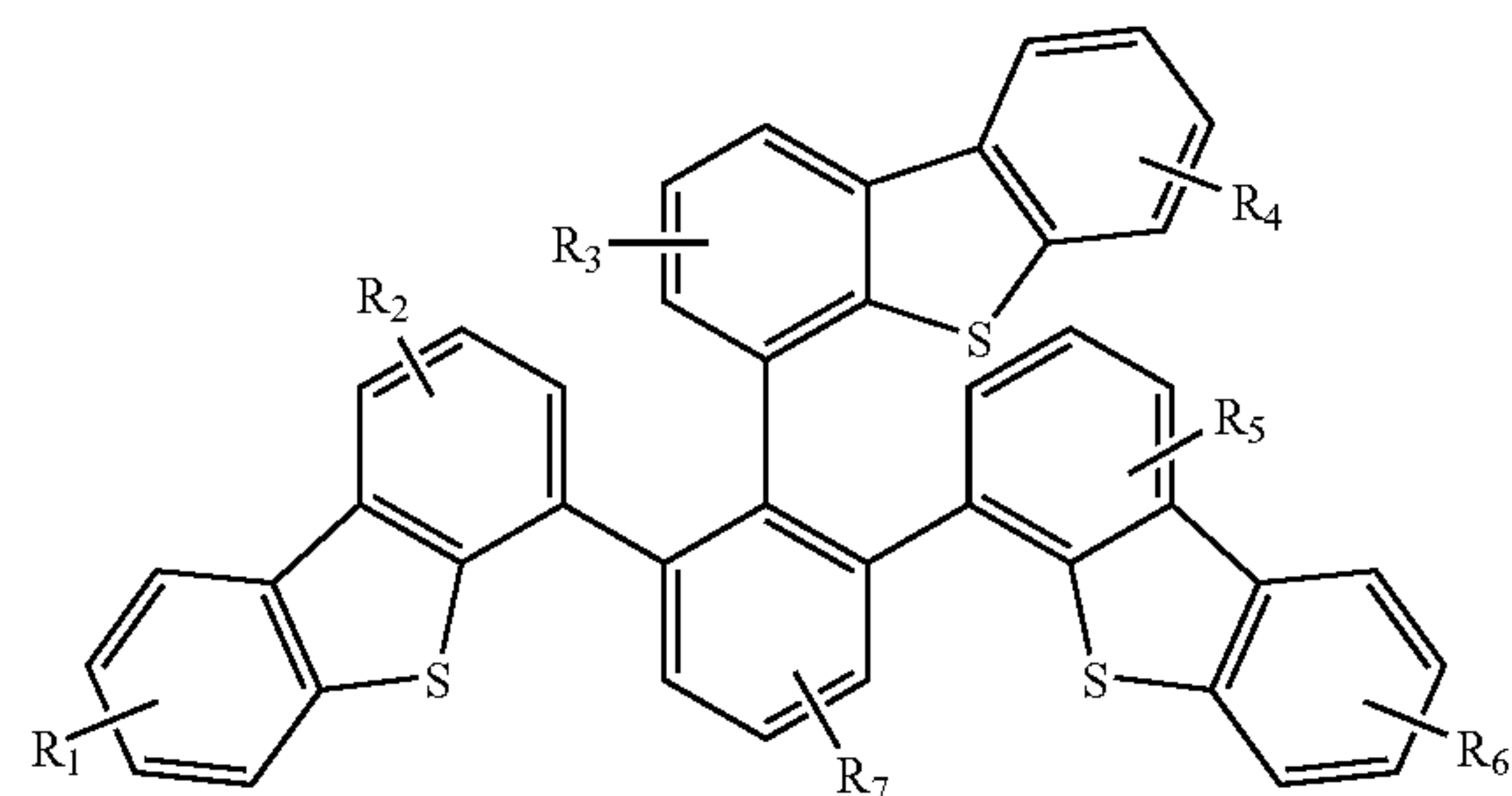
Compound 20G
