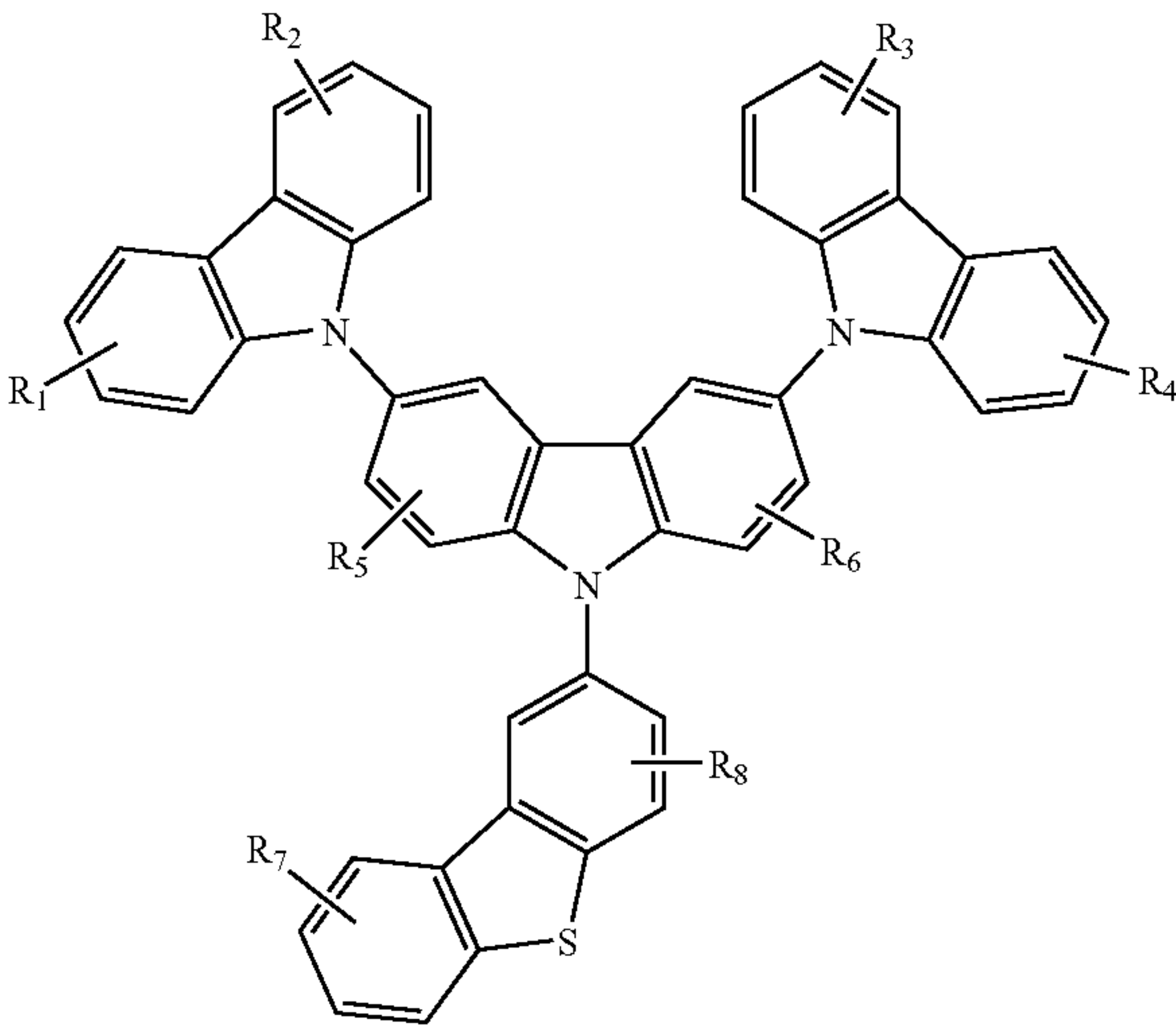
Compound 18G
