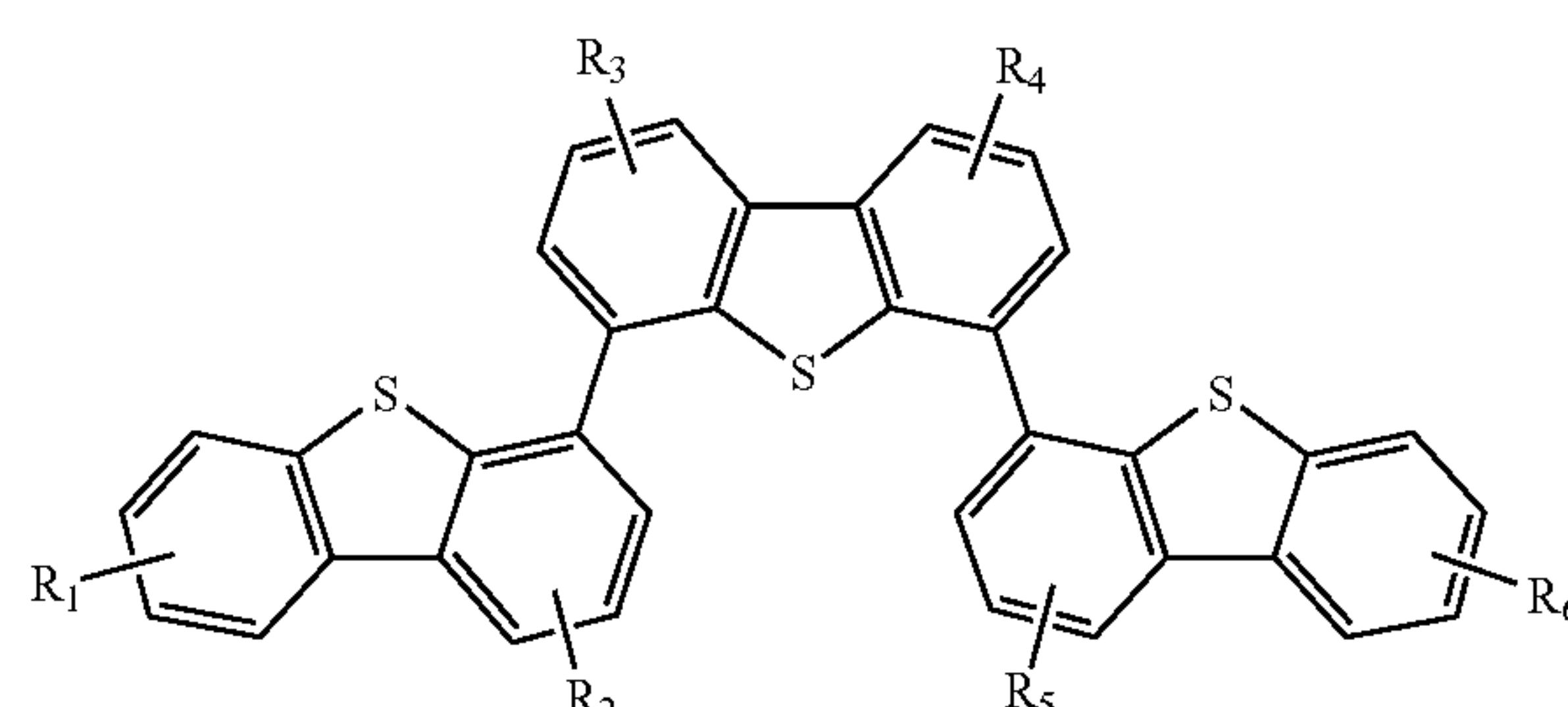
Compound 3G
