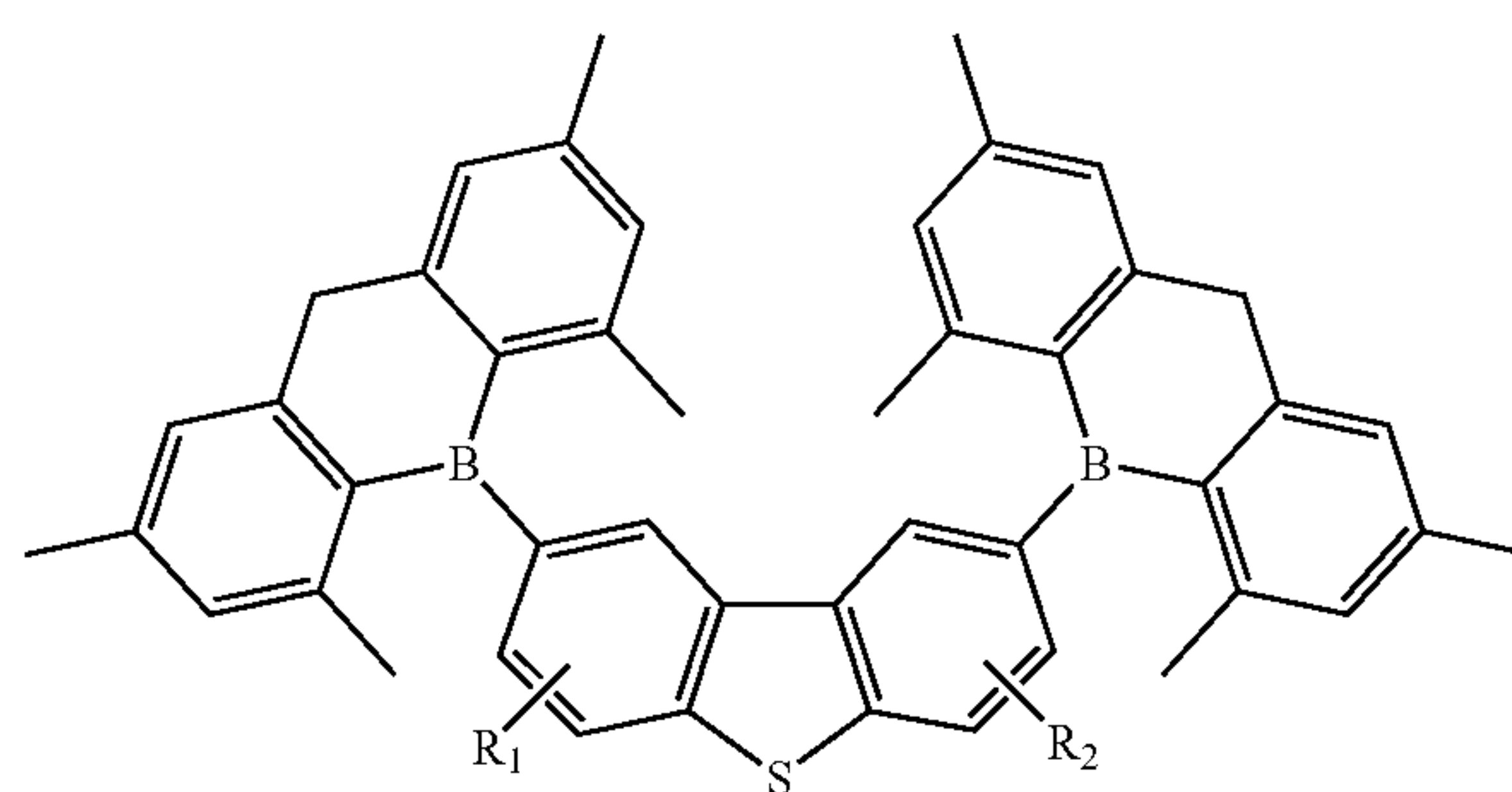
Compound 8G
