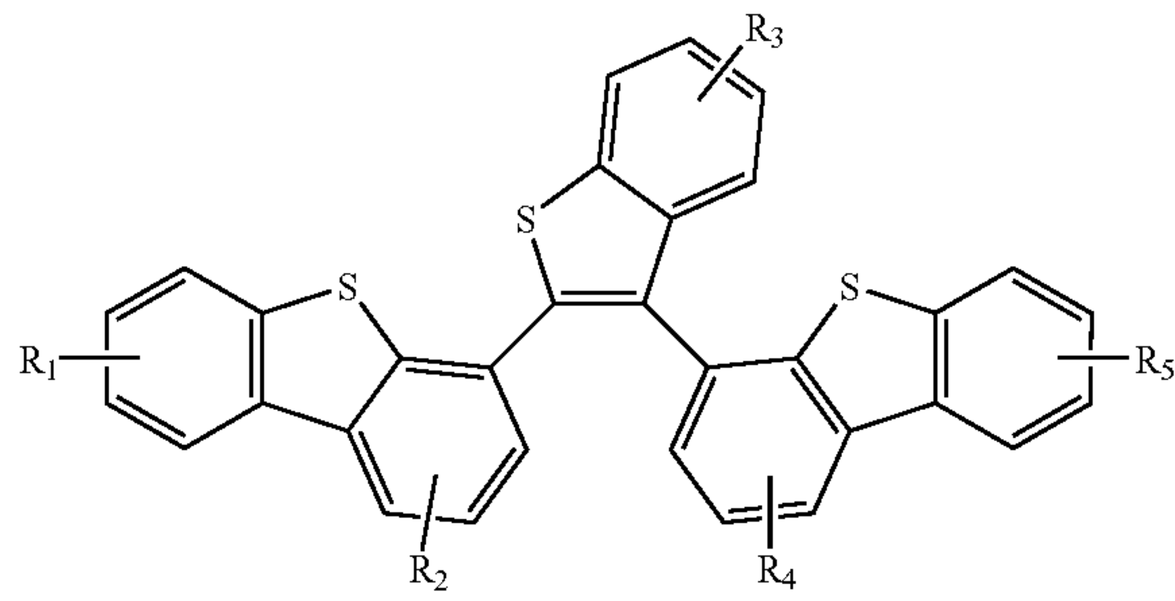
Compound 10G
