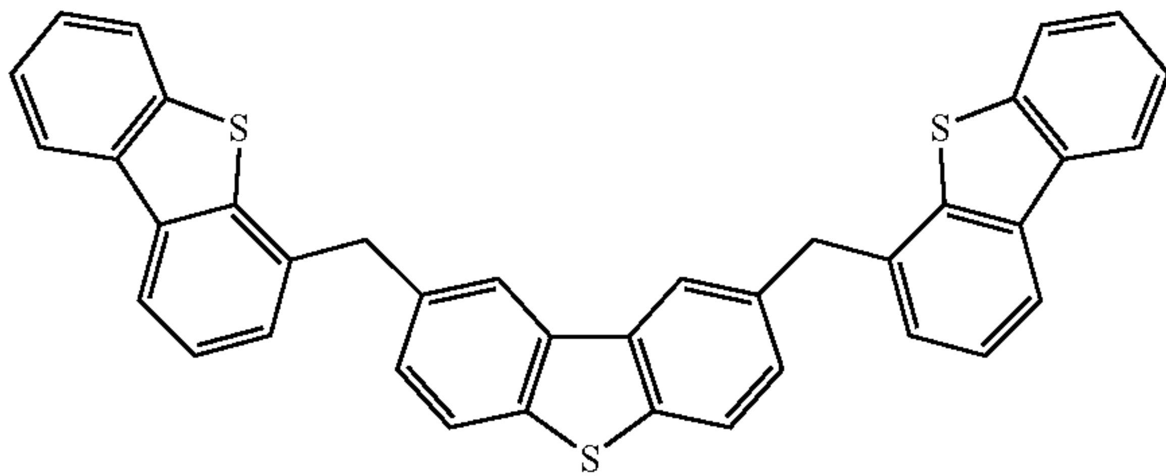
Compound 15
