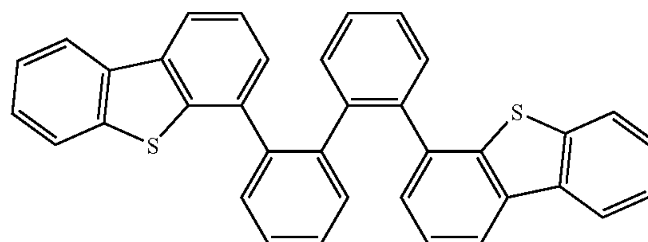
Compound 3
