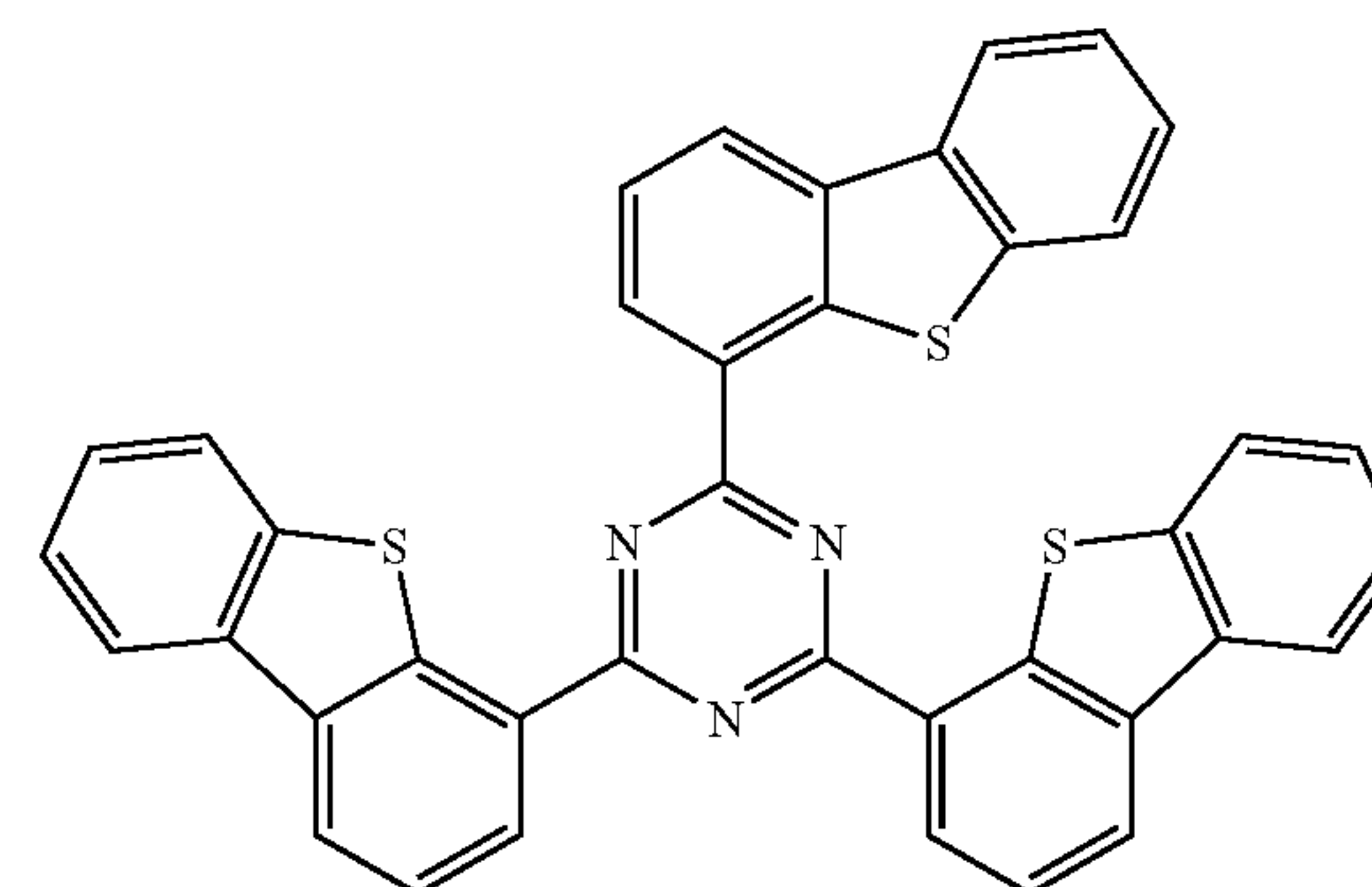
Compound 6
