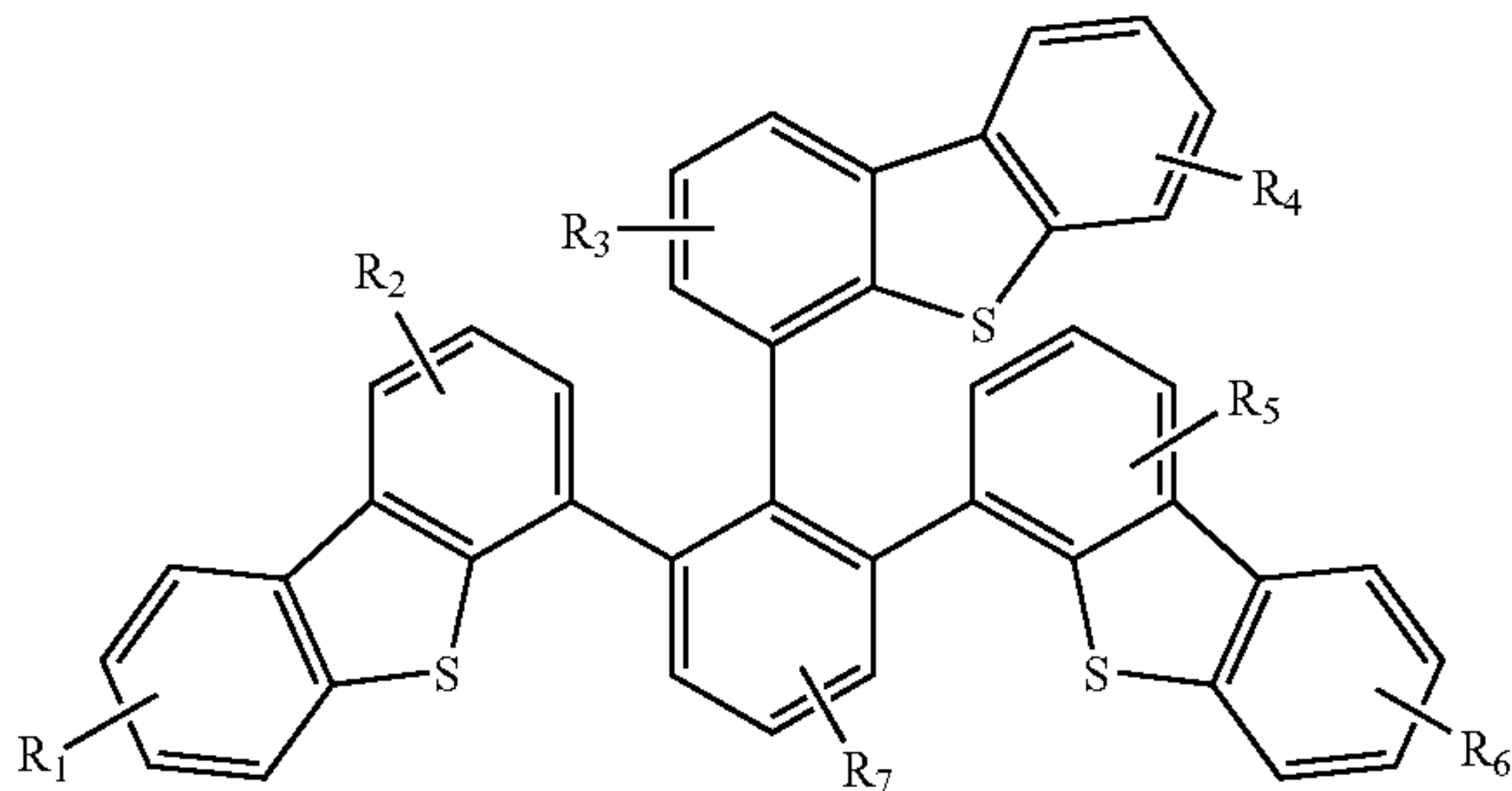
Compound 20G
