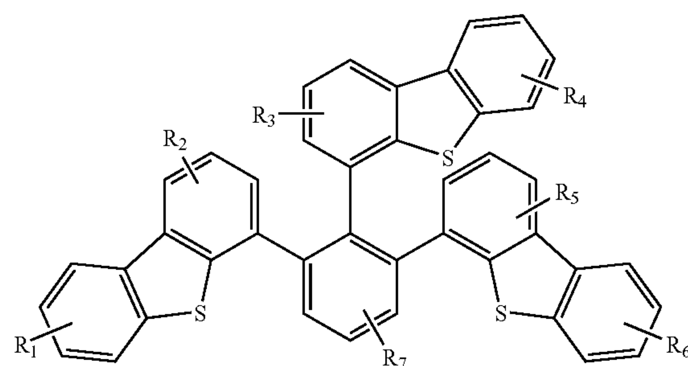
Compound 21G
