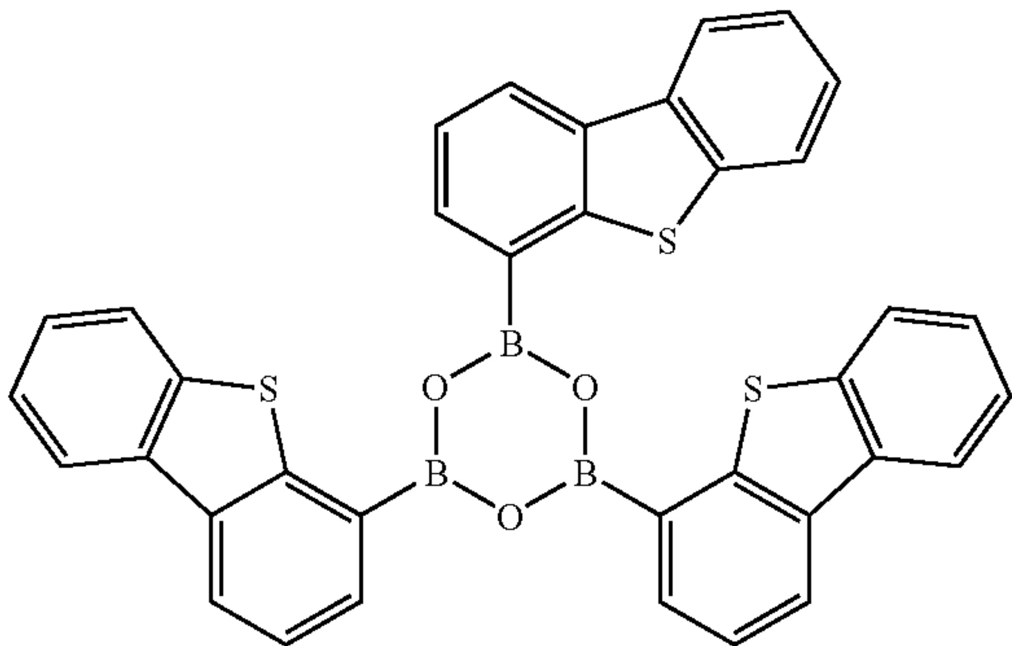
Compound 9
