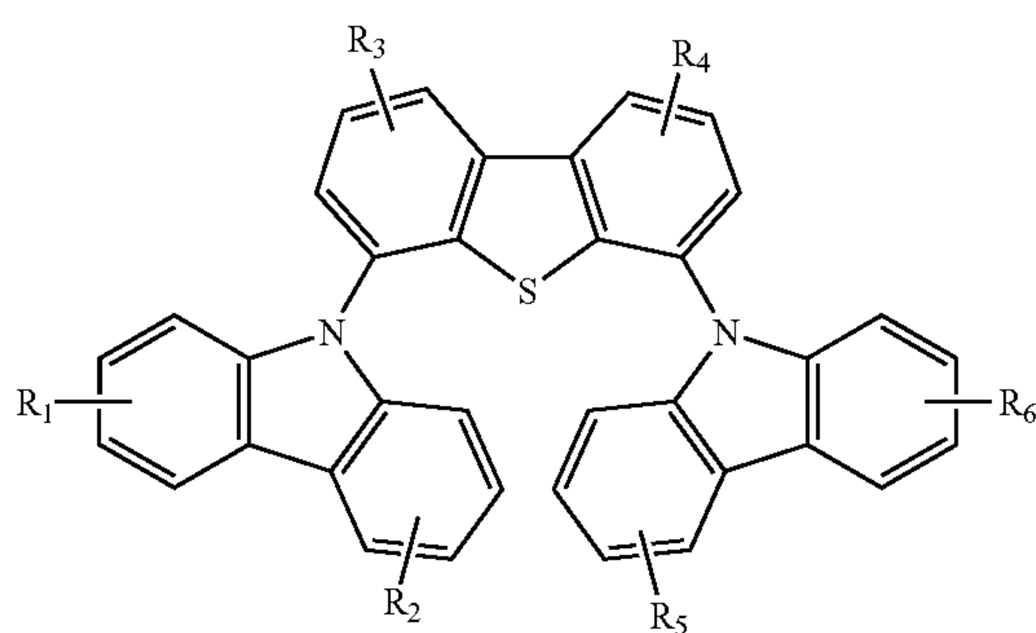
Compound 4G
