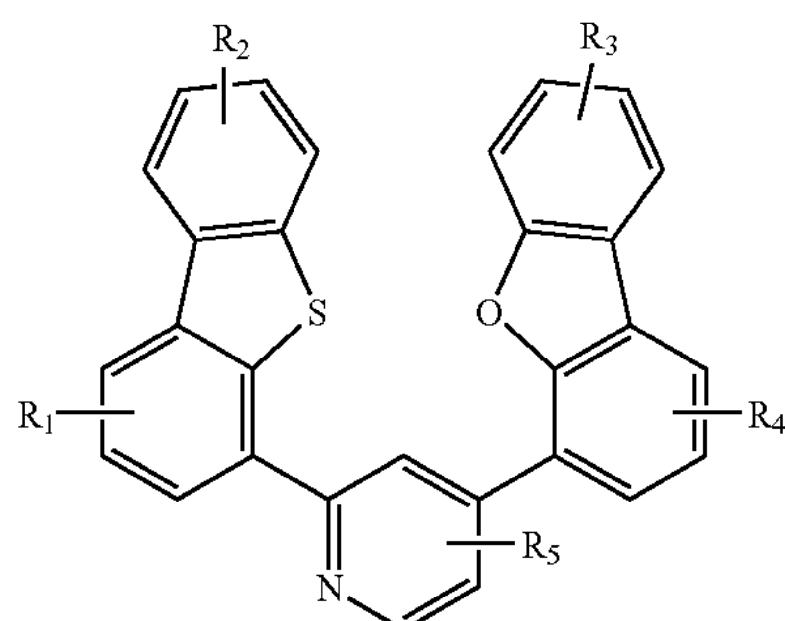
Compound 32G
