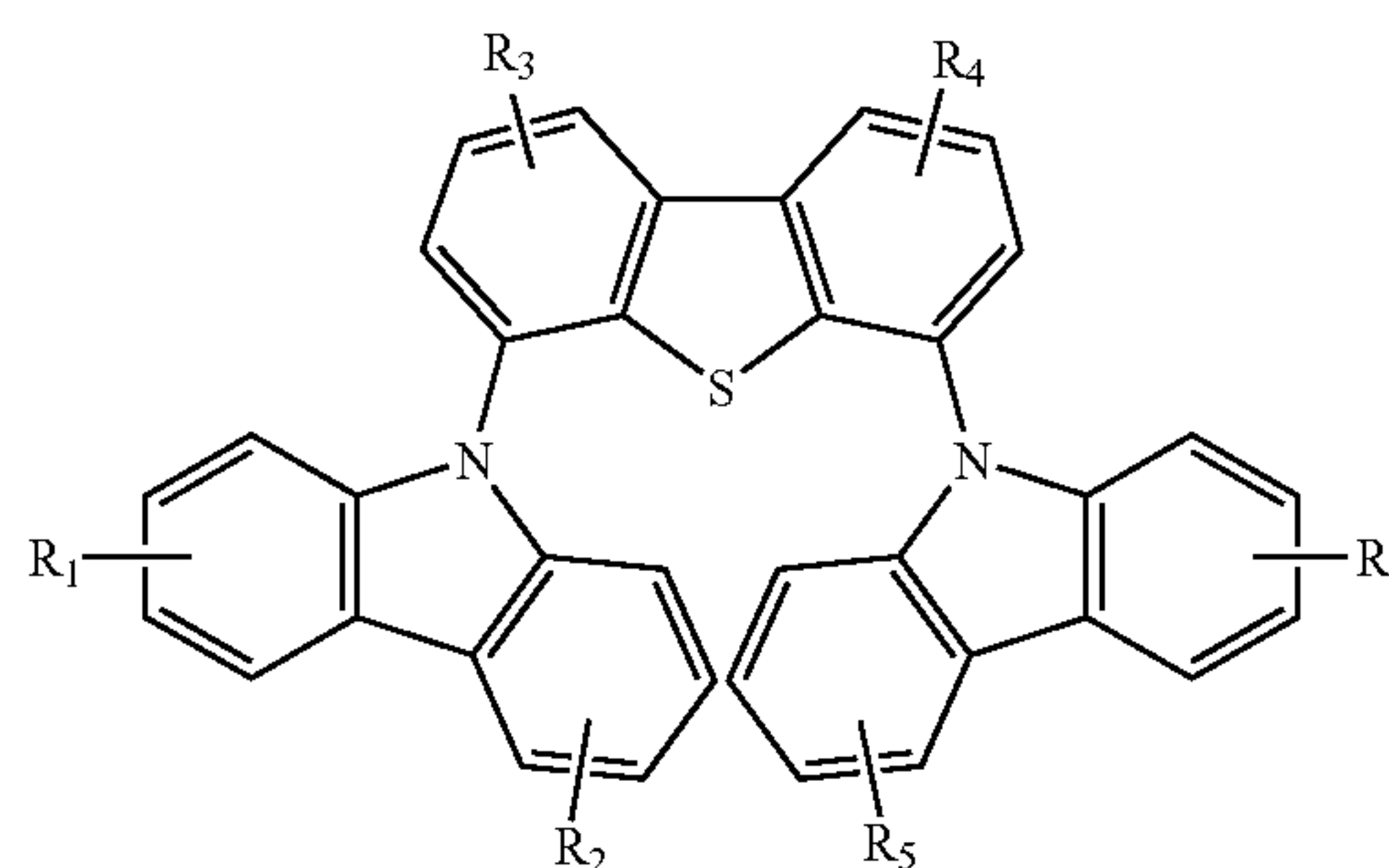
Compound 4G
