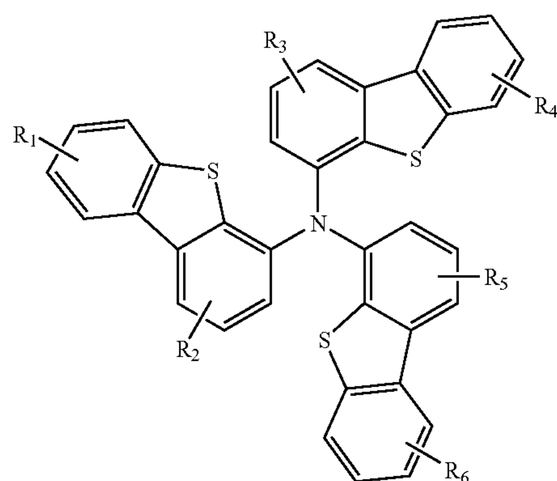
Compound 9G
