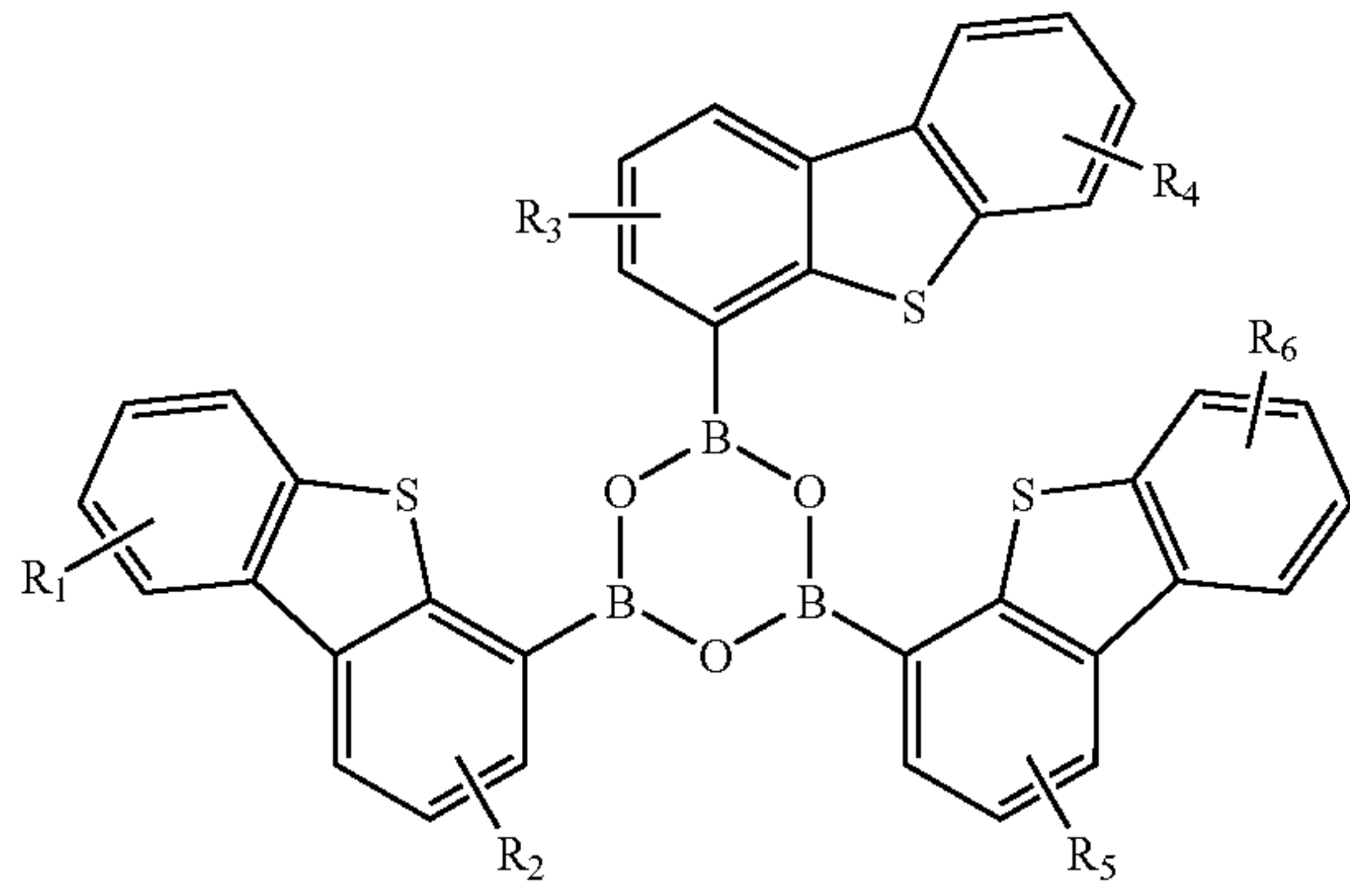
Compound 8G
