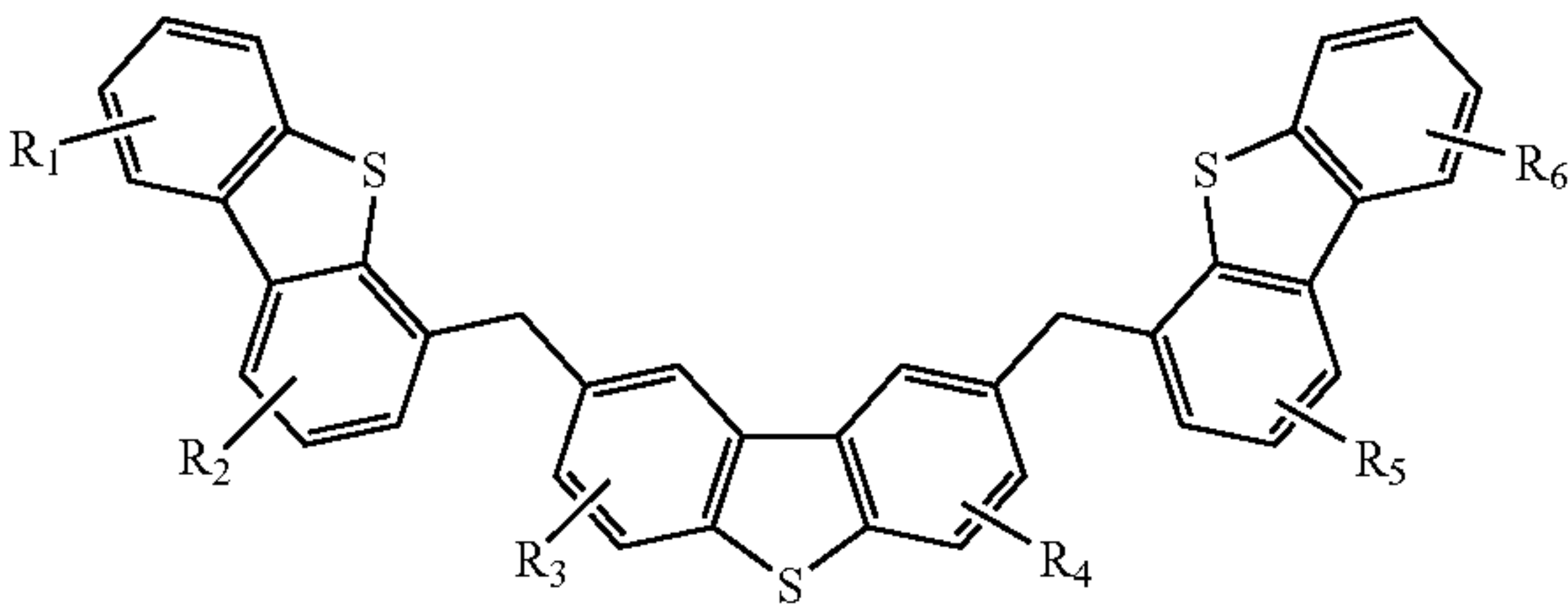
Compound 16G
