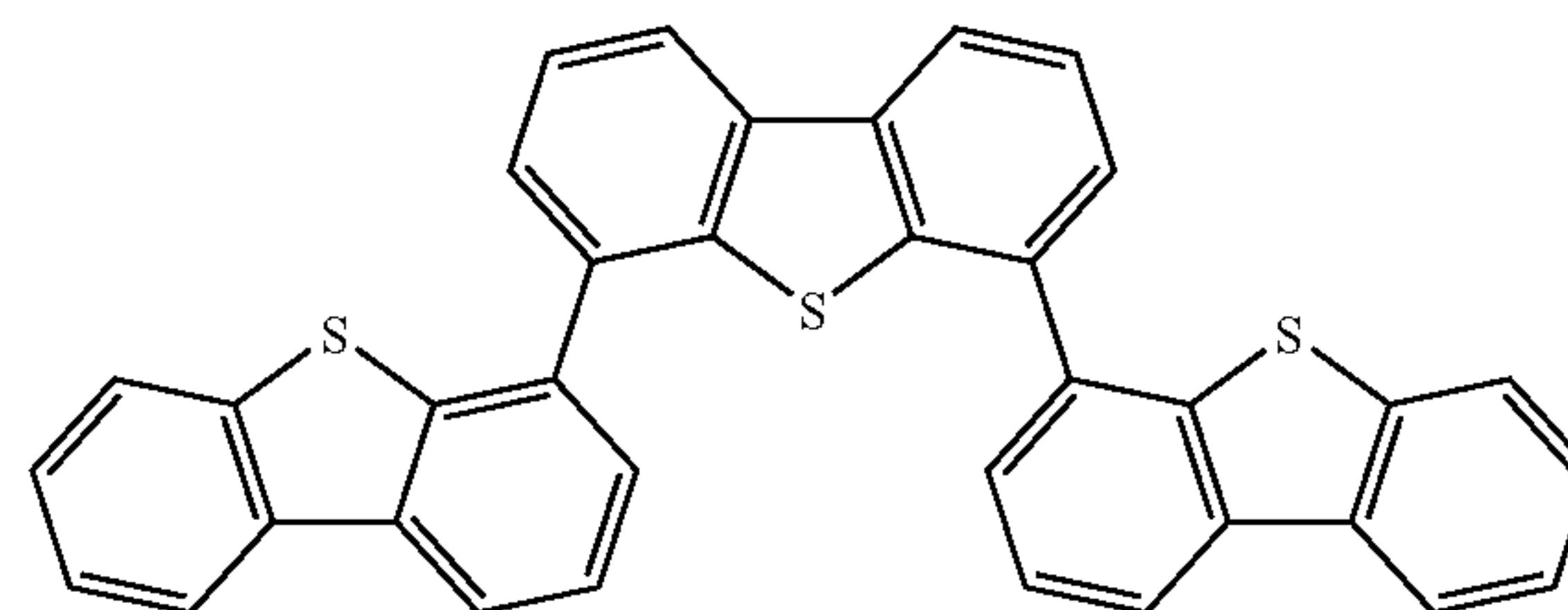
Compound 4
