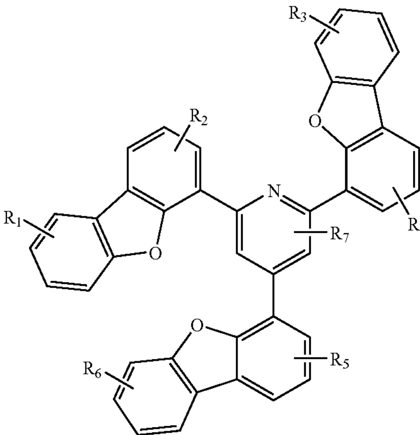
Compound 34G
