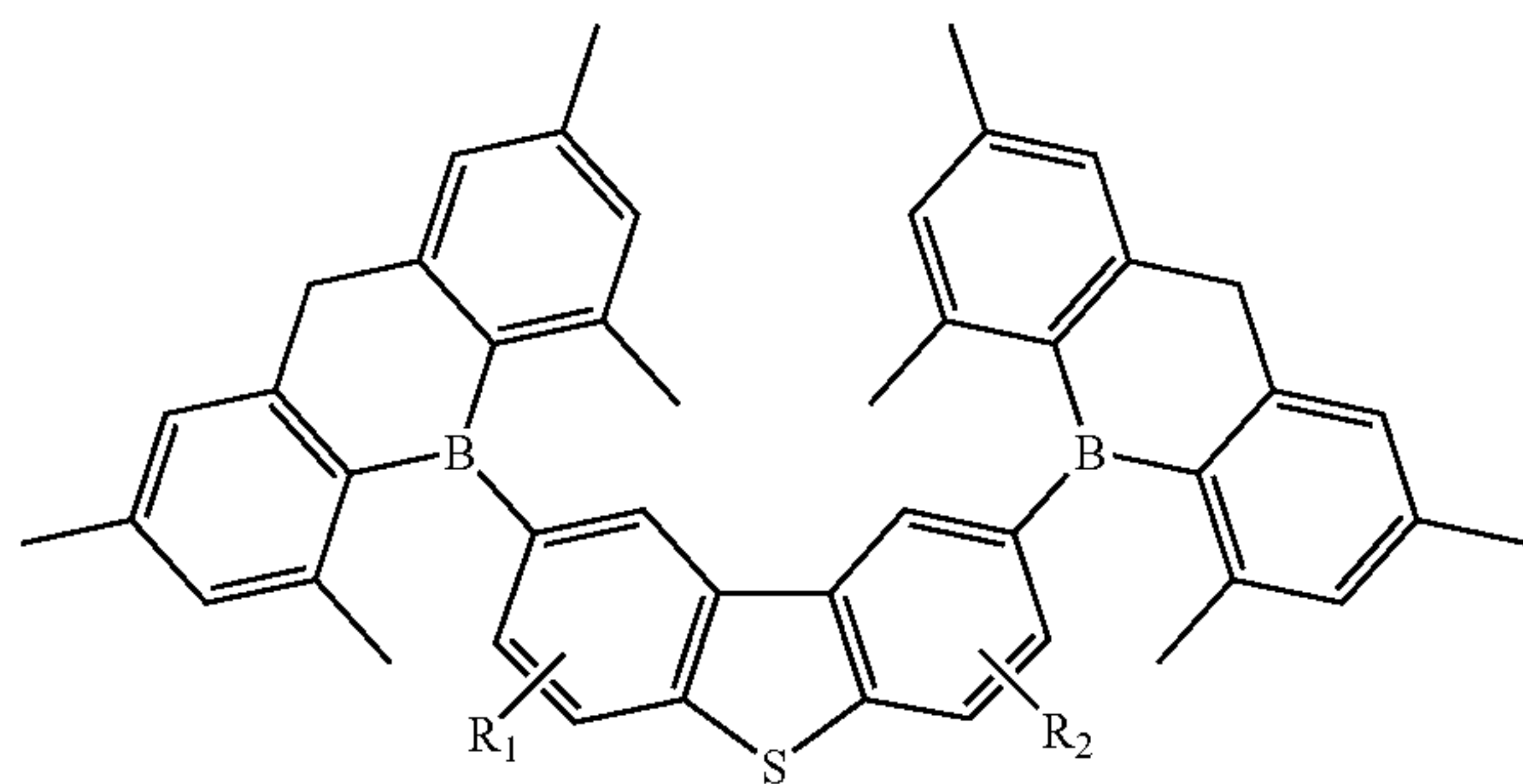
Compound 7G
