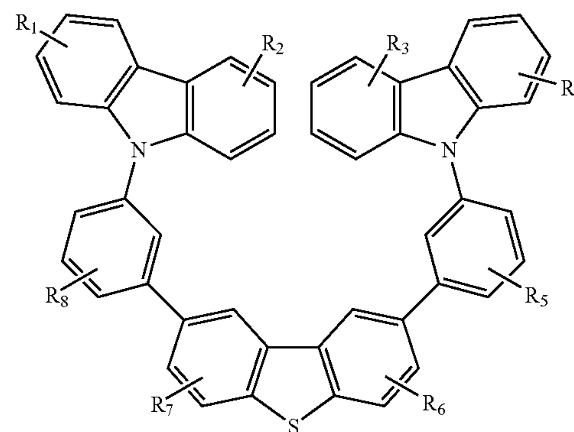
Compound 19G
