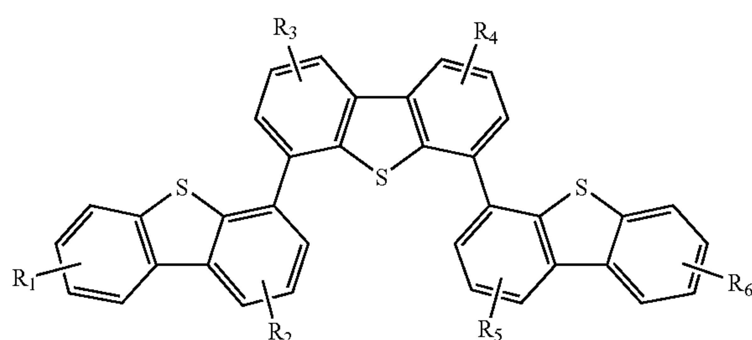
Compound 3G
