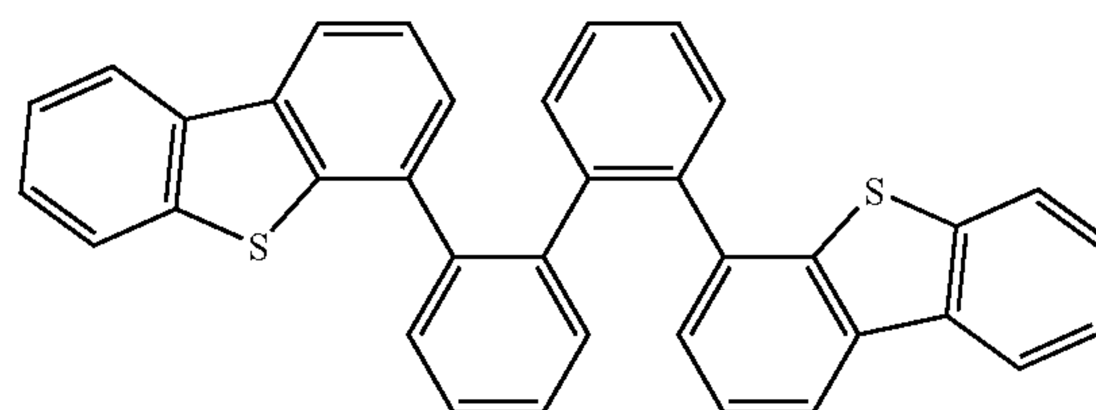
Compound 2
