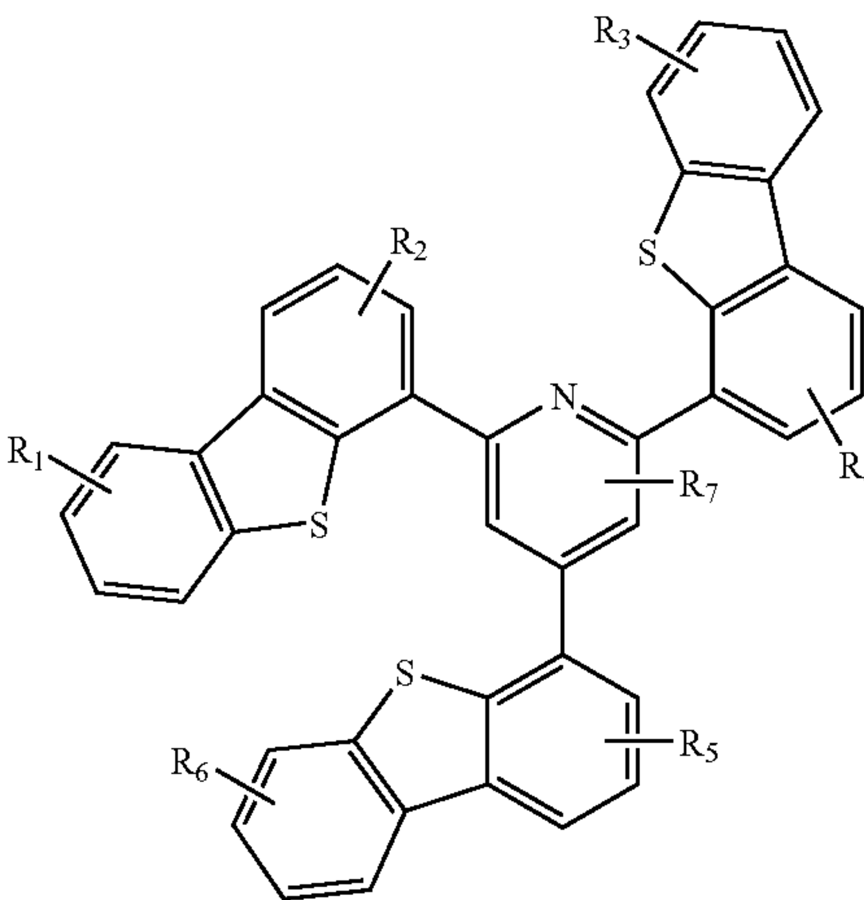
Compound 34G
