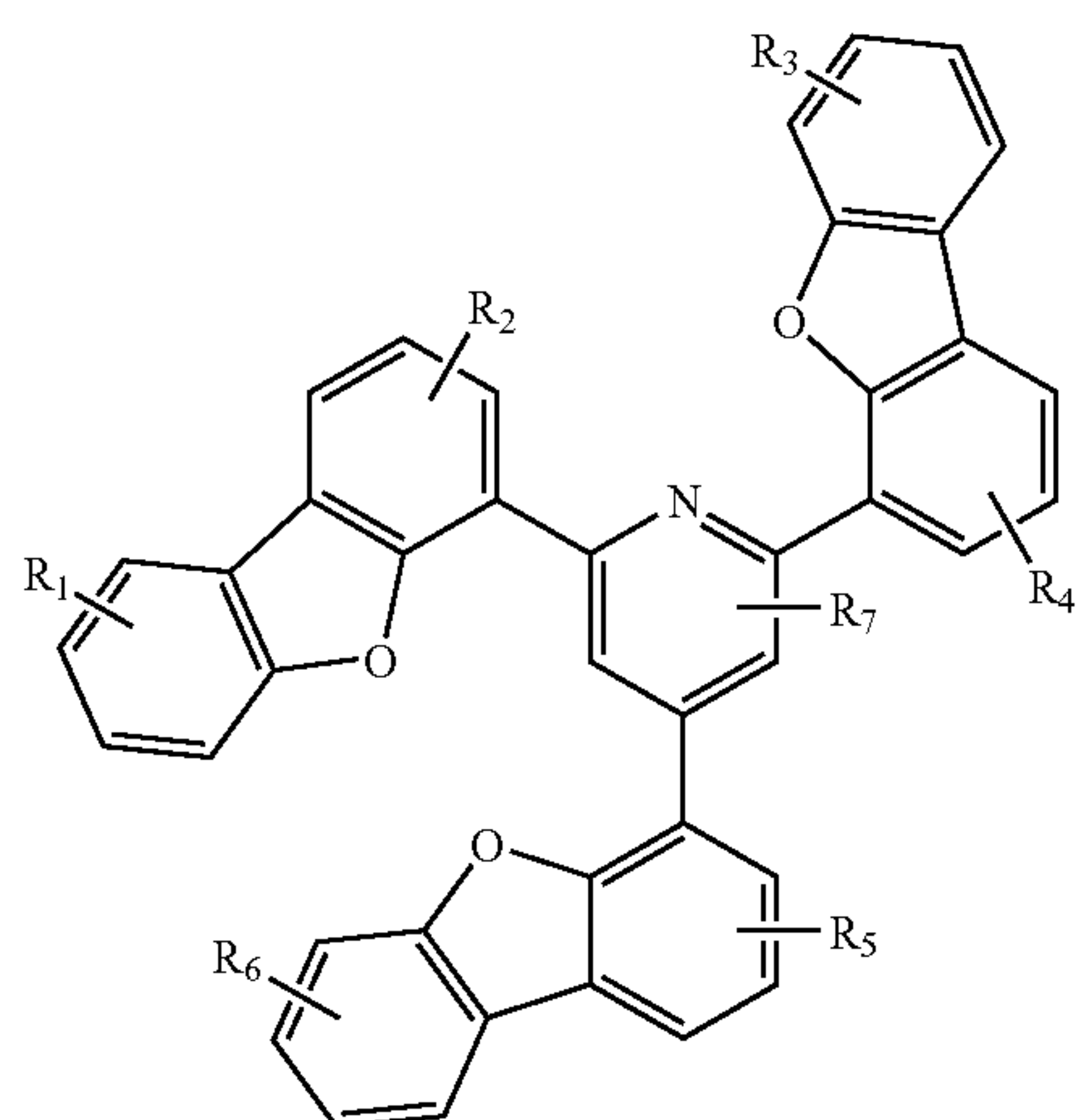
Compound 34G
