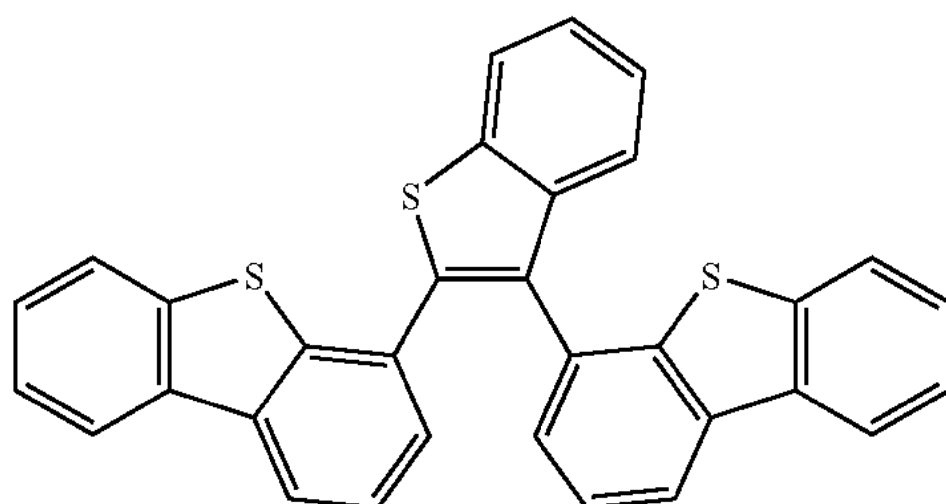
Compound 10
