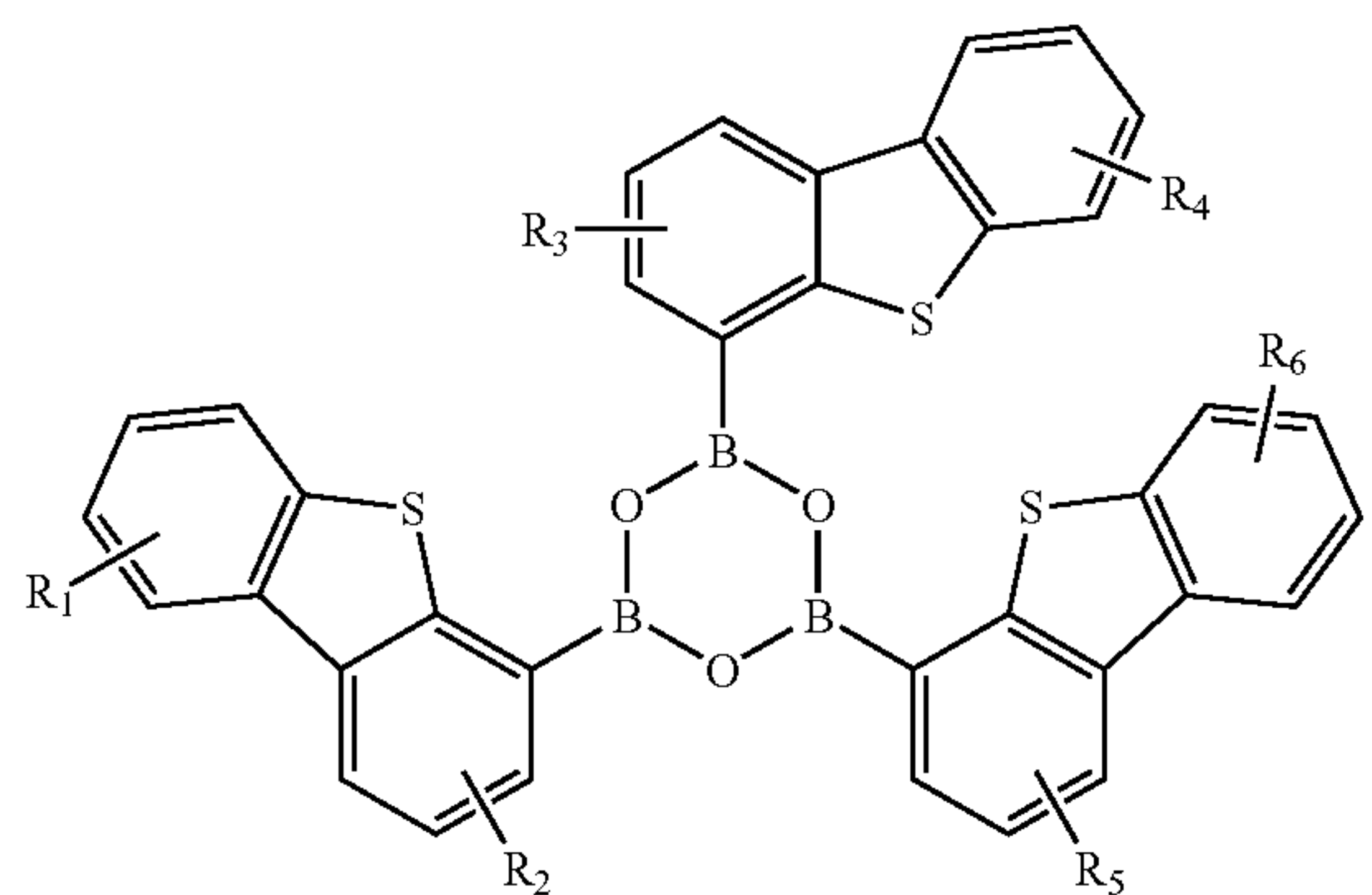
Compound 8G
