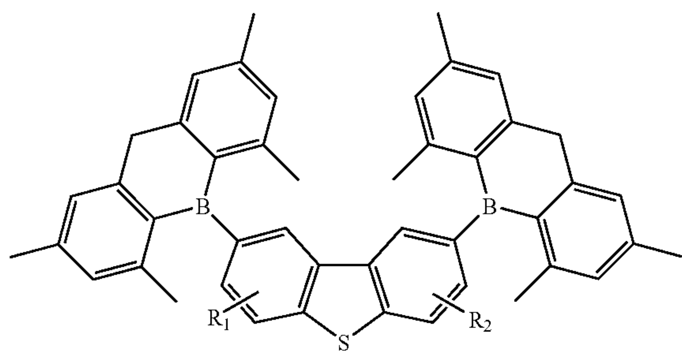
Compound 8G
