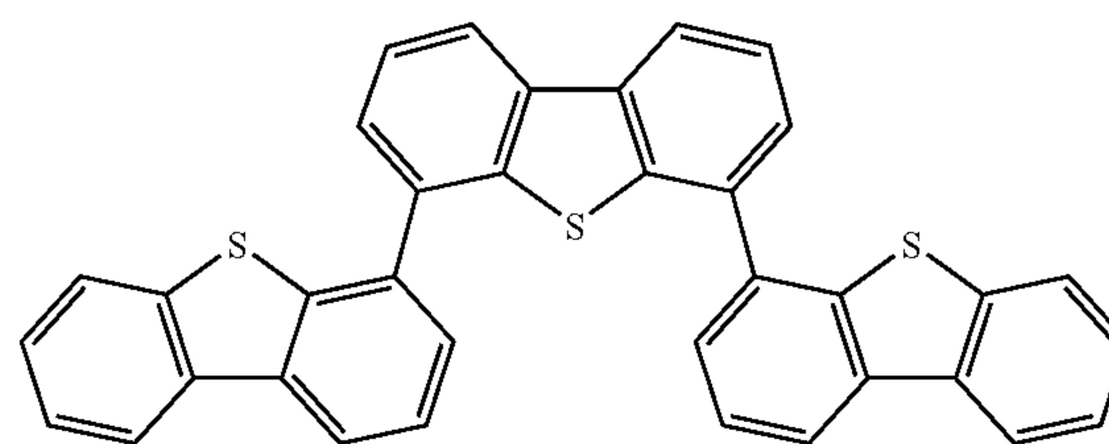
Compound 4
