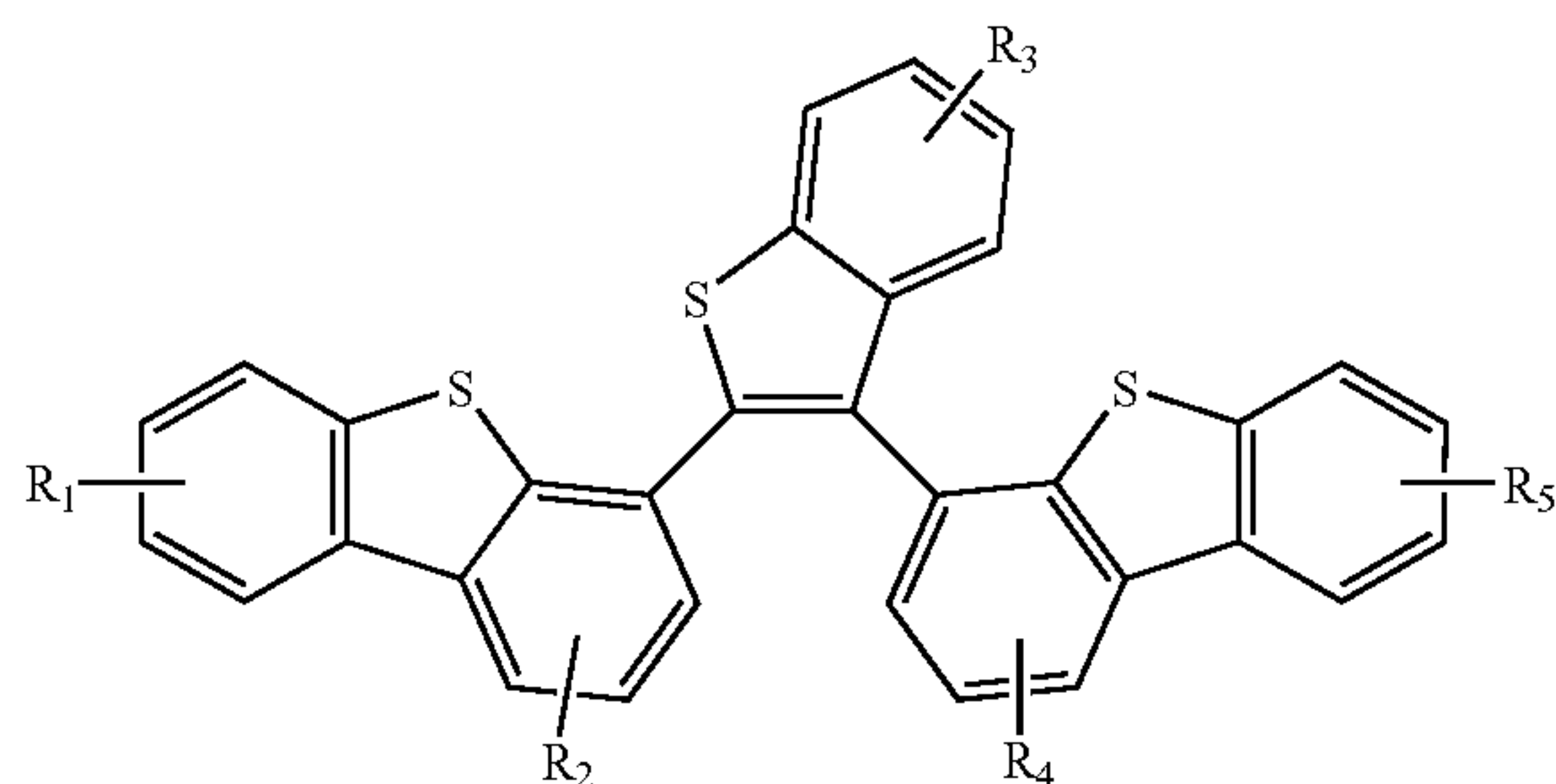
Compound 11G
