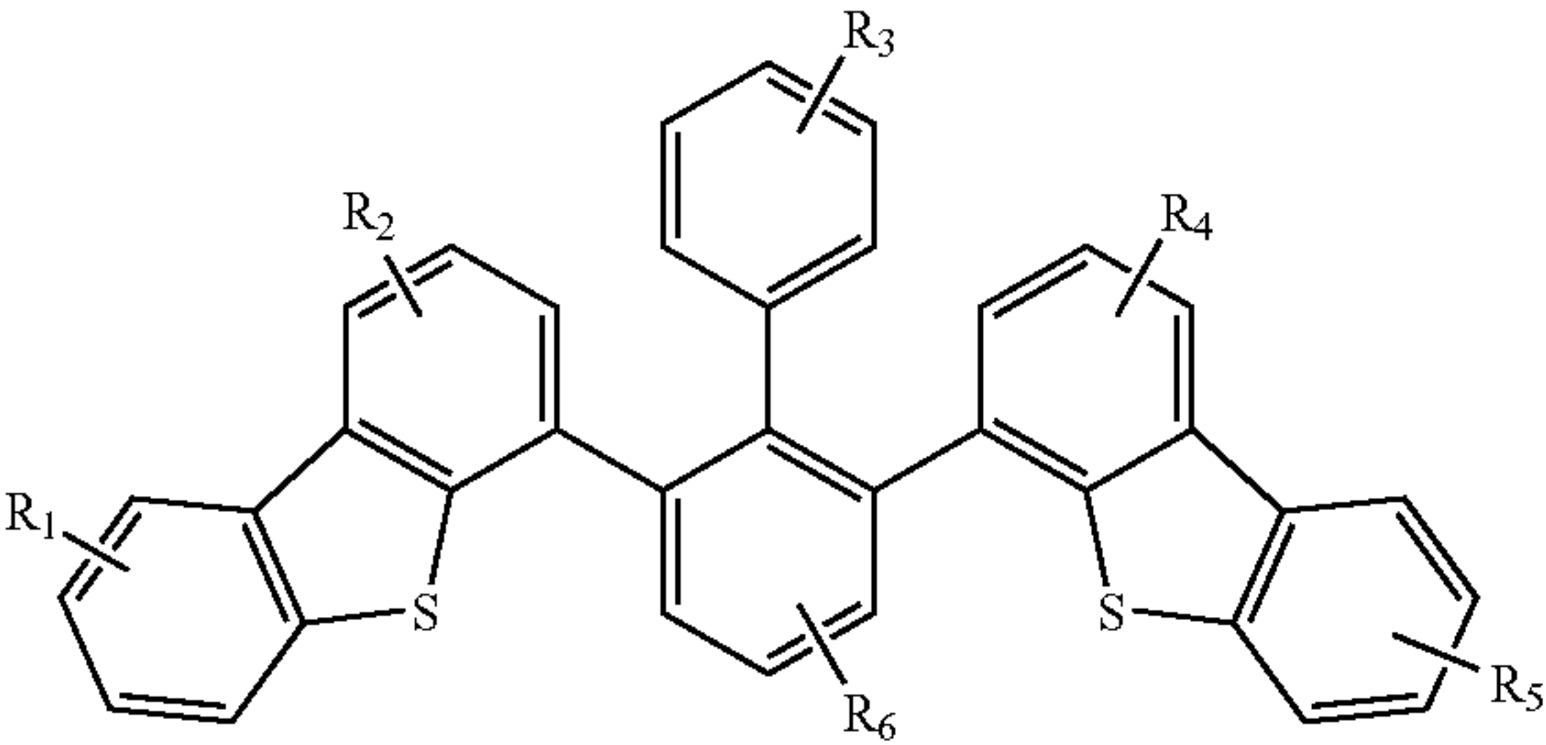
Compound 22G
