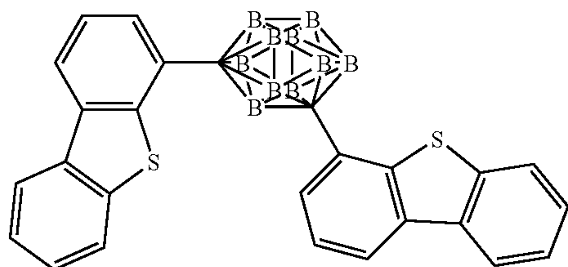
Compound 14
