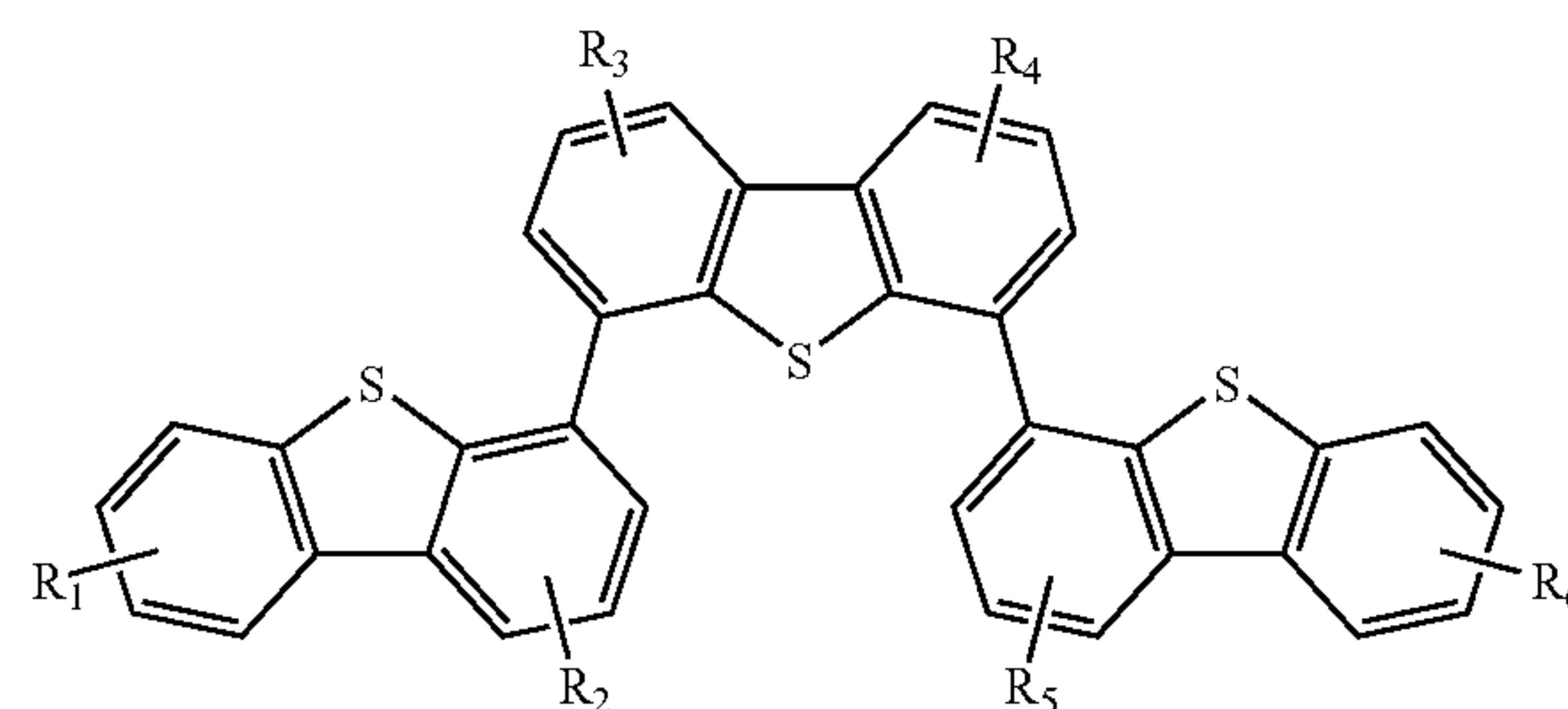
Compound 3G
