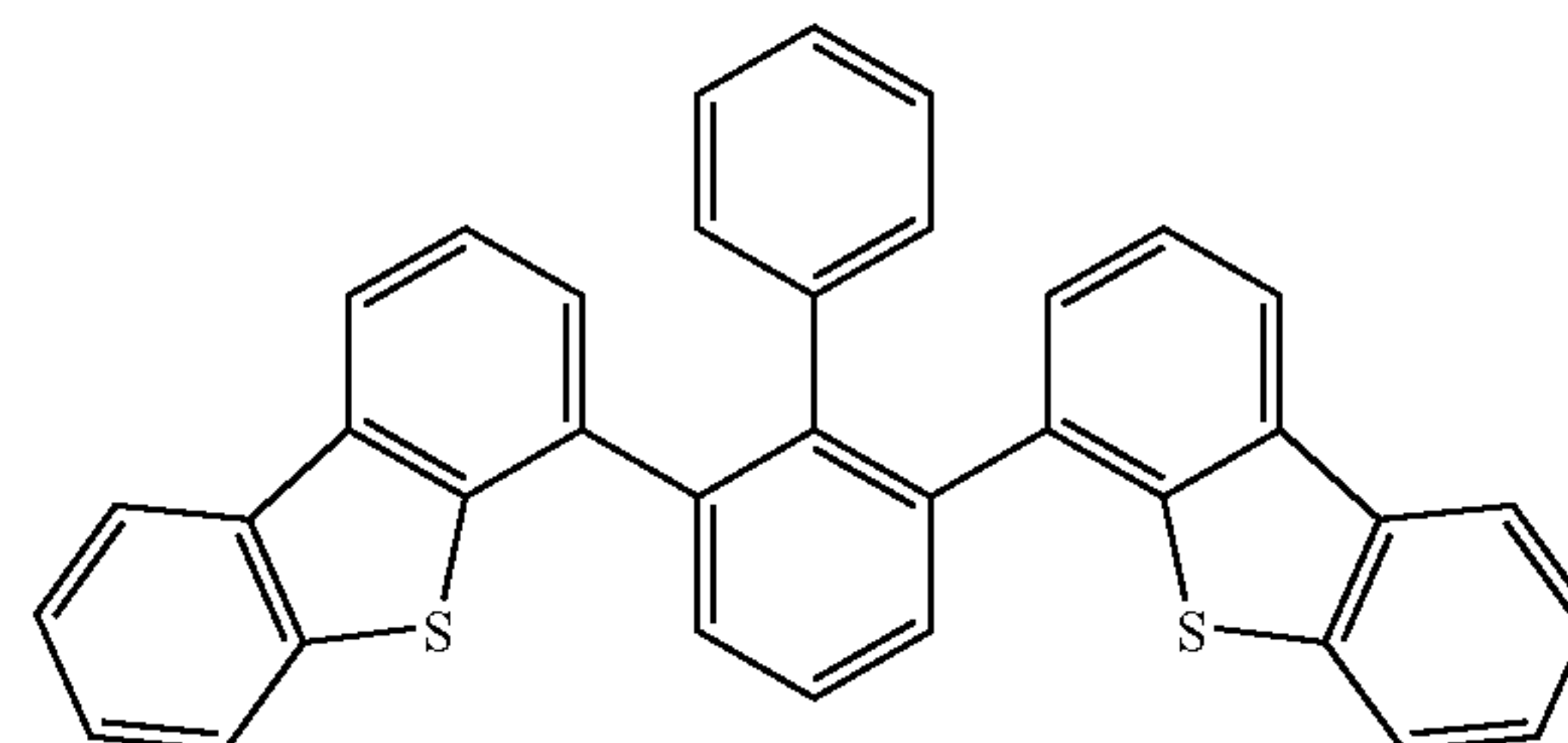
Compound 22
