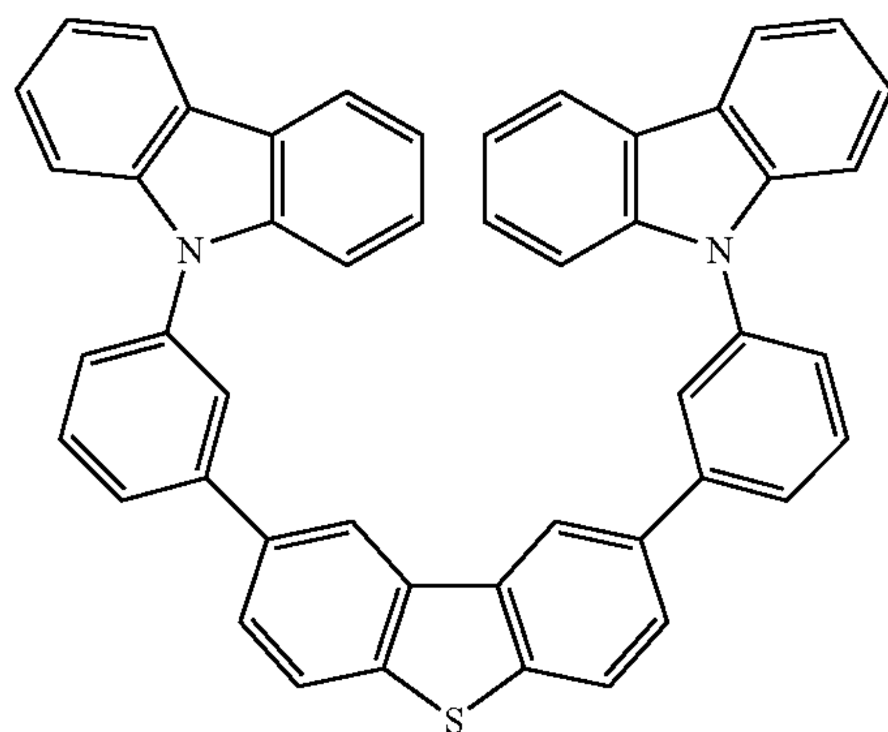
Compound 18
