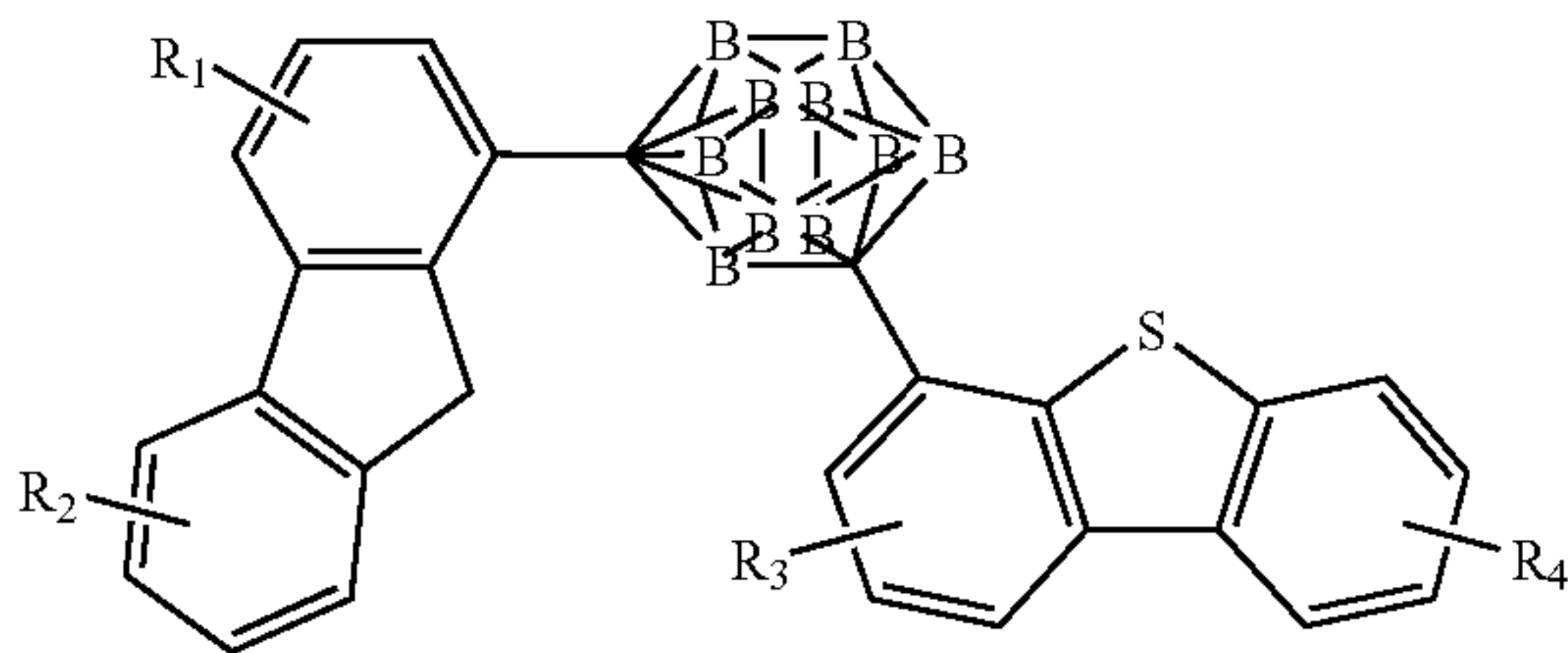
Compound 14G
