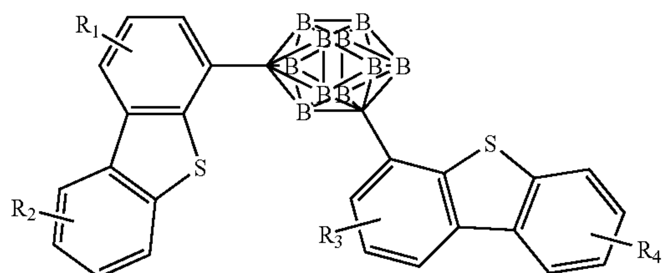
Compound 15G
