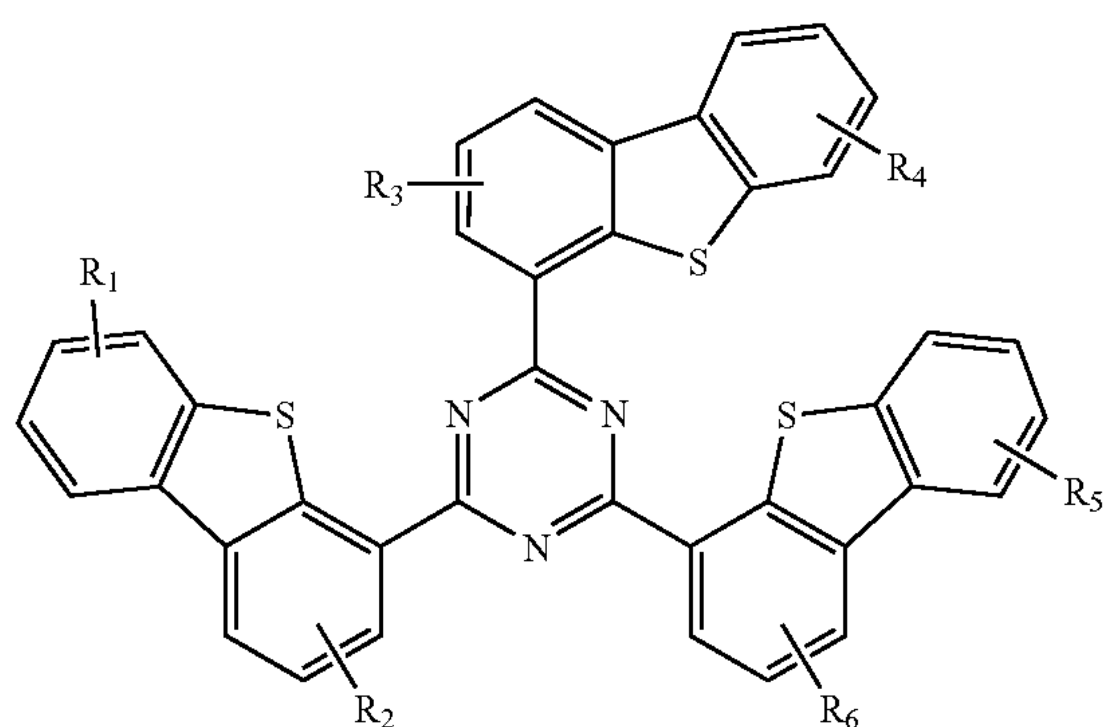
Compound 7G
