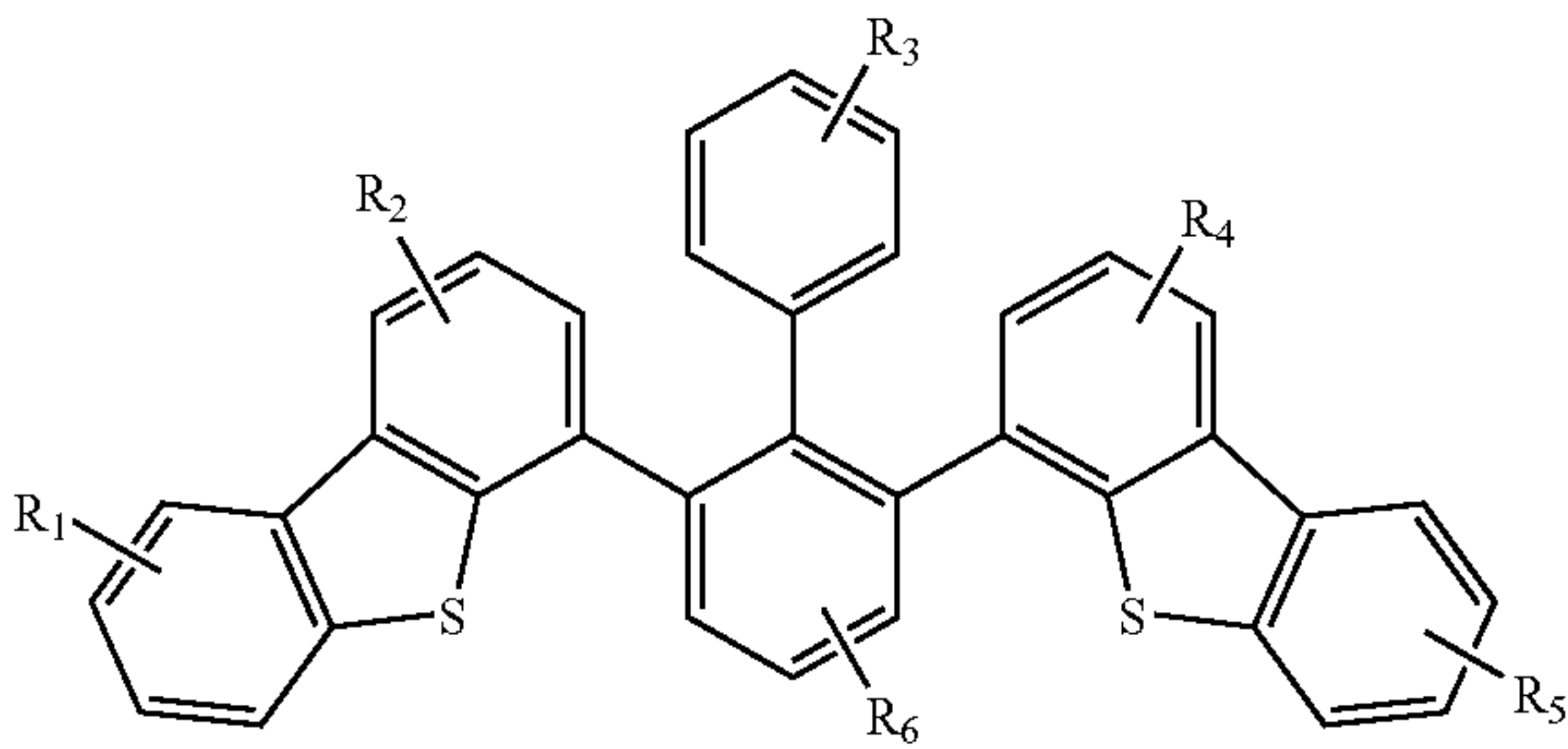
Compound 22G
