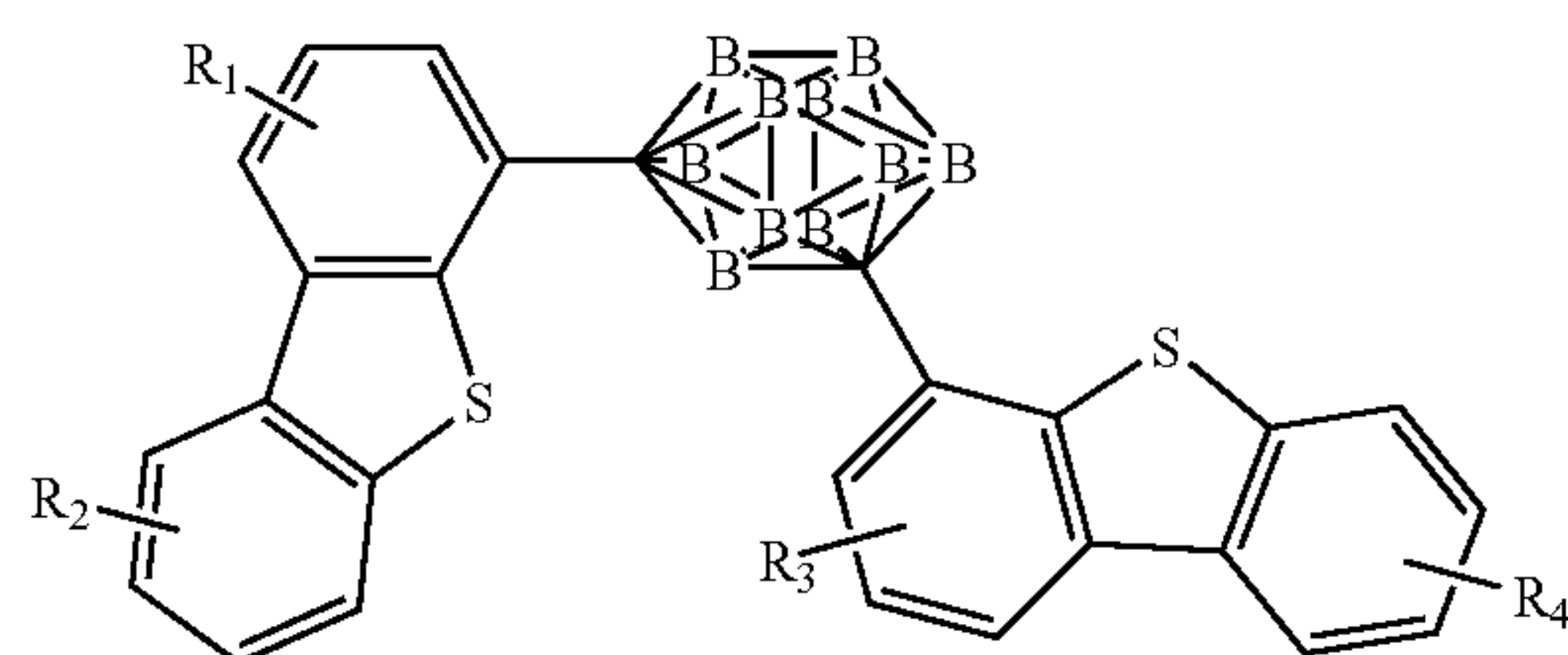
Compound 14G
