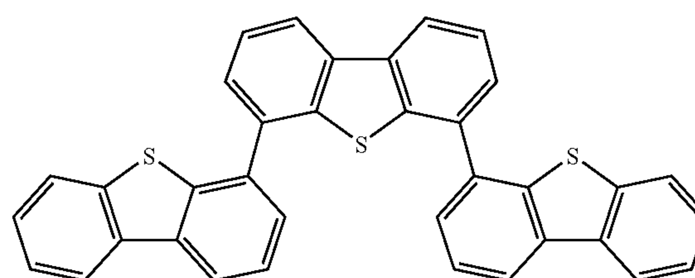
Compound 4
