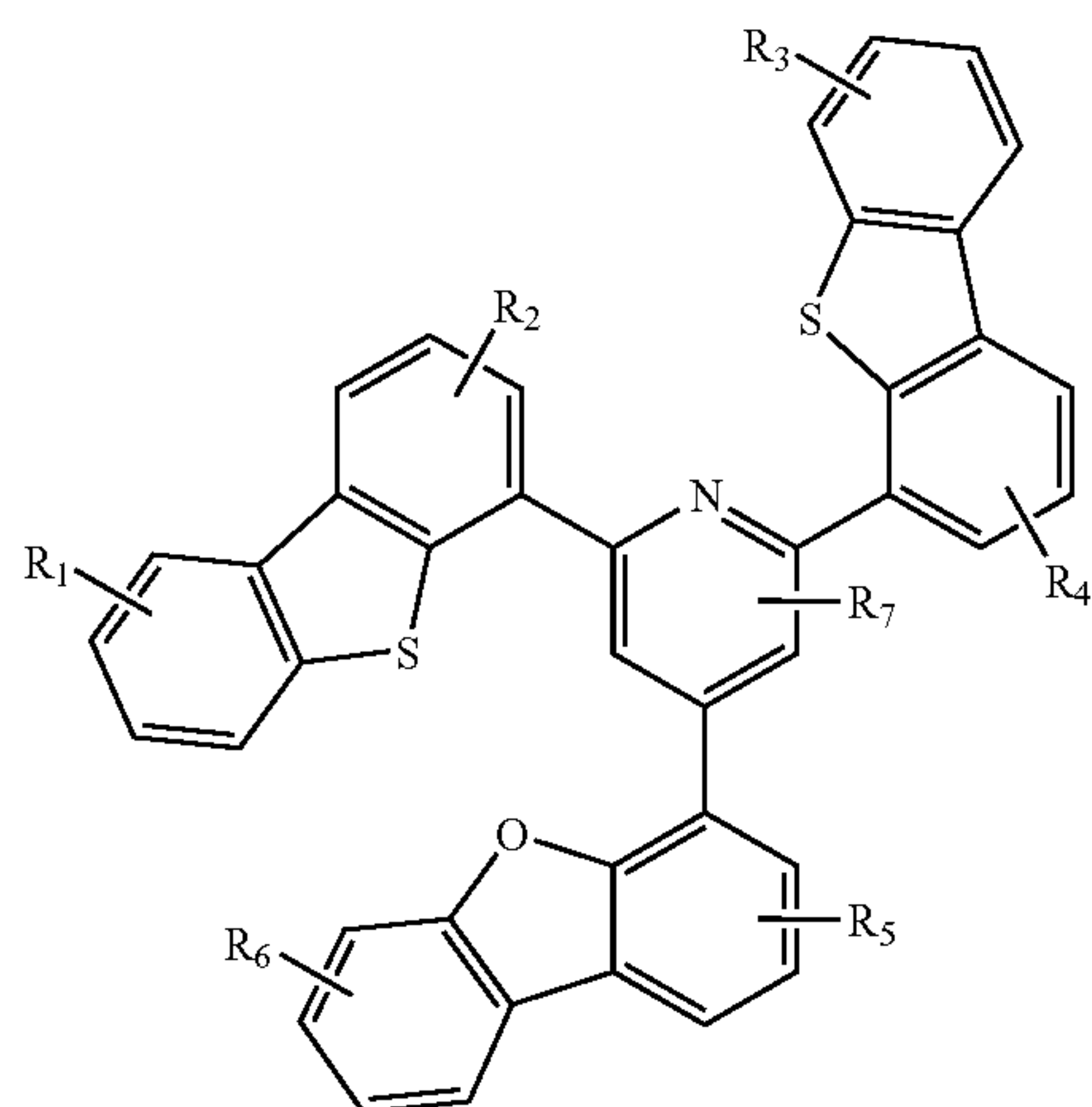
Compound 35G
