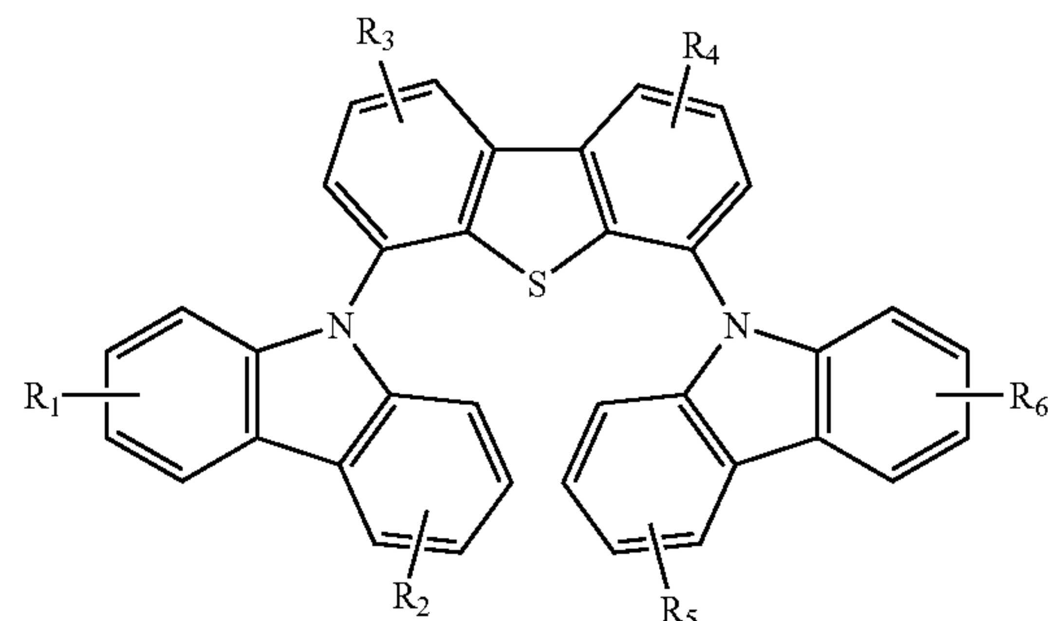
Compound 5G
