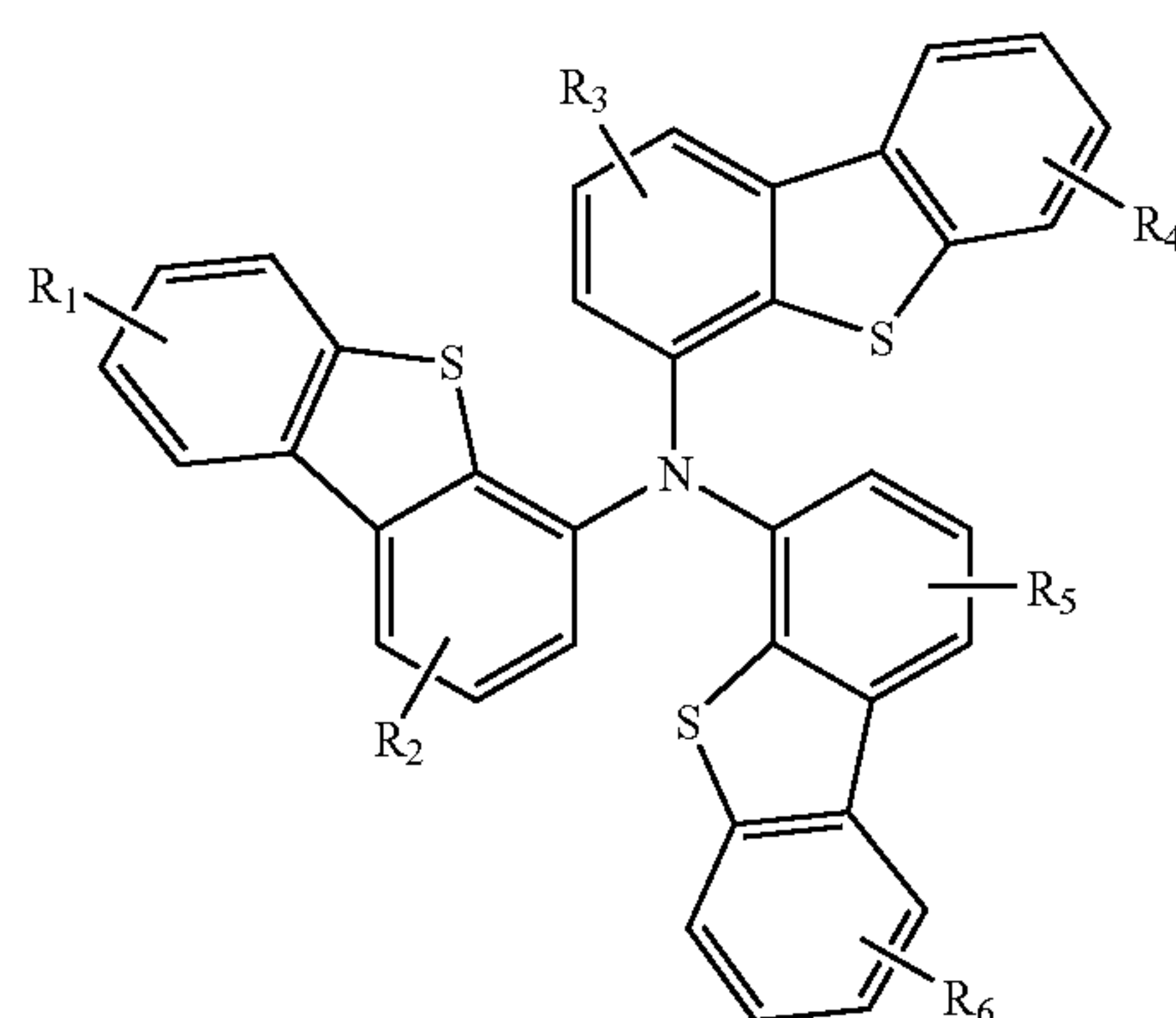
Compound 9G
