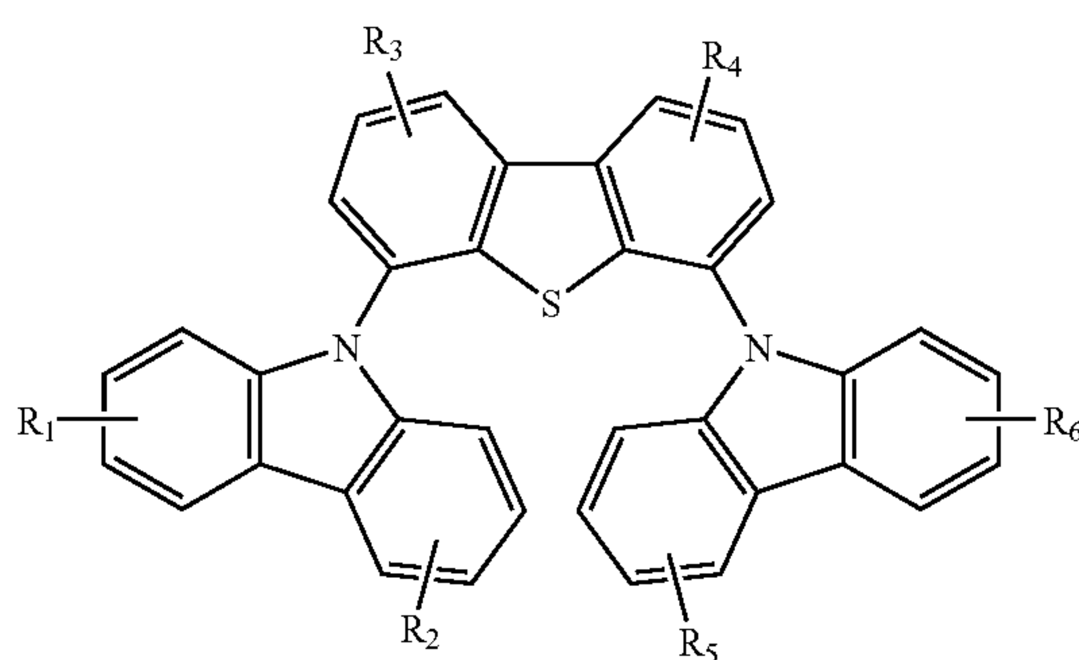
Compound 4G
