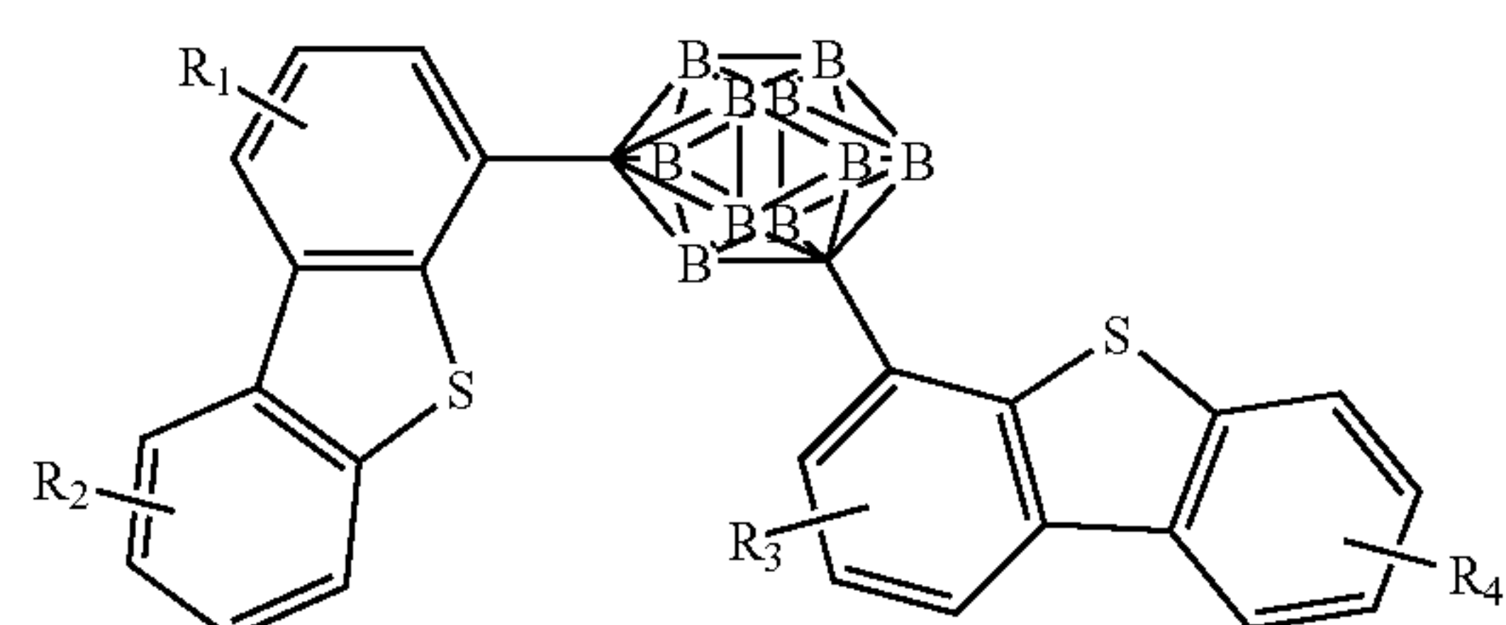
Compound 14G
