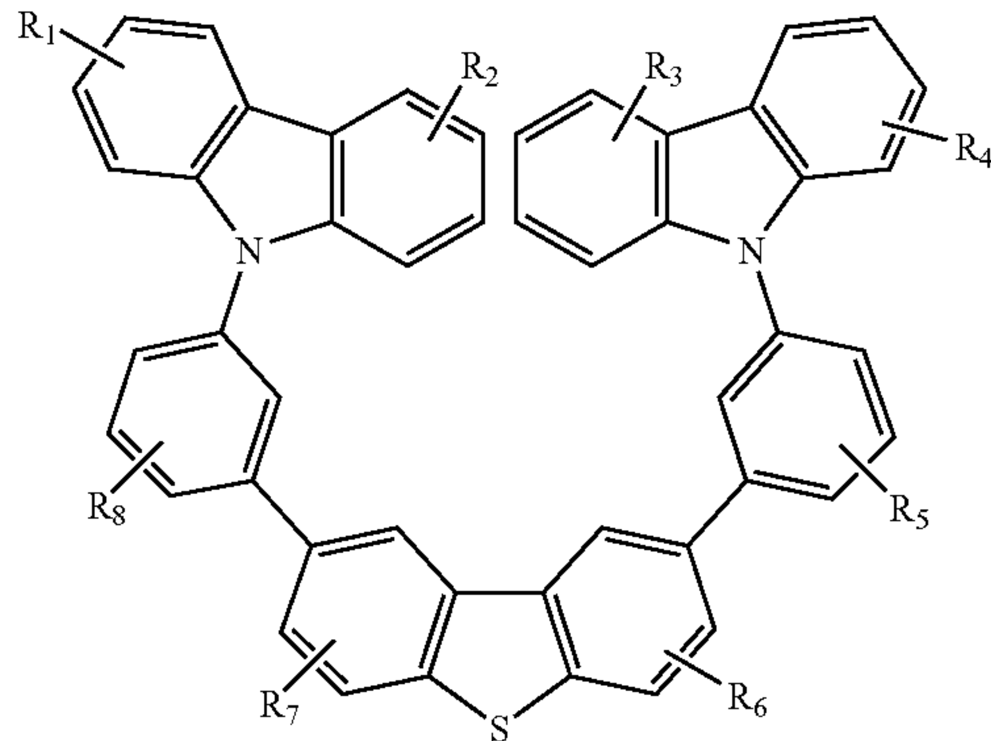
Compound 18G
