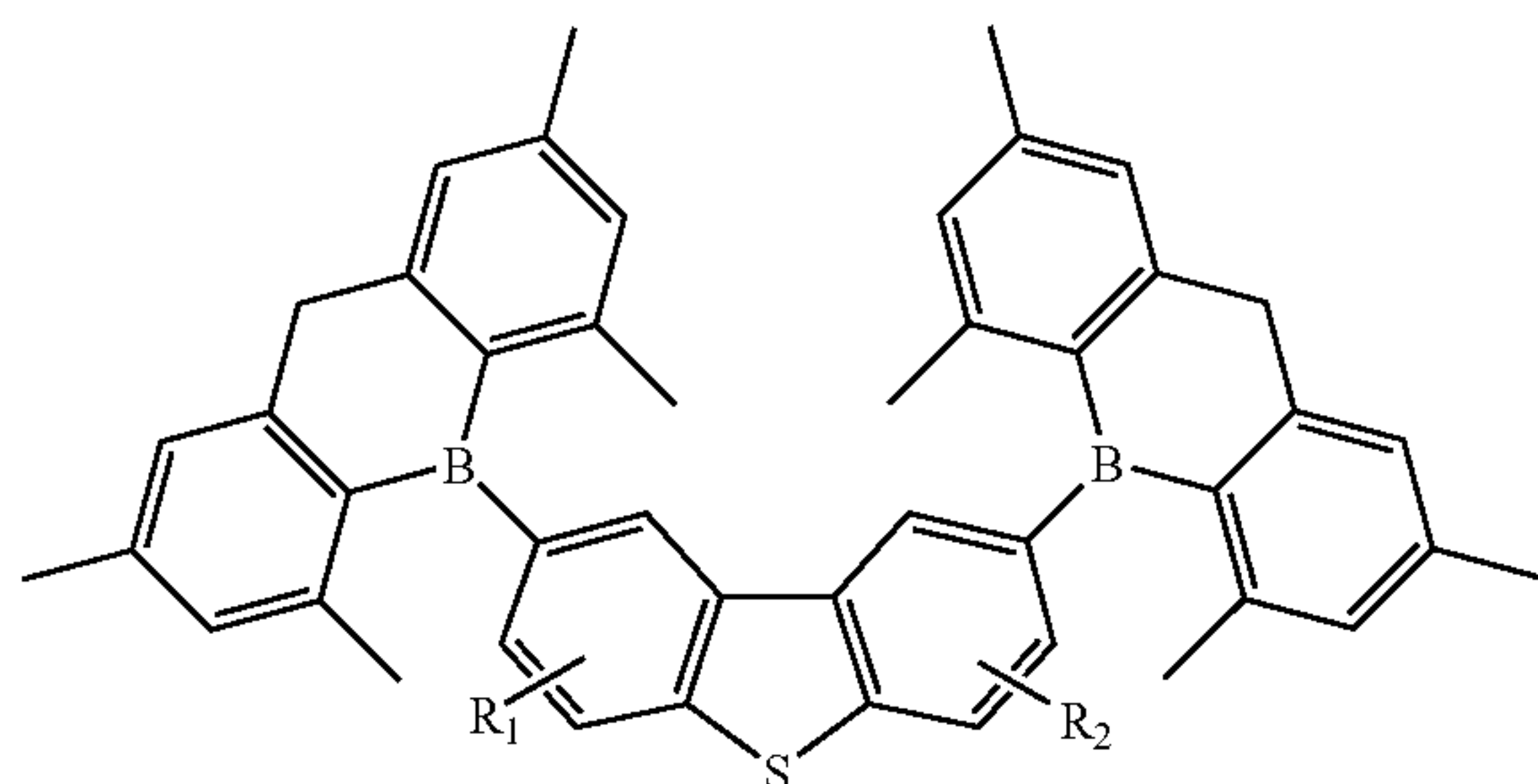
Compound 7G
