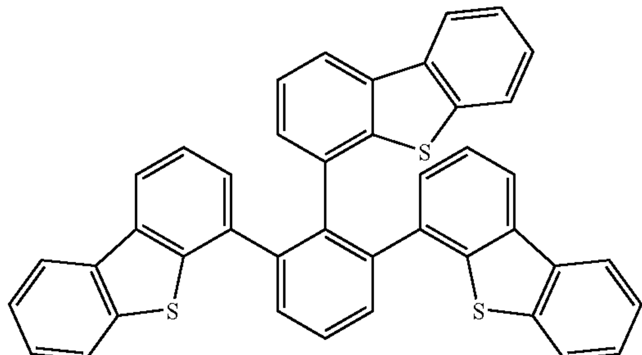
Compound 20
