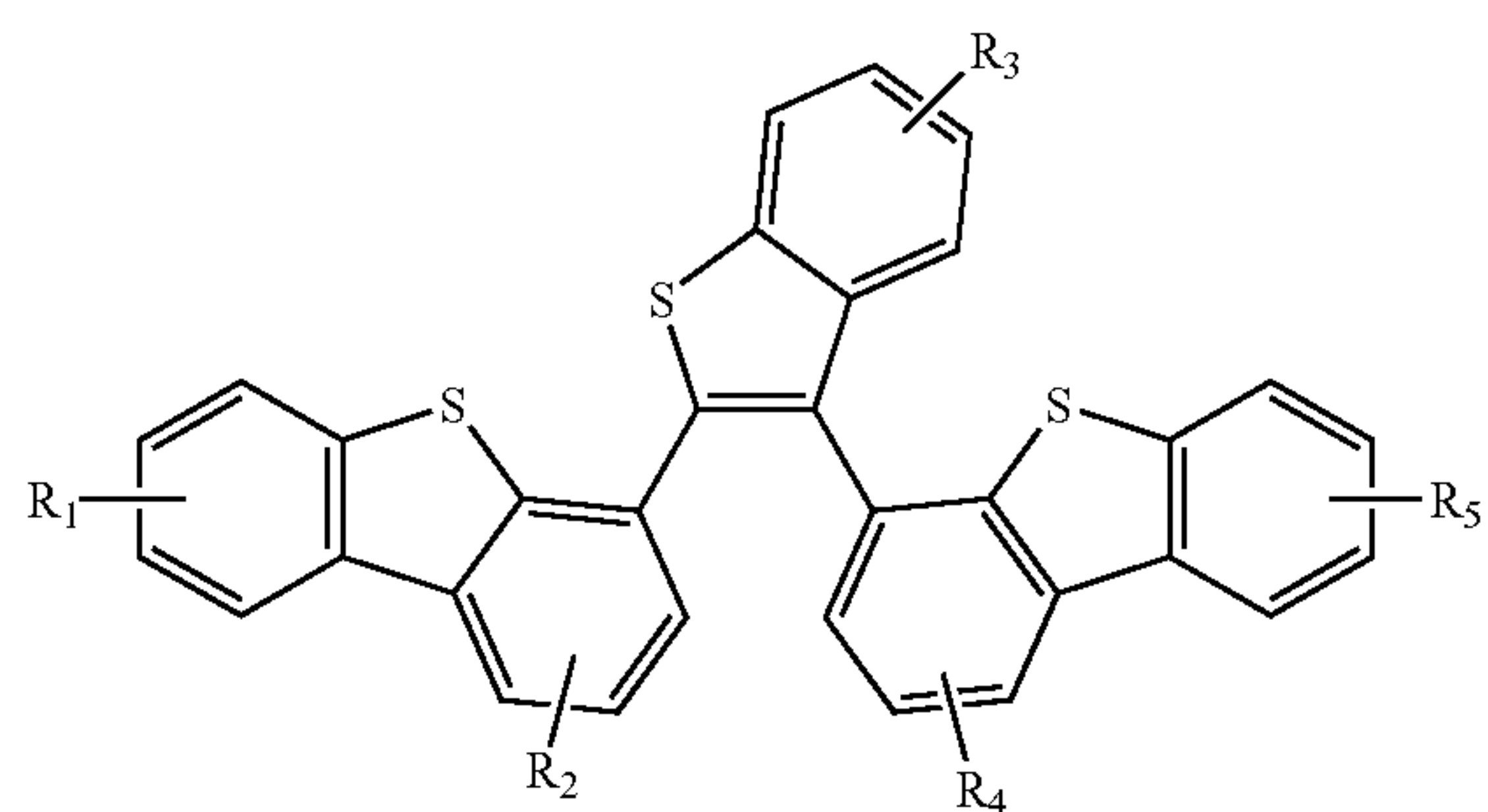
Compound 10G
