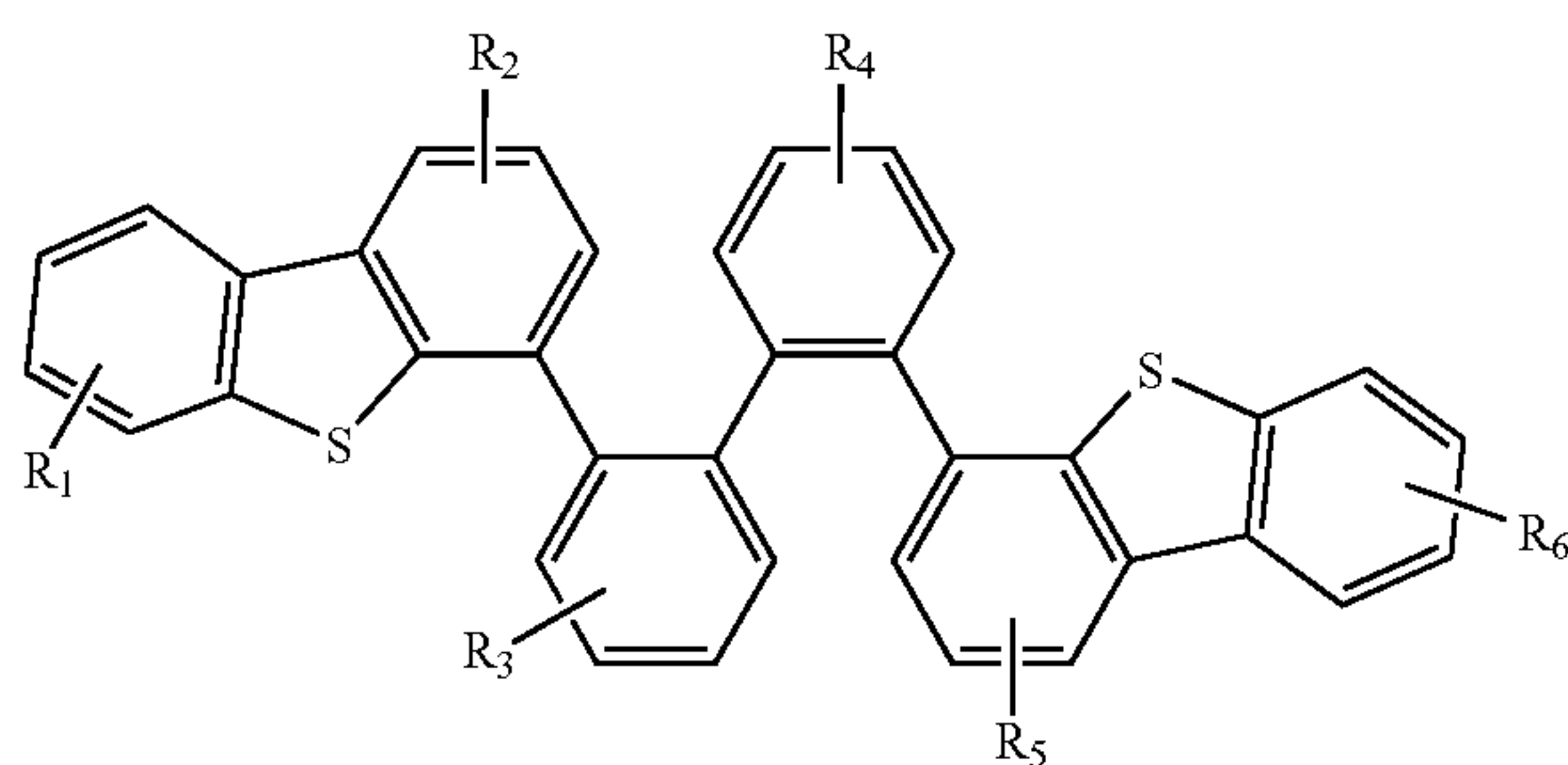
Compound 2G
