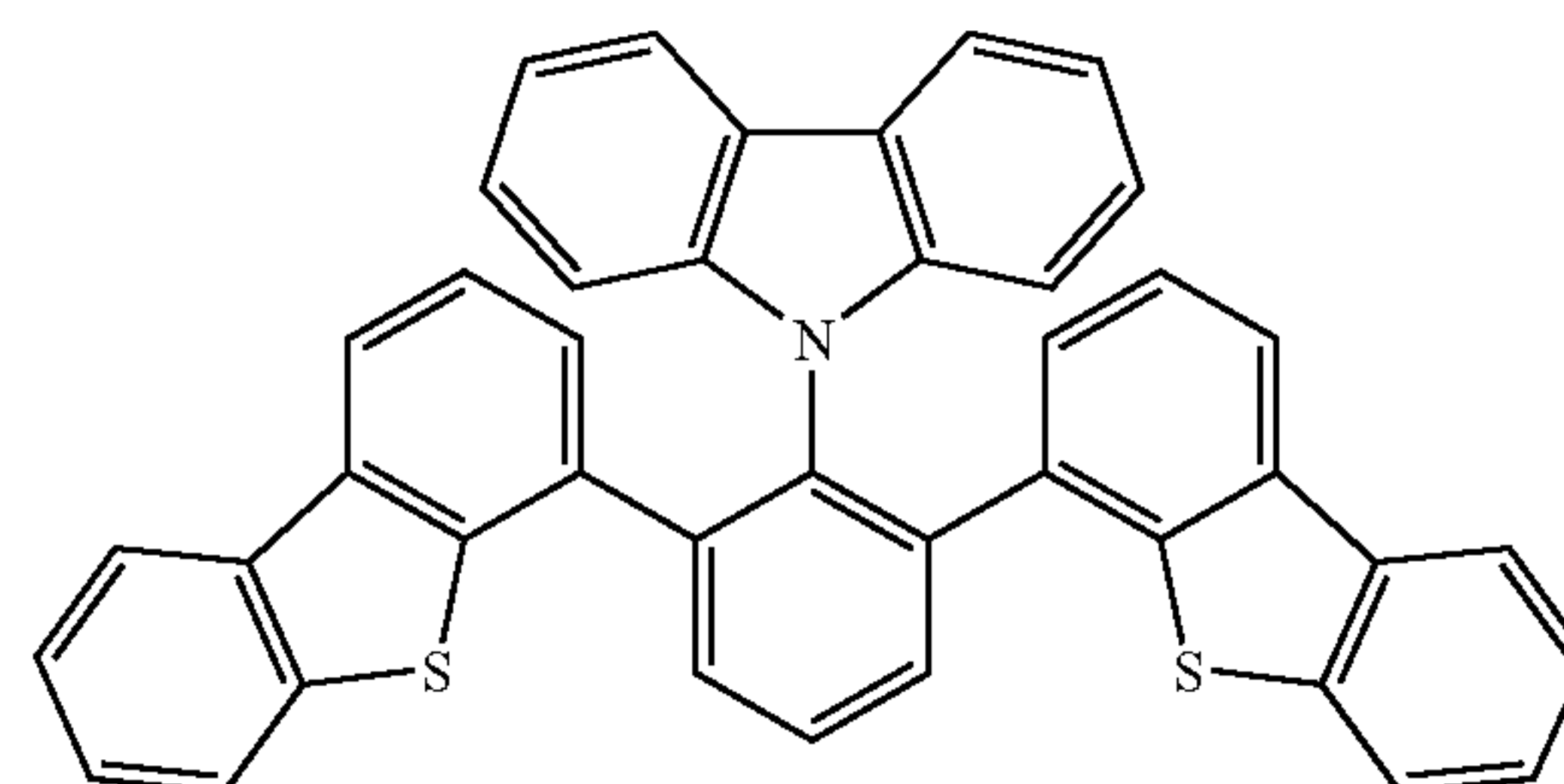
Compound 20
