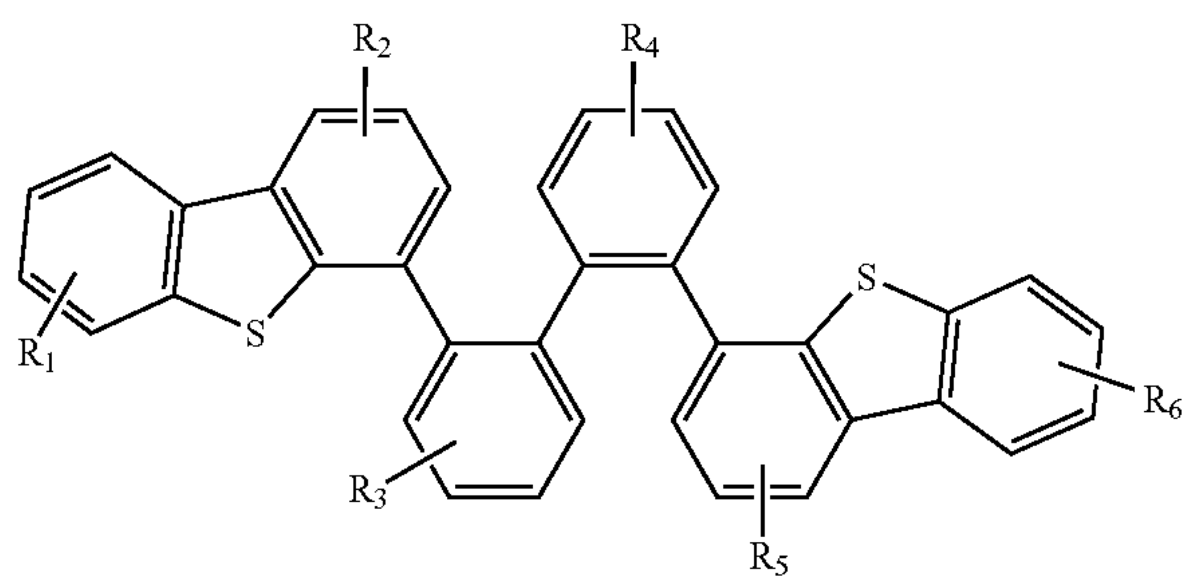
Compound 3G
