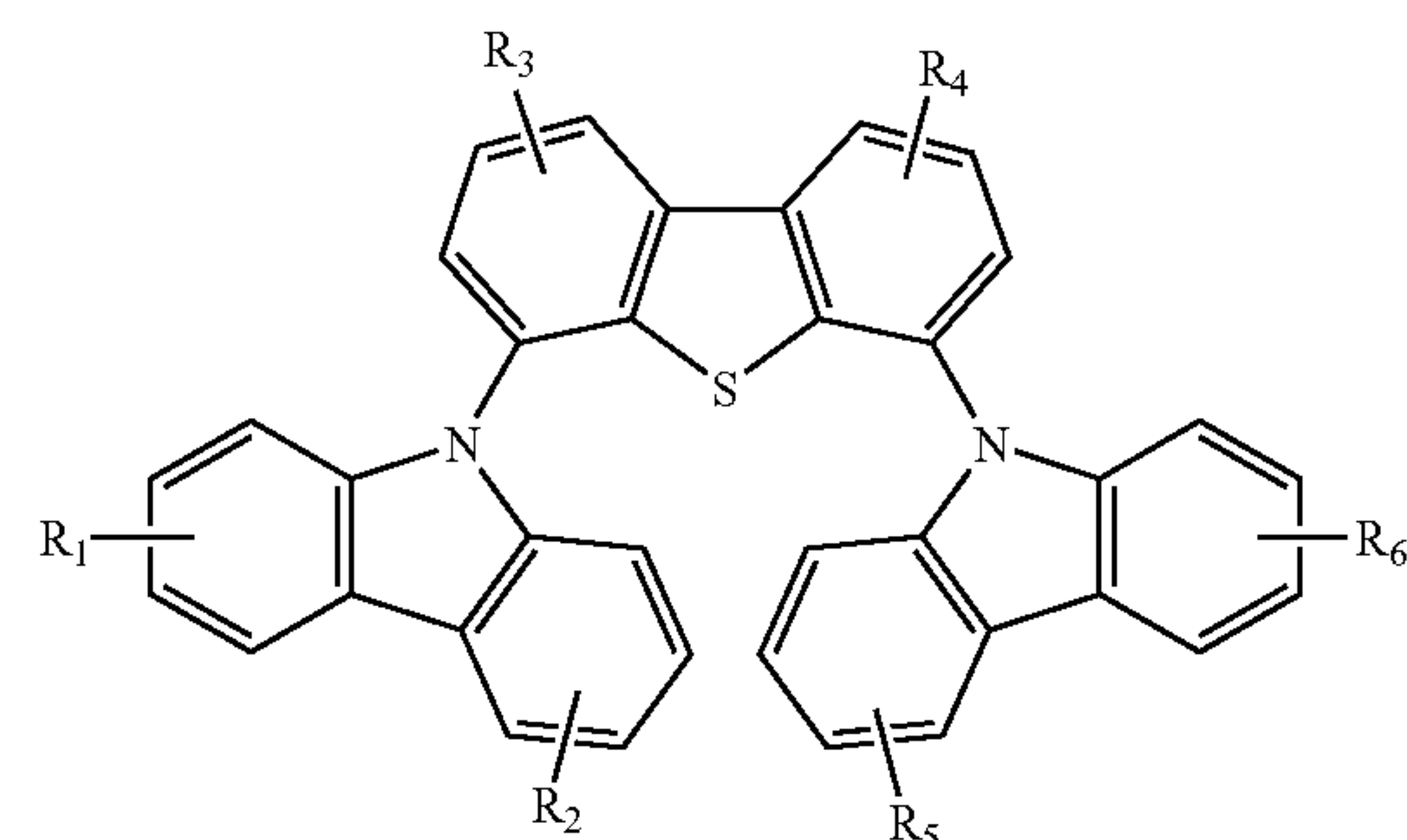
Compound 4G
