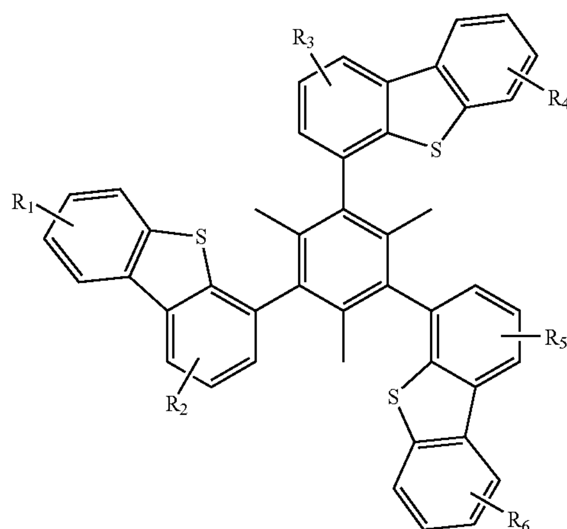
Compound 5G
