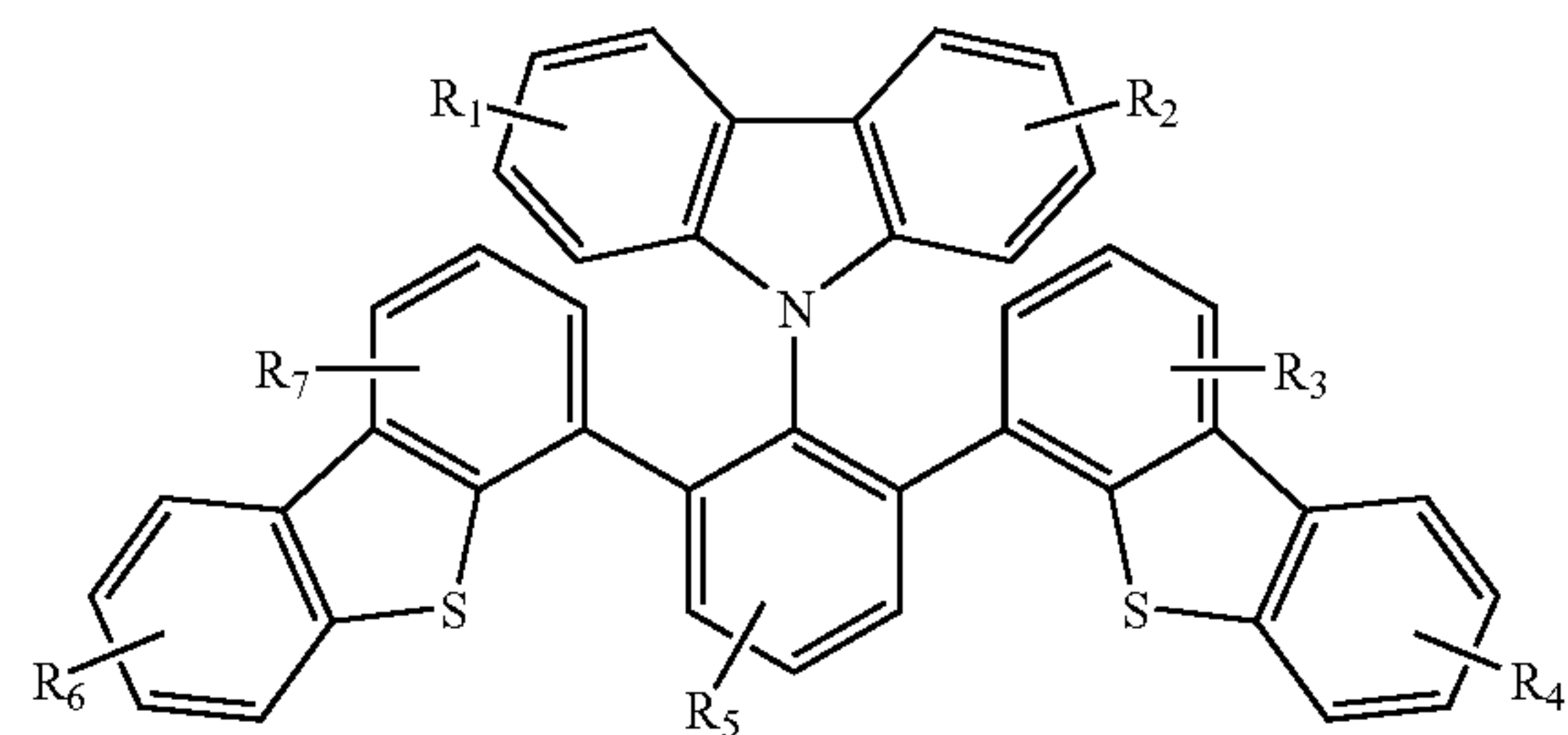
Compound 19G
