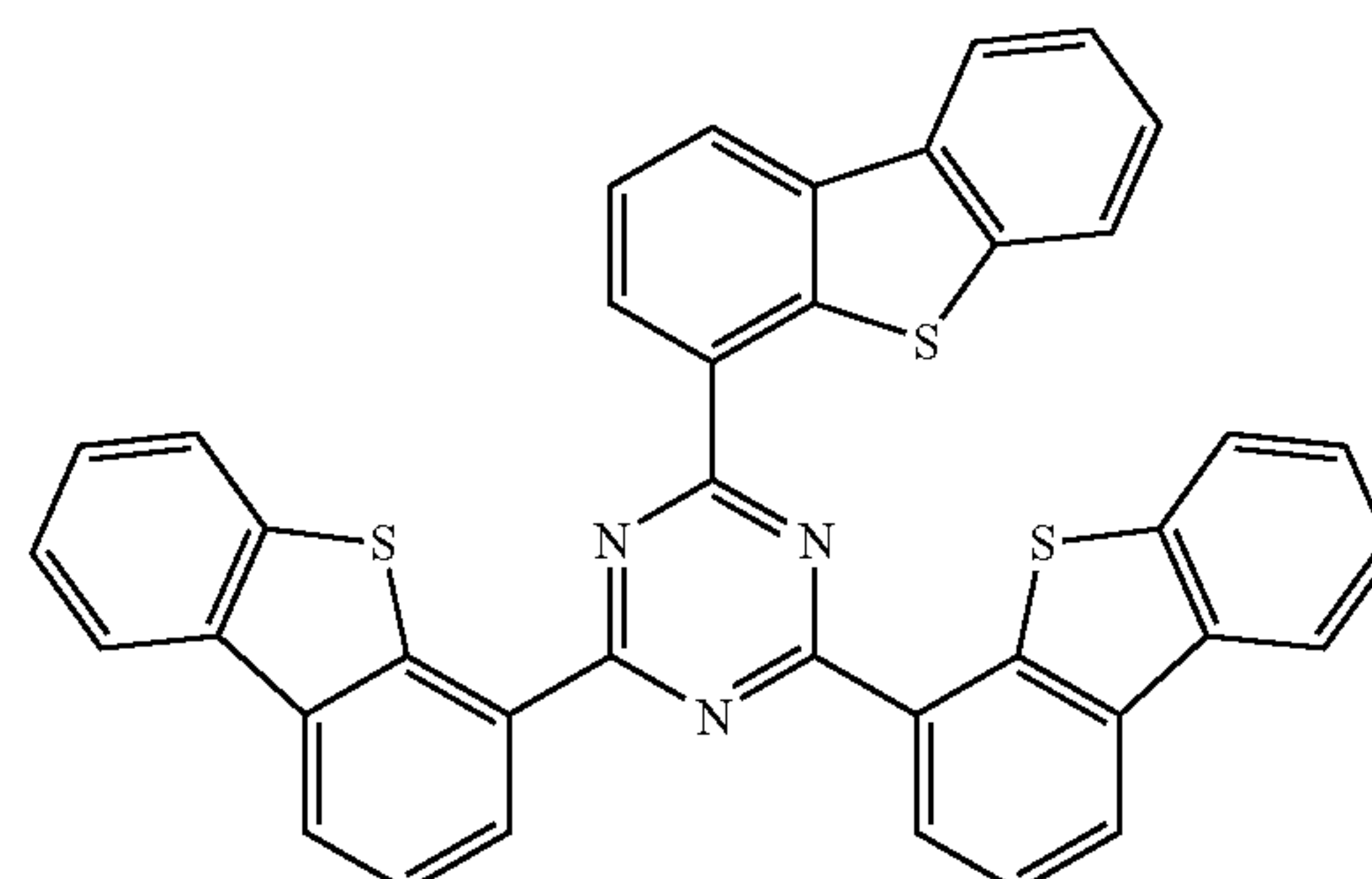
Compound 6
