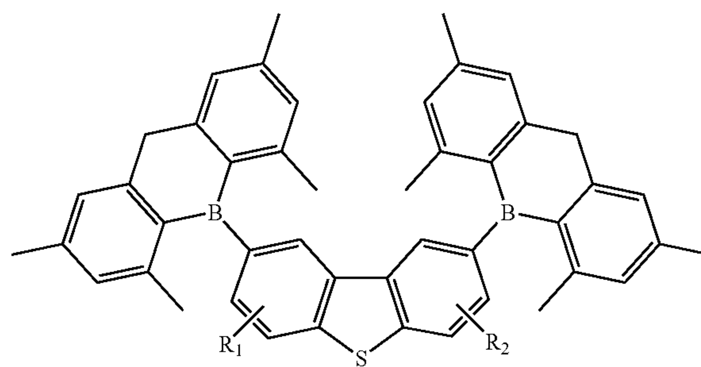
Compound 8G
