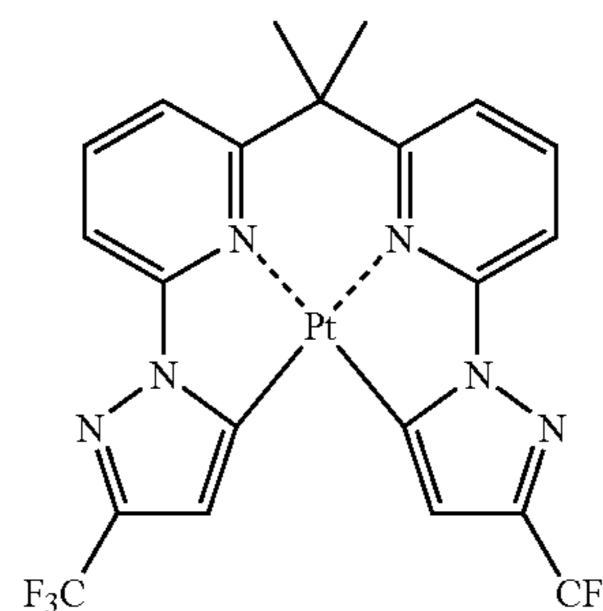
Compound 2 described in JP-A-2007-19462
