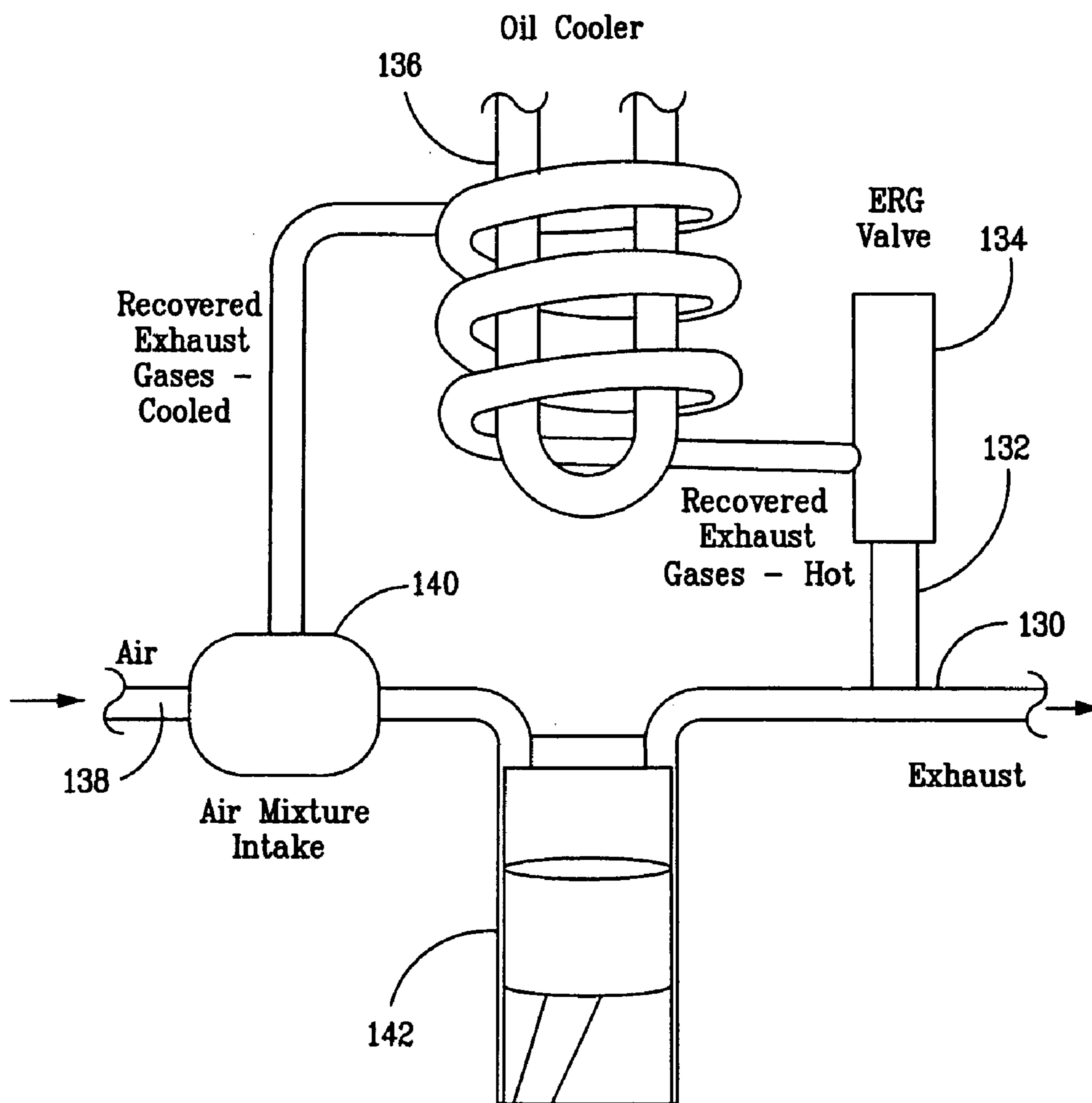
Prior Art FIG. 22
