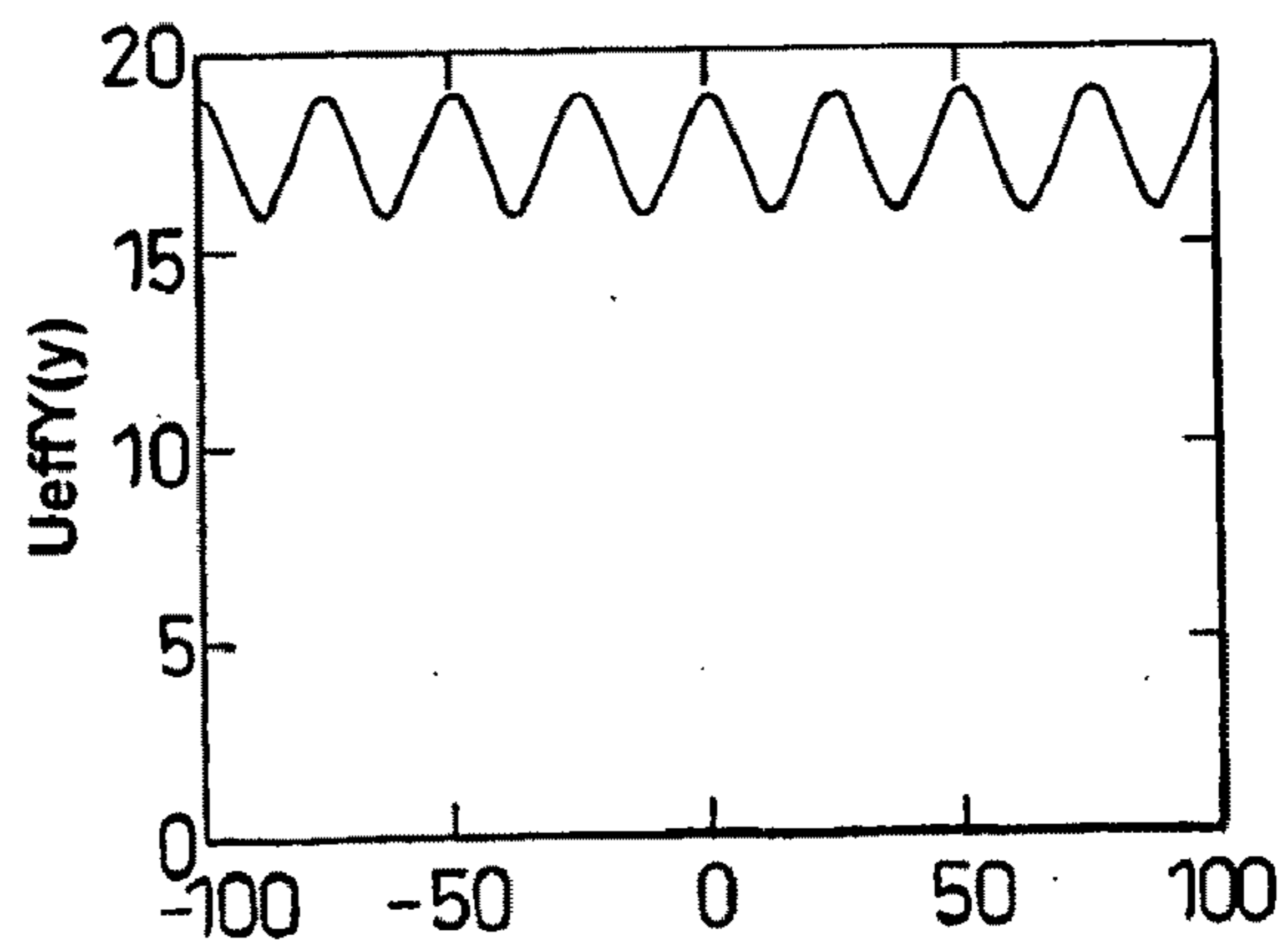
M = 200 at rf plates 3V ripple
