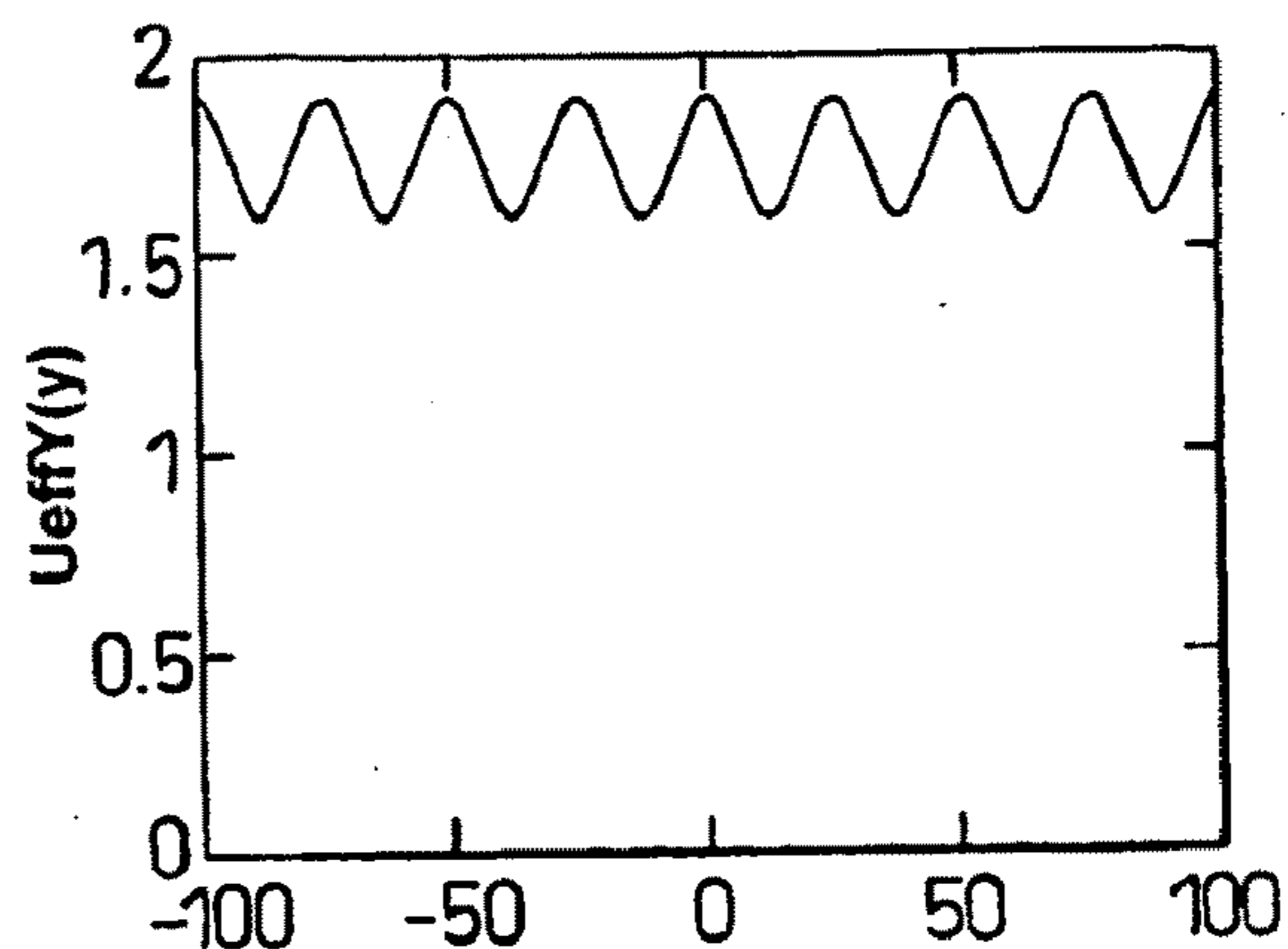
M = 2000 at rf plates 0.3V ripple
