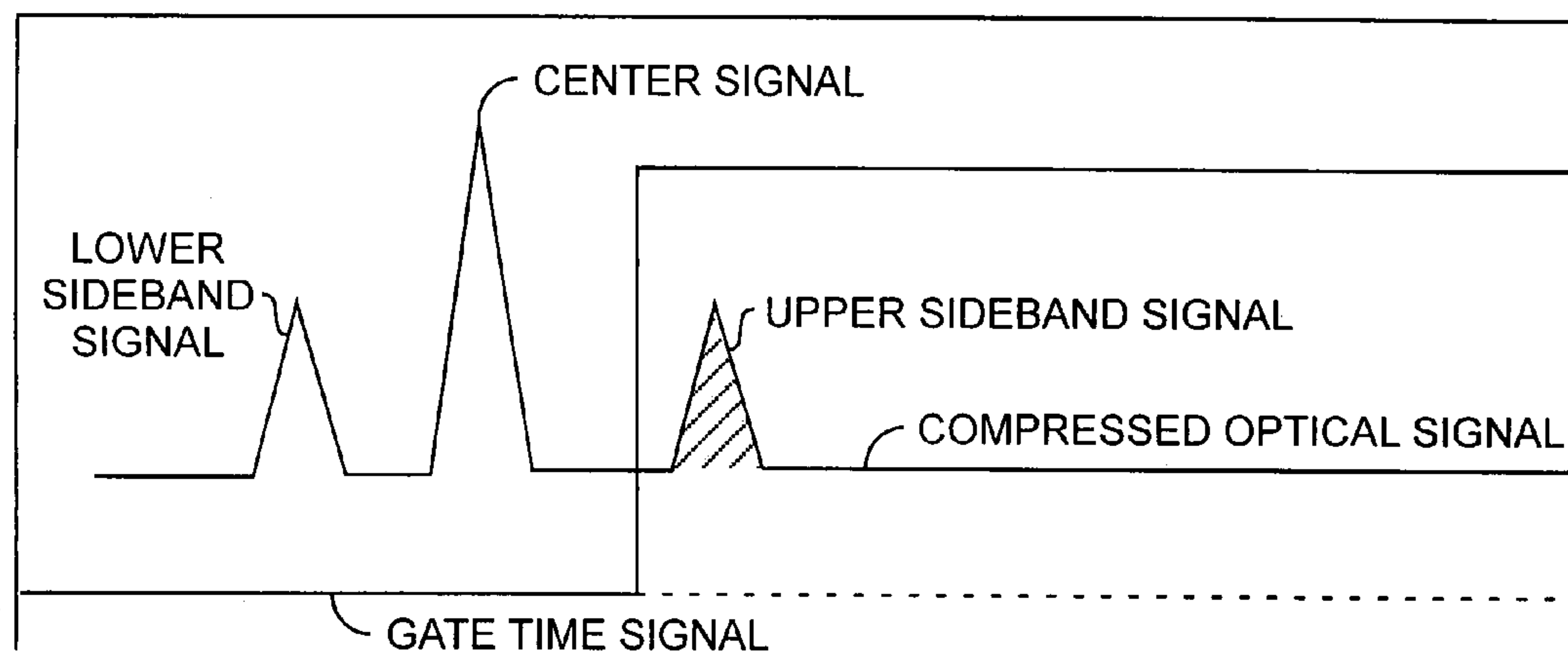
GATE TIMING
