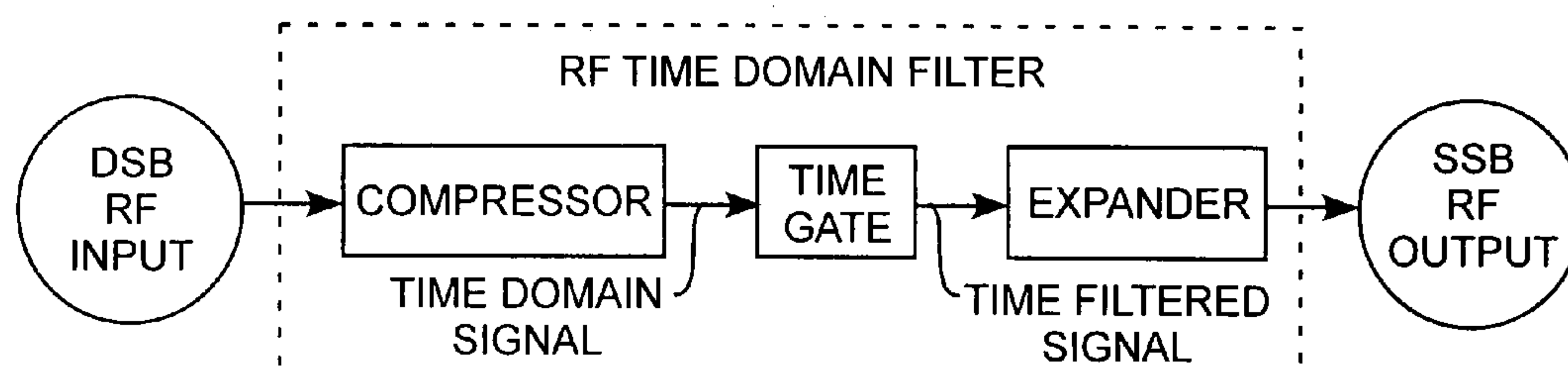
RF TIME DOMAIN FILTER
