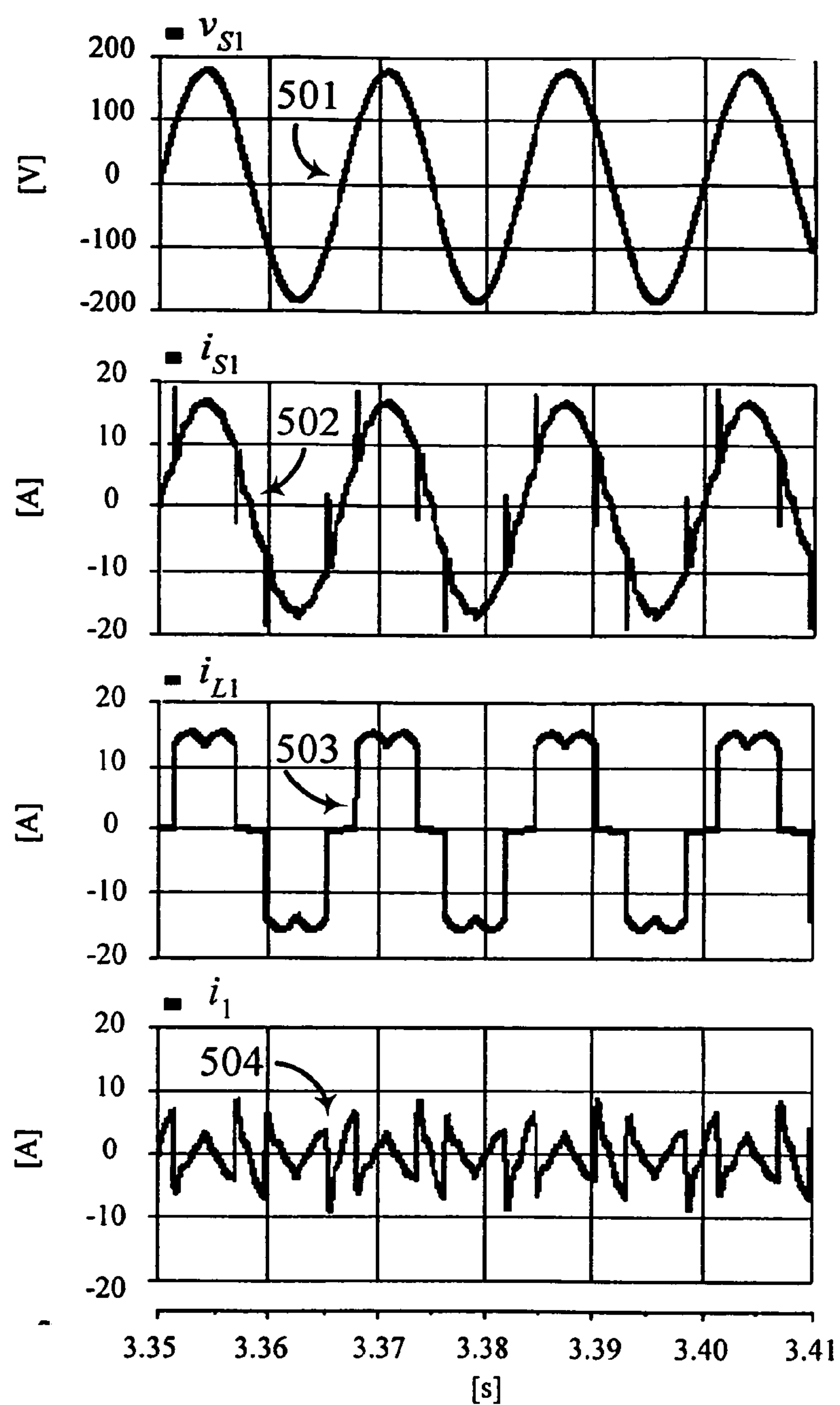
Fig. 5. Steady state responses of the proposed solution: (from top to bottom) line voltage v_{s1} , line current i_{s1} , load current i_{01} and injected current i_1 .
