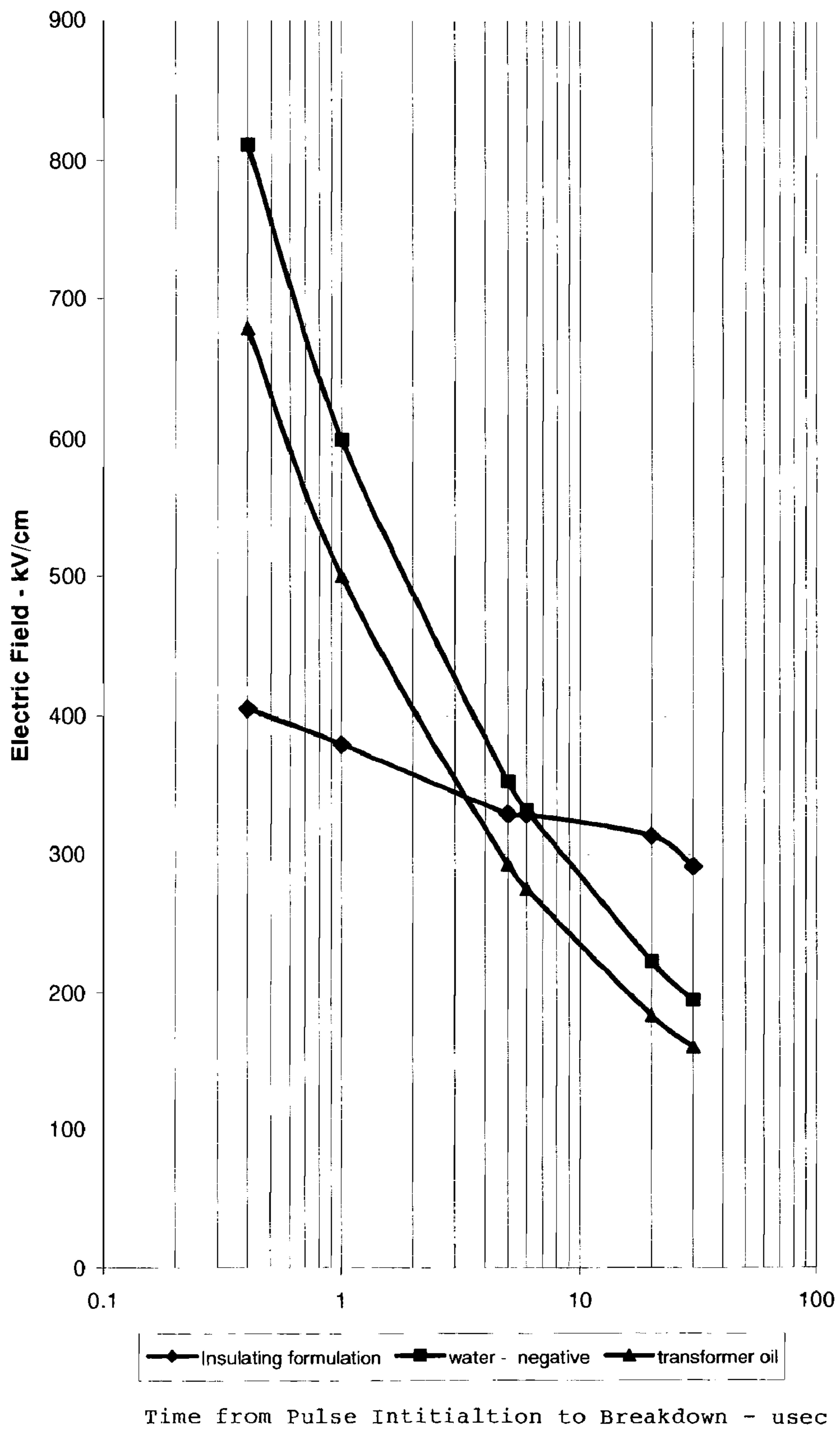
Dielectric Strength vs. Delay To Breakdown Figure 32
