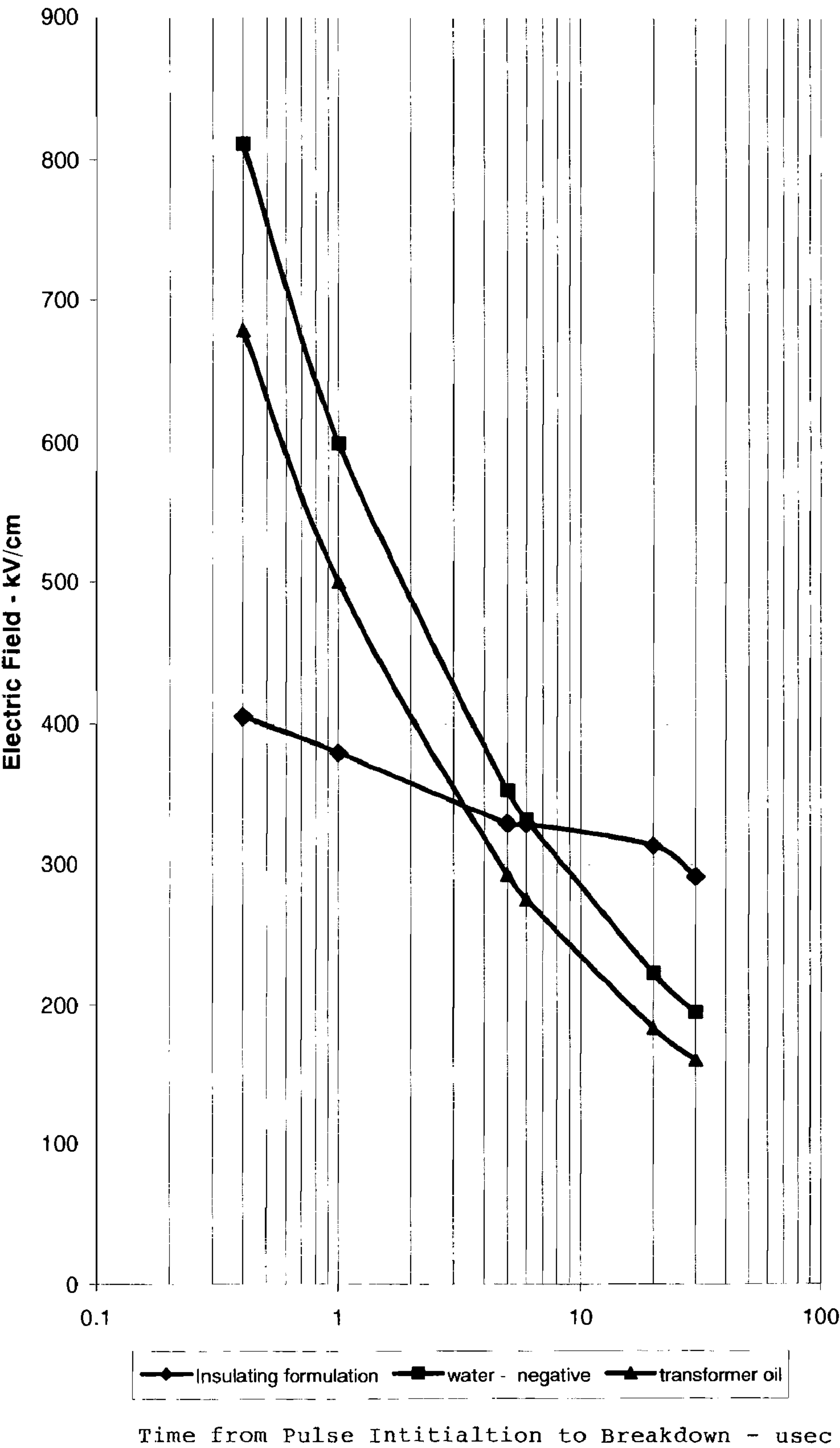
Dielectric Strength vs. Delay To Breakdown Figure 32
