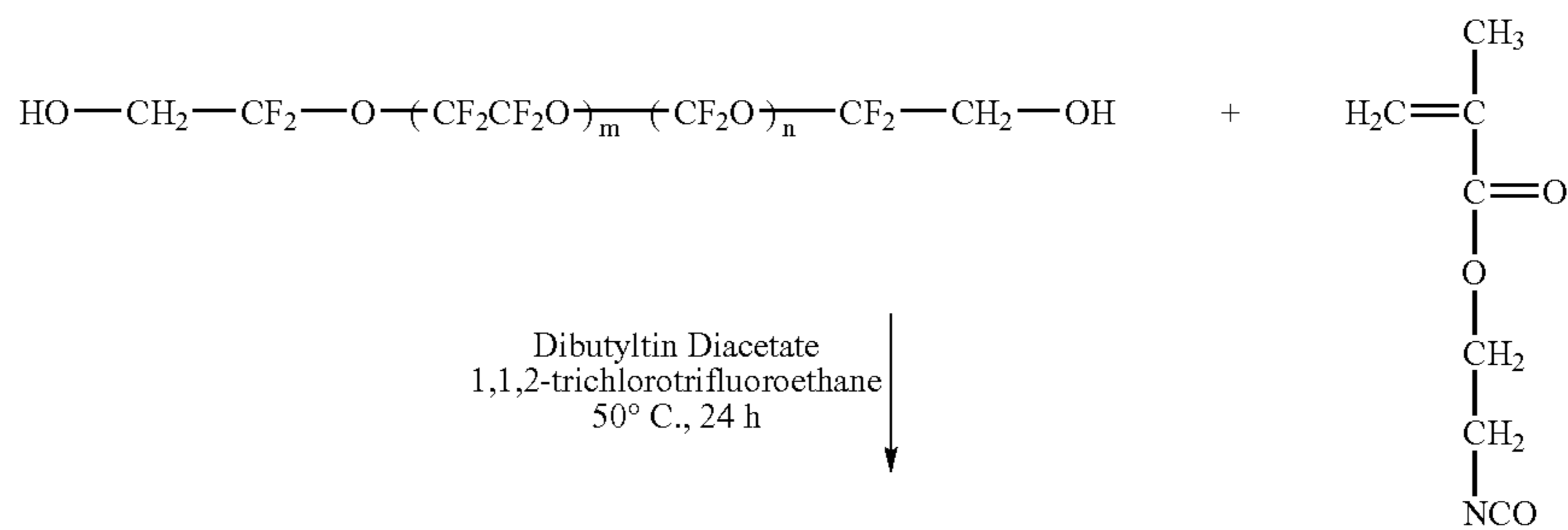
Scheme 1. Synthesis and Photocuring of Functional Perfluoropolyethers.
