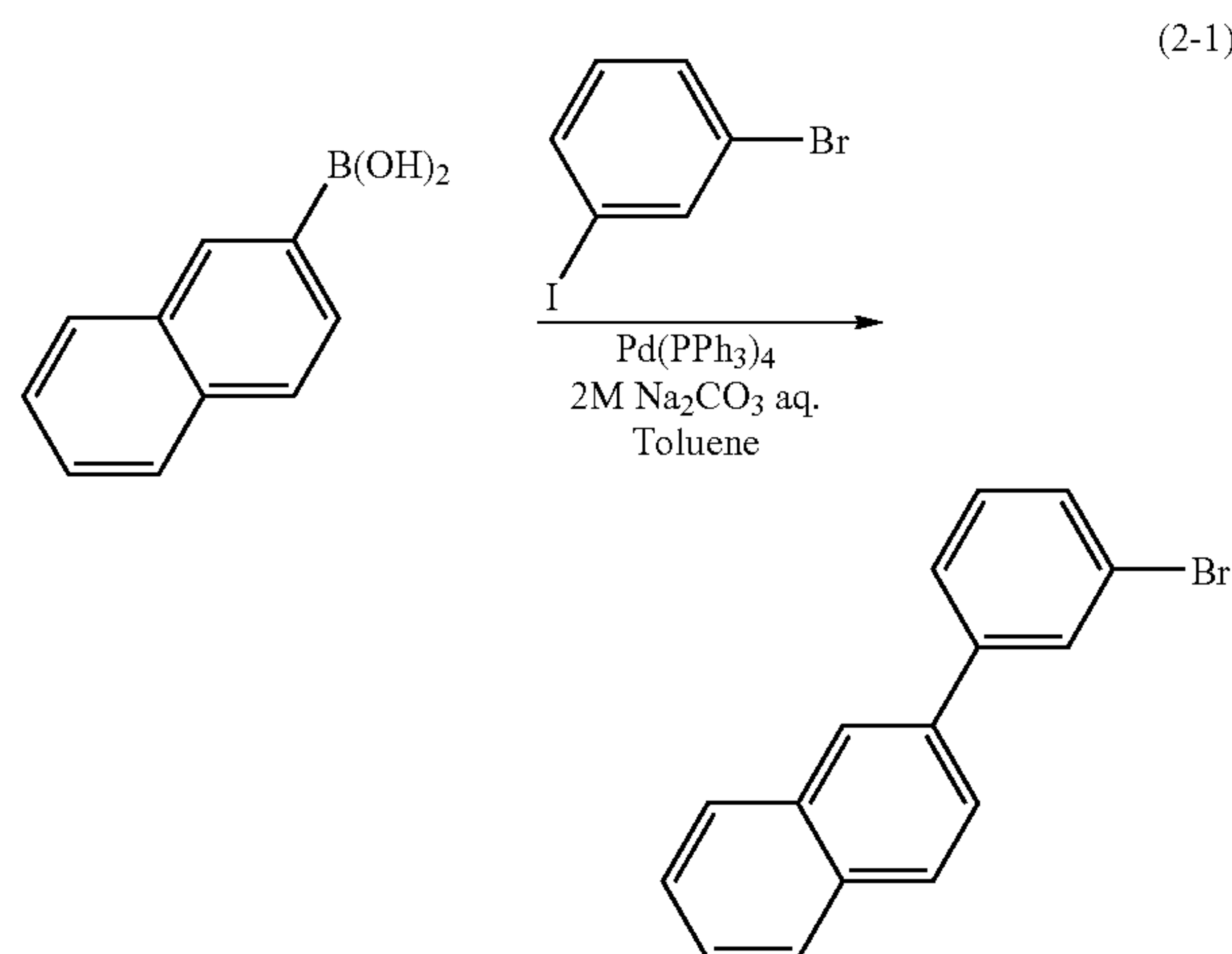
Synthesis of 2-(3-bromophenyl) naphthalene
