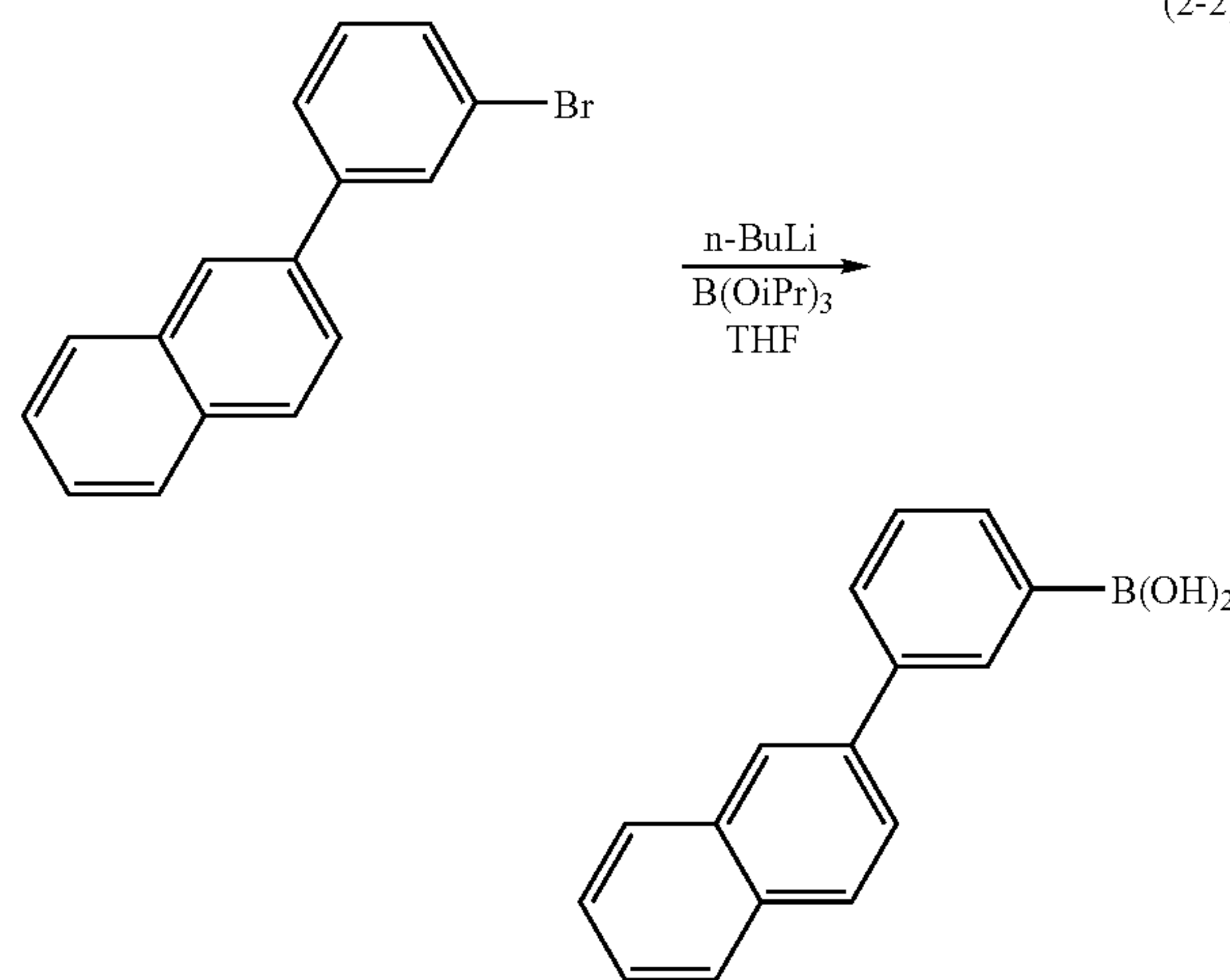
Synthesis of 3-(2-naphthyl) phenylboronic acid
