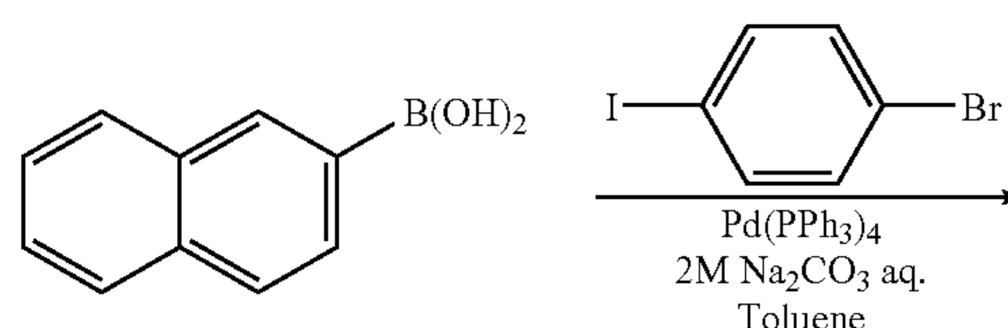
Synthesis of 2-(4-bromophenyl) naphthalene
