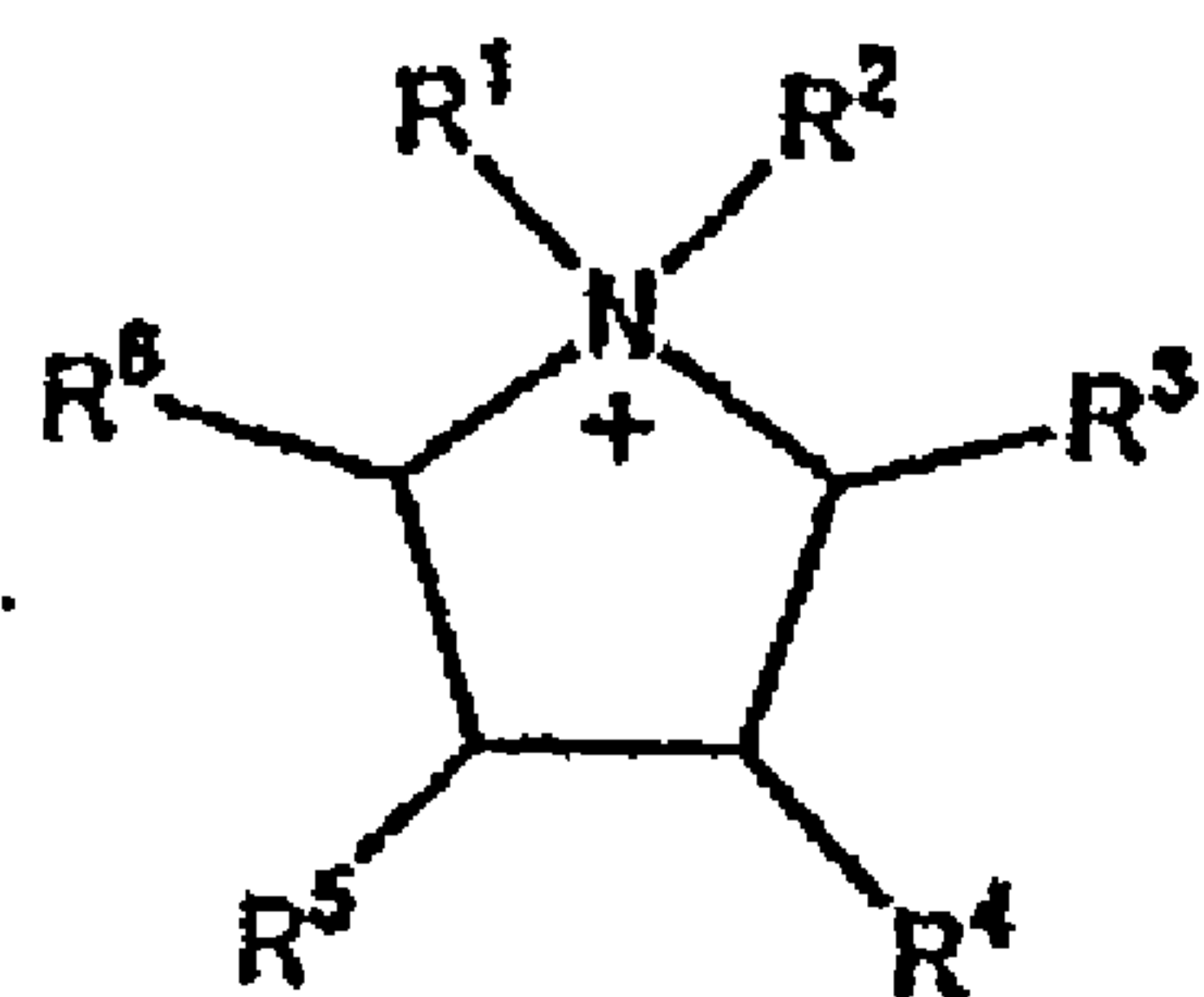
pyrrolidinium
