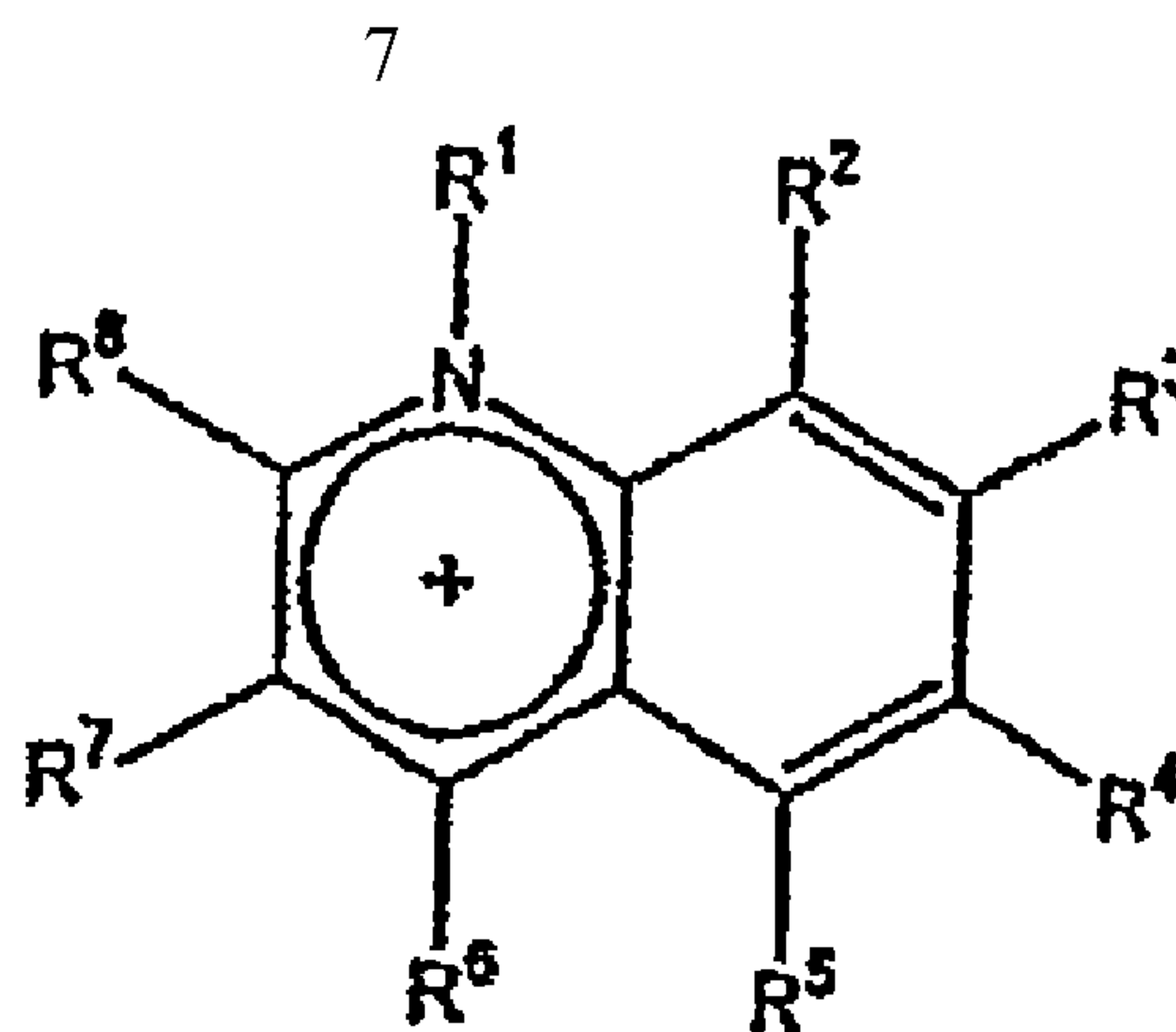
quinolinium
