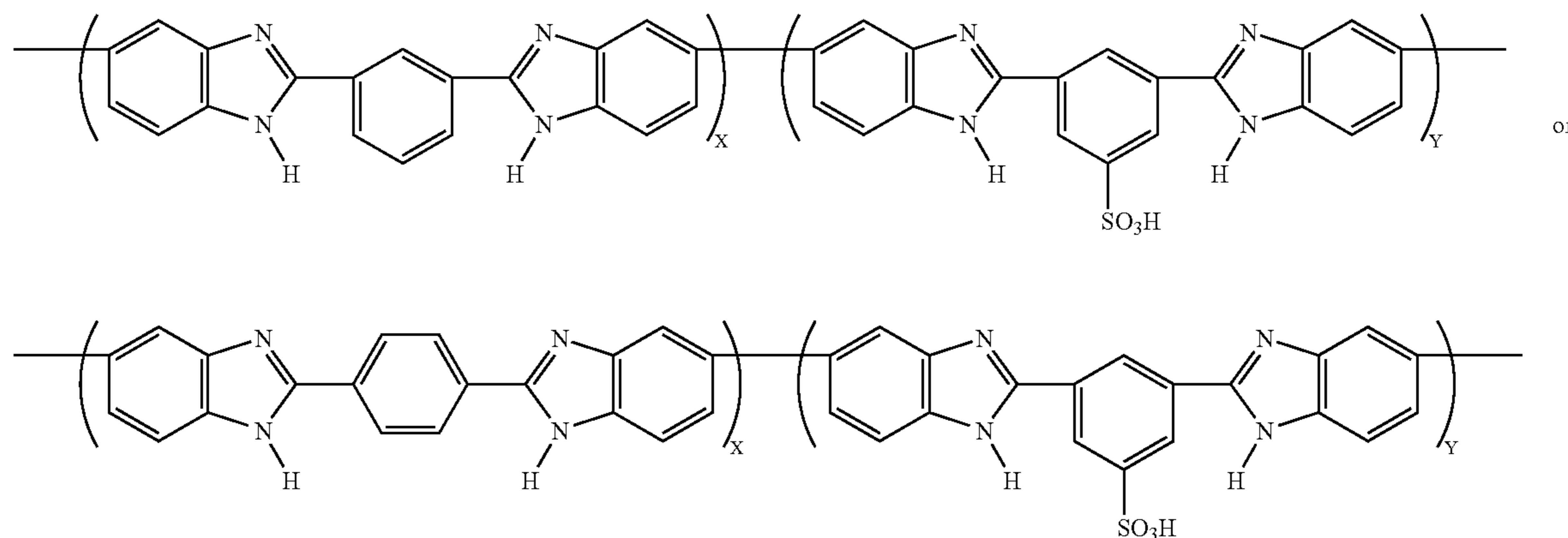
[Chemical Formula 1]
