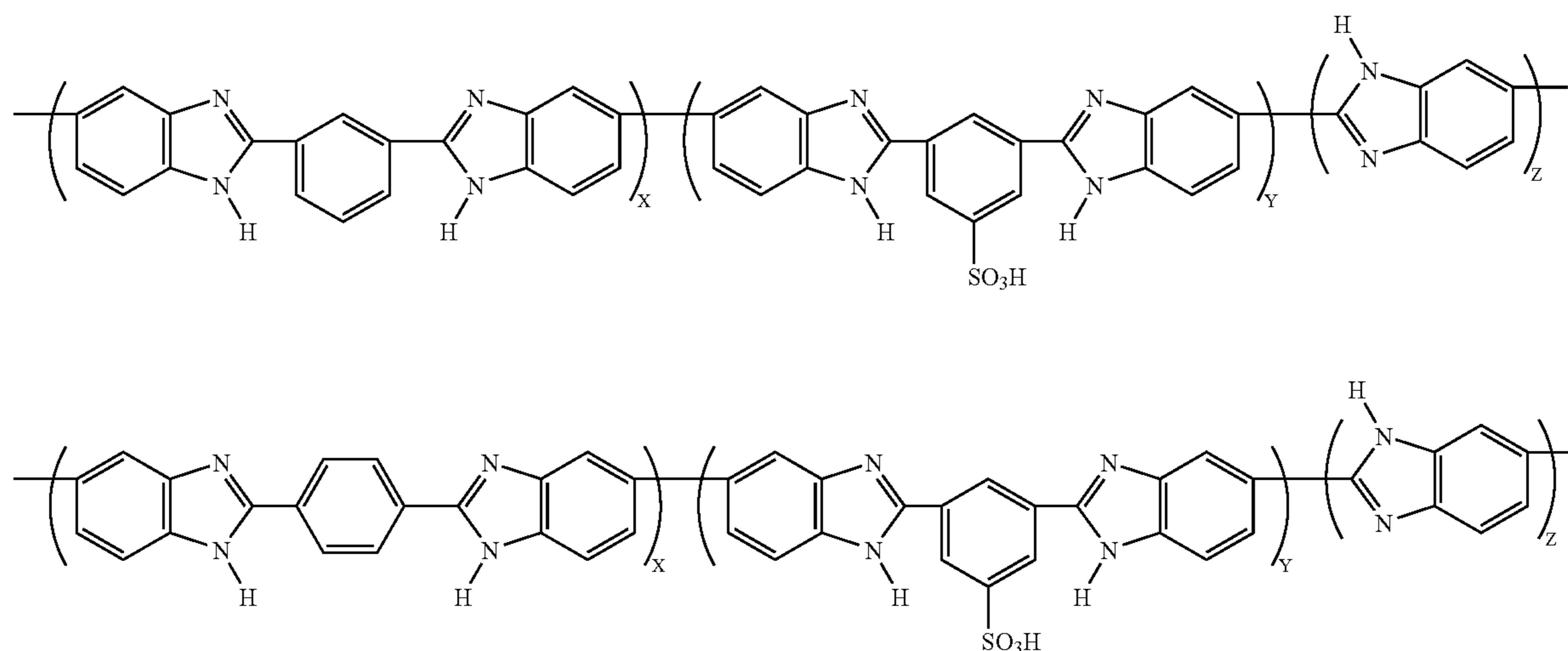
[Chemical Formula 2]
