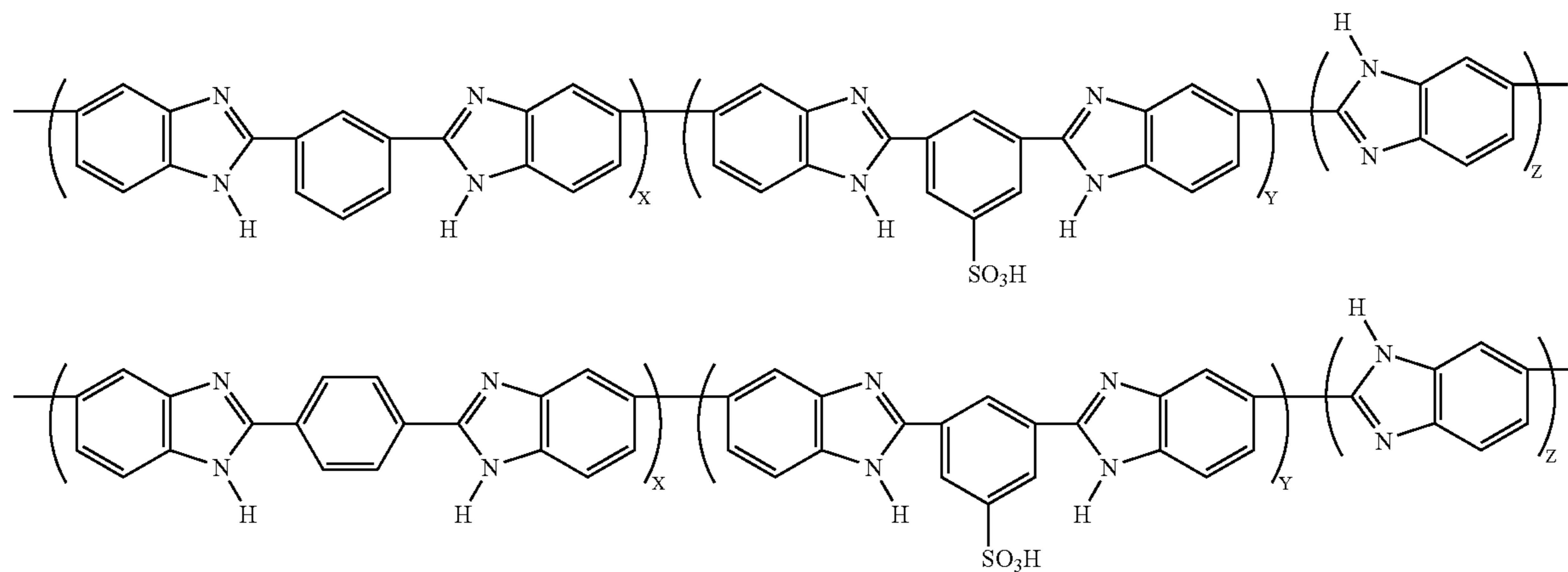
[Chemical Formula 2]
