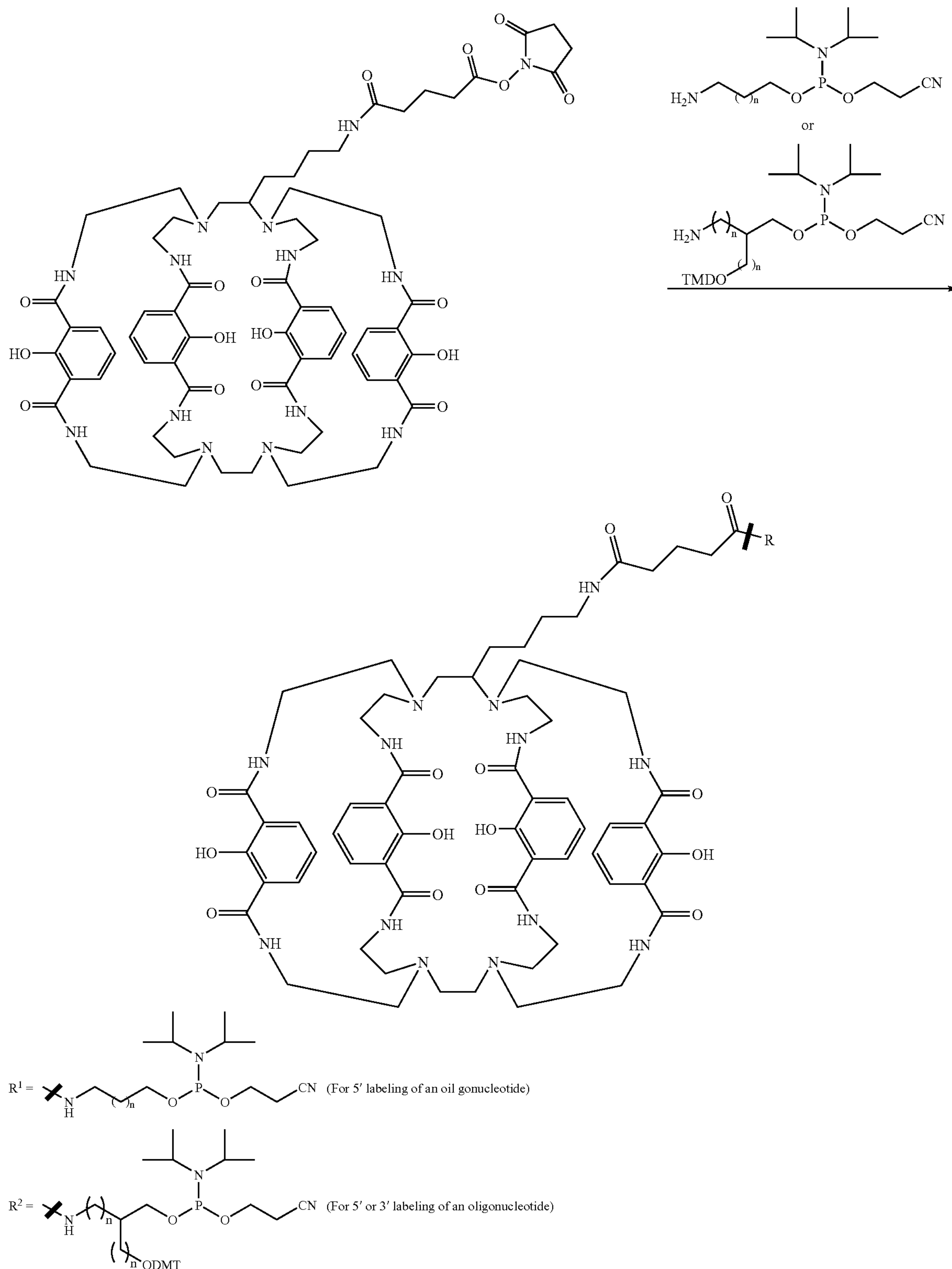
Scheme 20
