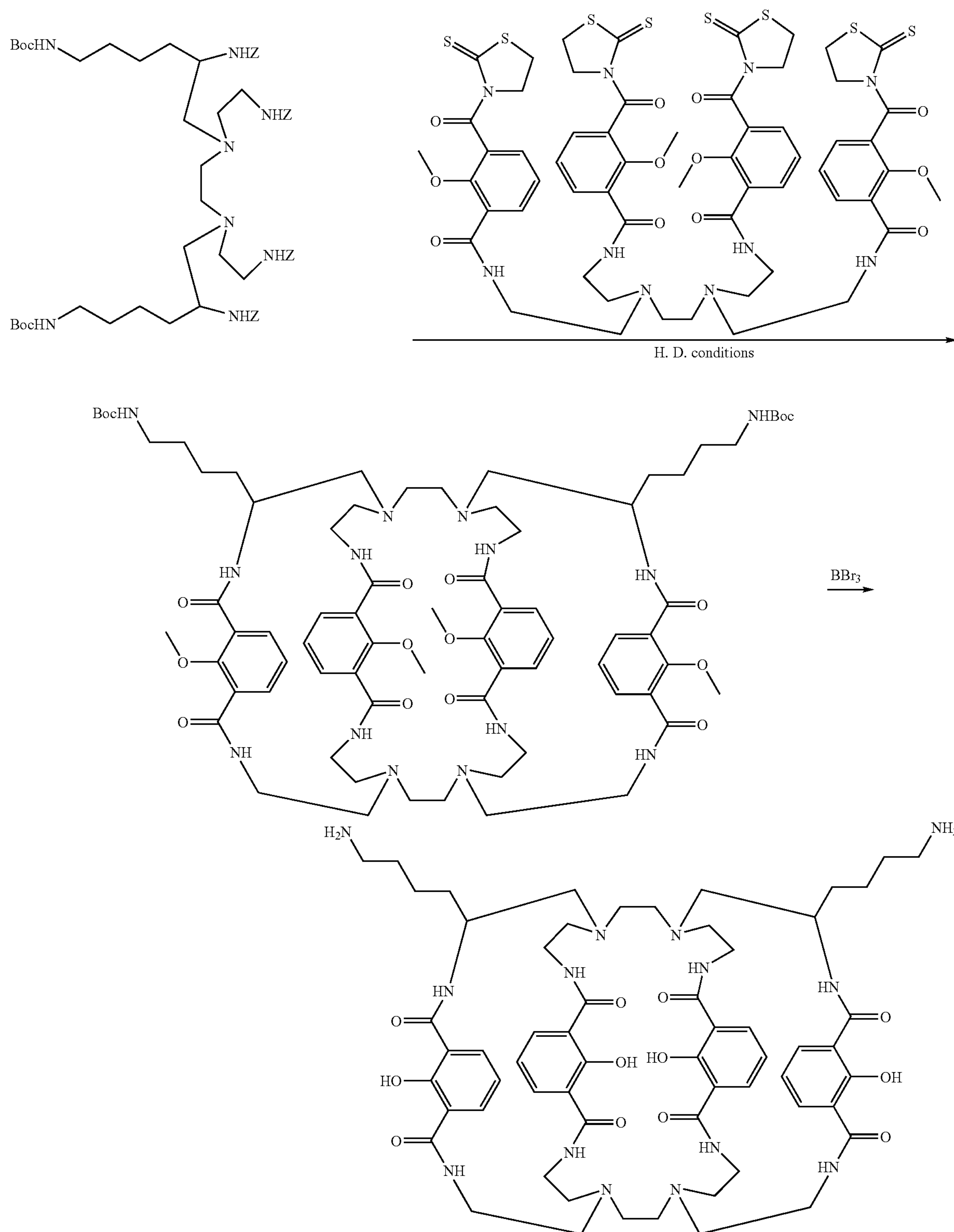
Scheme 15
