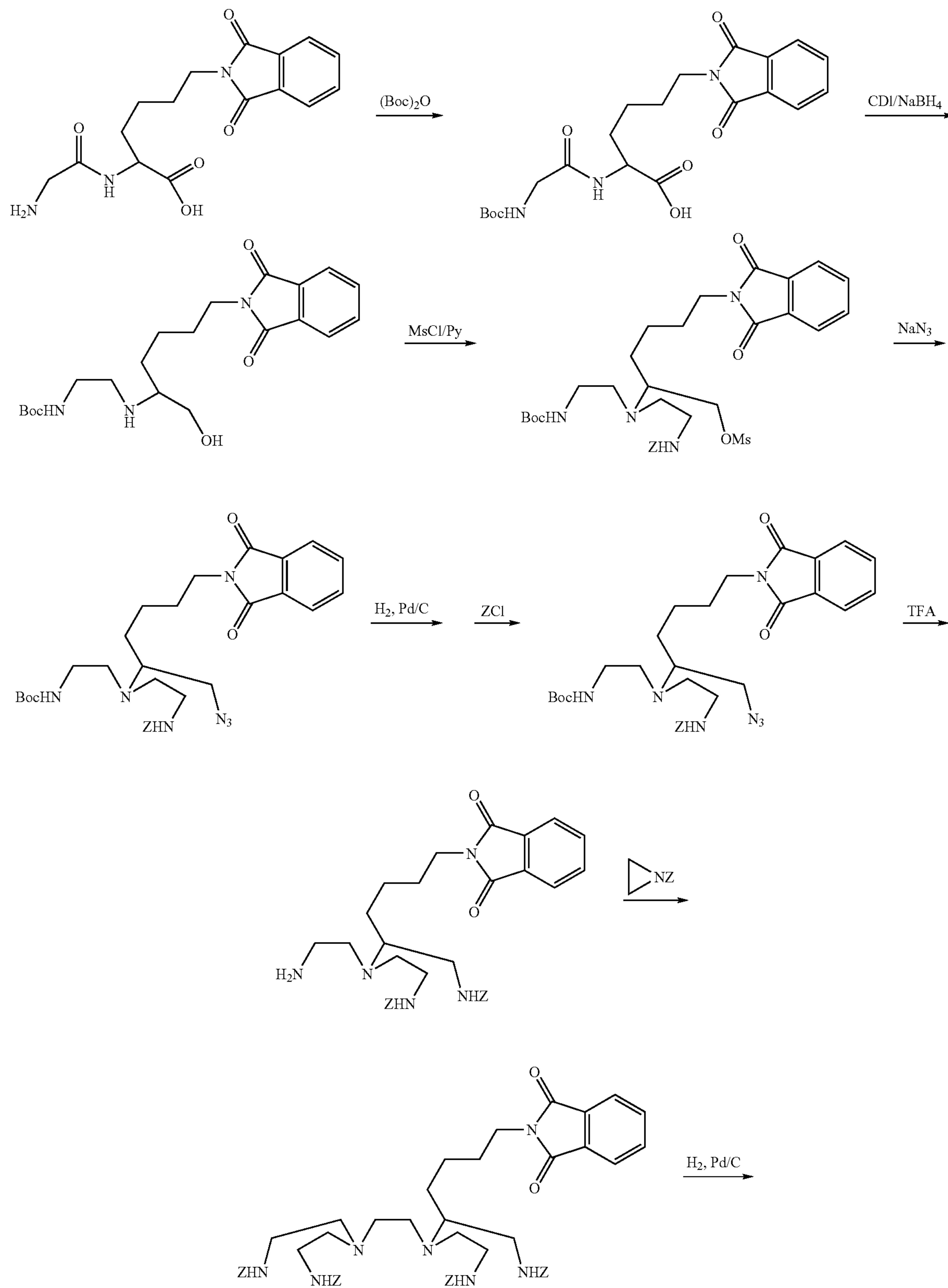
Scheme 3
