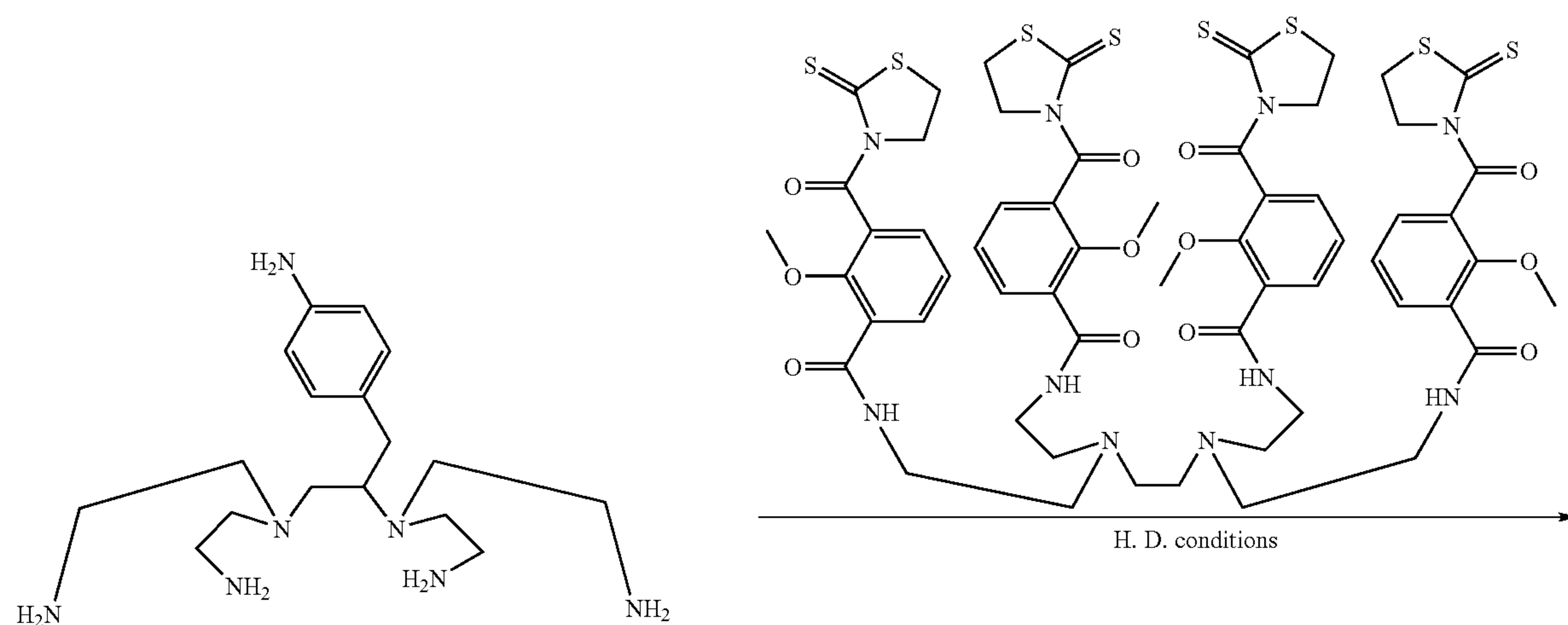
Scheme 14
