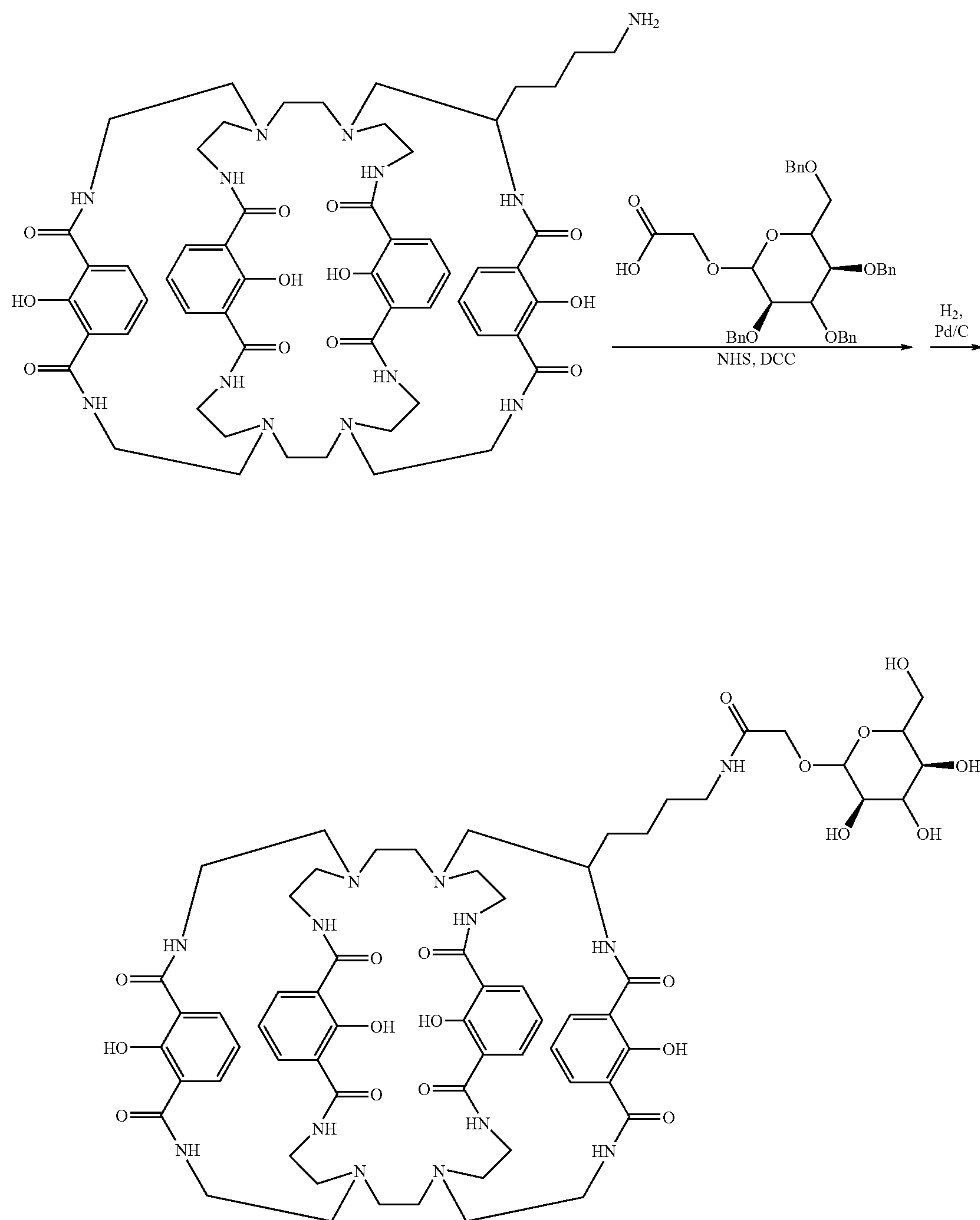
Scheme 21
