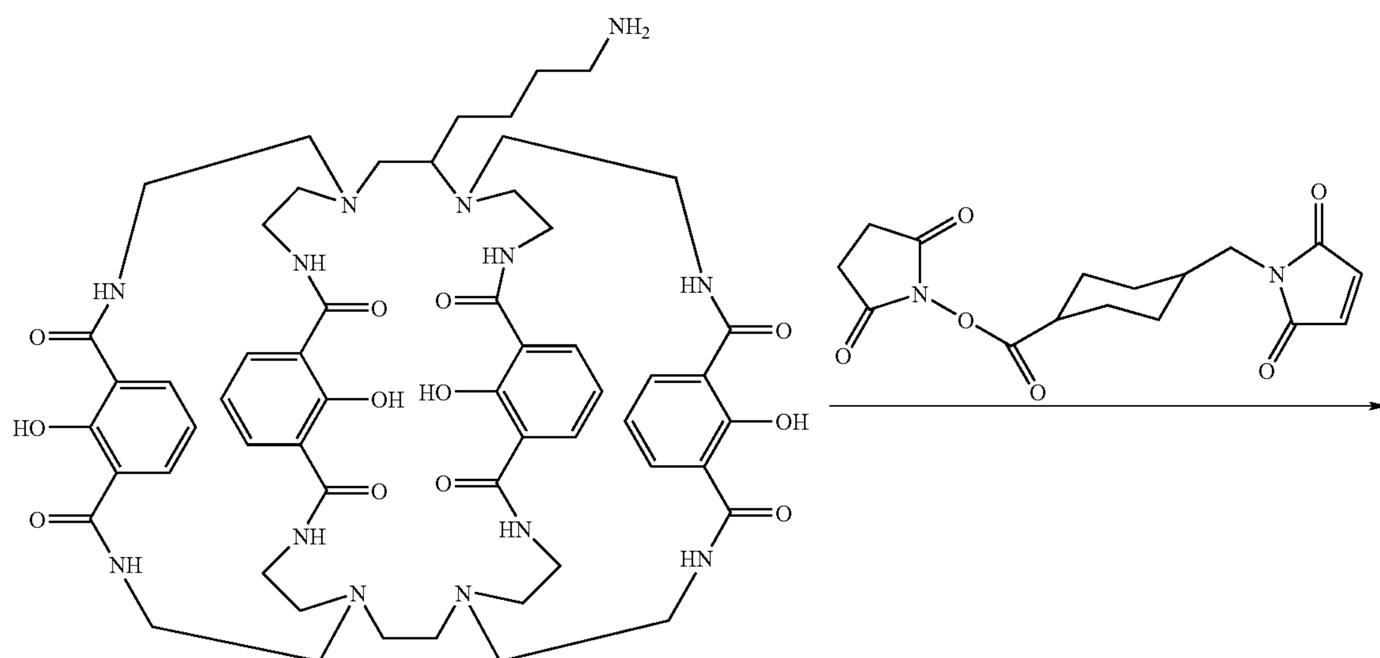
Scheme 18
