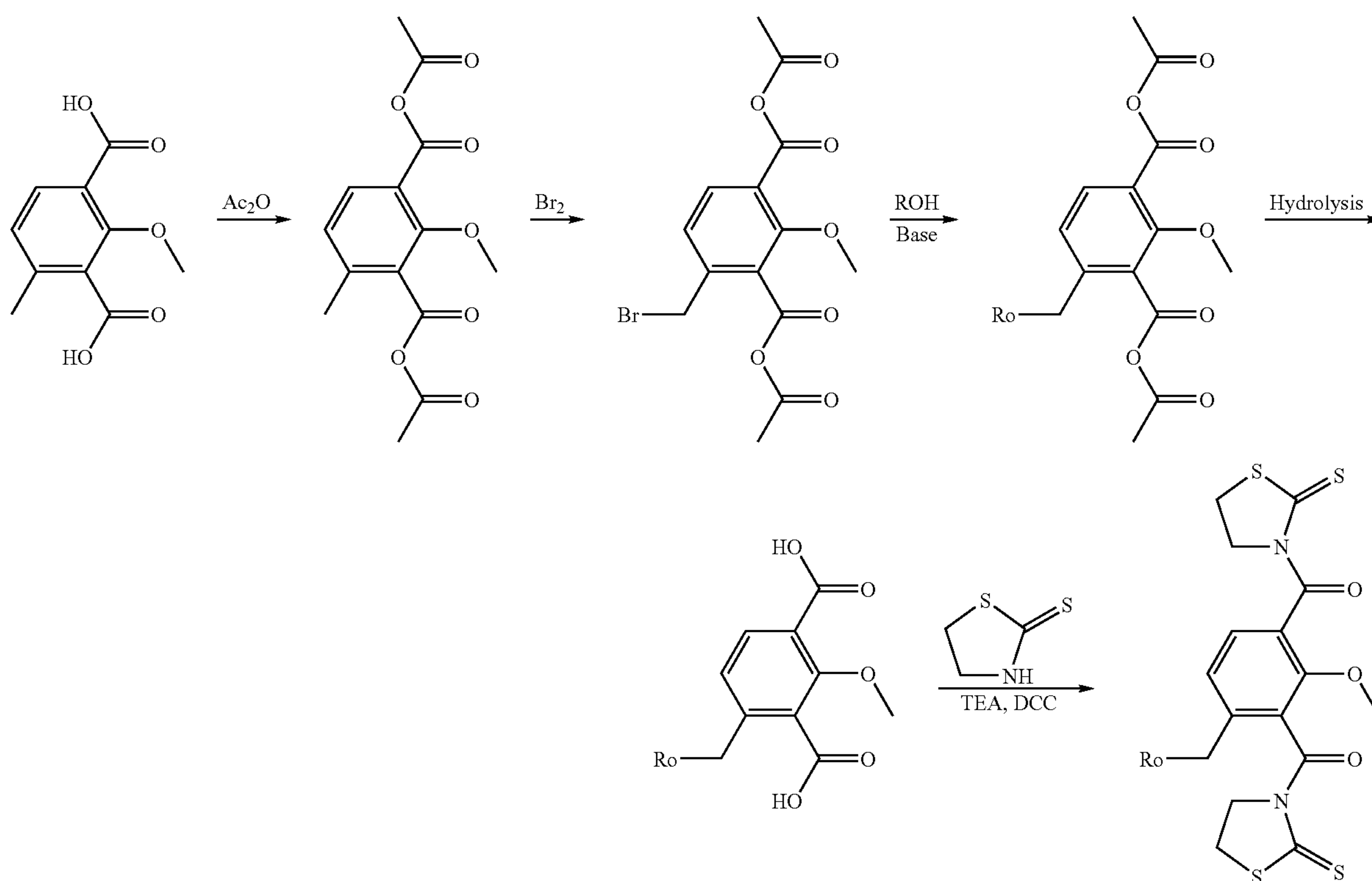
Scheme 11
