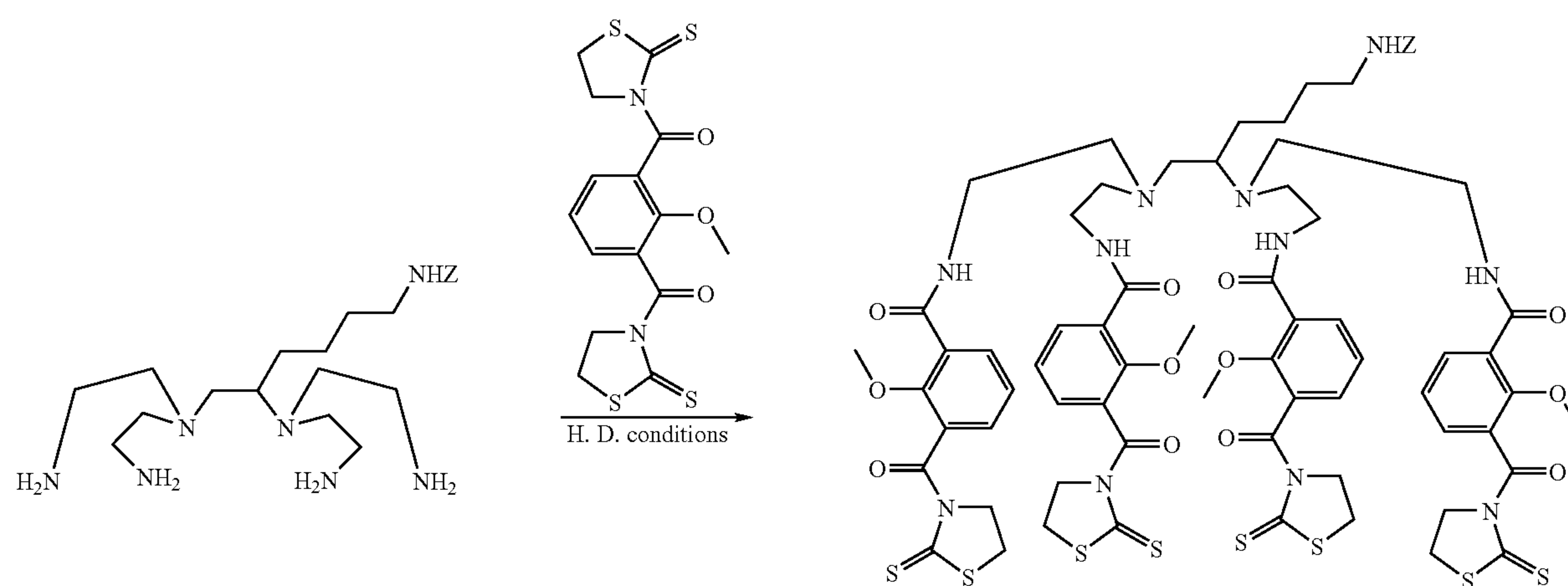
Scheme 12
