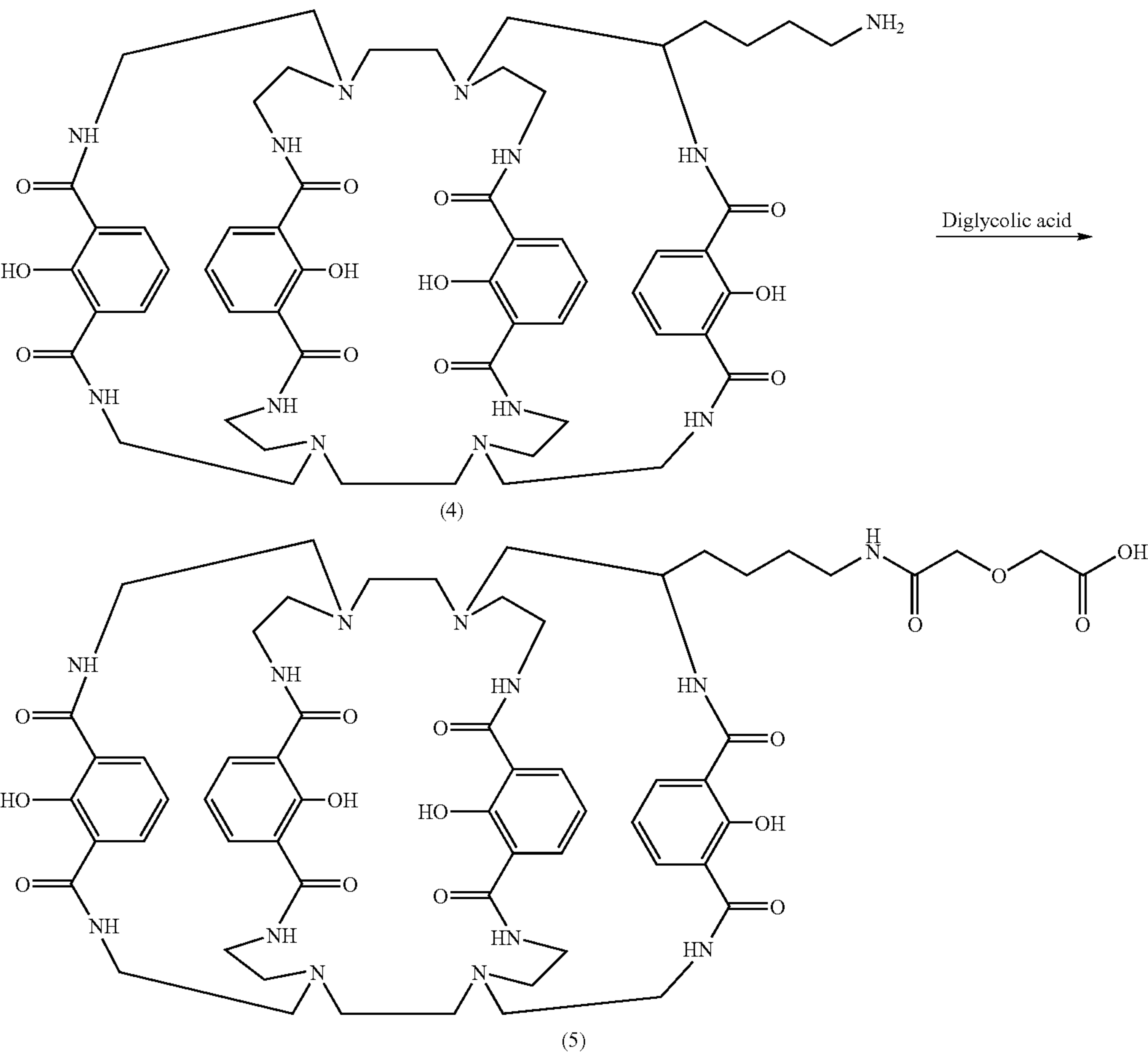
Example 5 Synthesis of Donor-Acceptor Conjugate (4a) [0261]
