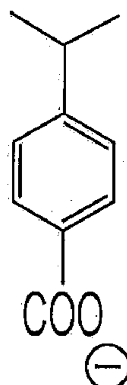
4-isopropyl-benzoate IPB
