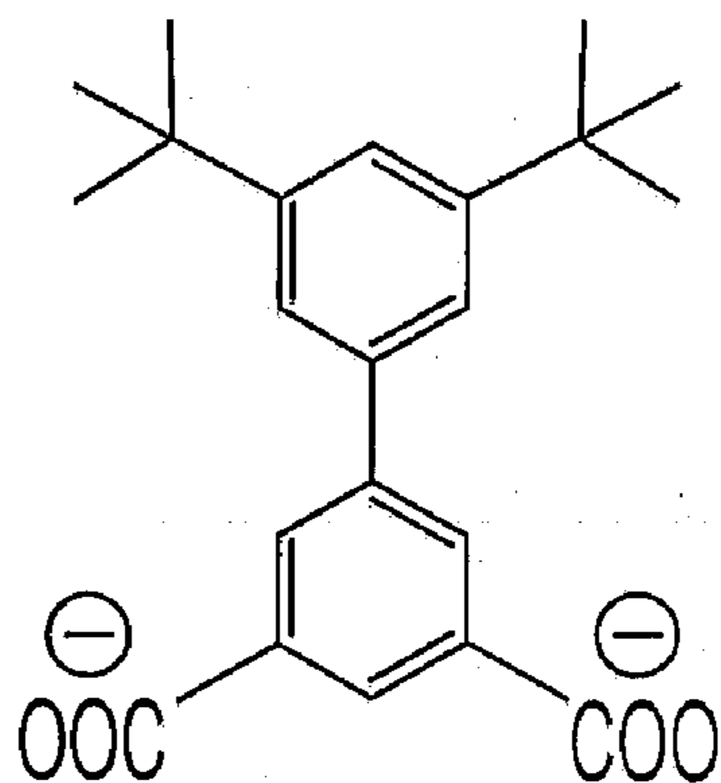
3',5'-di-tert-butyl-biphenyl-3,5-dicarboxylate DBBPDC
