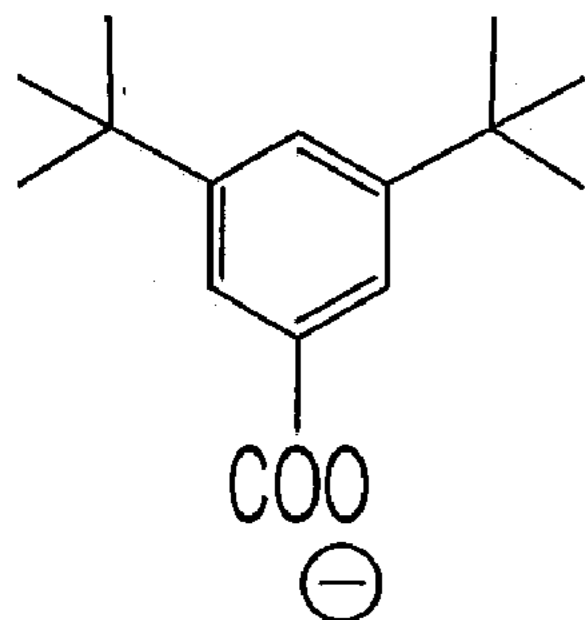
3,5-di-tert-butyl-benzoate DBB
