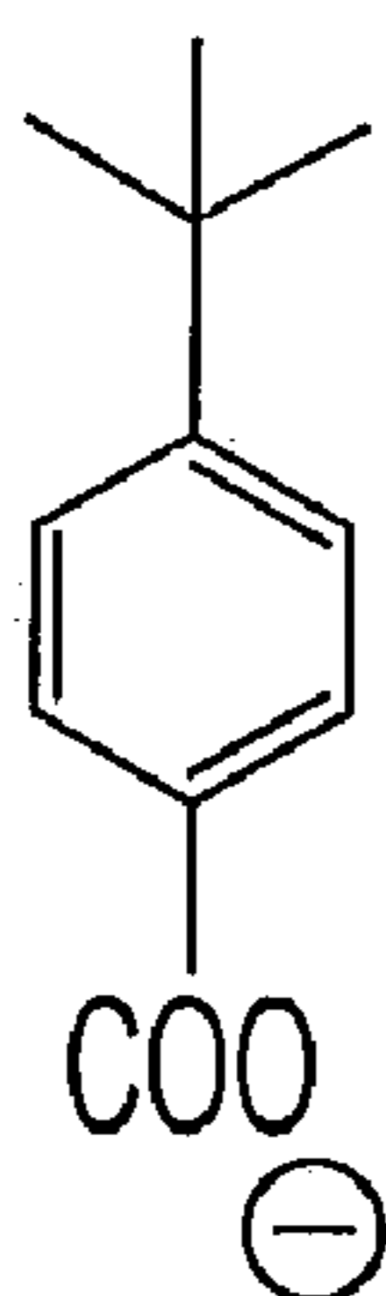
4-tert-butyl-benzoate TBB
