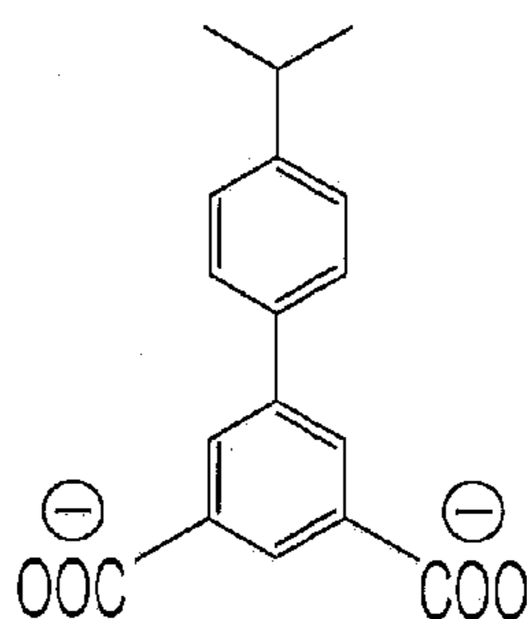
4'-isopropyl-biphenyl-3,5-dicarboxylate PBPDC
