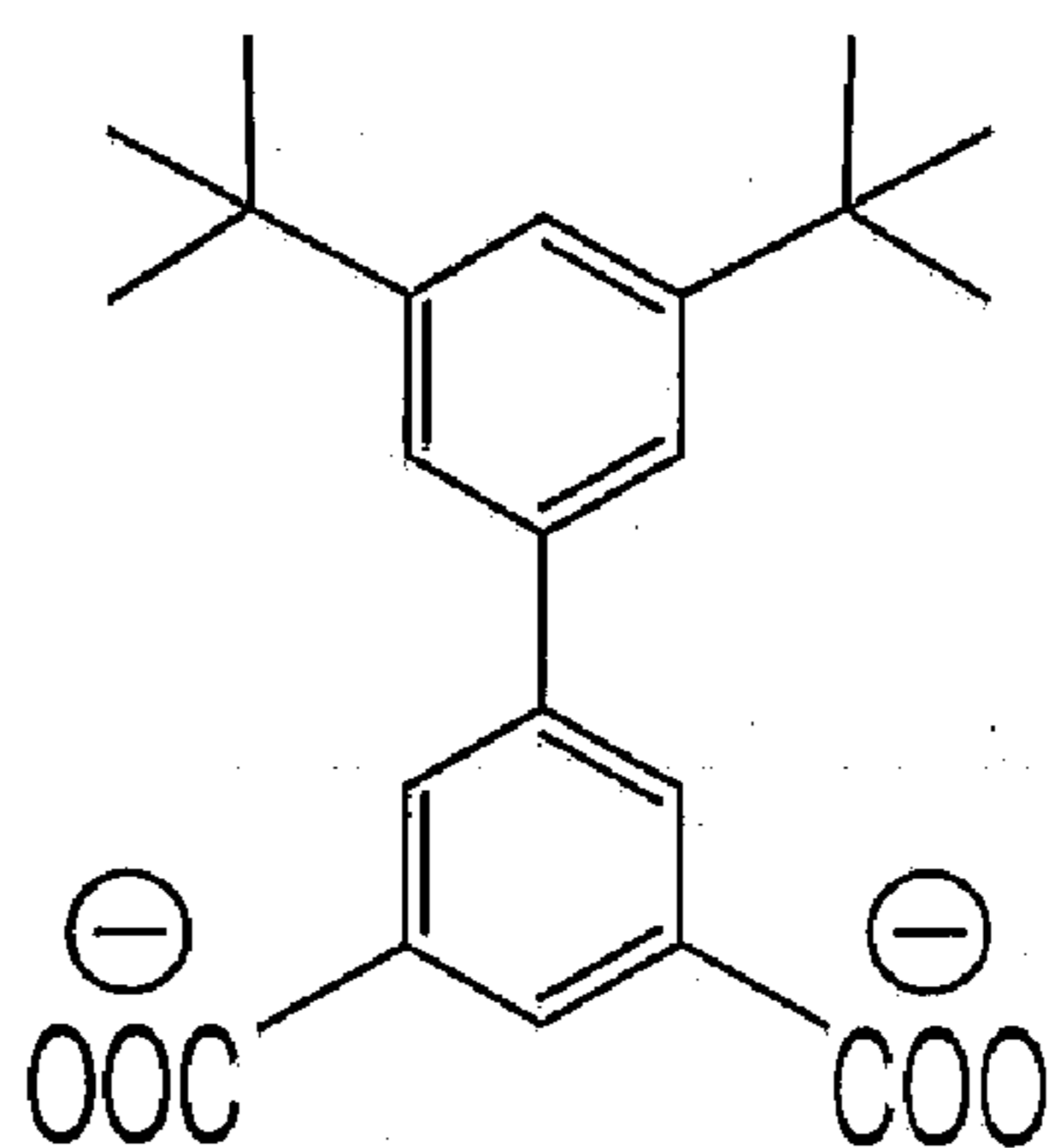
3',5'-di-tert-butyl-biphenyl-3,5-dicarboxylate DBBPDC
