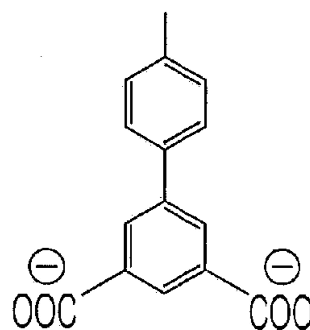
4'-methyl-biphenyl-3,5-dicarboxylate MBPDC
