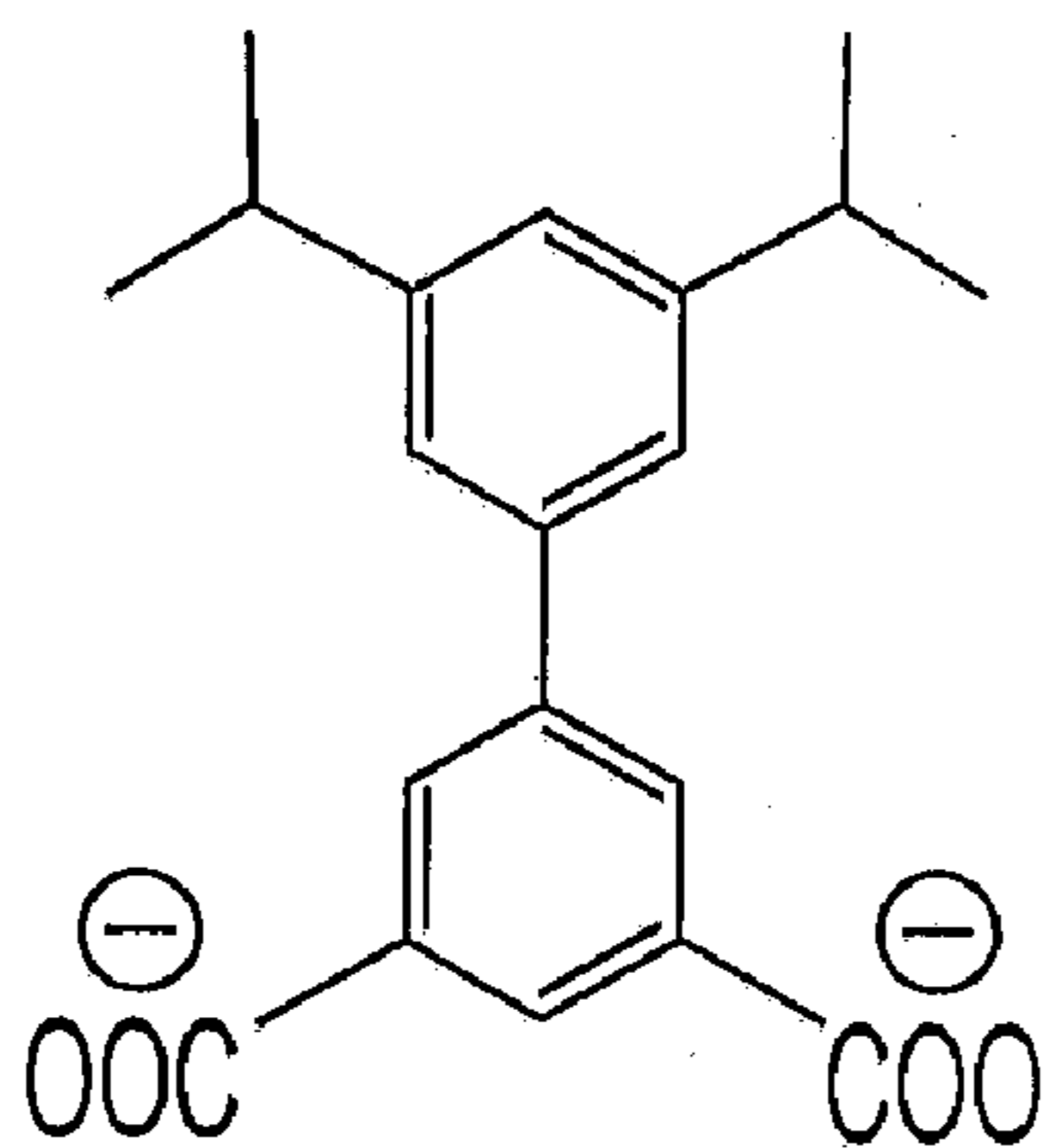
3',5'-diisopropyl-biphenyl-3,5-dicarboxylate DPBPDC
