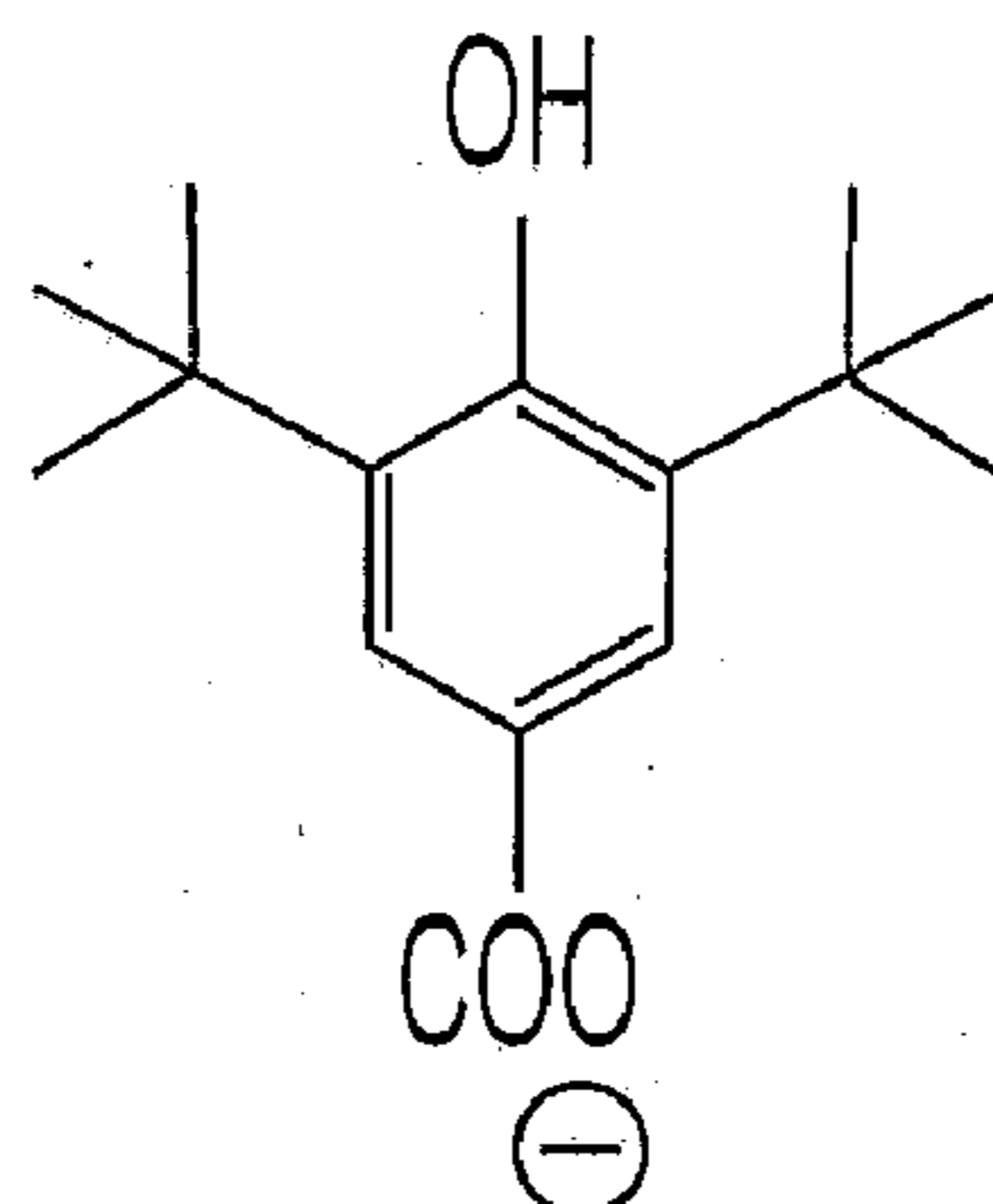
3,5-di-tert-butyl-4-hydroxy-benzoate DBHB
