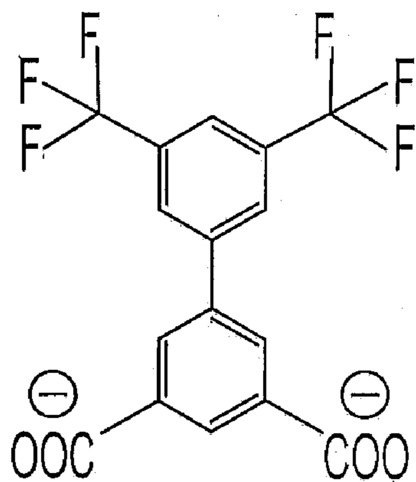
3',5'-bis-trifluoromethyl-biphenyl-3,5-dicarboxylate BTFMBPDC
