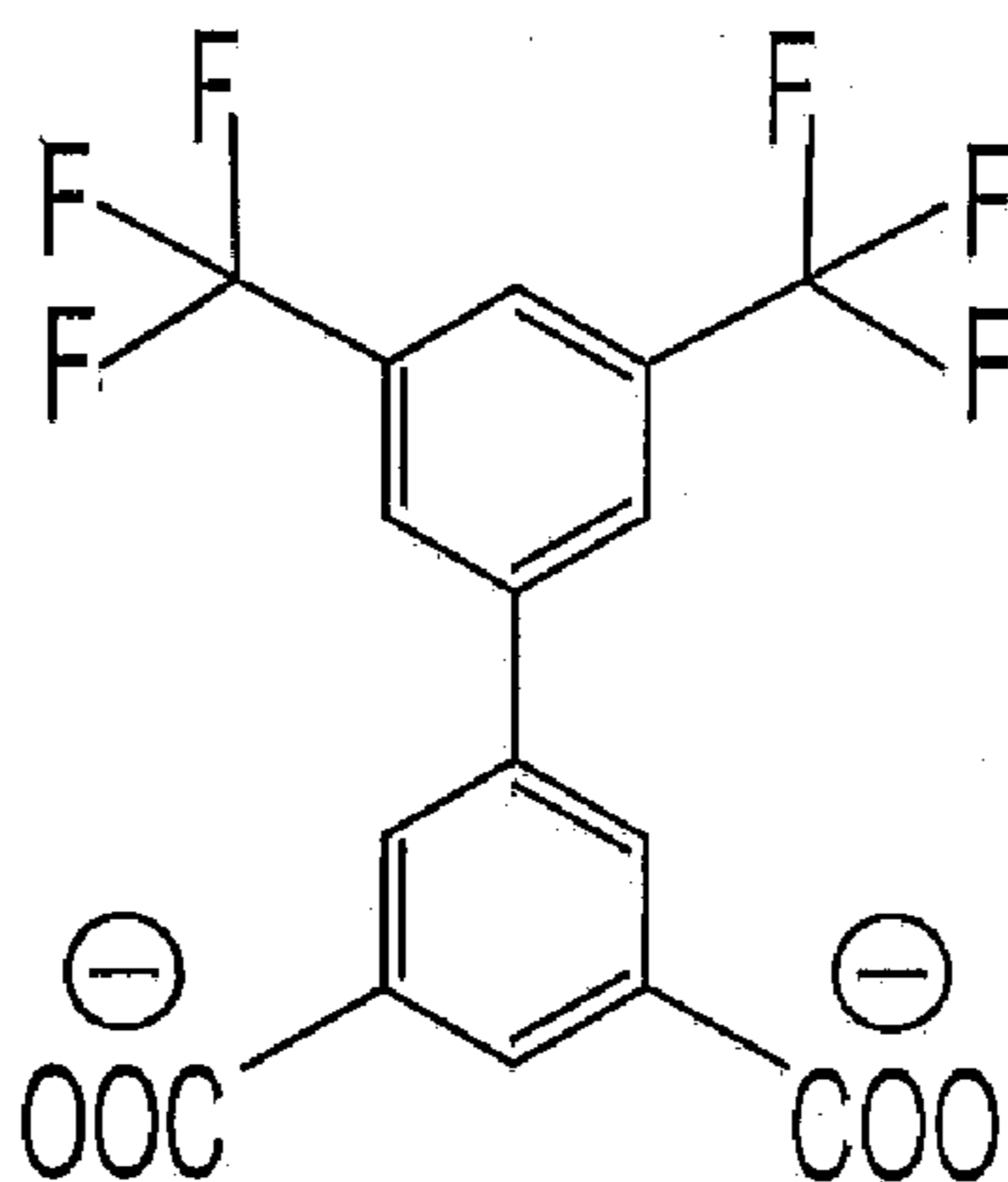
3',5'-bis-trifluoromethyl-biphenyl-3,5-dicarboxylate BTFMBPDC
