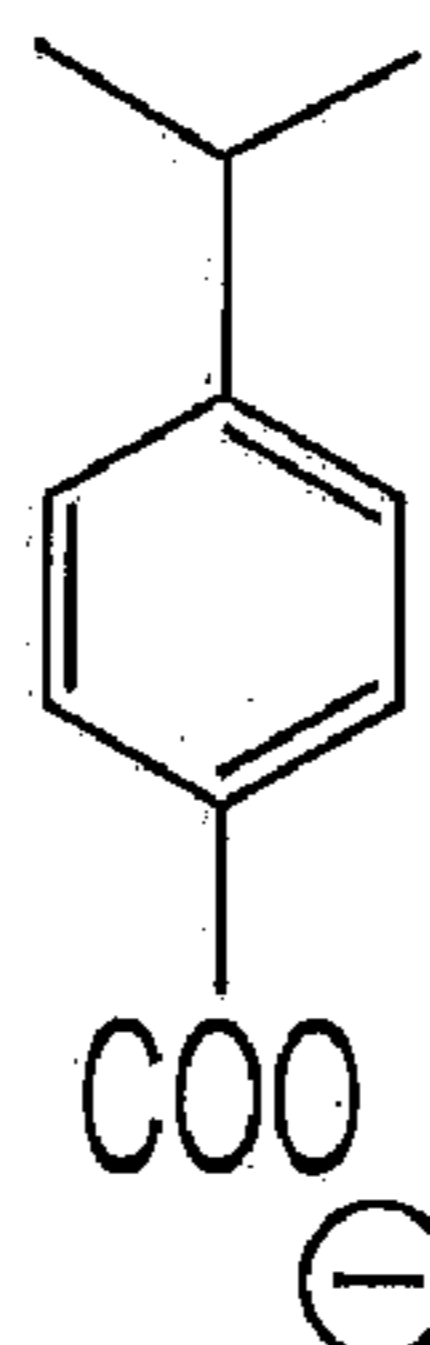
4-isopropyl-benzoate IPB
