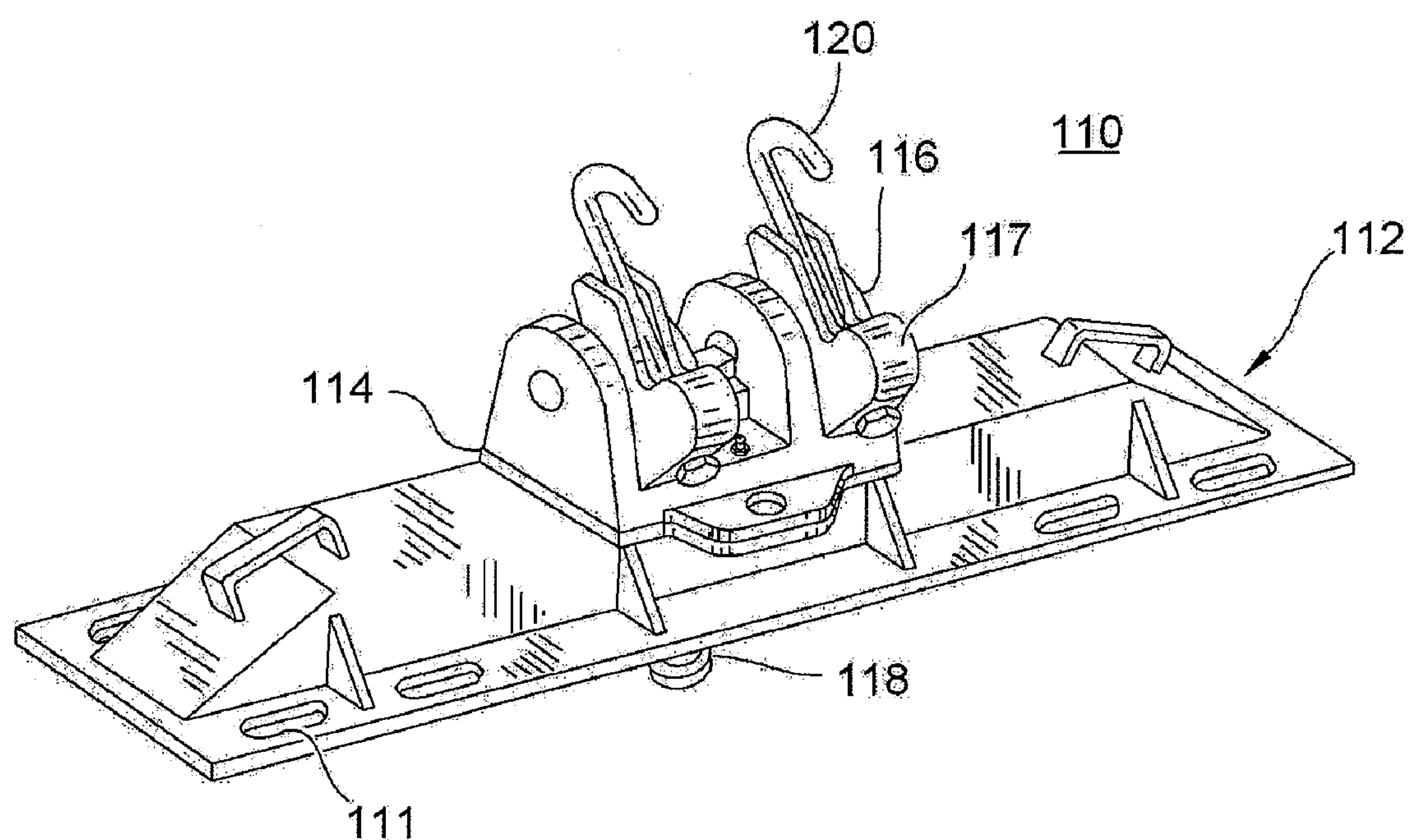
FIG. 9 PRIOR ART
