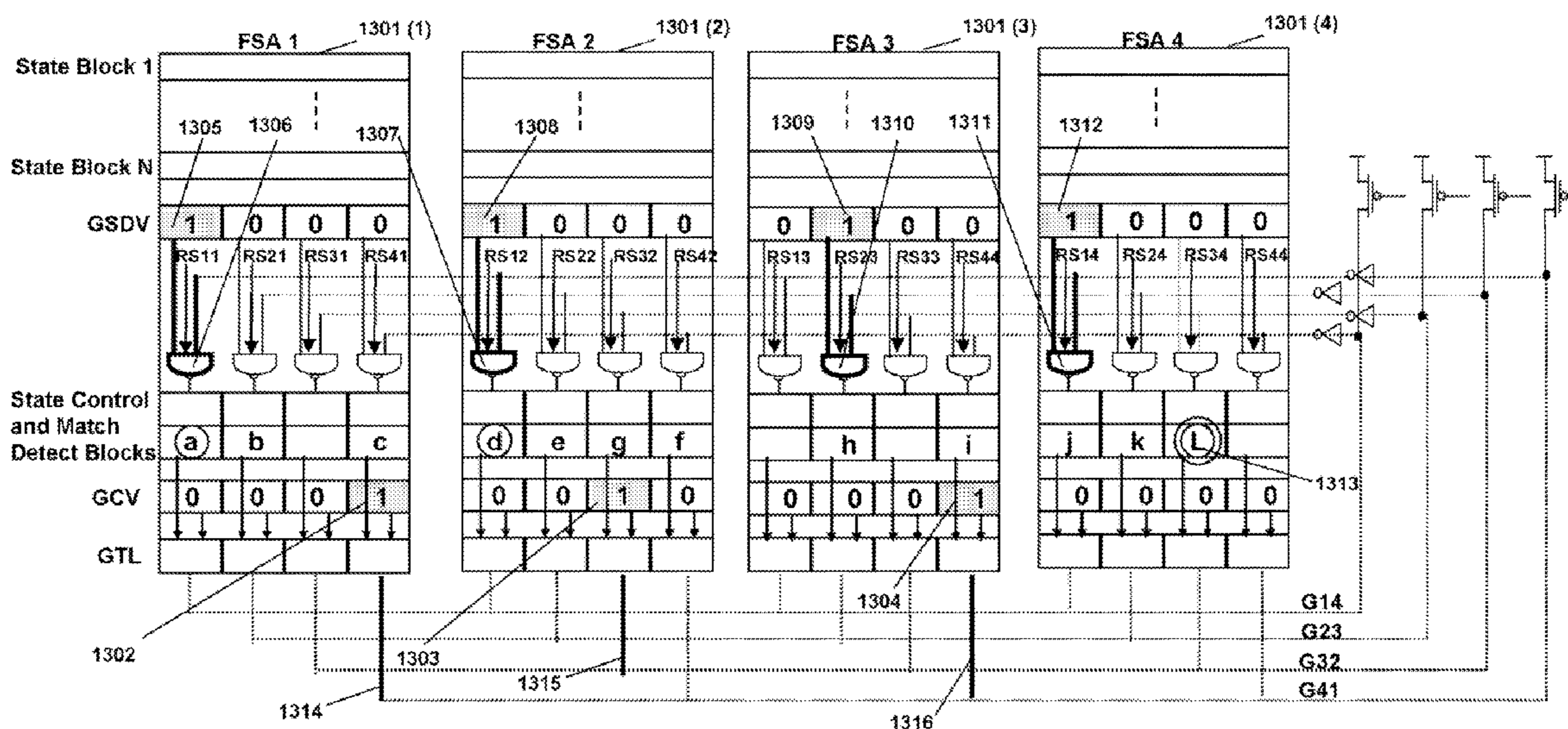
PRISM Row-wise FSA Extension Example #2
