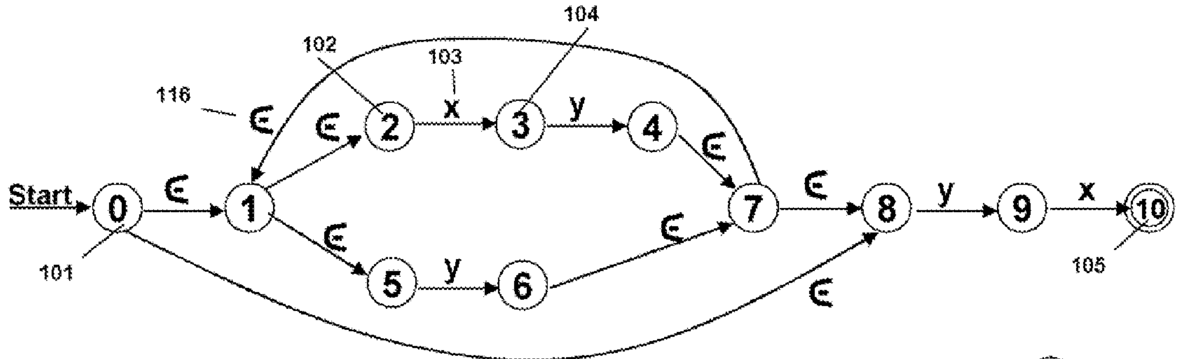
Fig. 1a Thompson's NFA (Prior Art)
