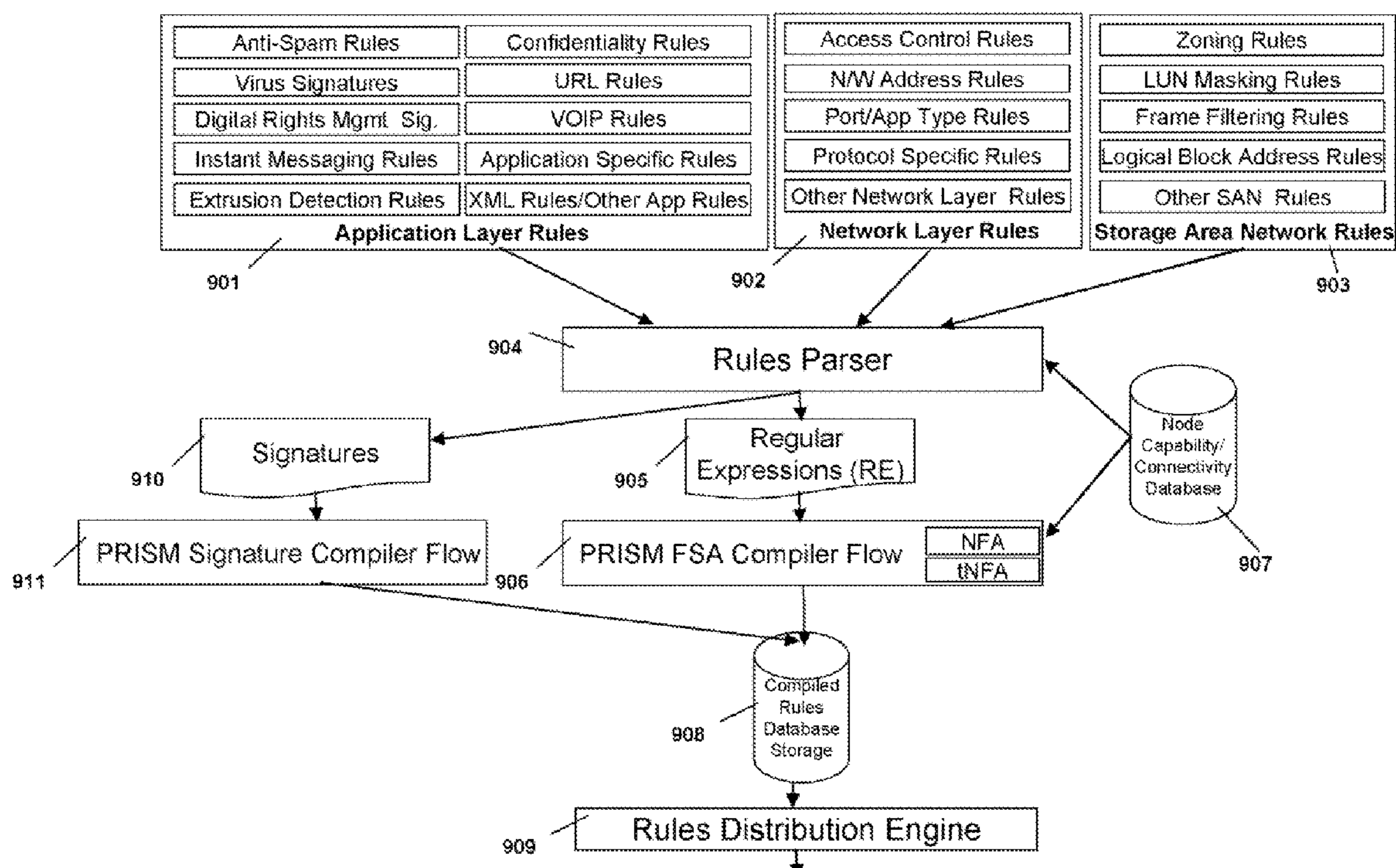
Fig. 9 PRISM Search compiler flow (full + incremental rule distribution)
