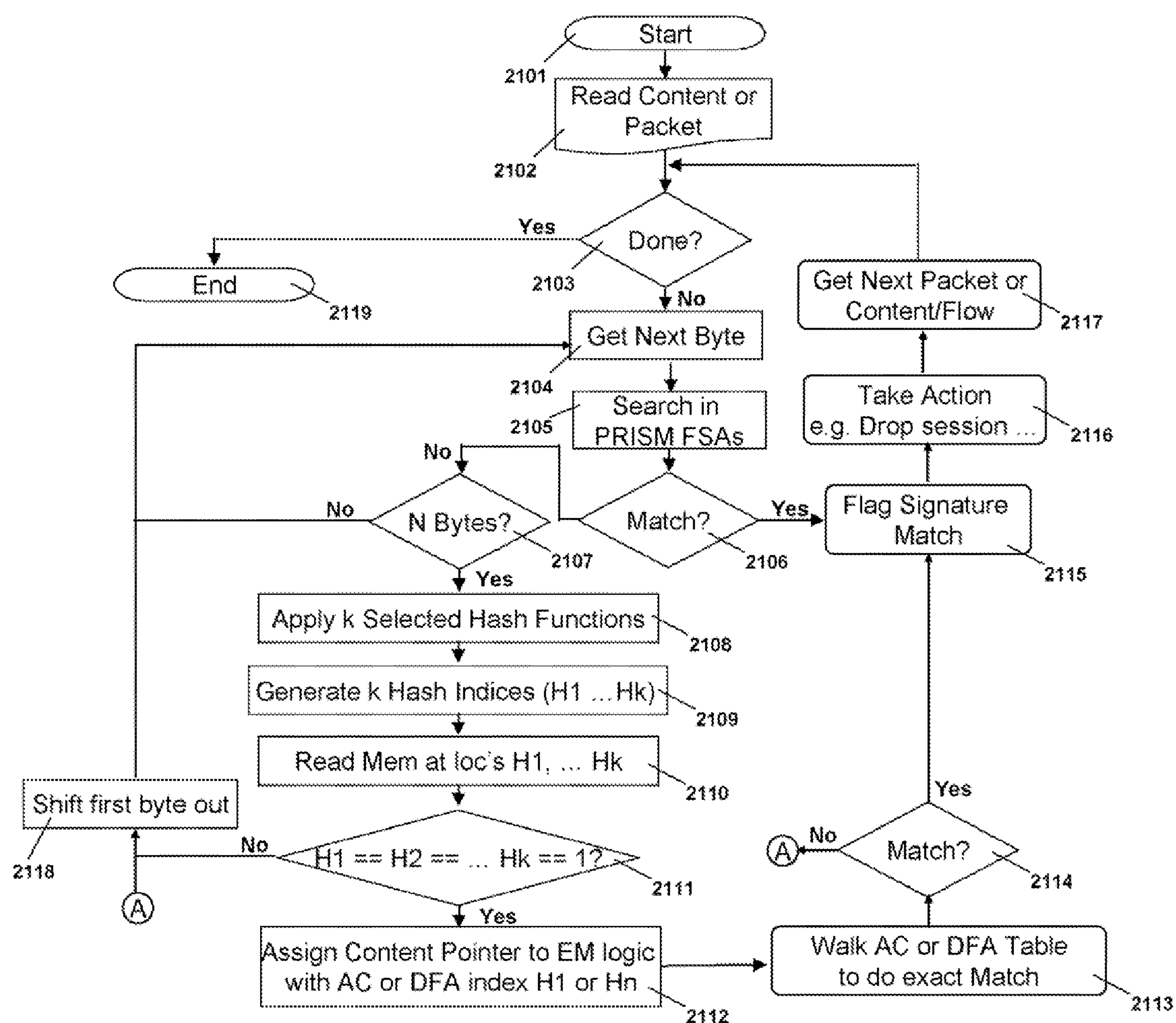
Fig. 21 PRISM Signature Search Flow
