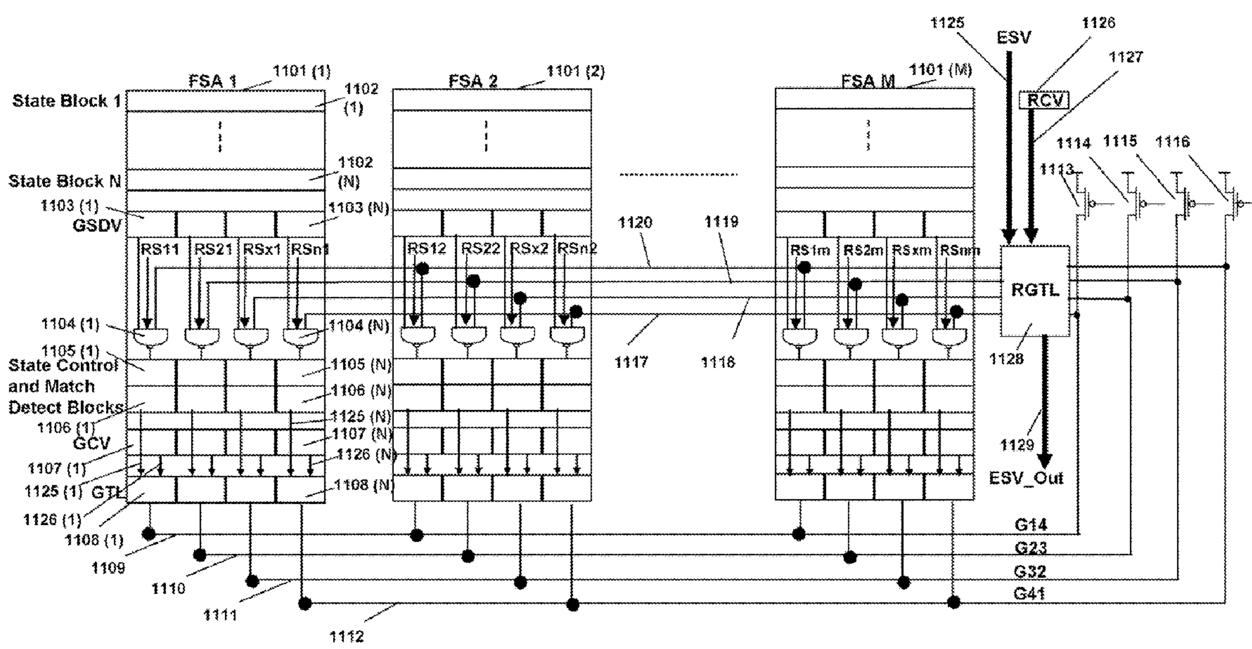
Fig. 11A PRISM Rule Group FSA Extension
