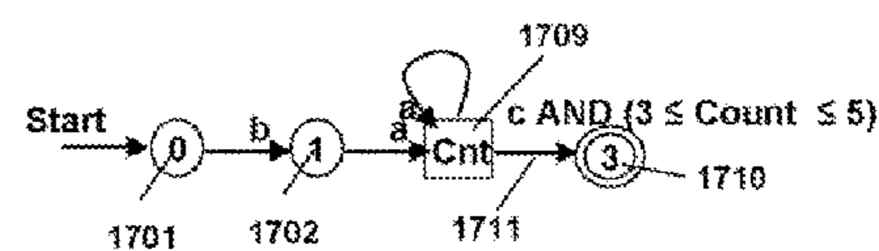
Fig. 17B PRISM FSA with Interval Symbol
