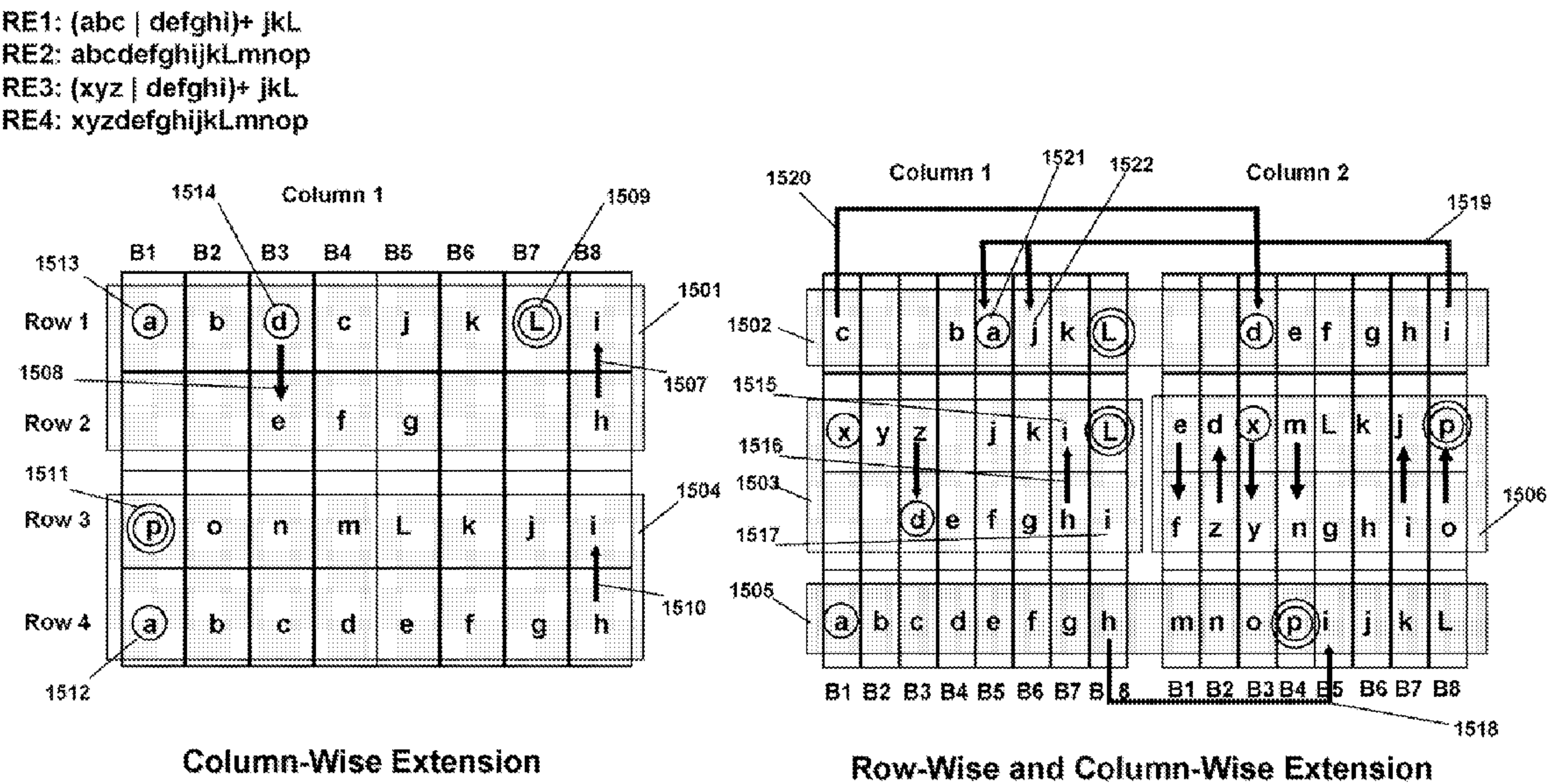
Fig. 15 PRISM FSA Extension Example #1
