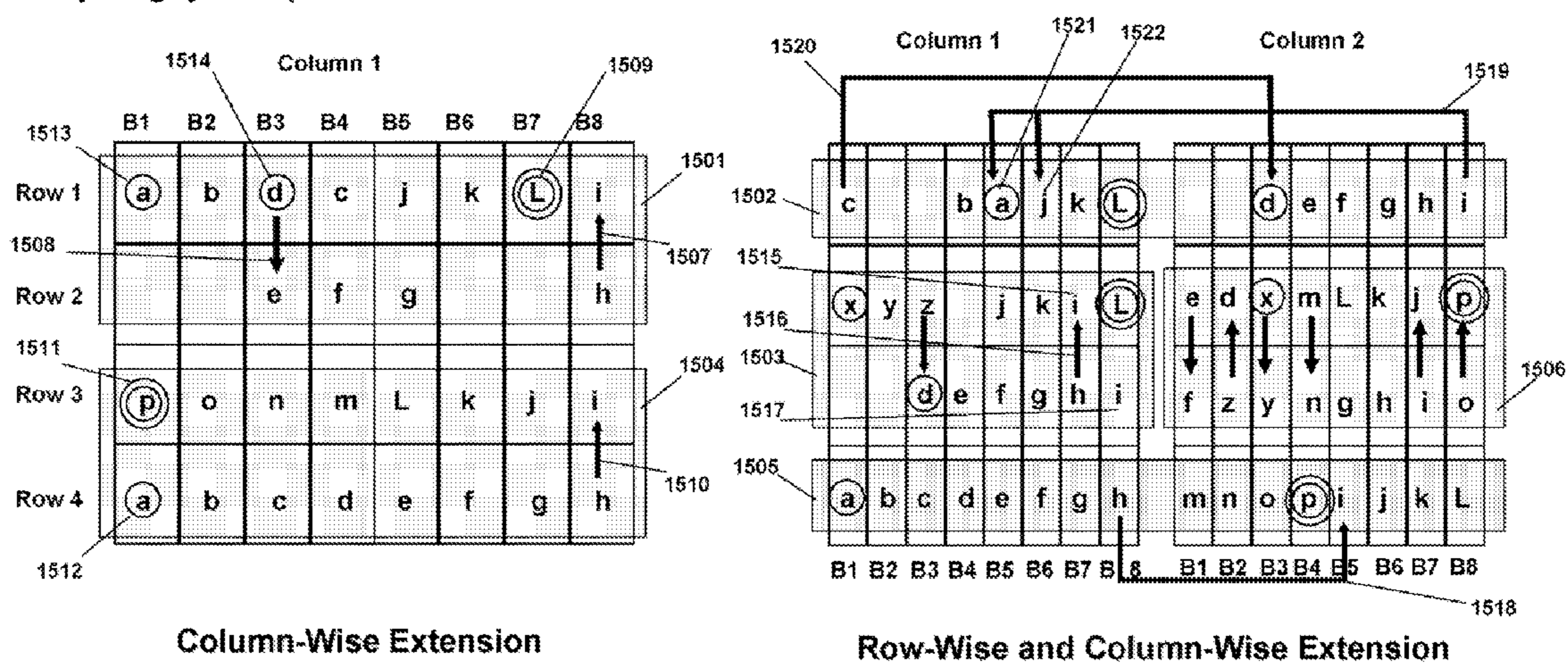
Fig. 15 PRISM FSA Extension Example #1
