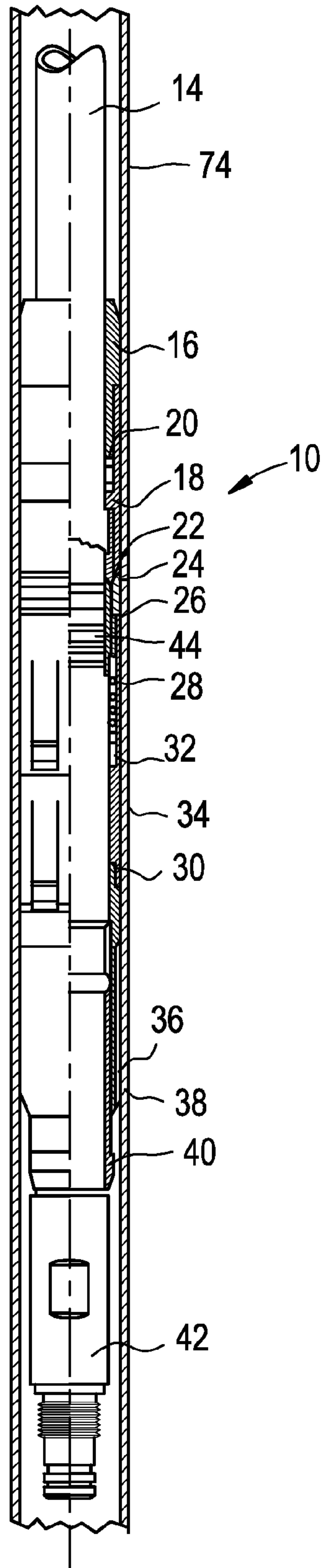
FIG. 3 (PRIOR ART)
