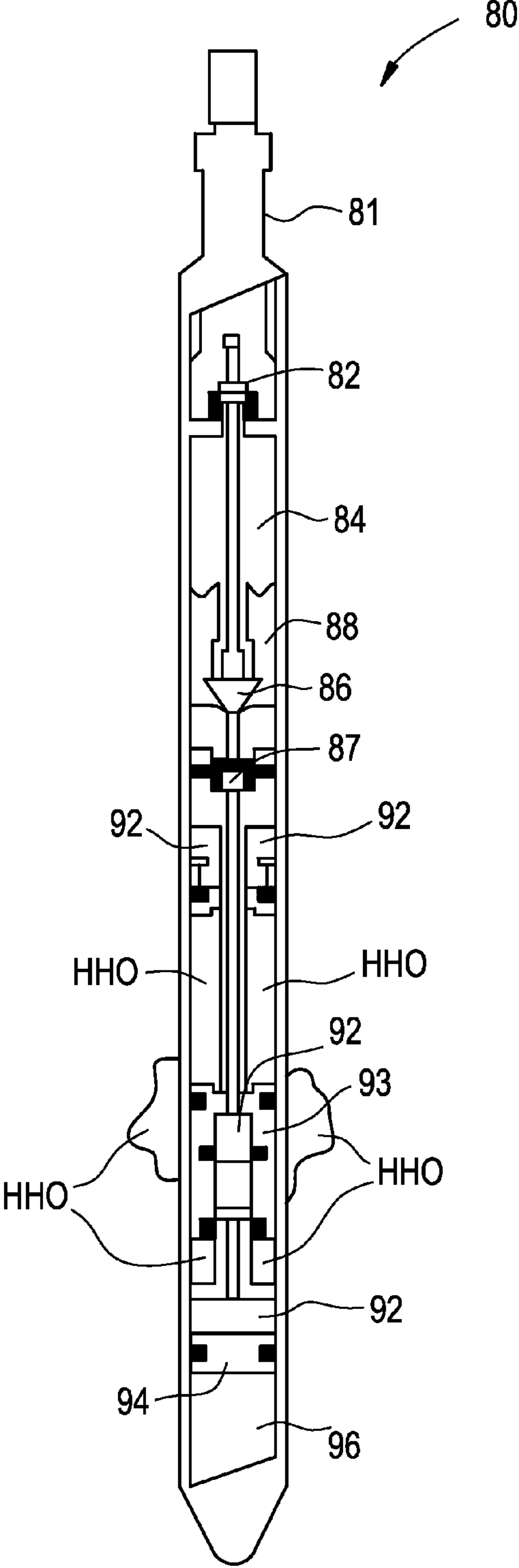
FIG. 5D (PRIOR ART)
