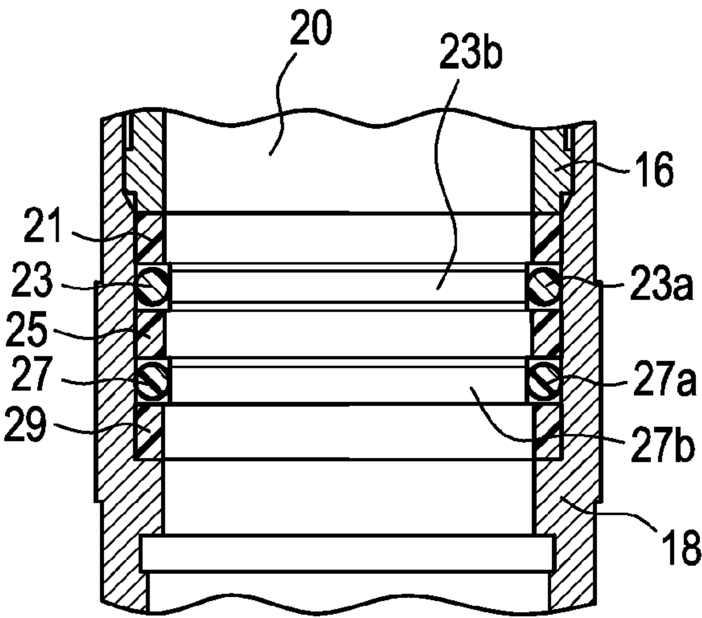
FIG. 4 (PRIOR ART)
