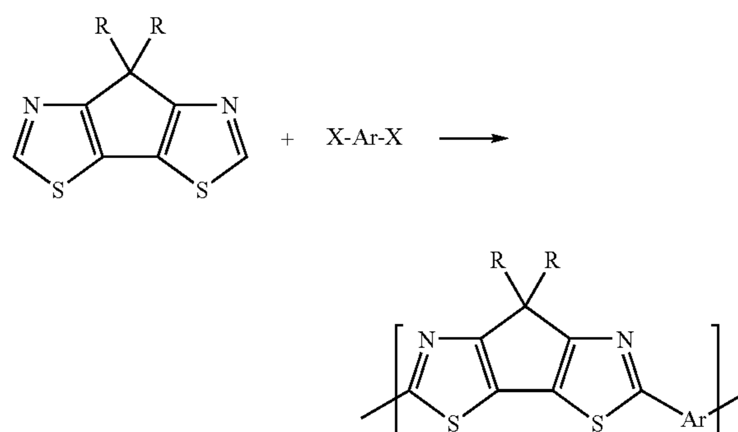
Scheme II
