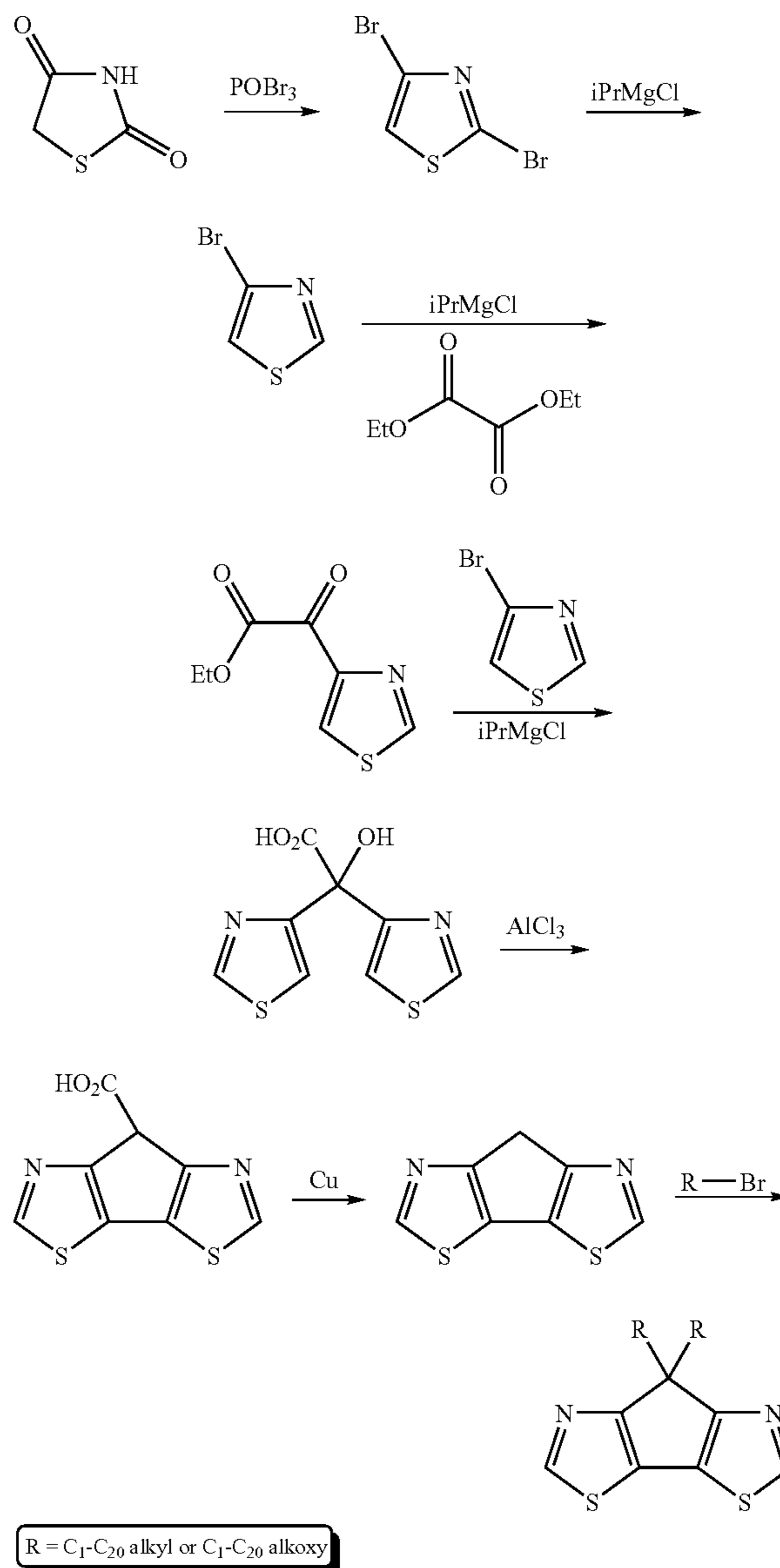
Scheme I
