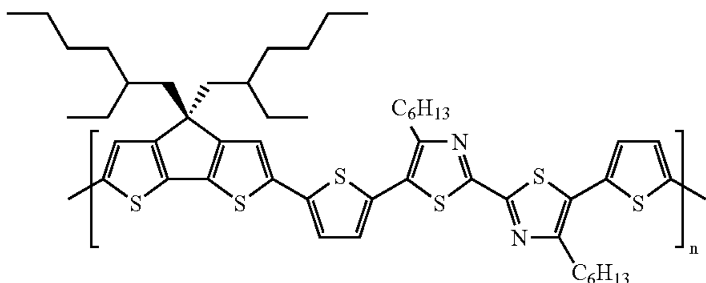
Polymer 1
