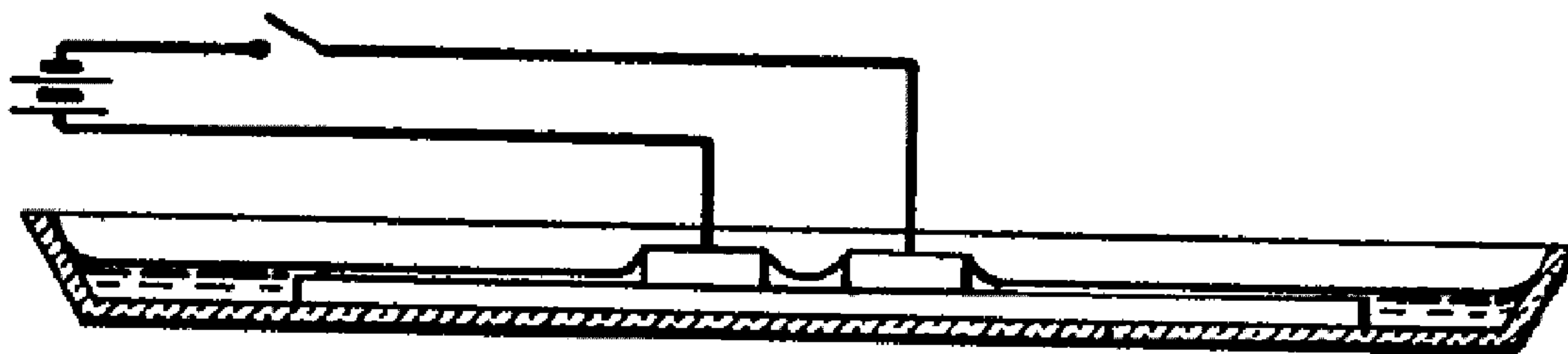
FIG. 105 (Matz, US 2,062,468)
