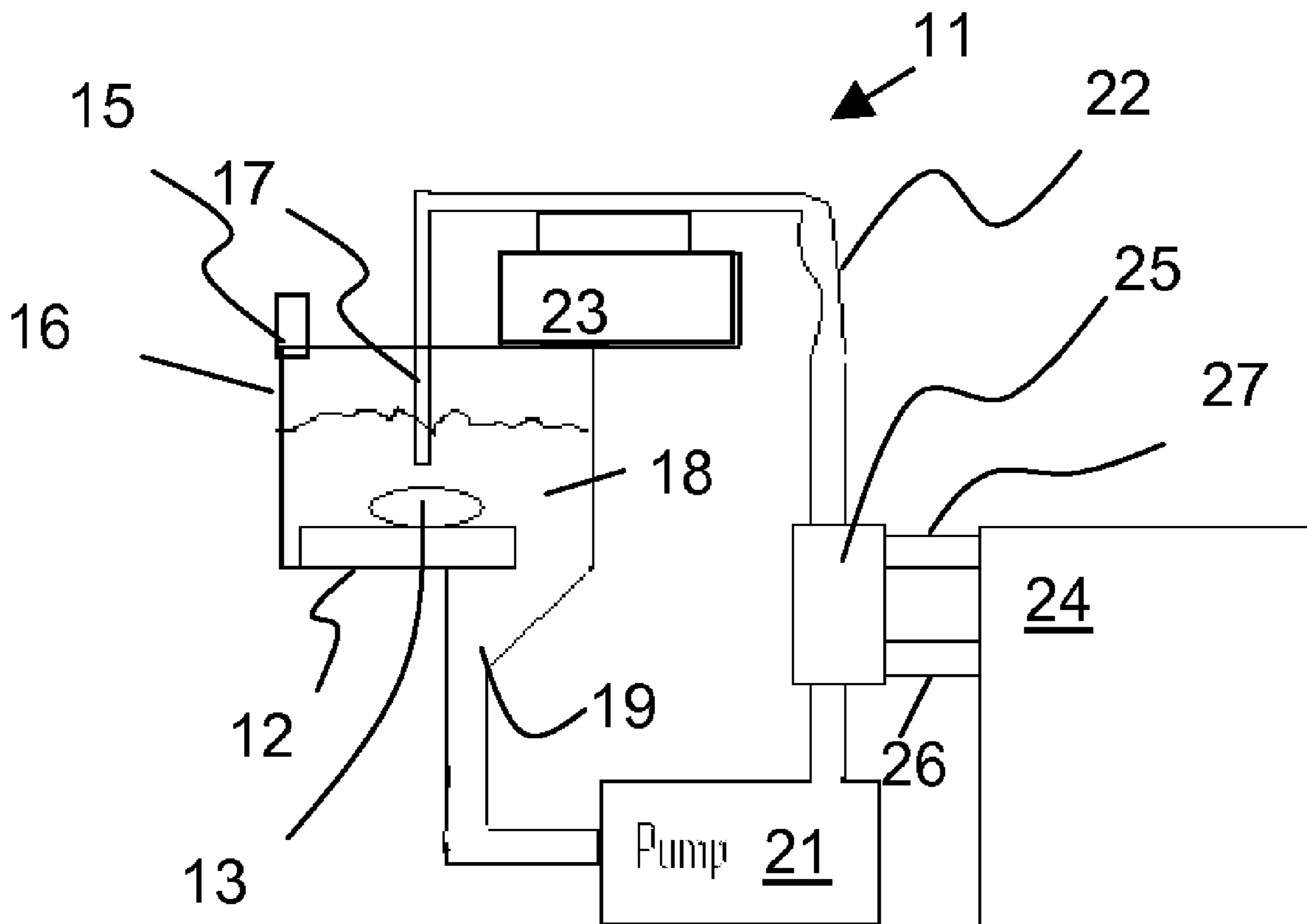
Closed loop submerged fluid jet polishing
