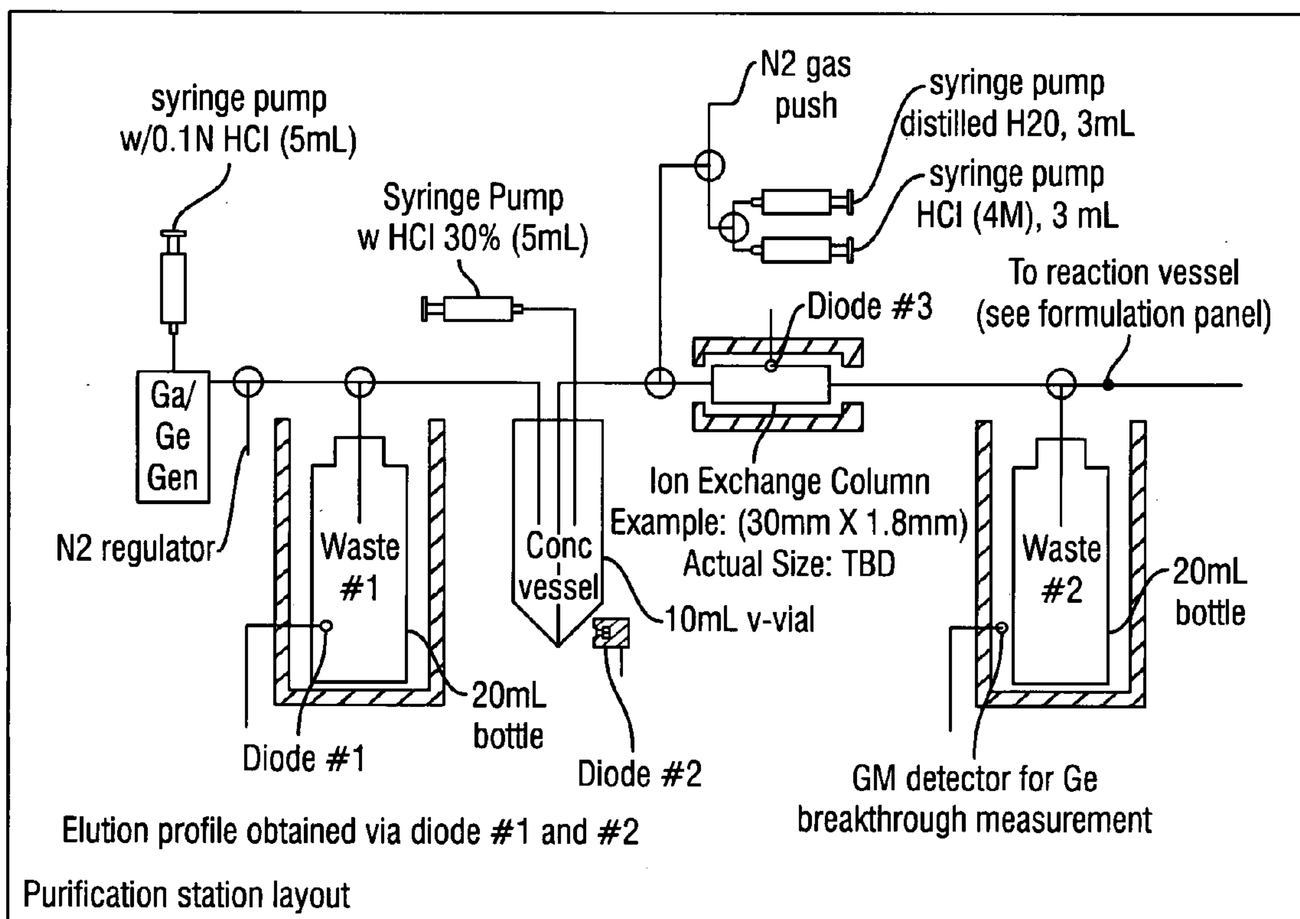
Step 4. Concentration of 68 GaCl 3 with 30% HCl
