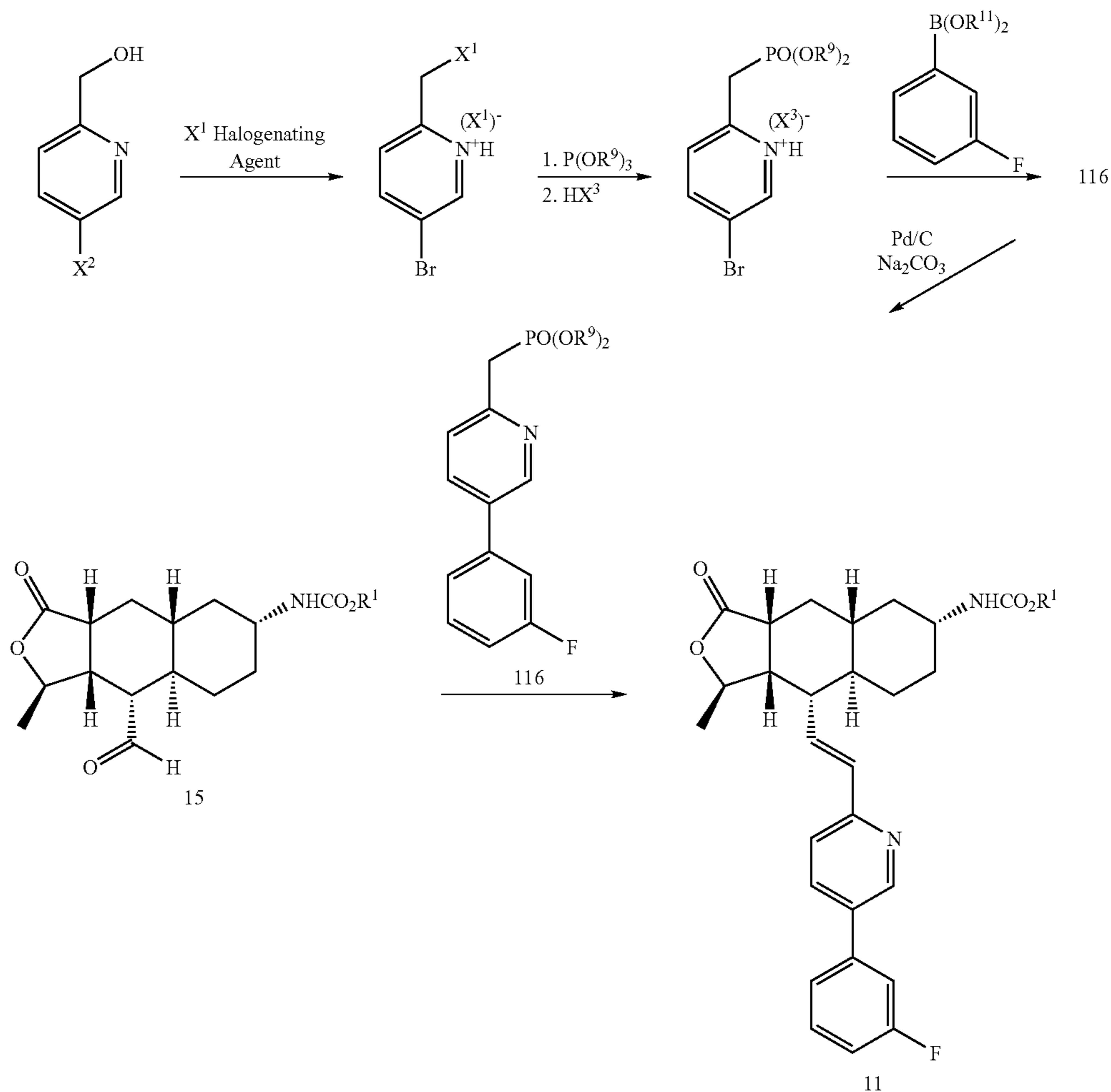
SCHEME III
