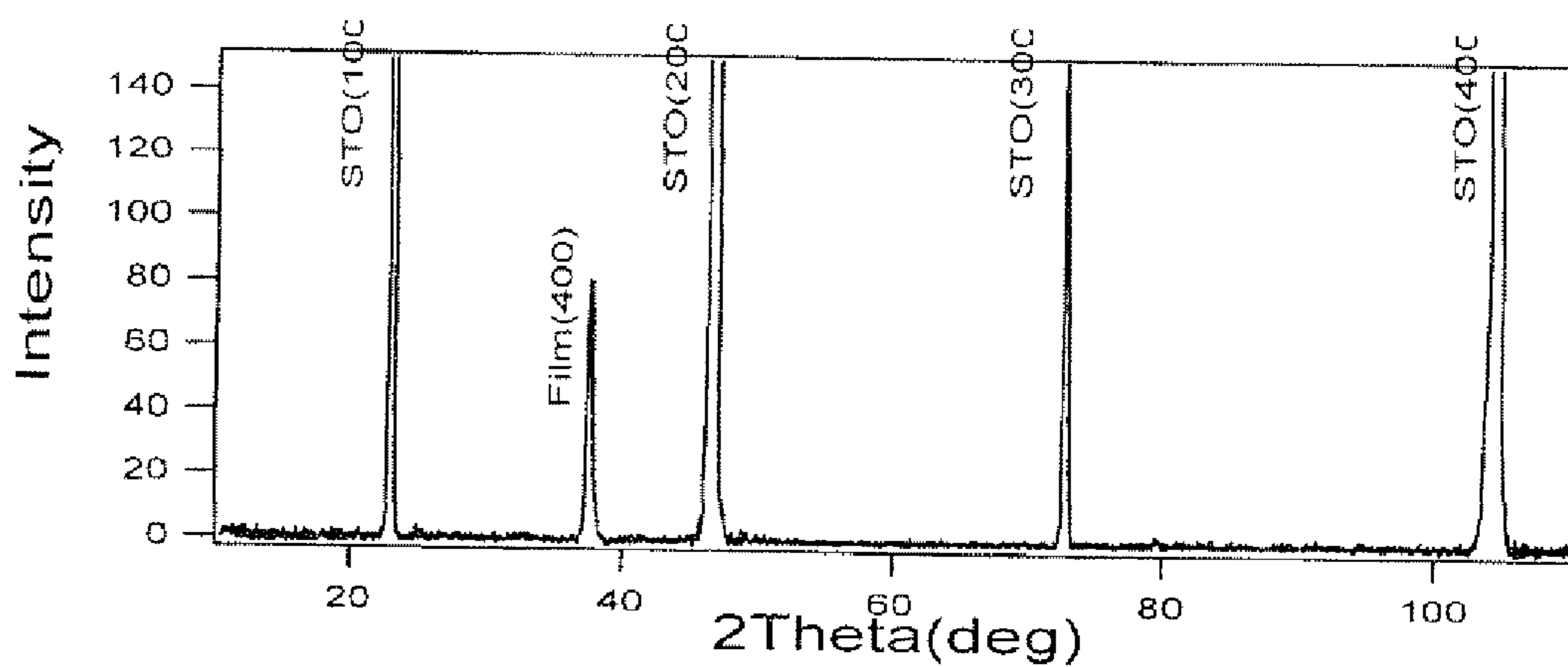
(a)Ta15%
