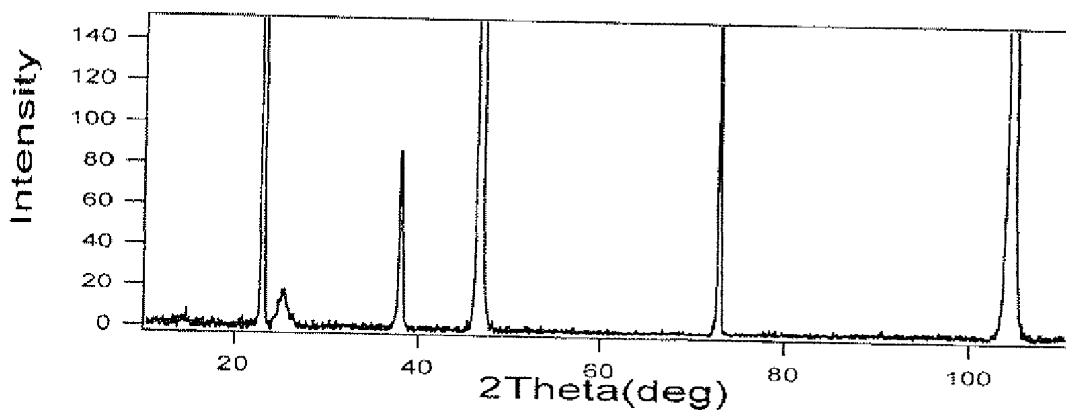
(b) Ta0.5%
