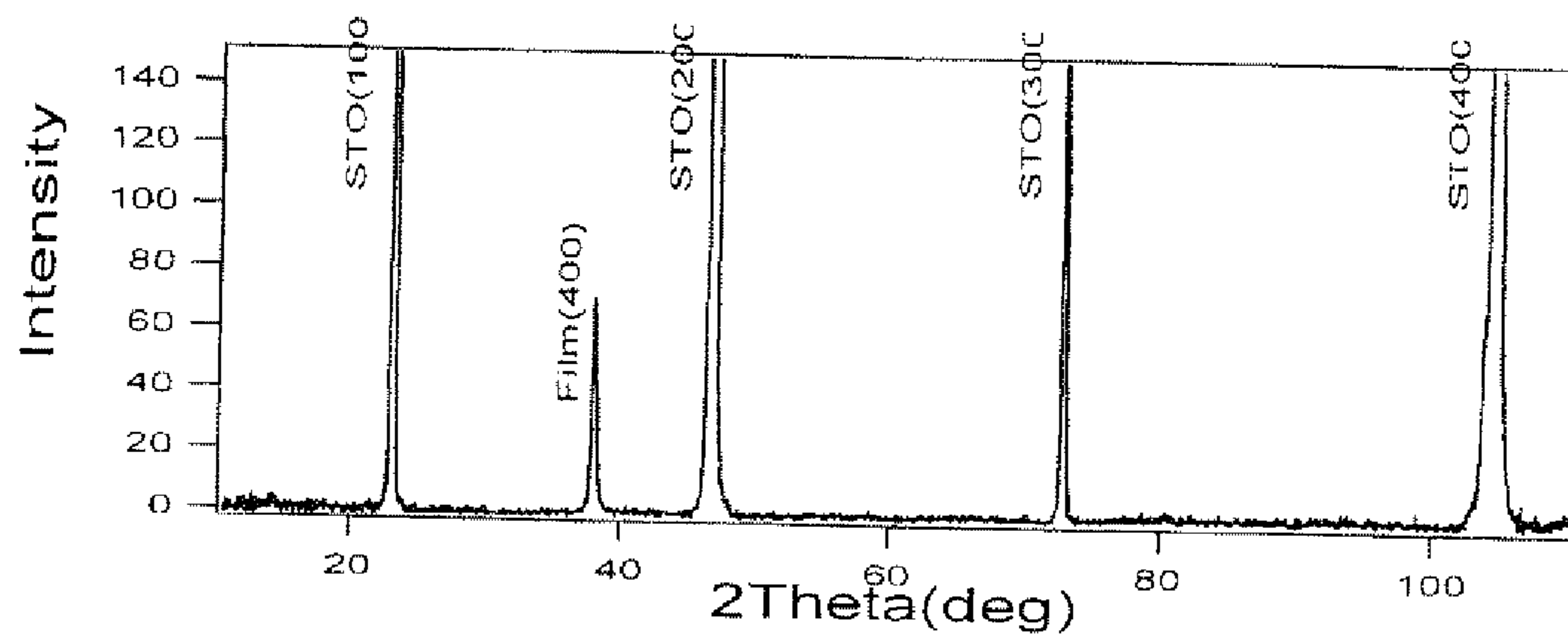
(a) Ta0.2%
