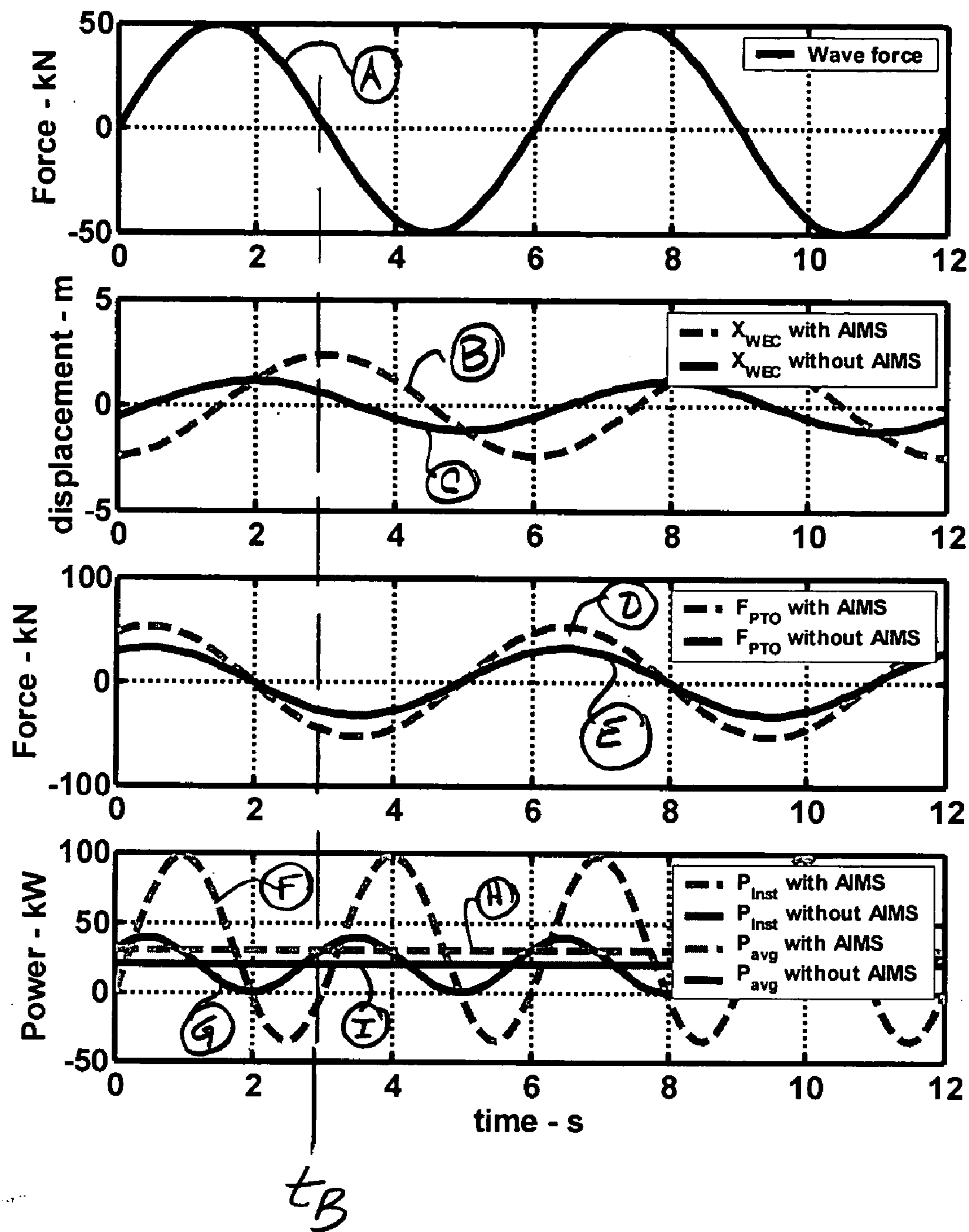
Power conversion - Strong restoring case.
