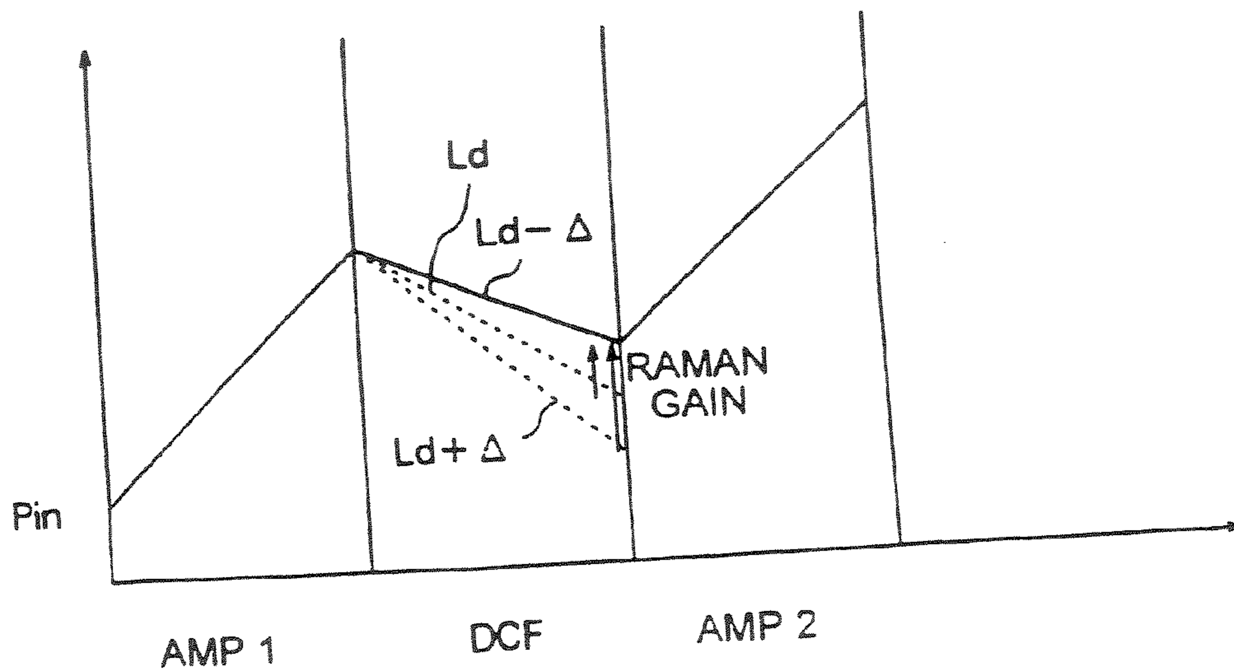
COMPENSATION FOR FLUCTUATION IN LOSS OF DCF DUE TO RAMAN AMPLIFYING EFFECT
