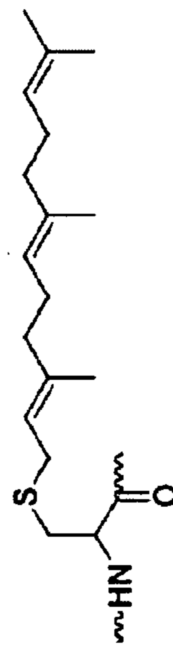
farnesylcysteine (4)
