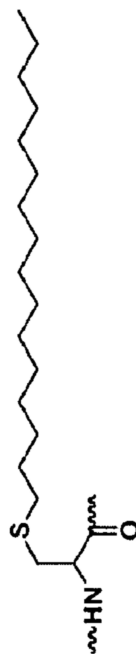
S-hexadecylcysteine (5)
