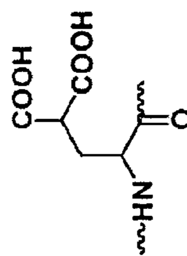
γ-carboxyglutamic acid (6)
