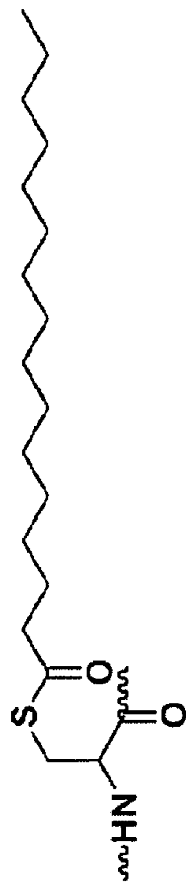
palmitoylcysteine (3)
