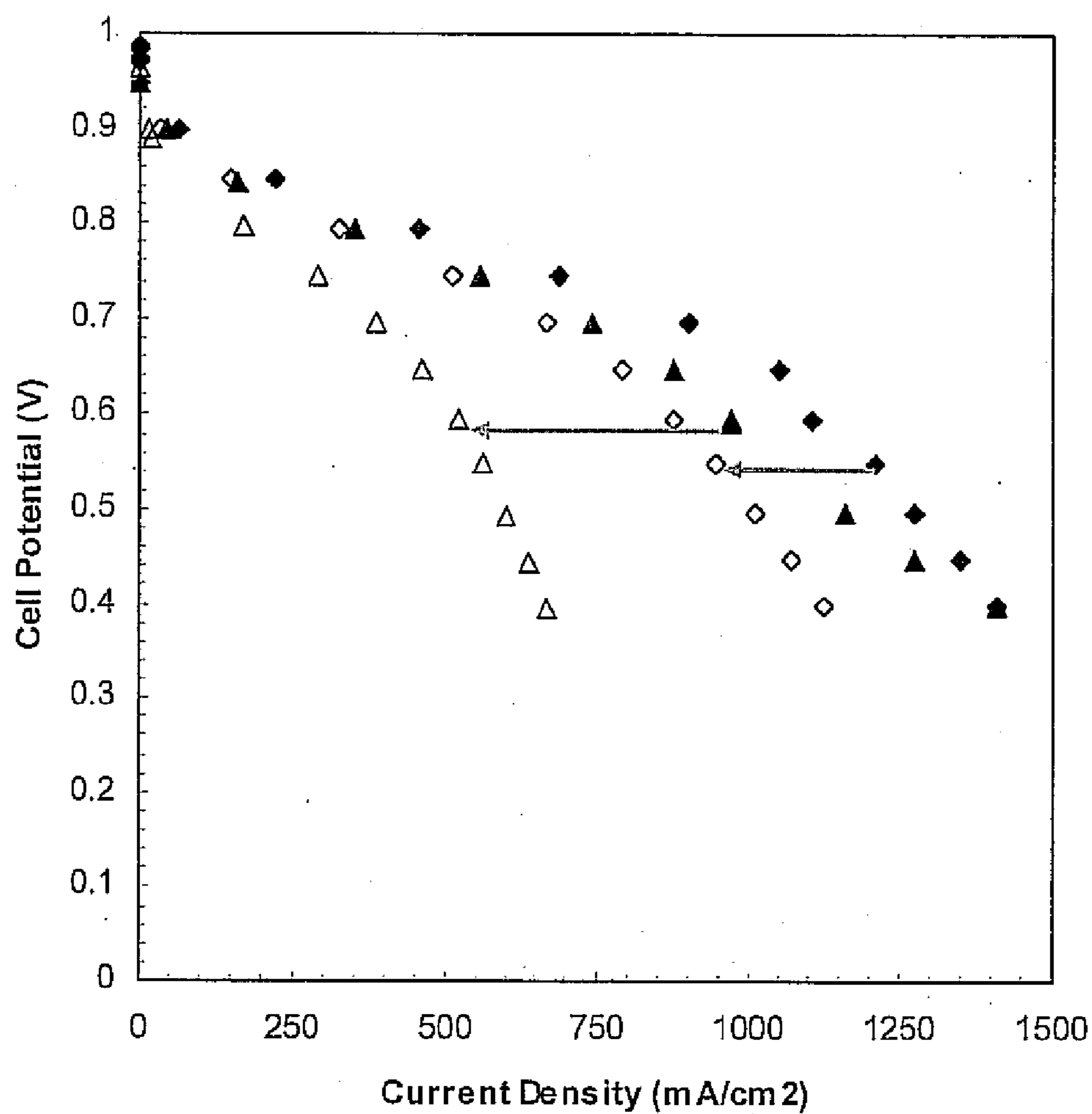
Figure 4. Polarization curves before and after 75 hour potentiostatic tests on MEAs prepared with Pt nanosheets at time 0 (◆) and 75 h (◇) and with Pt black at time 0 (▲) and 75 h (△) for loadings of 7 mg/cm 2 .
