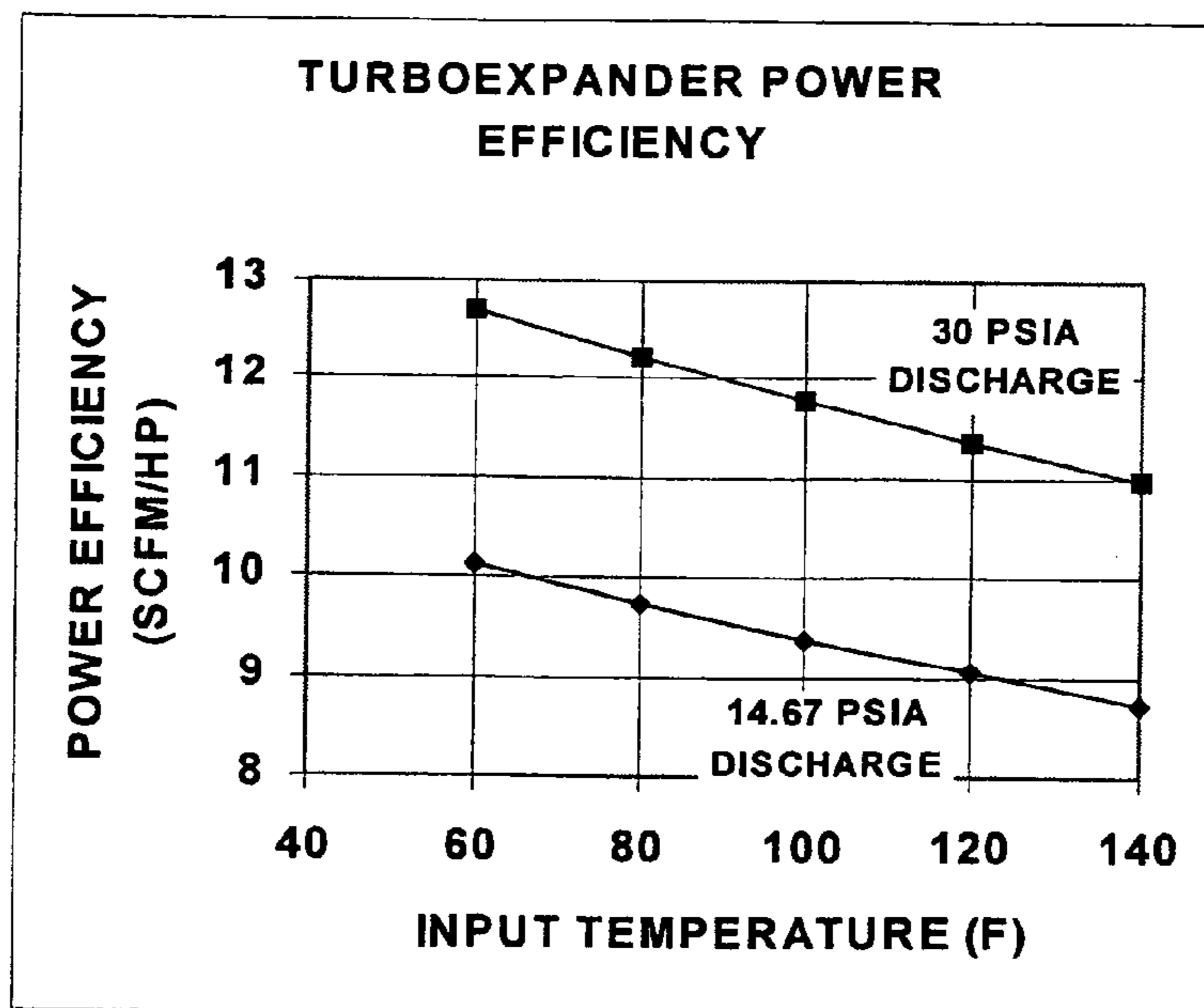
Figure 10 Turboexpander Performance with 85% Thermodynamic Efficiency
