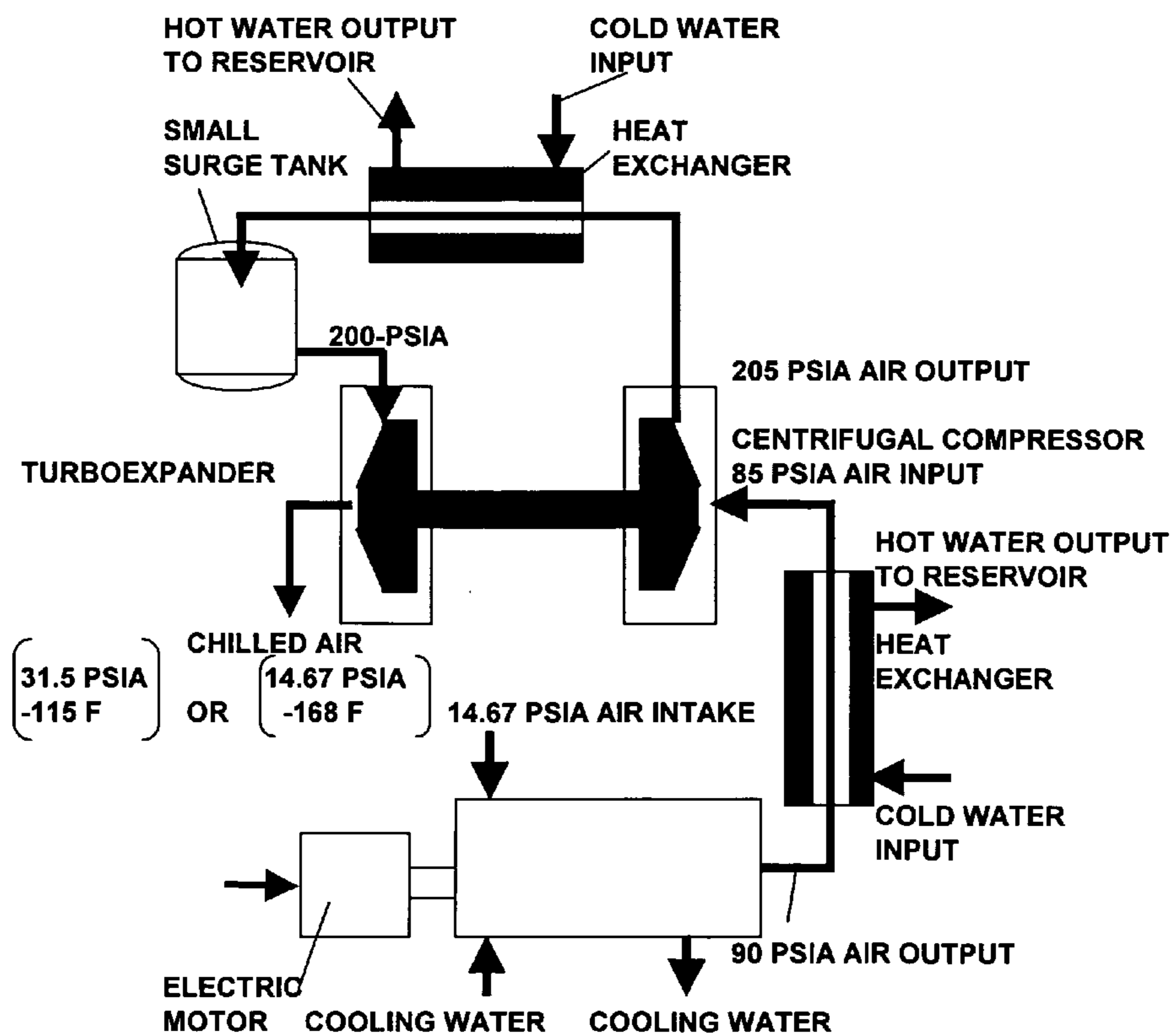
Figure 9. Chilled Air Generated by Turbocompressor and Turboexpander (Turbocompressor and Turboexpander Configuration)
