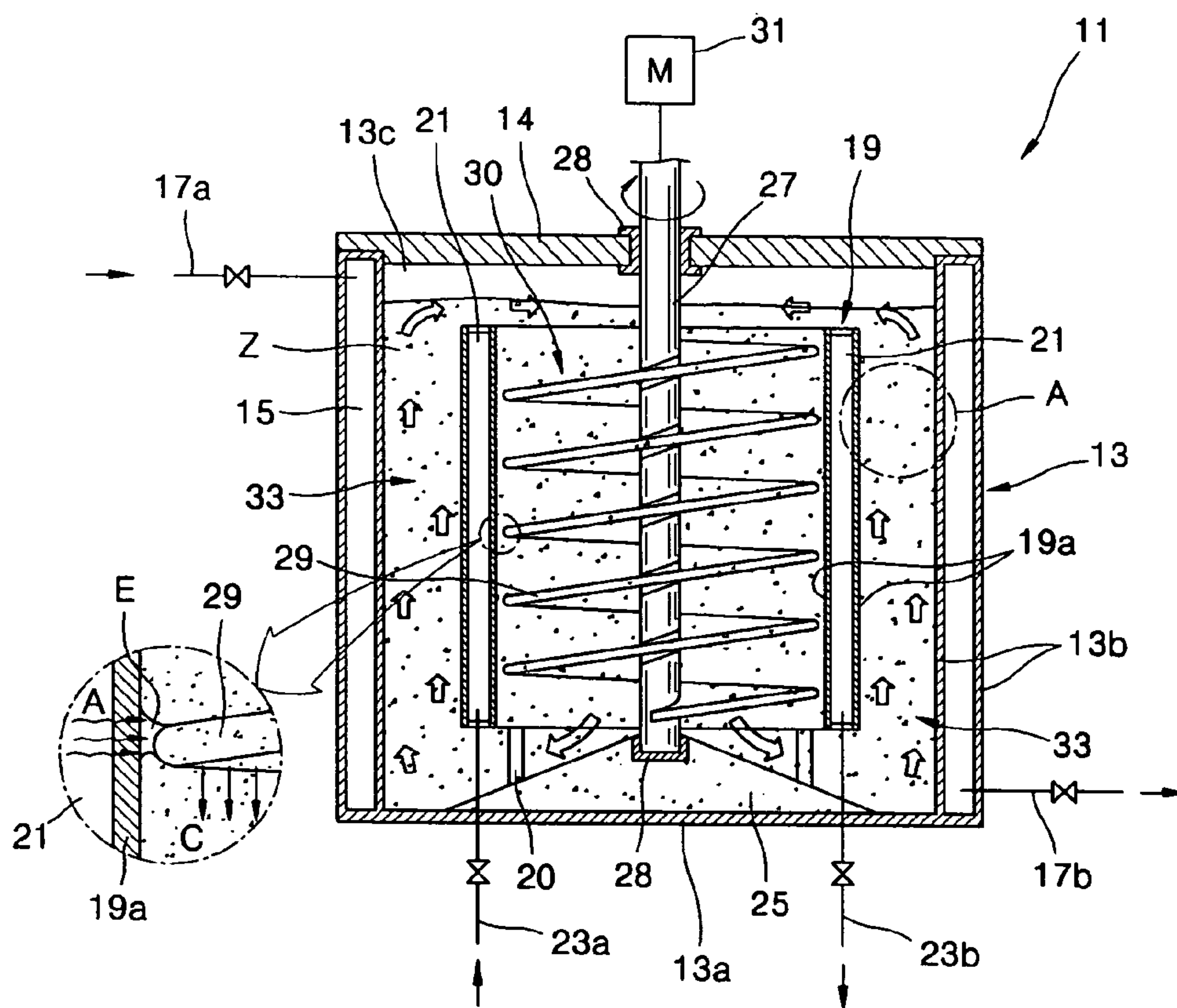
FIG. 1 (PRIOR ART)
