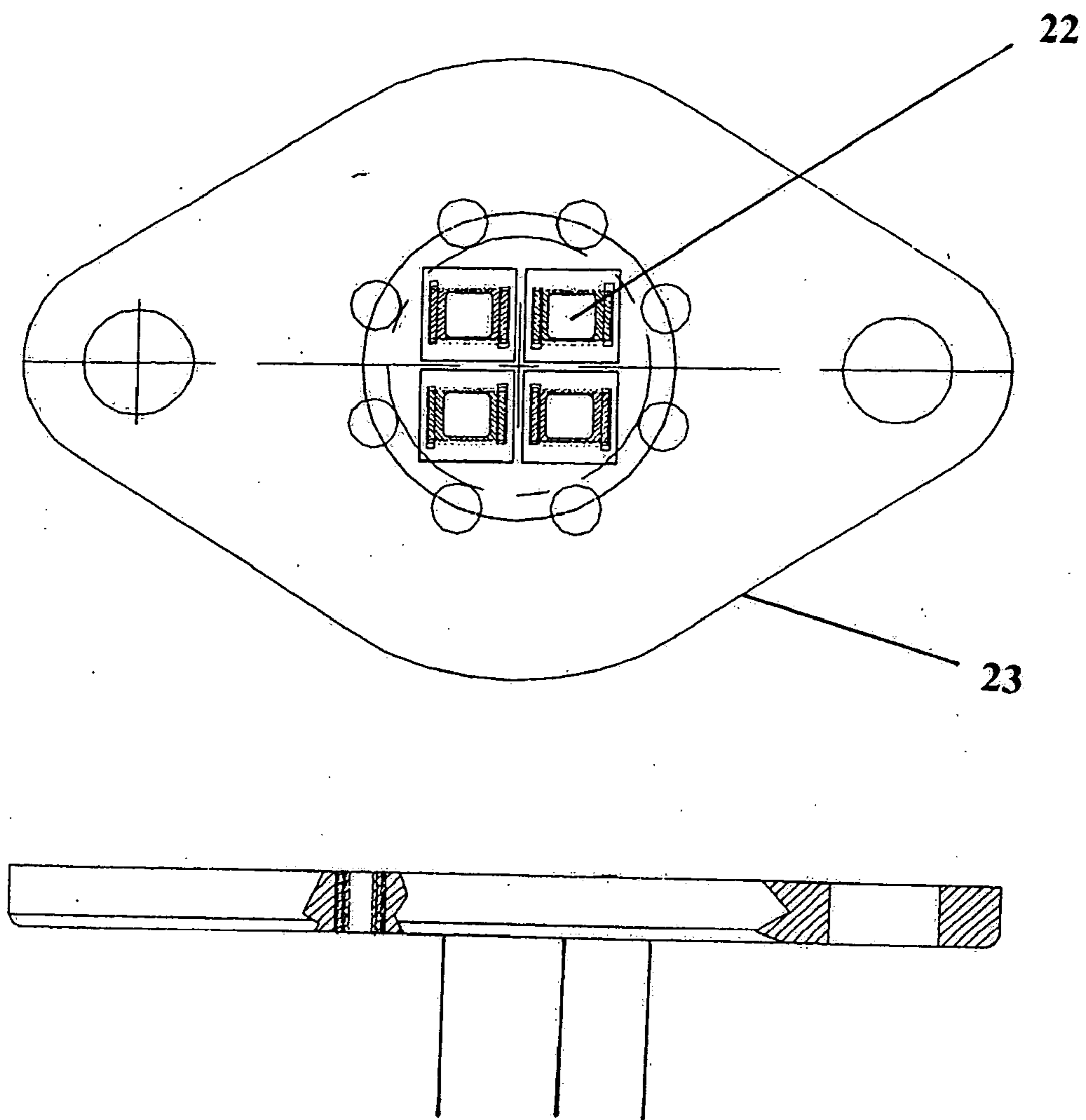
Figure 8. A packaging scheme for mounting four standard infrared sources onto a special TO8 header.
