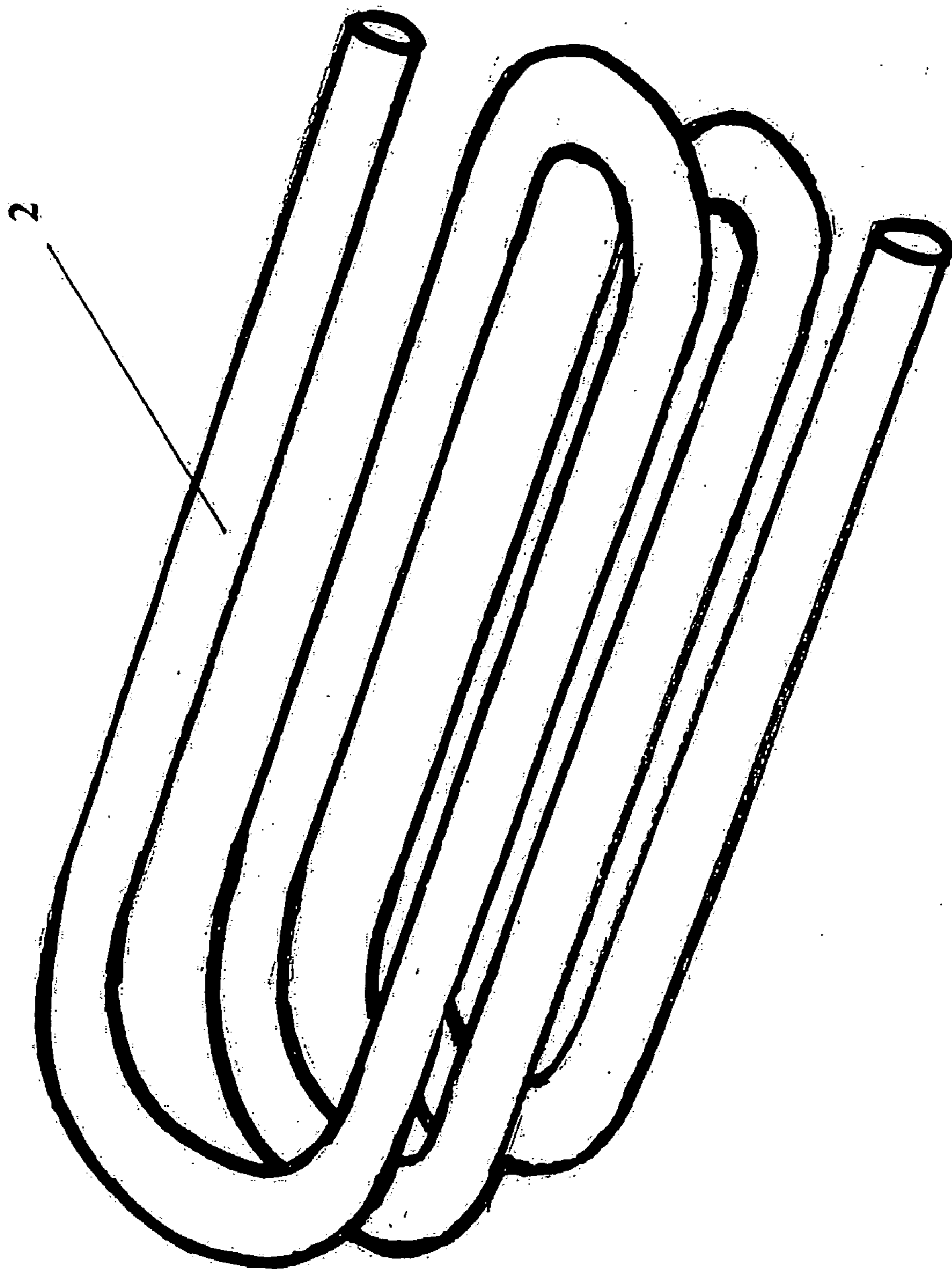
Figure 2. A schematic layout drawing of the Super Tube invention showing a bending angle of 90^\circ from the original orientation with five U ( 180^\circ ) turns.
