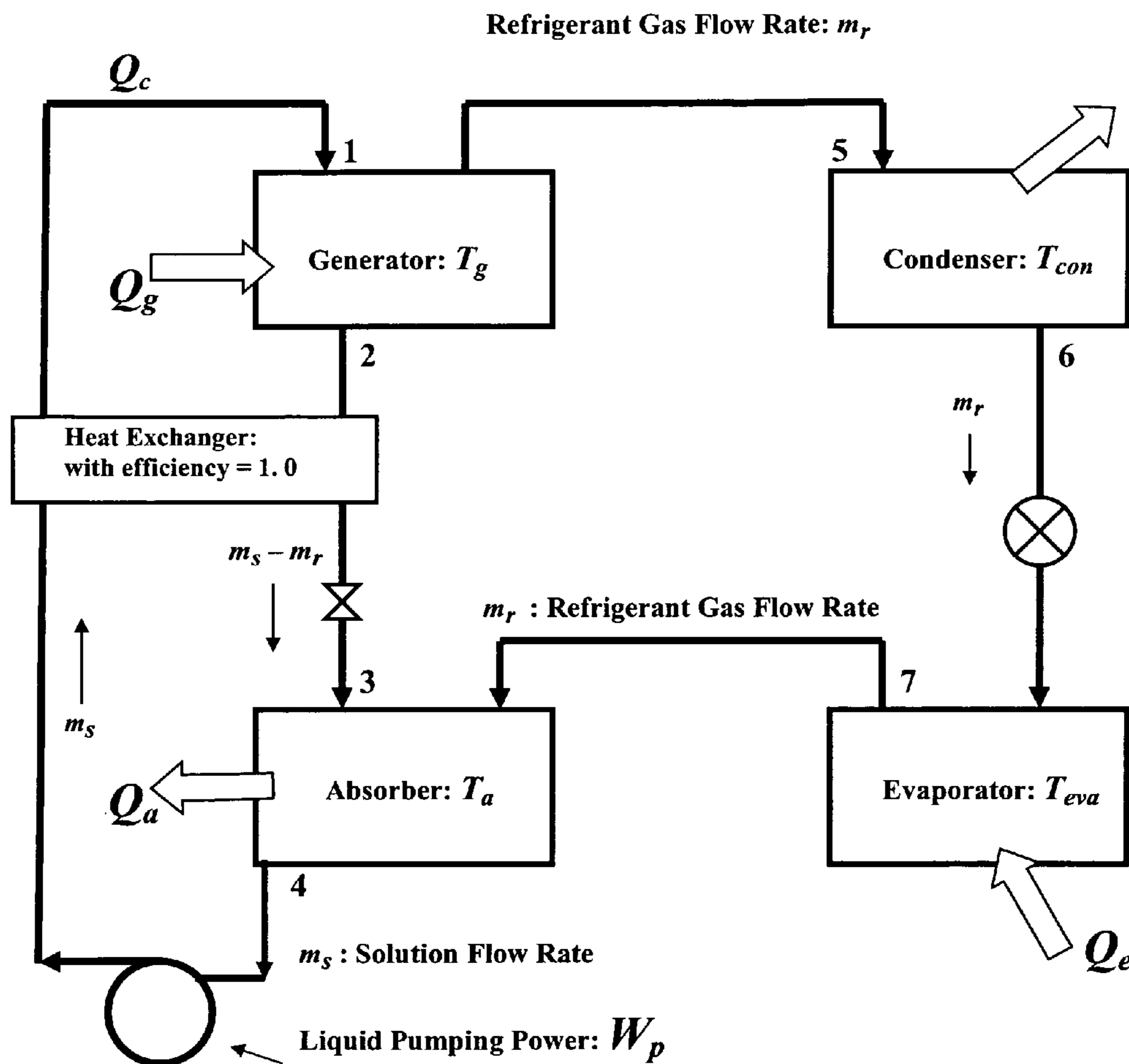
A schematic diagram of a simple absorption refrigeration cycle.
