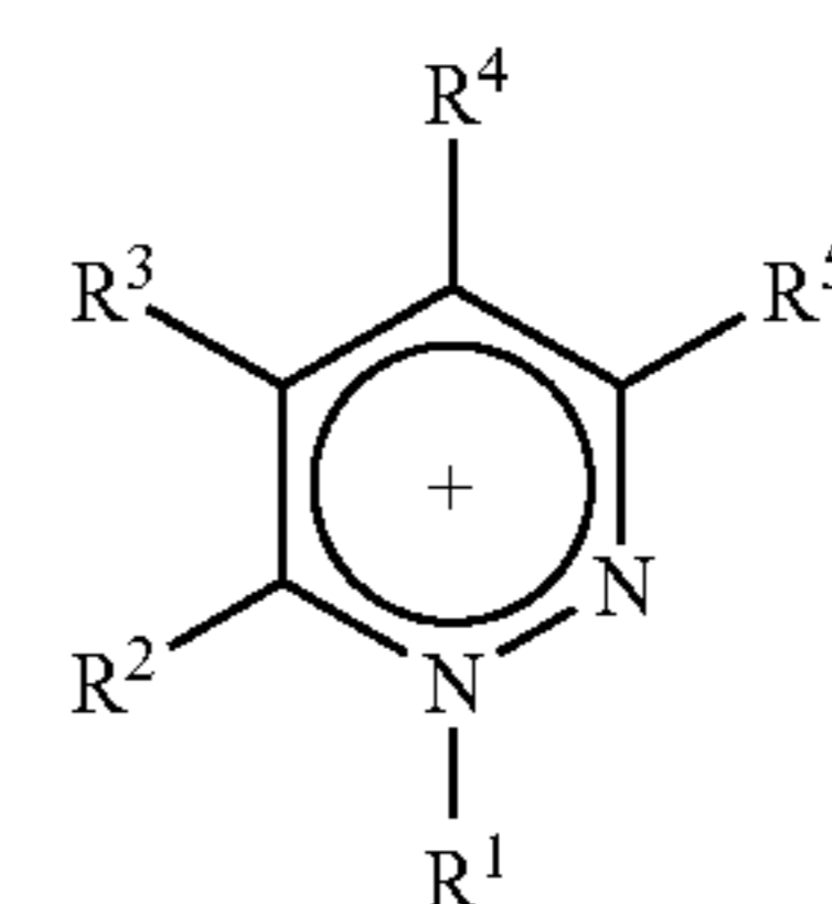
Pyridazinium
