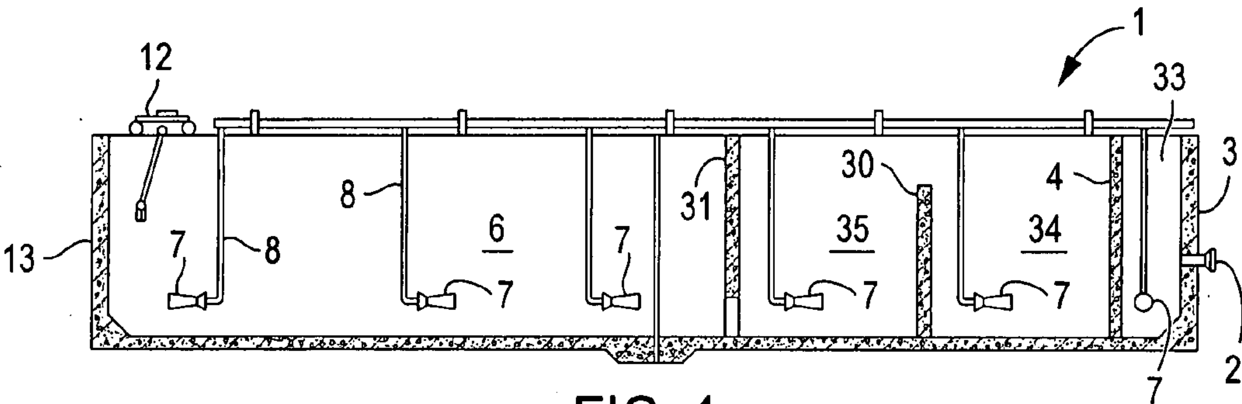
FIG. 1 PRIOR ART
