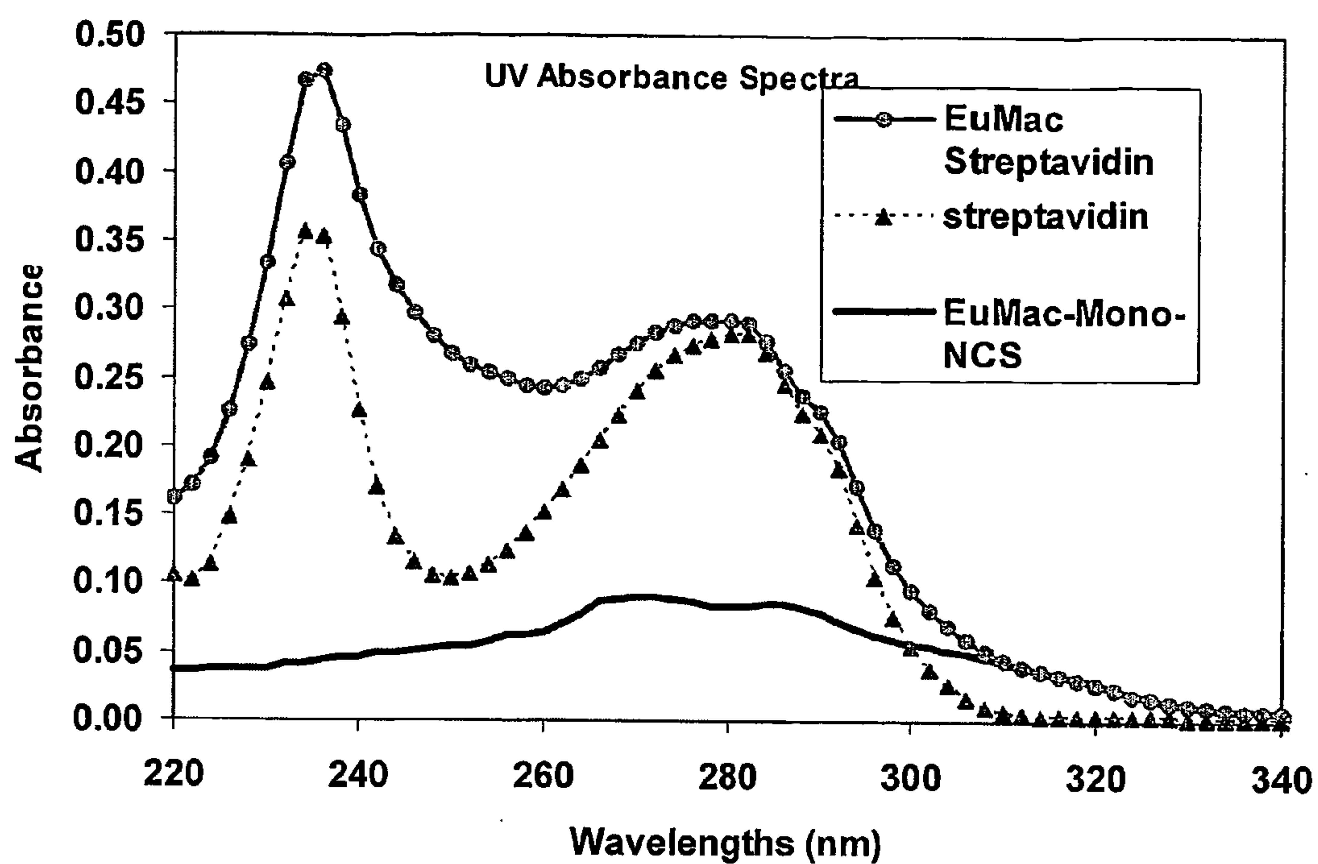
Figure 4 is a graphical presentation of the ultraviolet absorption spectra of the EuMac-mono-NCS, the EuMac coupled to streptavidin, and streptavidin.
