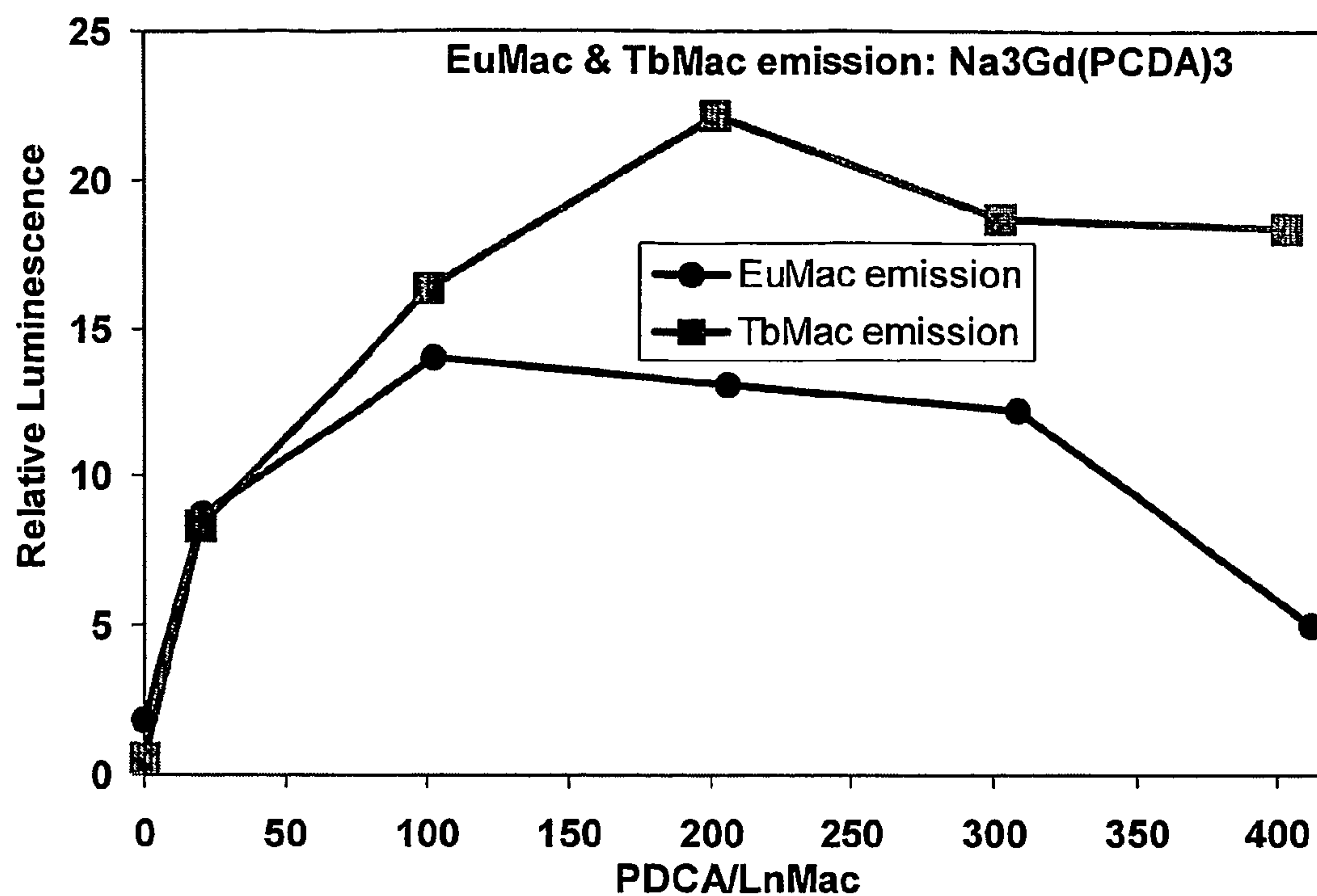
Figure 9b is a graph showing the effect of differing concentrations of \text{Na}_3\text{Gd}(\text{PDCA})_3 on the luminescence of two different lanthanide macrocycles.
