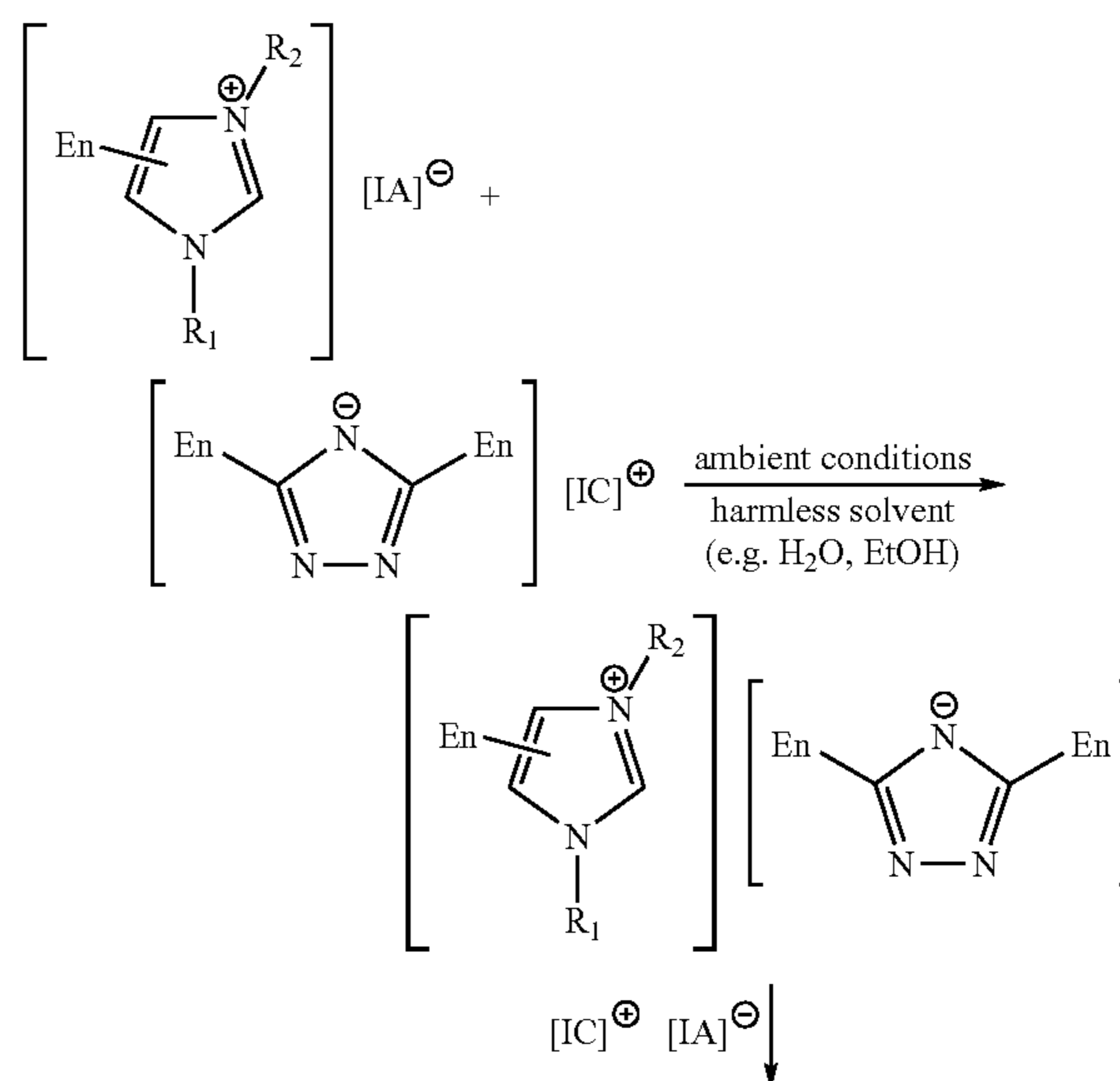
Scheme 1: Protocol 1
