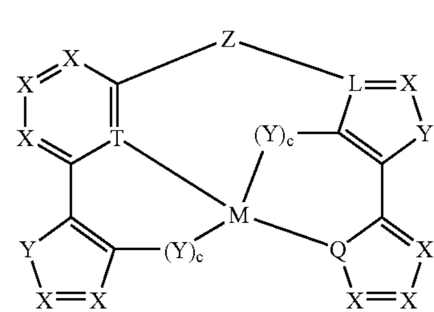
Compounds (26)
