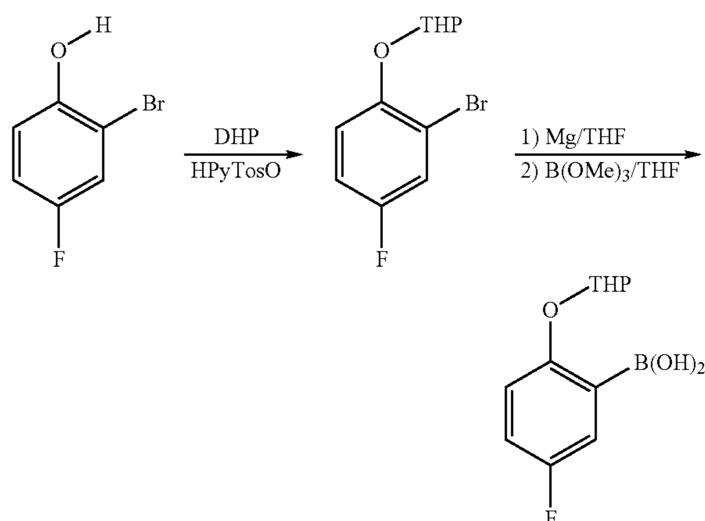
Scheme 6:
