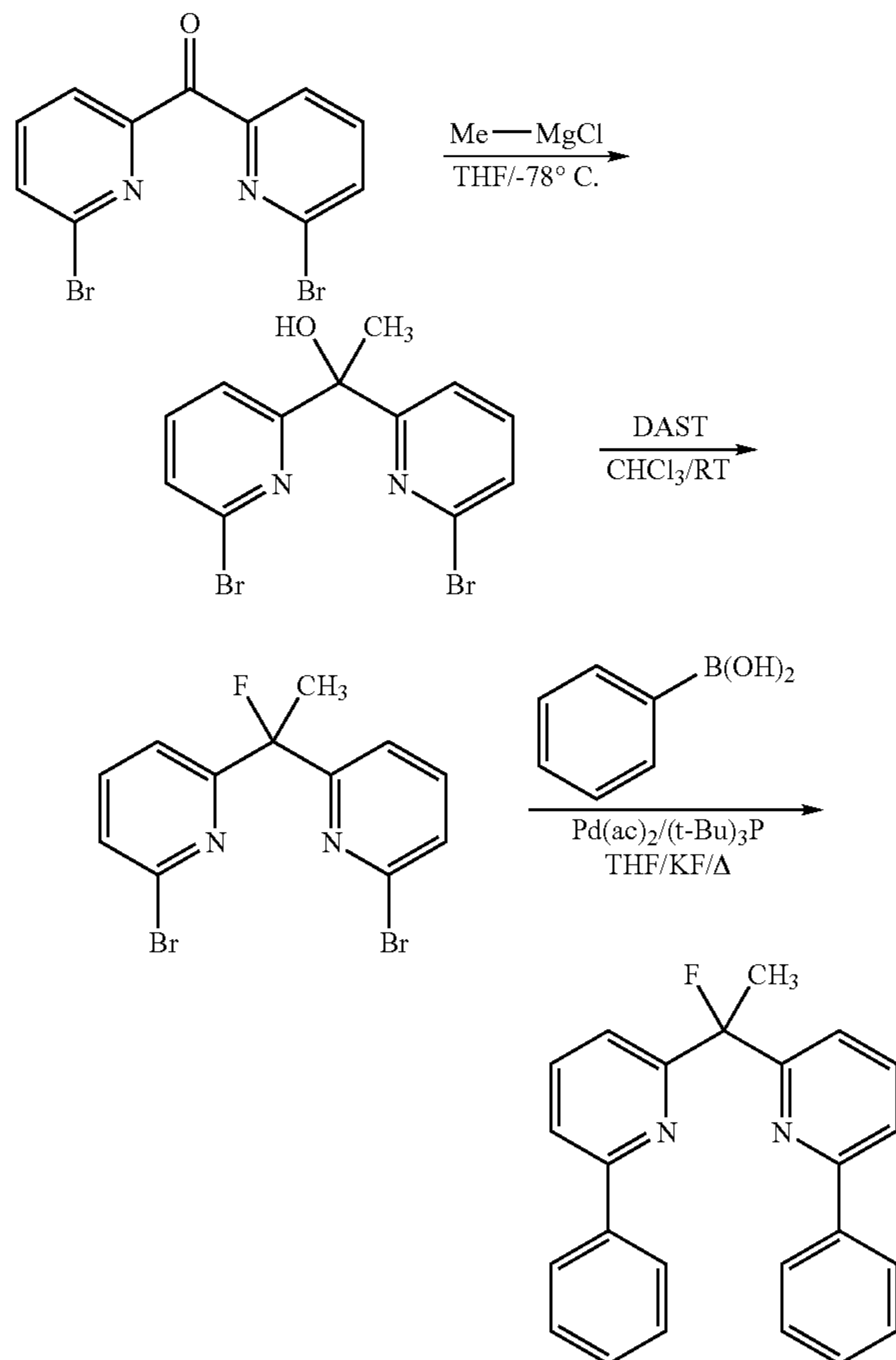
Scheme 5:
