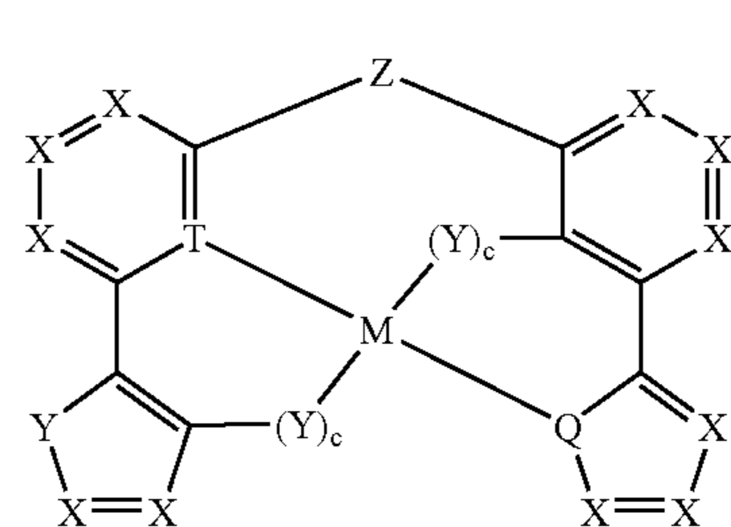
Compounds (23)
