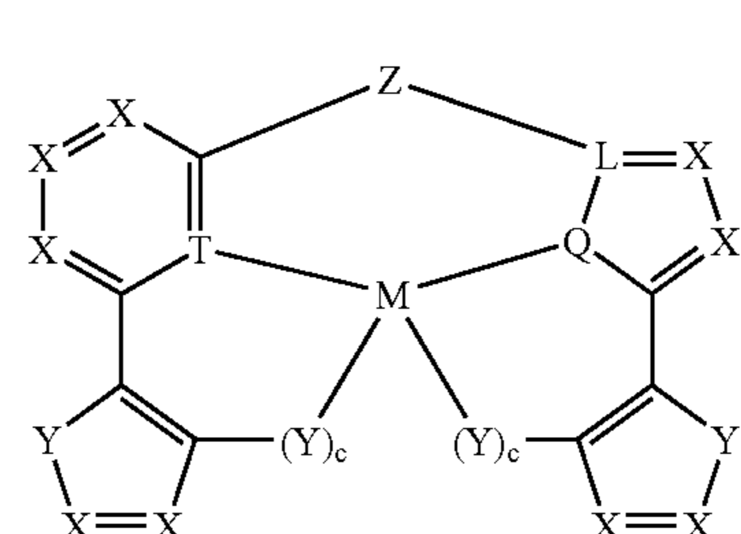
Compounds (25)
