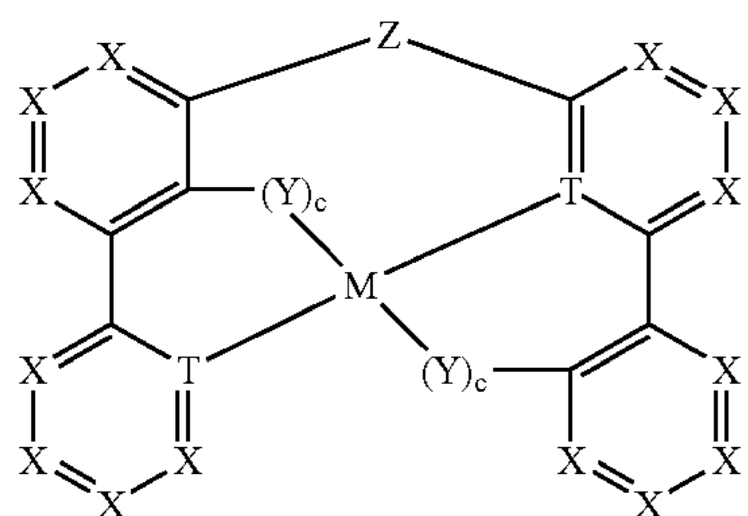
Scheme 2:
