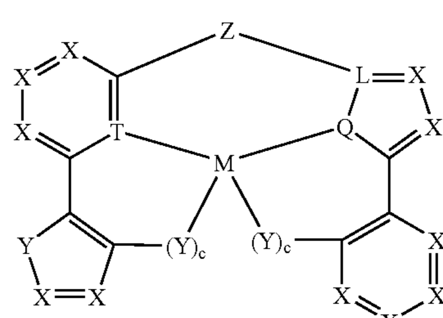
Compounds (22)
