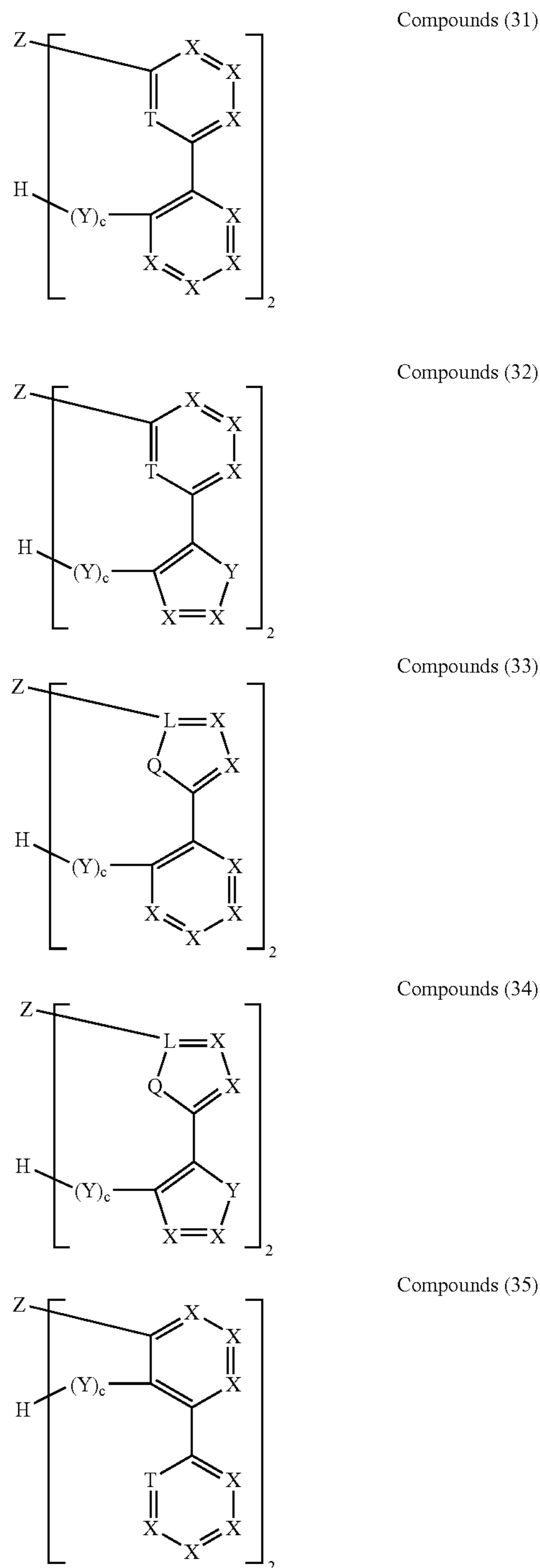
Scheme 4
