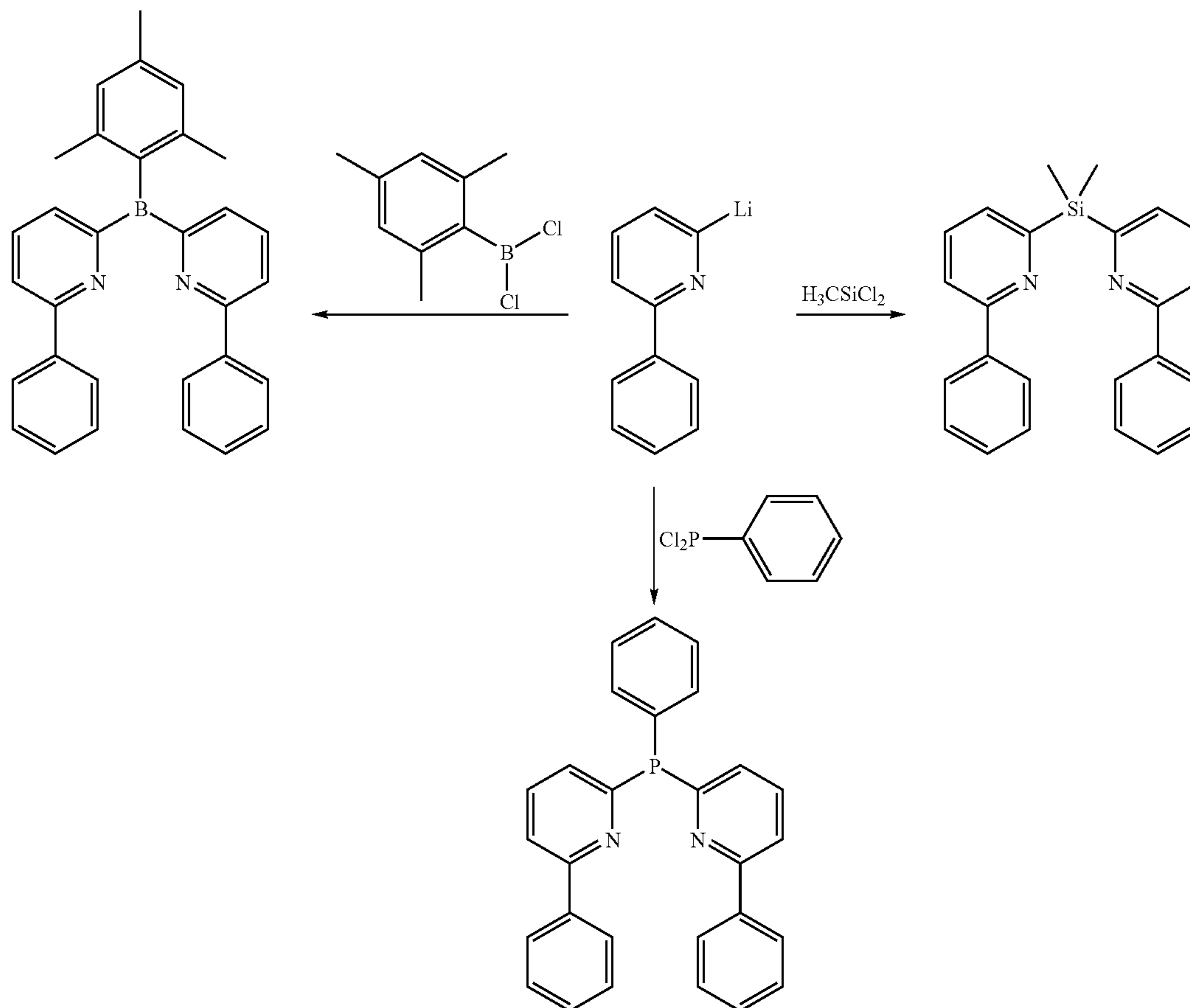
Scheme 8:
