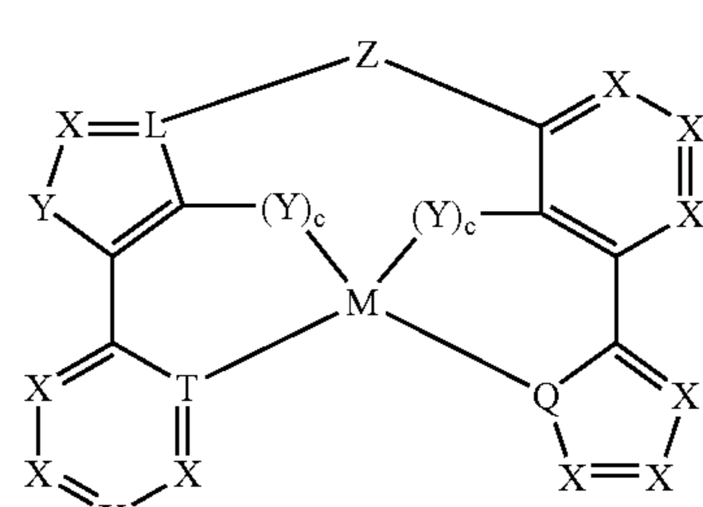
Compounds (24)
