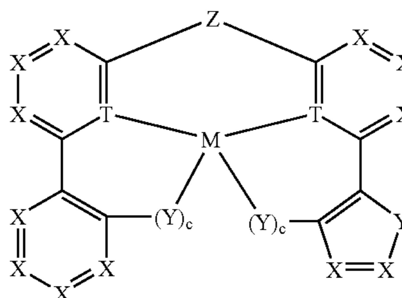
Scheme 3:
