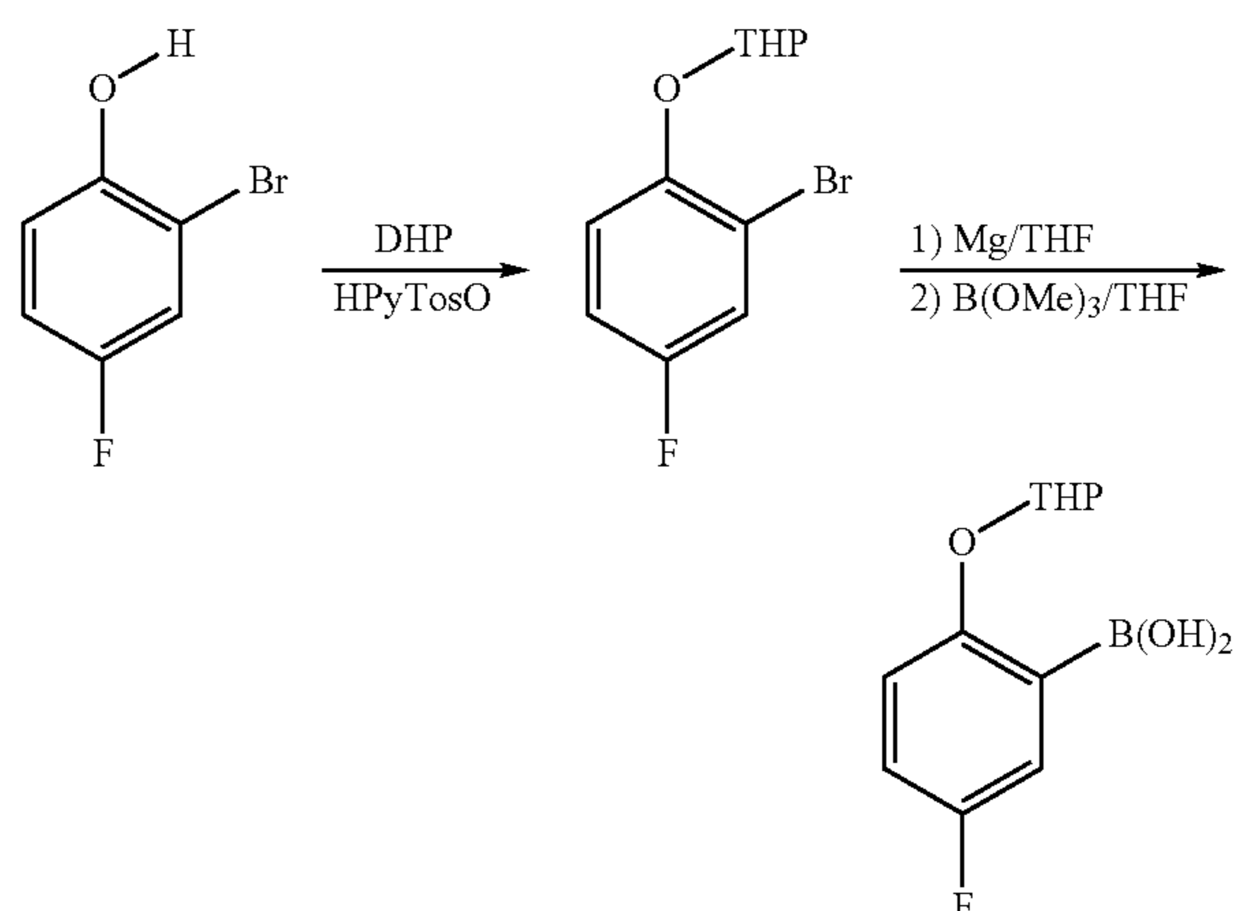
Scheme 6:
