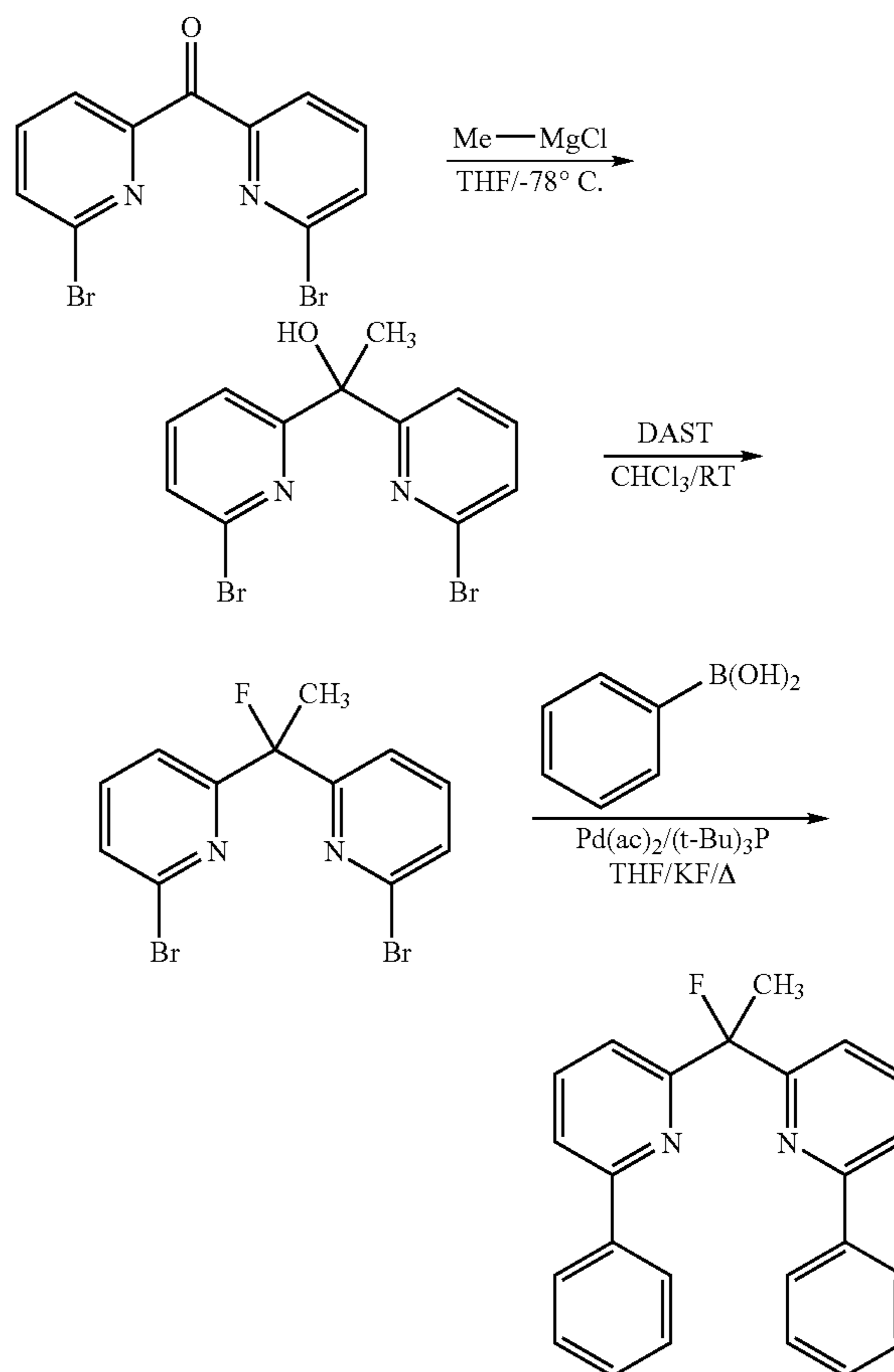
Scheme 5:
