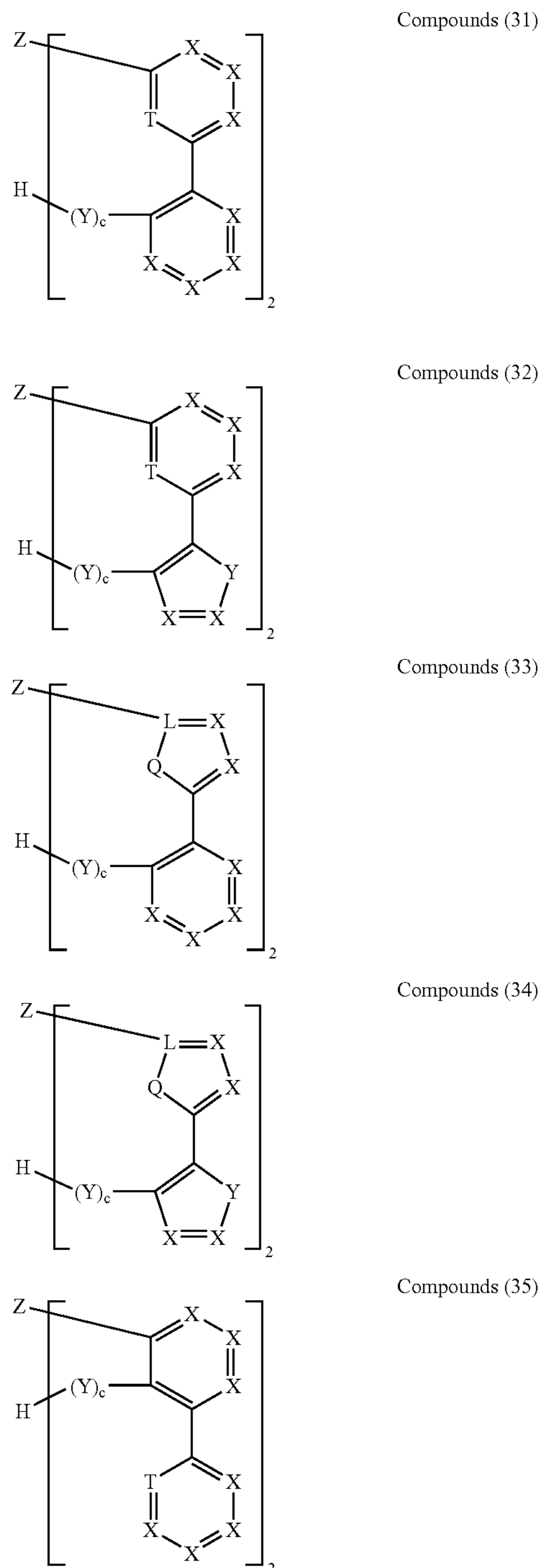
Scheme 4
