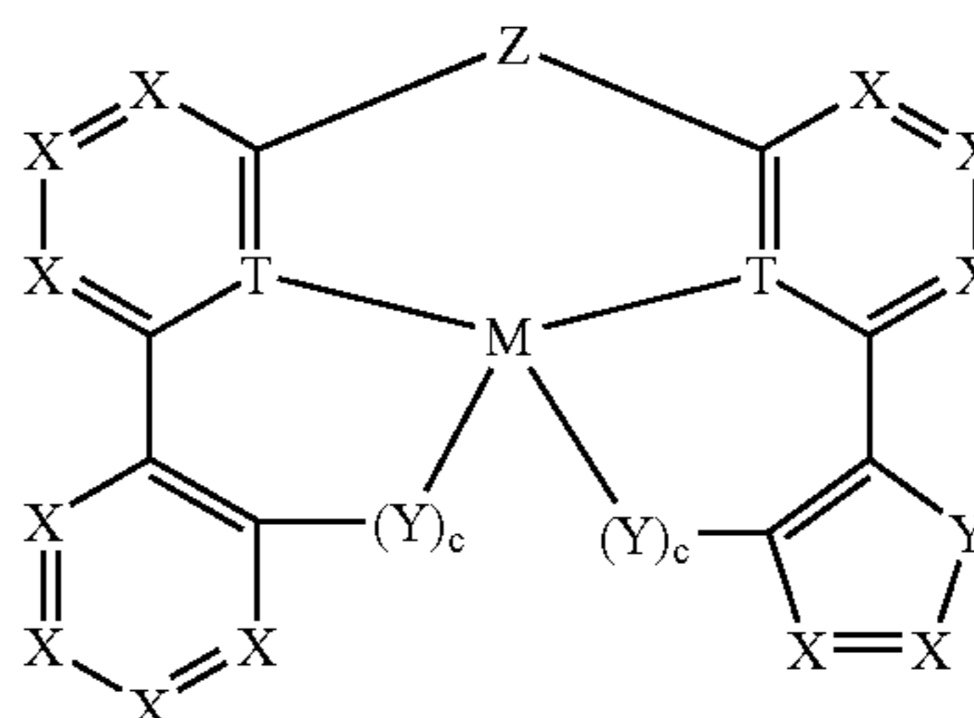
Scheme 3:
