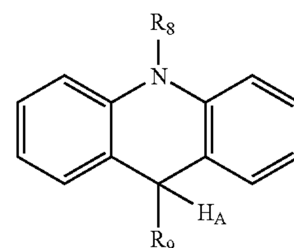
N-substituted acridan nitriles and carboxylate esters.
