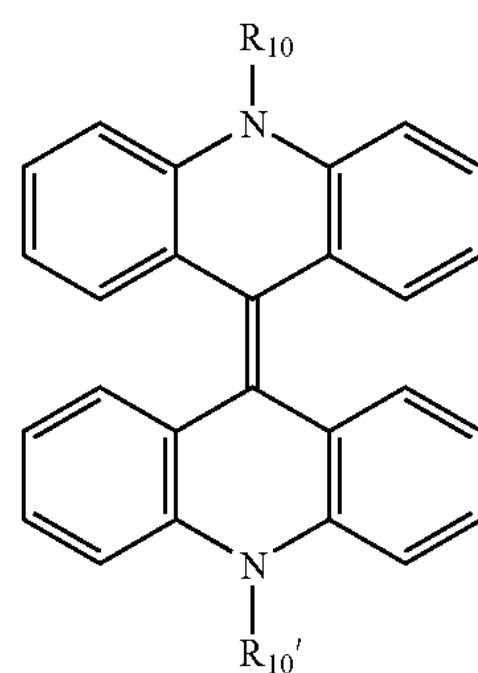
Biacridines.
