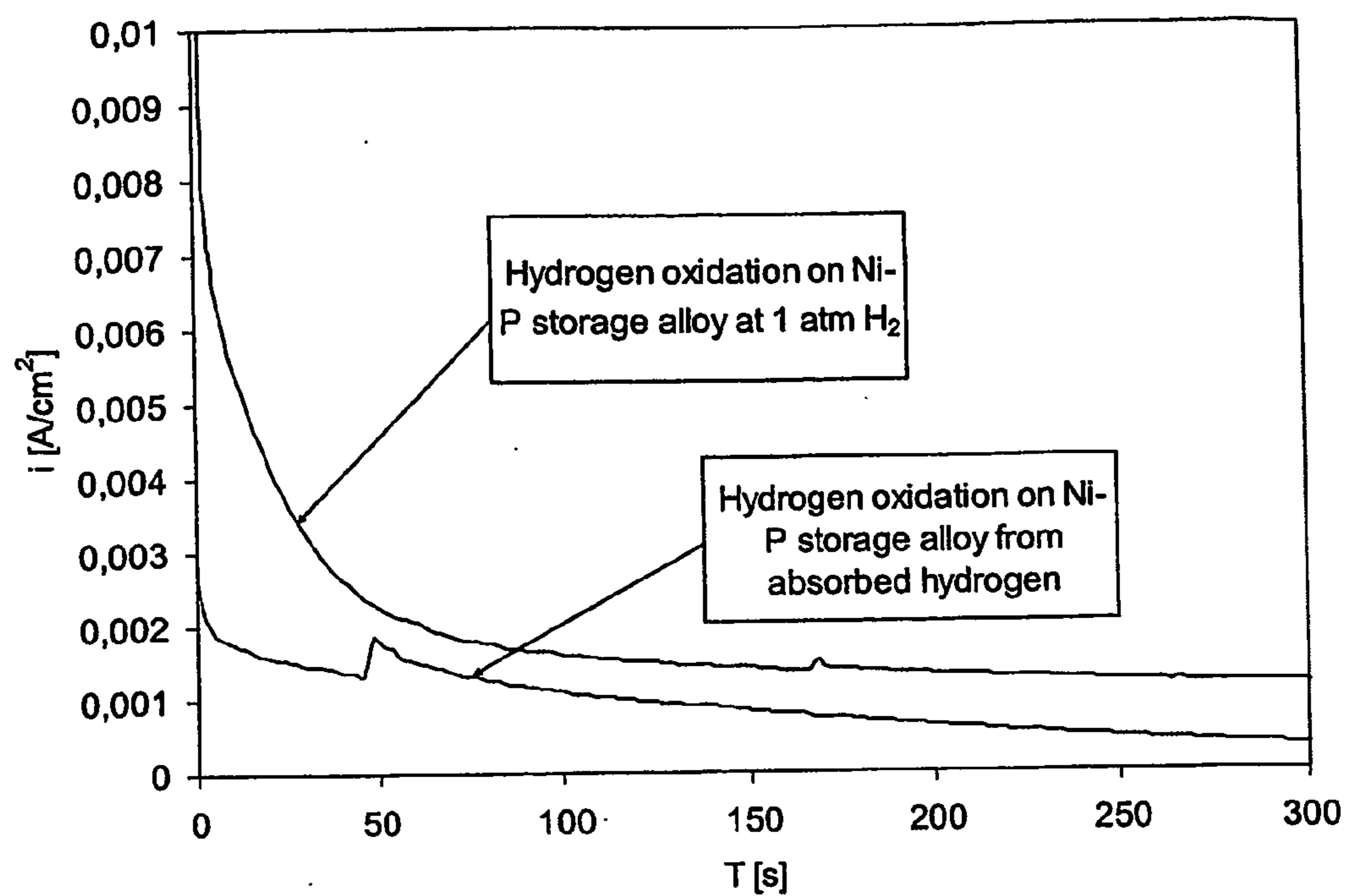
Figure 10. Hydrogen oxidation at overpotential of +100 mV in 6.6 M KOH on an electrode containing a Ni-P alloy that was deposited on Al and a carbon pore former. Corrosion of the Al produces hydrogen. This hydrogen was absorbed into the alloy. With anodic polarisation the absorbed hydrogen reacts on the surface. The current increases when additional hydrogen from the corrosion of an Al sheet is connected to the electrode
