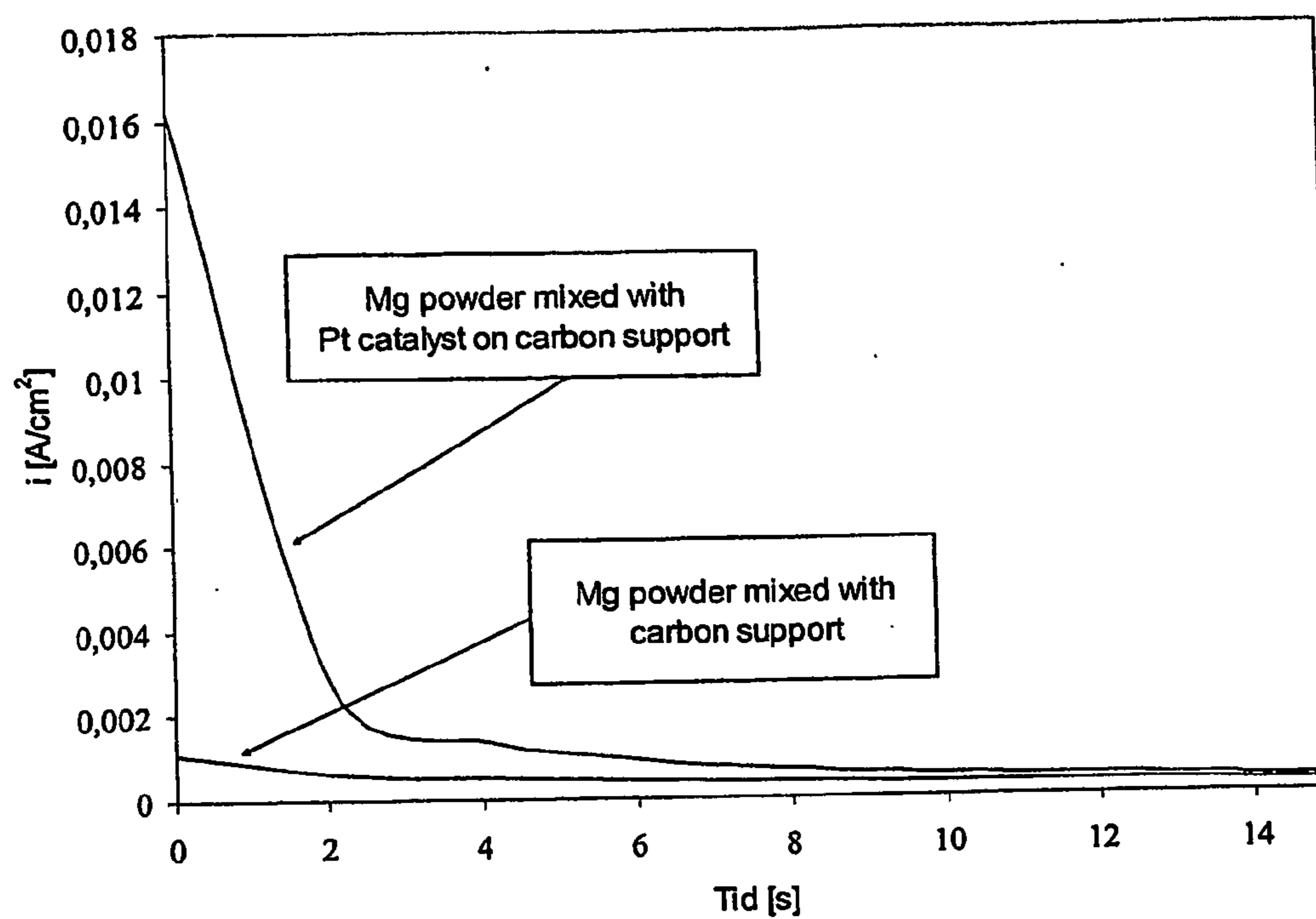
Figure 7. Current density for anodic polarisation of (+100 mV) of 20 wt% Mg mixed with 65 wt% carbon with and without 1 wt% Pt catalyst and 15 wt% PTFE. The electrolyte was 6.6 M KOH at 20 °C.
