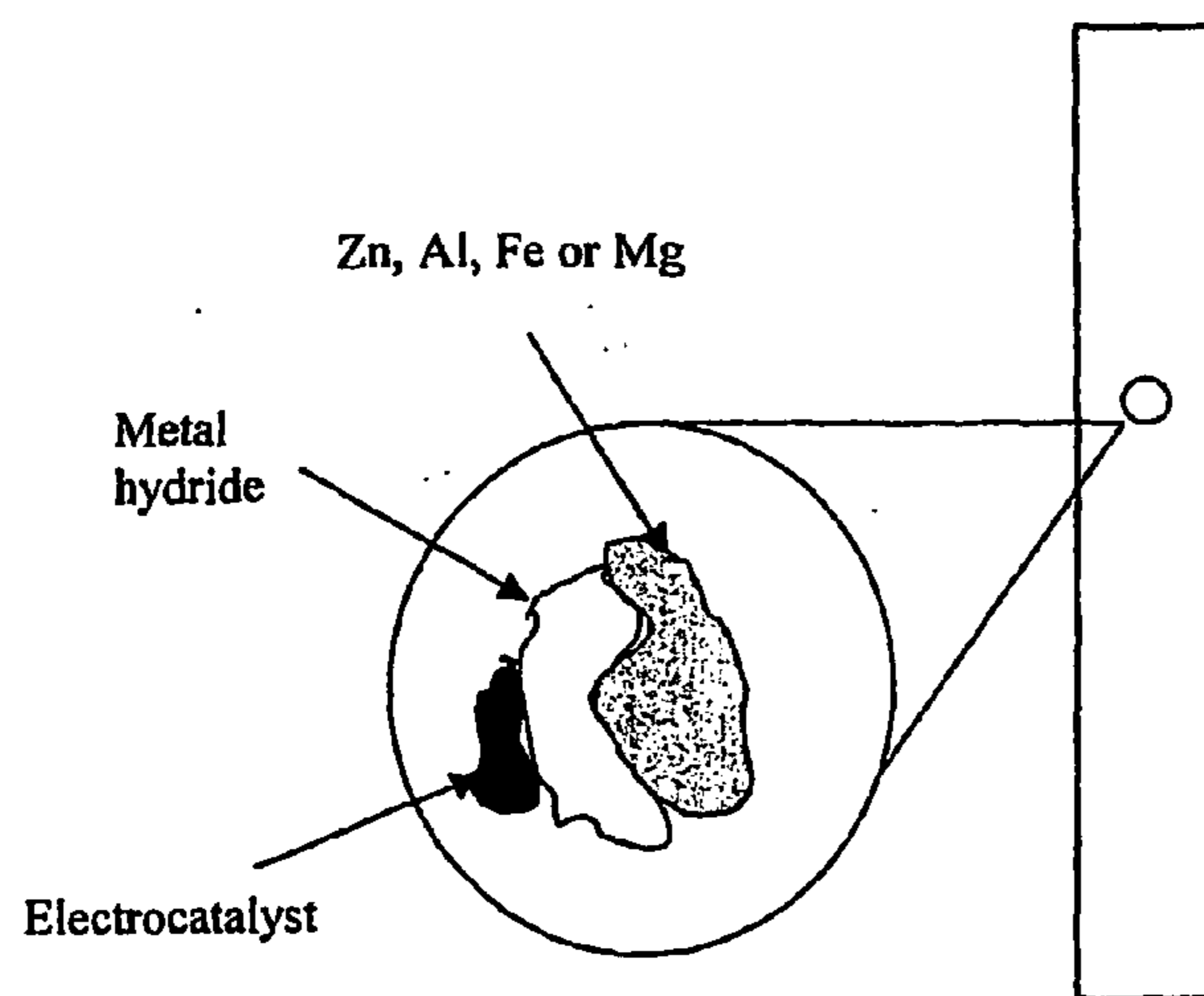
Figure 3. Illustration of electrode including the energy carrier (high energy density metals), the hydrogen absorber (metal hydrides) and the electrocatalyst.
