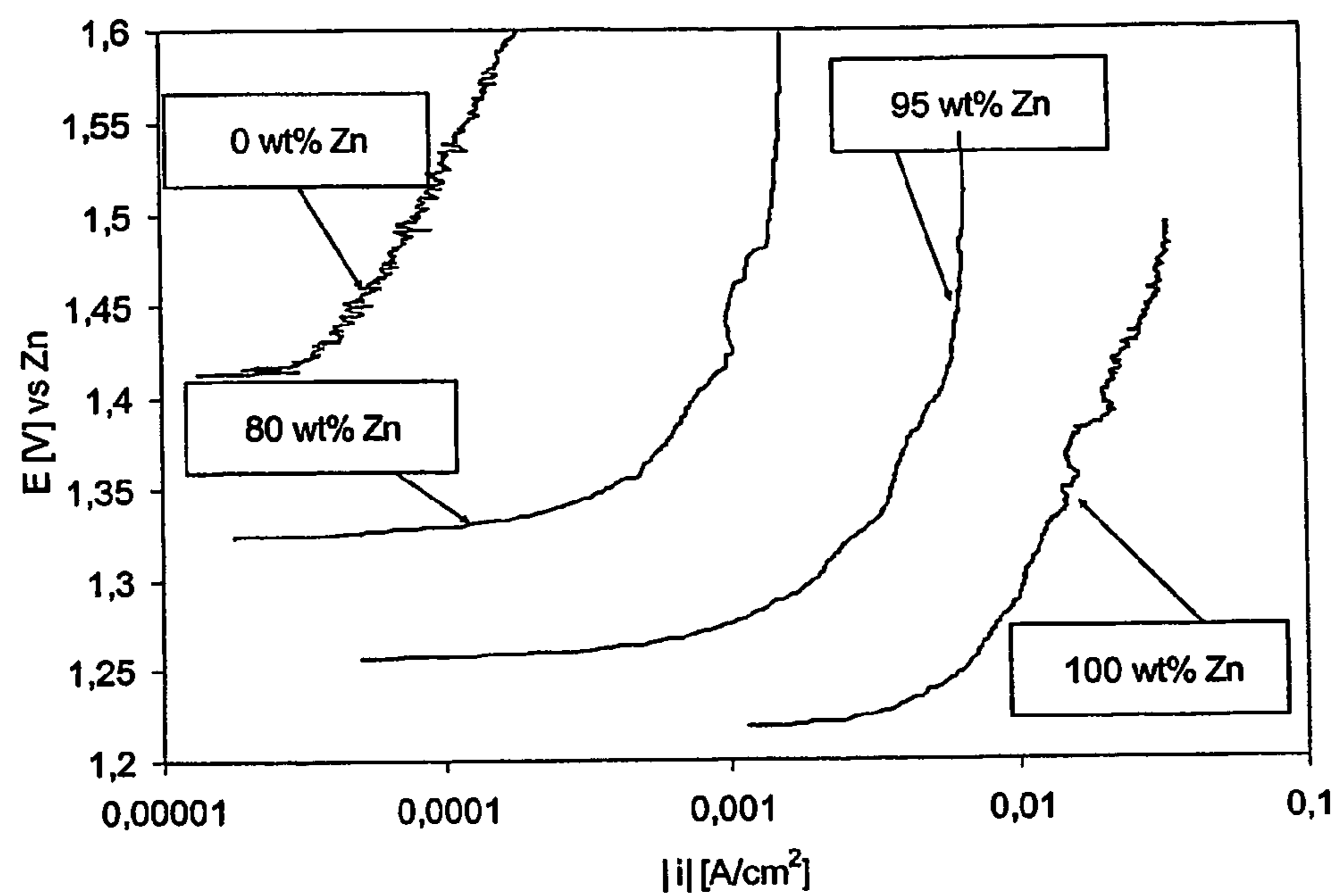
Figure 9. The rate of hydrogen oxidation in 6.6 M KOH at 20 °C on a PTFE bound carbon electrode with 1 wt% Pt catalyst on the carbon support. A hydrogen producing Zn electrode was pressed into the carbon electrode, however, separated by a isolating sheet that allowed gas diffusion. Hydrogen formed by corrosion of Zn reacts on the Pt catalyst of the carbon electrode. The amount of Zn in the Zn electrode was varied between 0 and 100 wt%.
