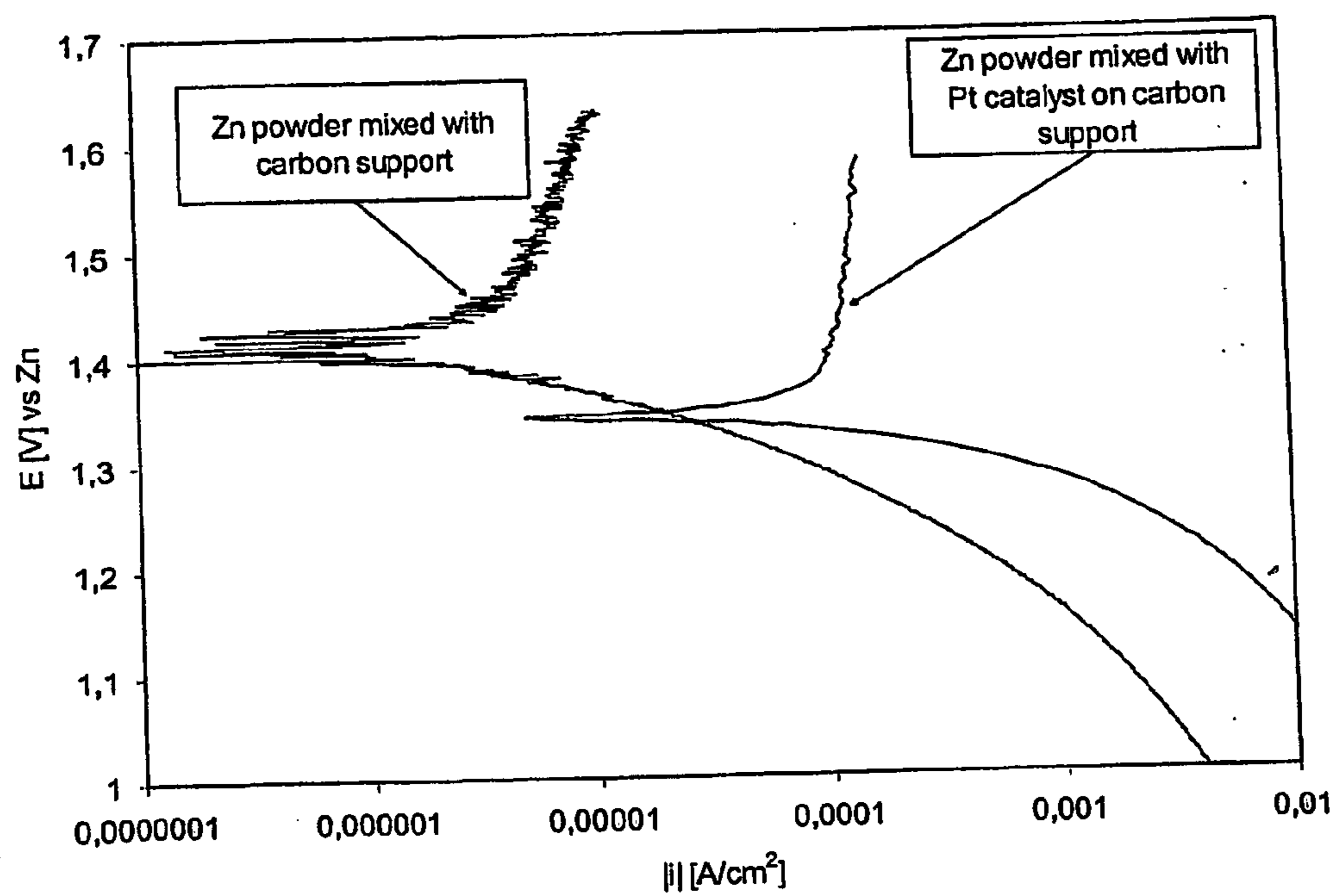
Figure 8. Polarisation sweeps of electrodes prepared from 20 wt% Zn, 65 wt% carbon support with or without 1 wt% Pt catalyst and 15 wt% PTFE. The electrolyte was 6.6 M KOH at 20 °C.
