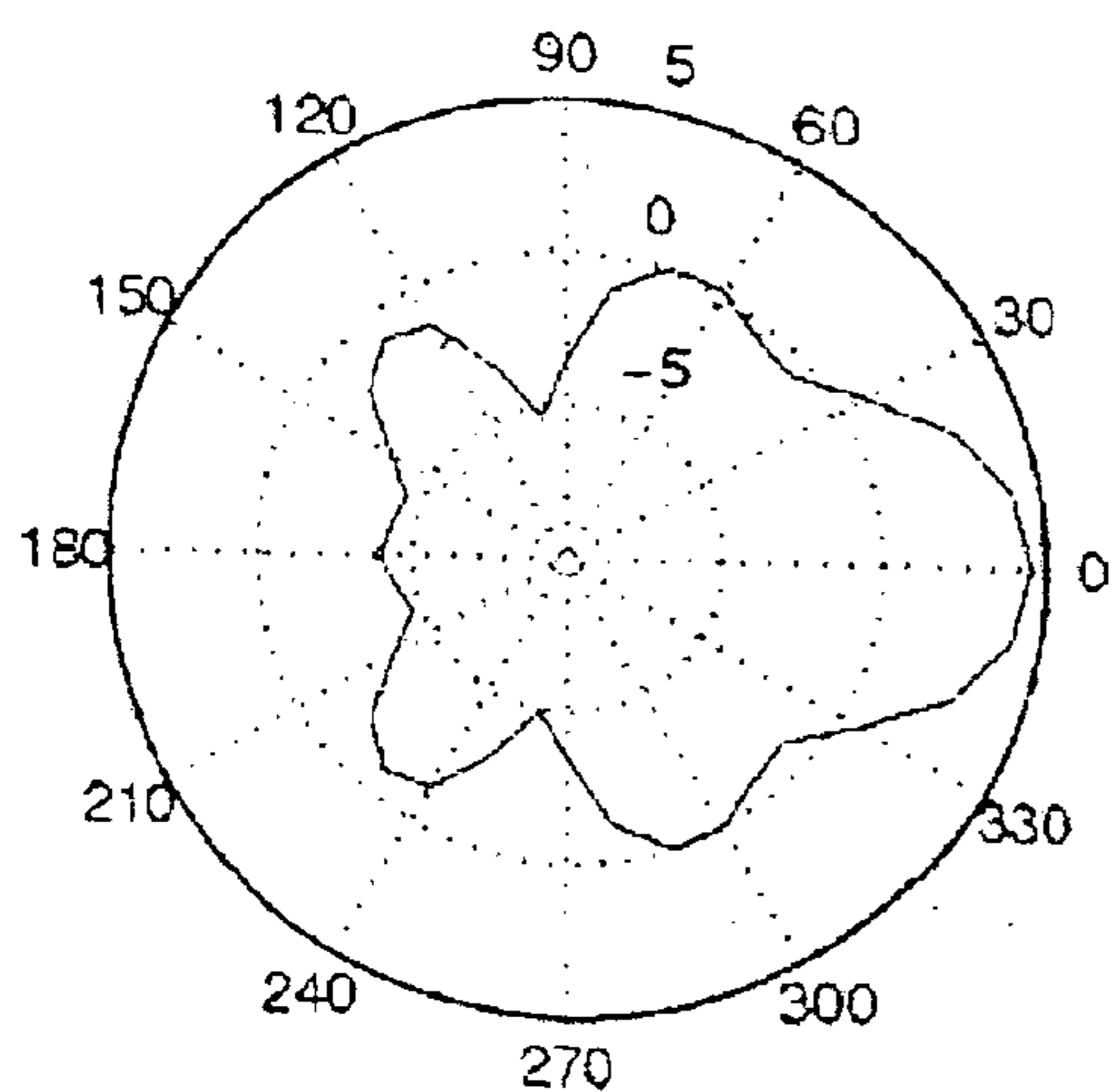
horizontal radiation pattern
