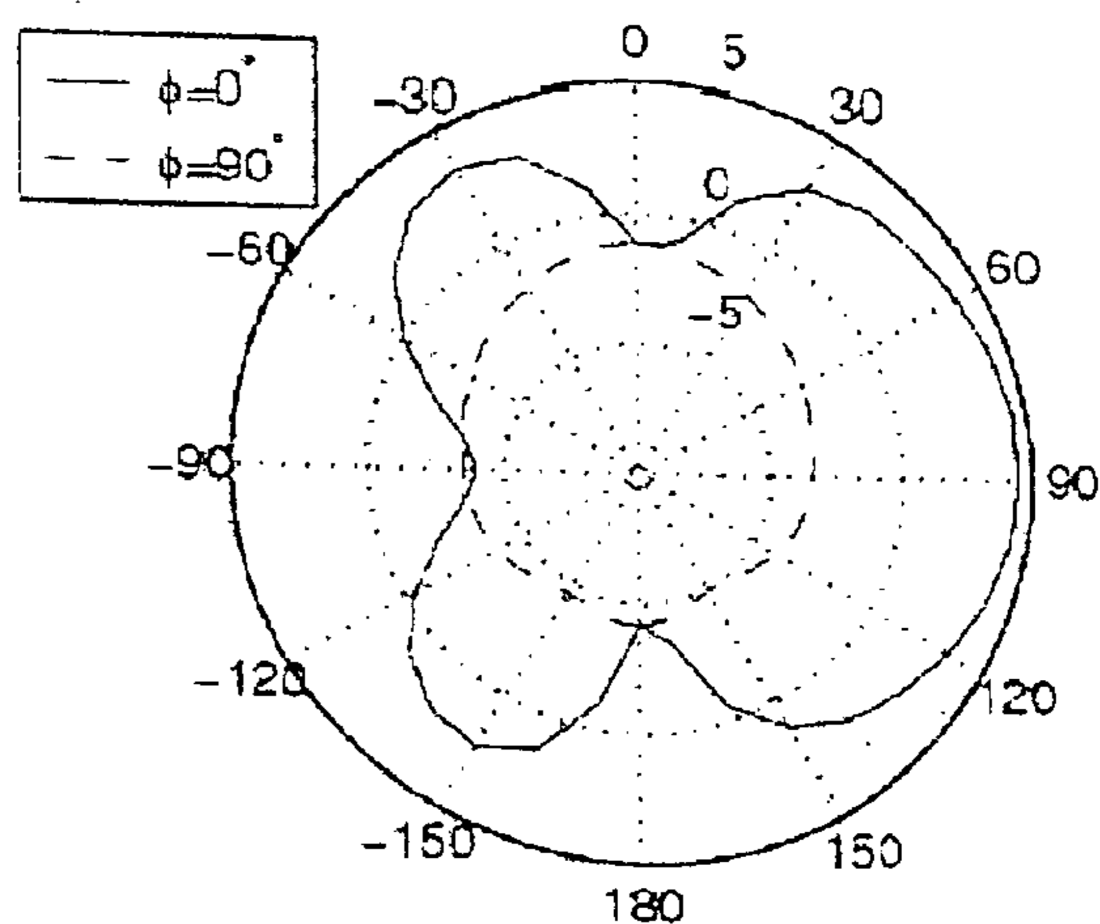
vertical radiation pattern
