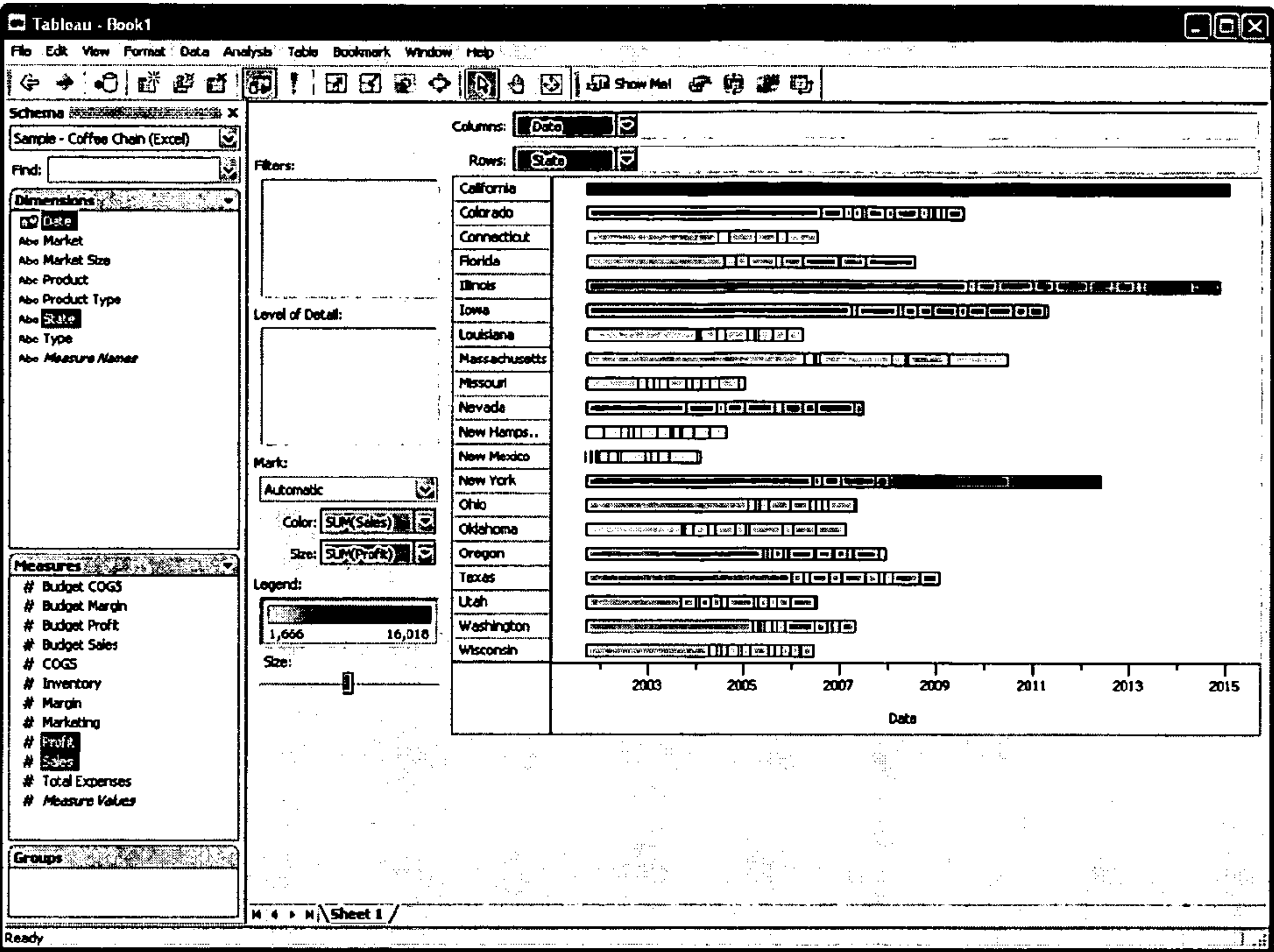
Figure 8i (Gantt)
