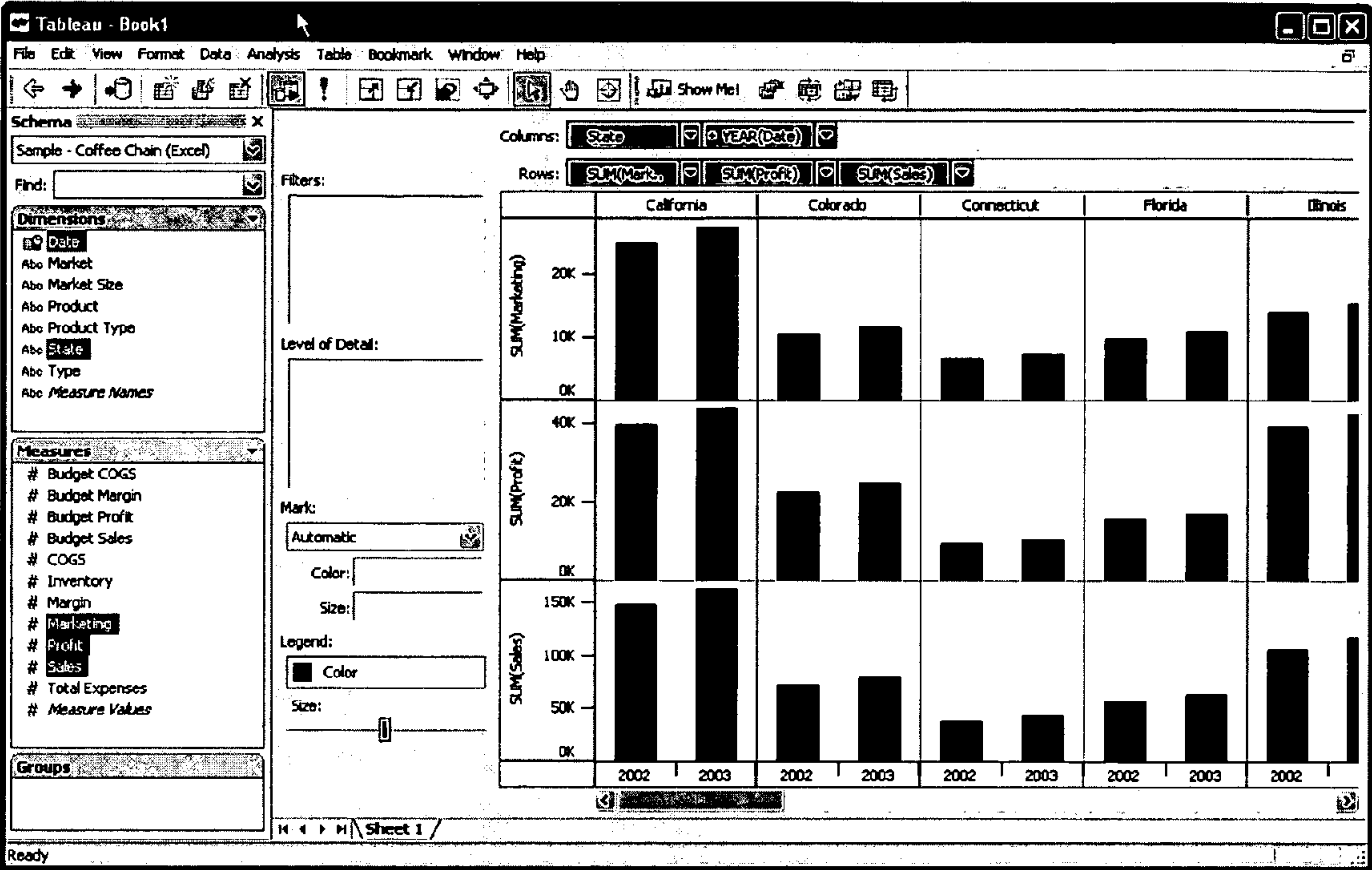
Figure 8c (Side-By-Side Bar)
