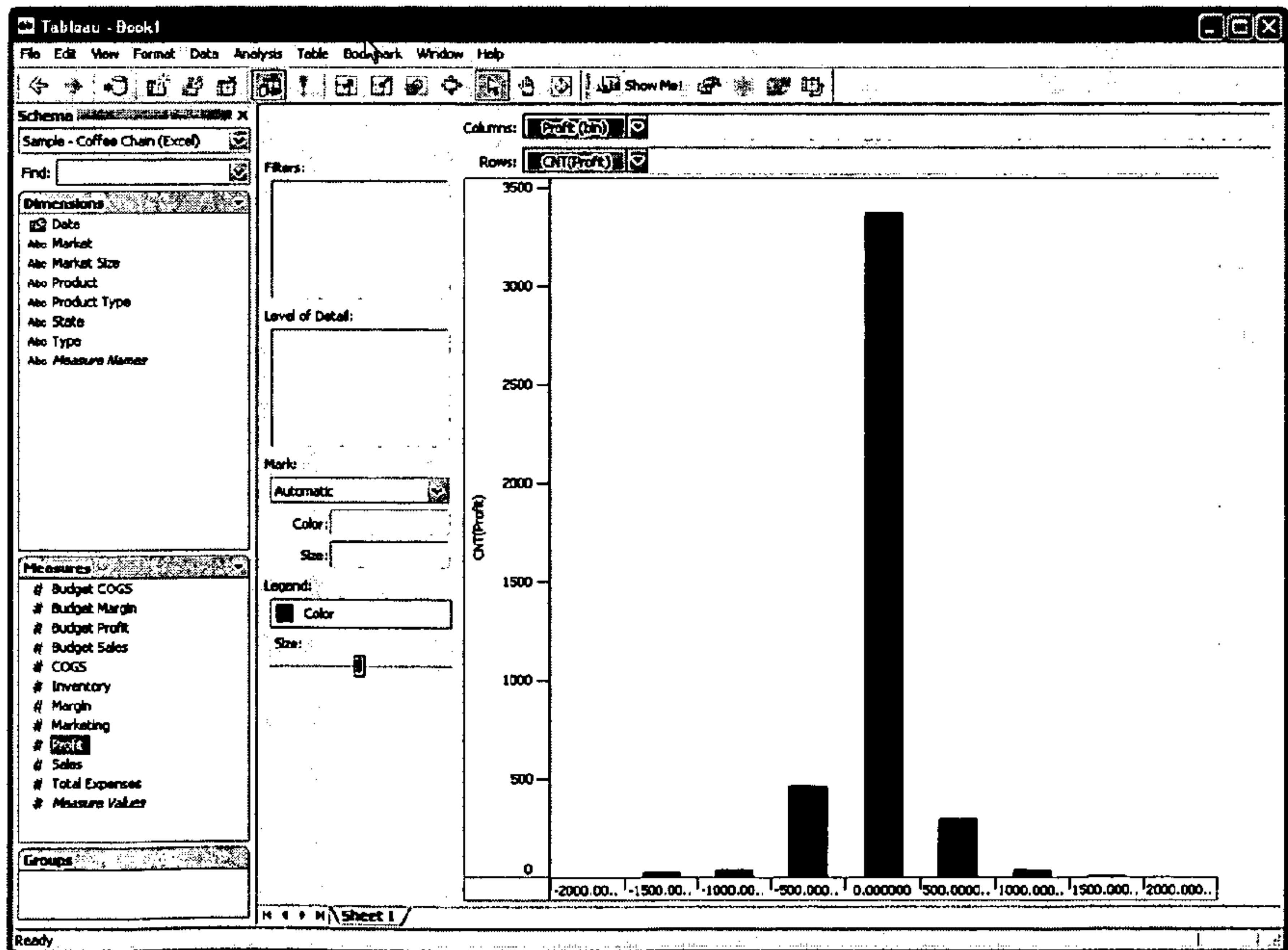
Figure 8l (Histogram)
