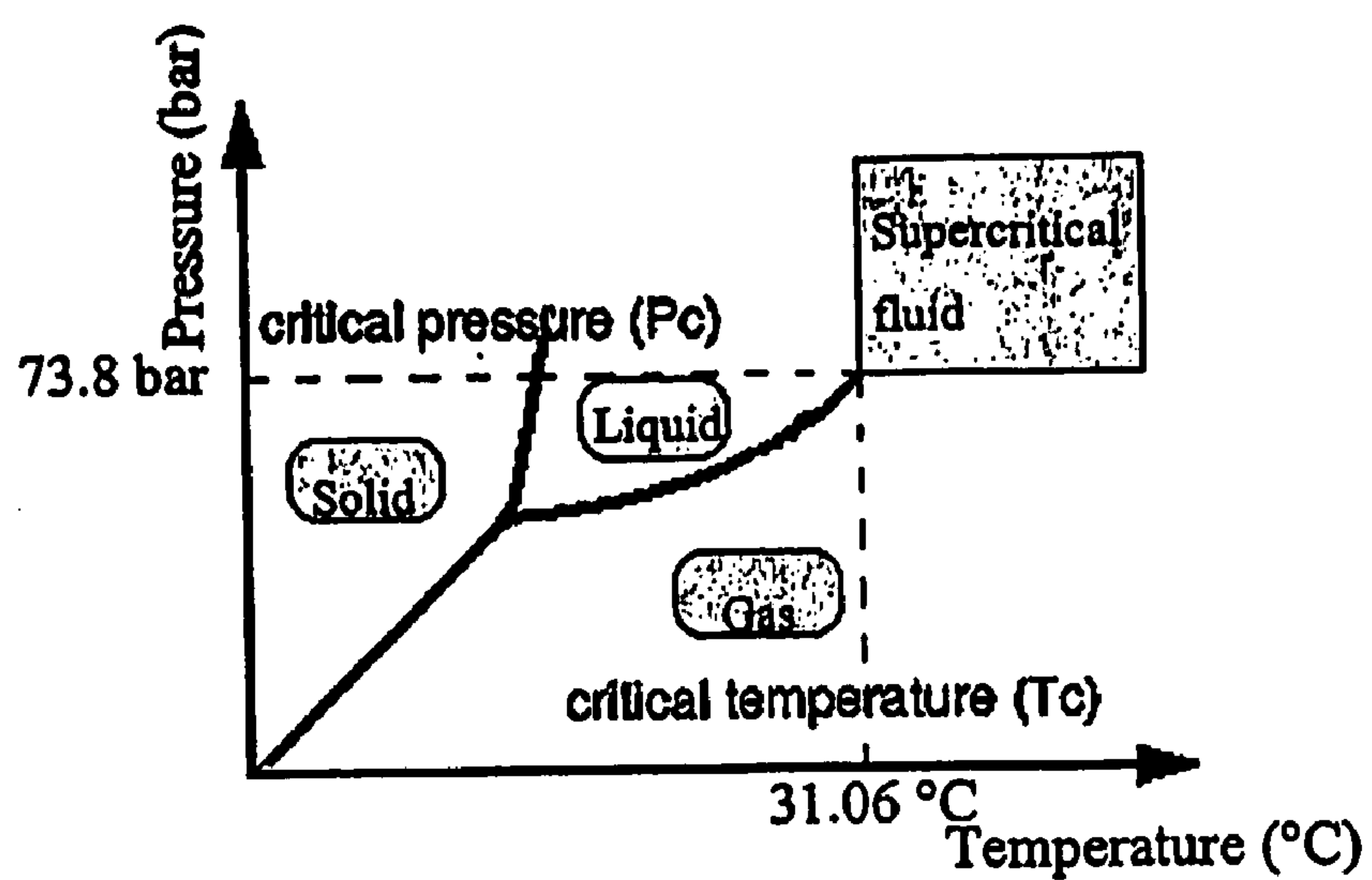
Fig 13. Pressure-temperature diagram of CO 2
